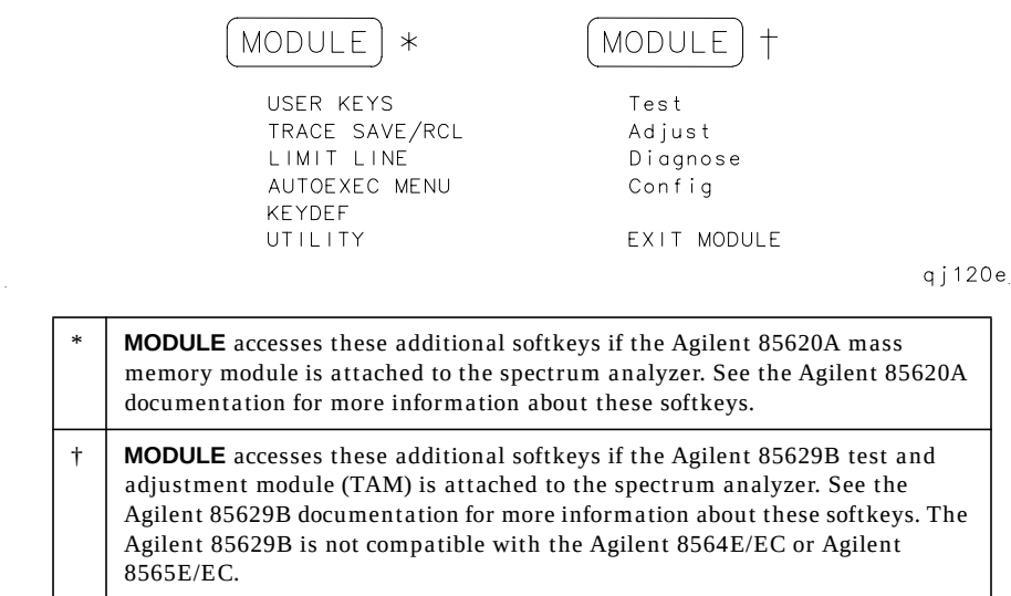
Figure 3-18 MODULE Key Menus
