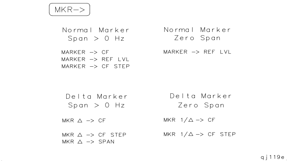
Figure 3-17 MKR-> Key Menu
