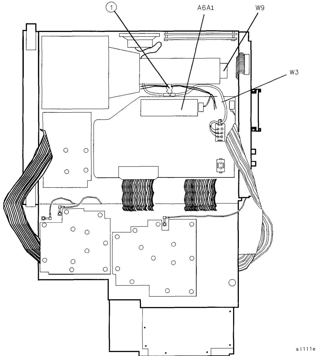
Figure 4-24. W3 Dress and Connection to A6 Power Supply
