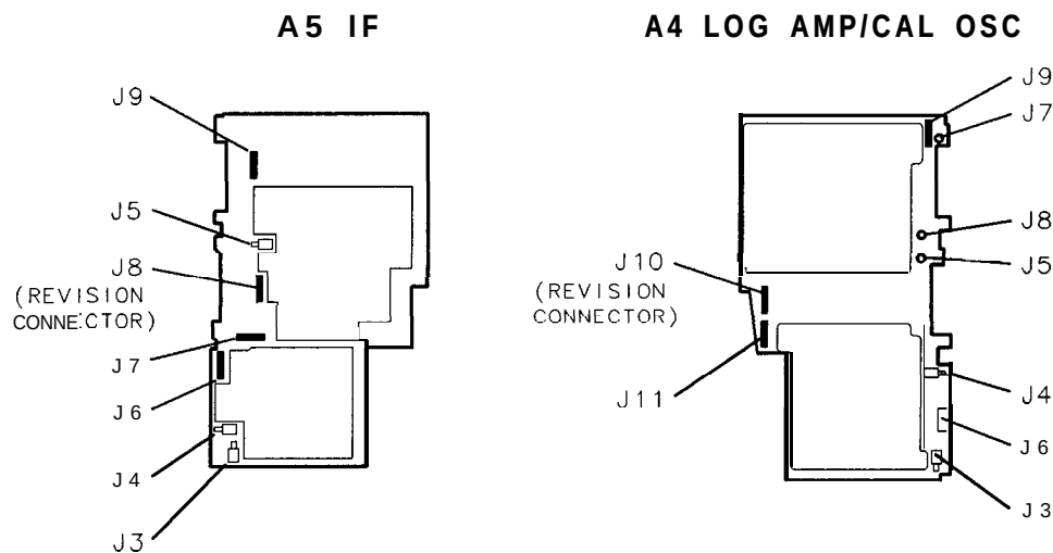
Figure 9-1. A4 and A5 Test Connectors
