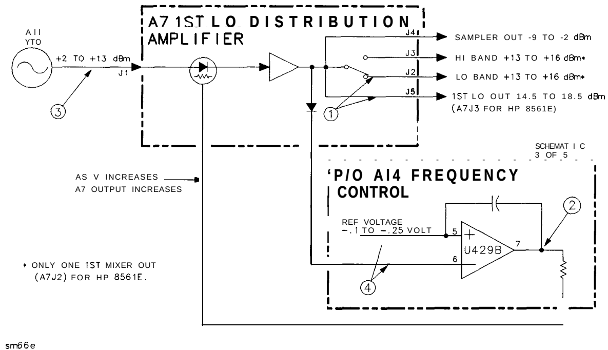
Figure 12-3. A7 First LO Distribution Amplifier Drive
