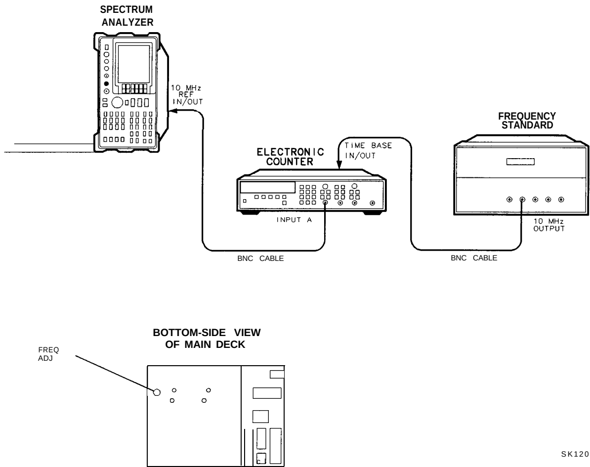
Figure 2-19. 10 MHz Reference Adjustment Setup and Adjustment Location
