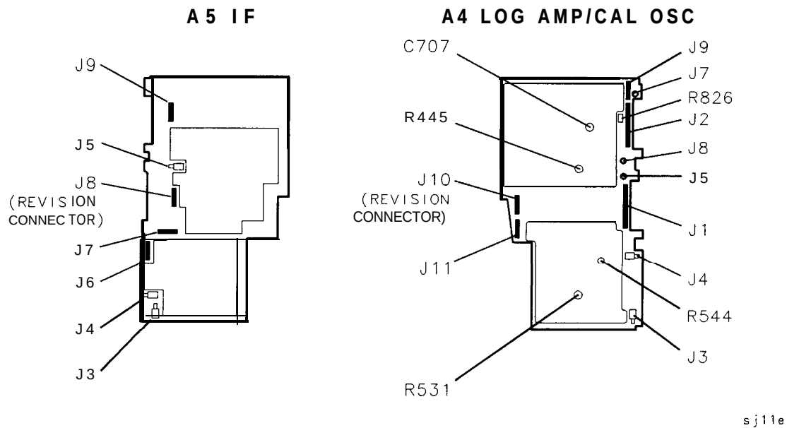
Figure 2-8. IF Amplitude Adjustment Locations
