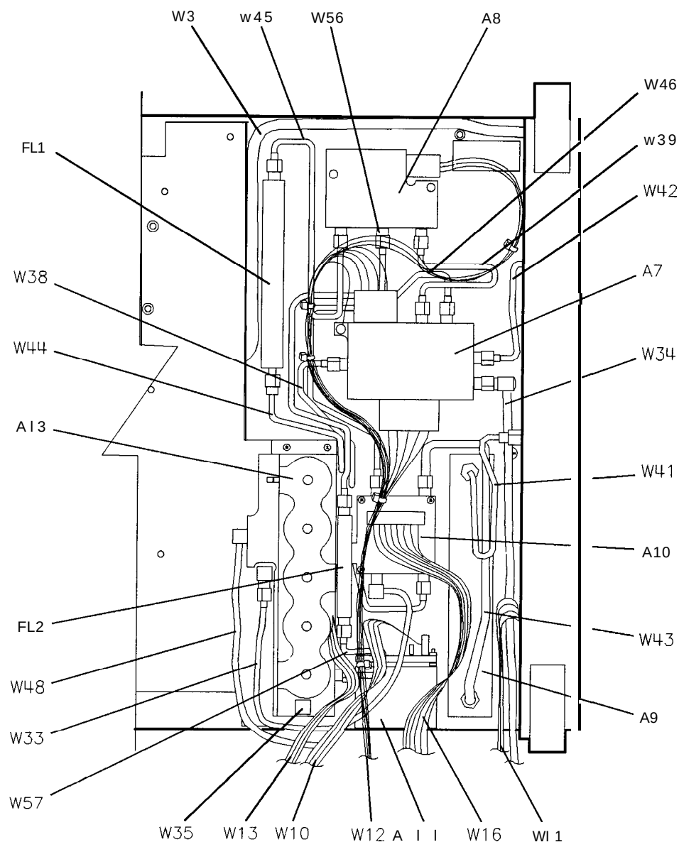
Figure 6-6. HP 6562E Front End
