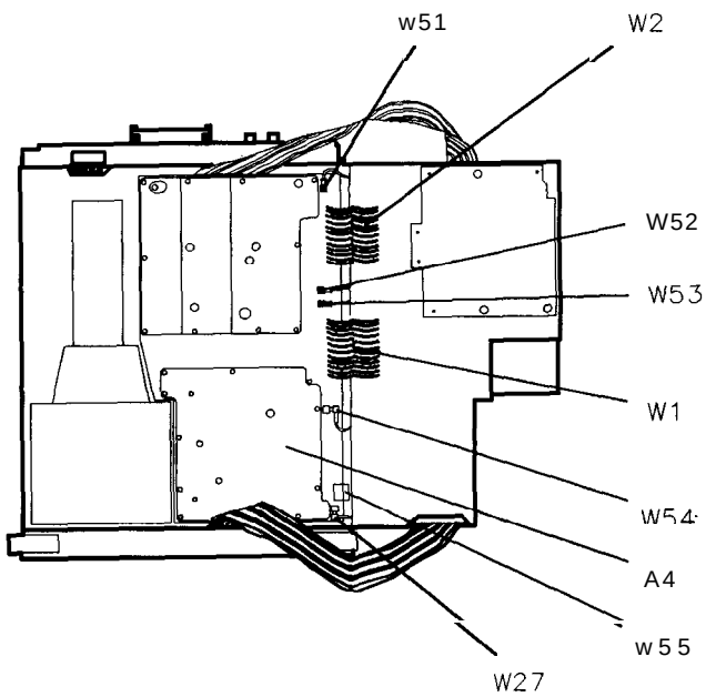
Figure 6-3. Top View (A2 and A3 Unfolded)
