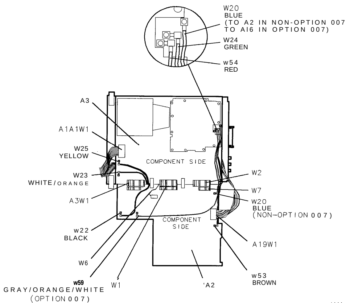
Figure 6-2. Top View (A2 Unfolded)
