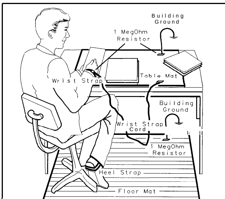
Figure I-I. Example of a Static-Safe Workstation
