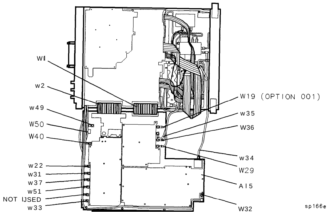
Figure 6-5. Bottom View (AI5 Unfolded)
