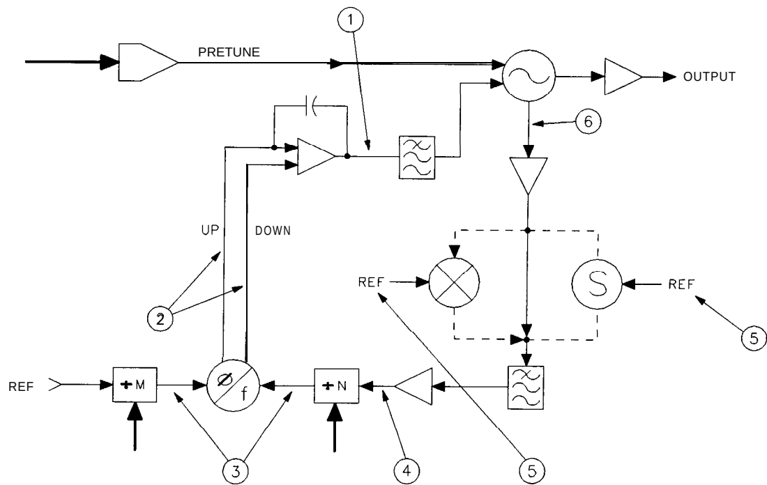
Figure 11-6. Unlocked PLL
