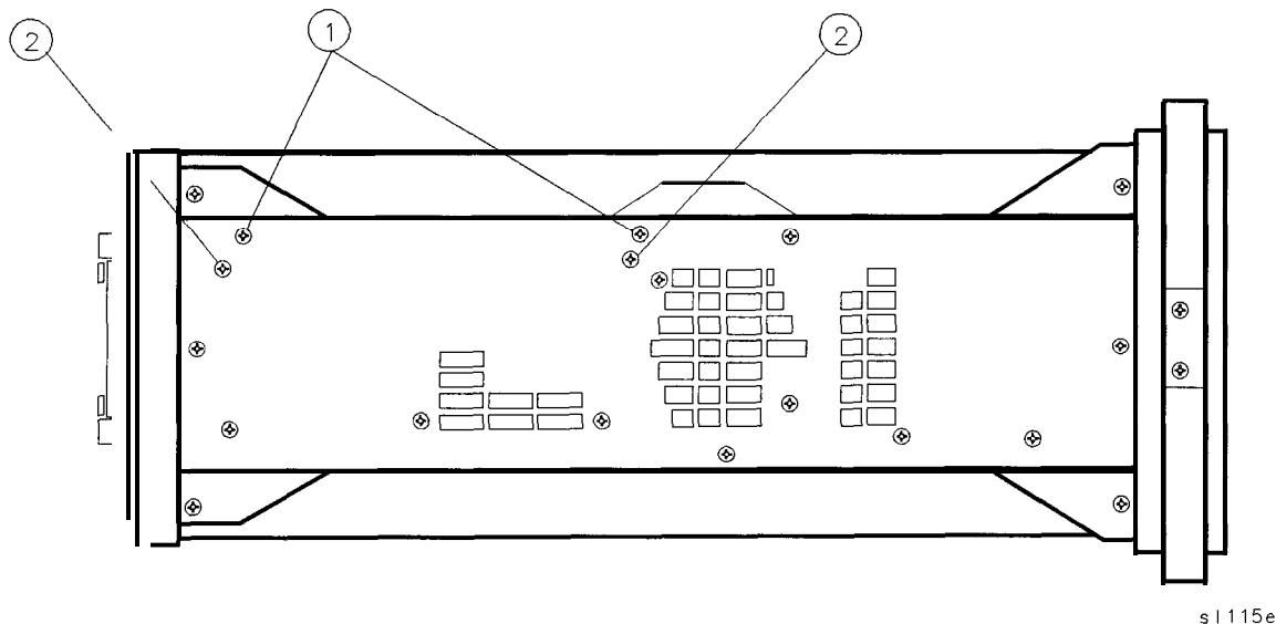
Figure 4-20. A16 and A17 Mounting Screws
