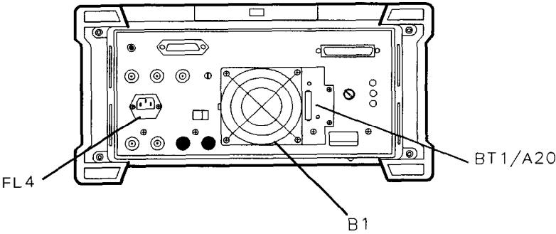
Figure 6-9. Rear View
