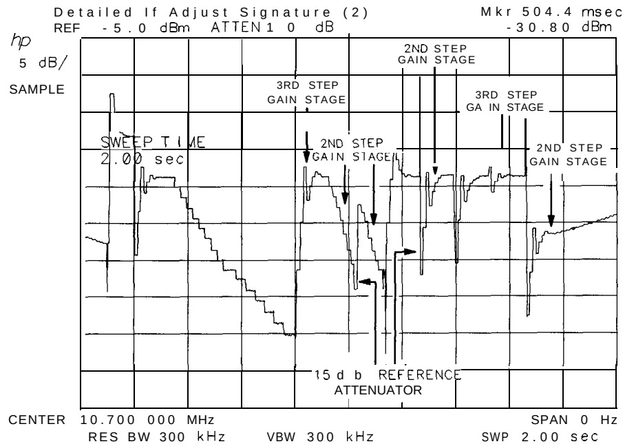
Figure 9-5. Detailed IF Adjust Signature (2)
