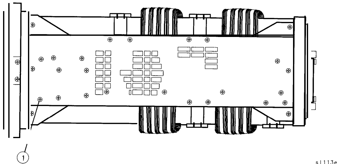
Figure 4-15. A9 Mounting Screw at Right Side Frame
