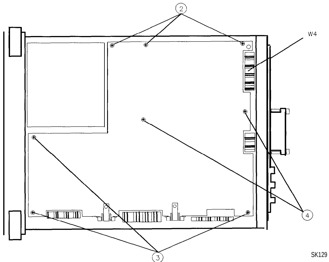
Figure 4-7. A2, A3, A4, and A5 Assembly Removal
