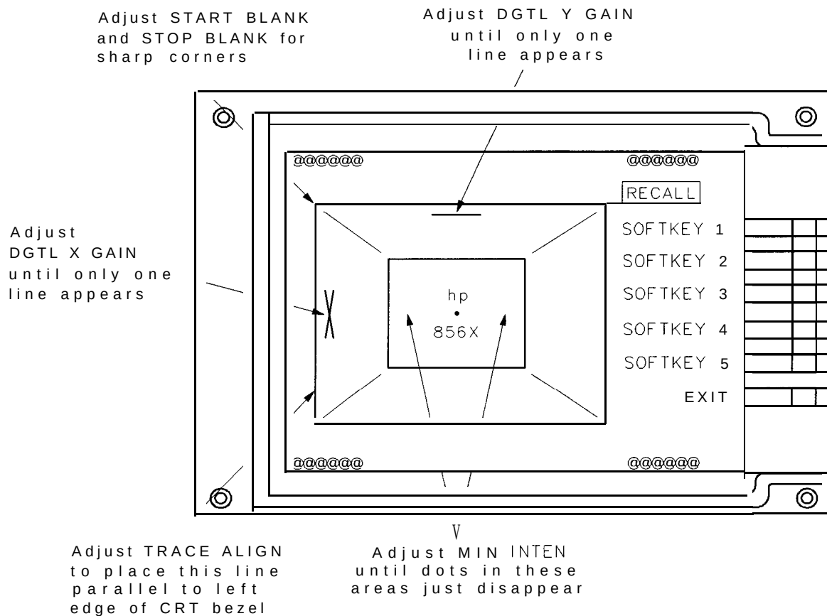
Figure 2-3. CRT Adjust Pattern
