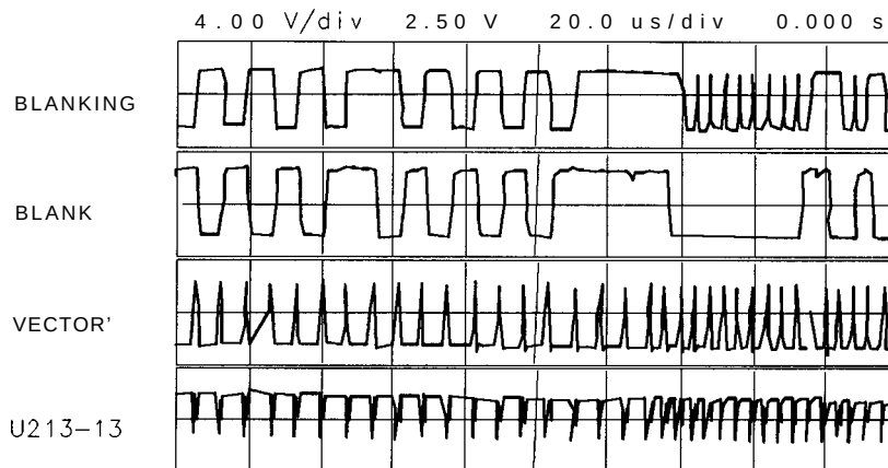
Figure 10-3. Blanking Waveforms
