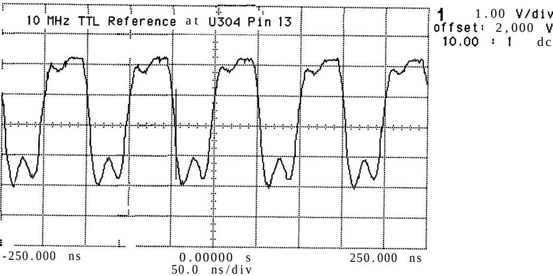
1 2.640 V Figure 12-7. 10 MHz TTL Reference at U304 Pin 13
