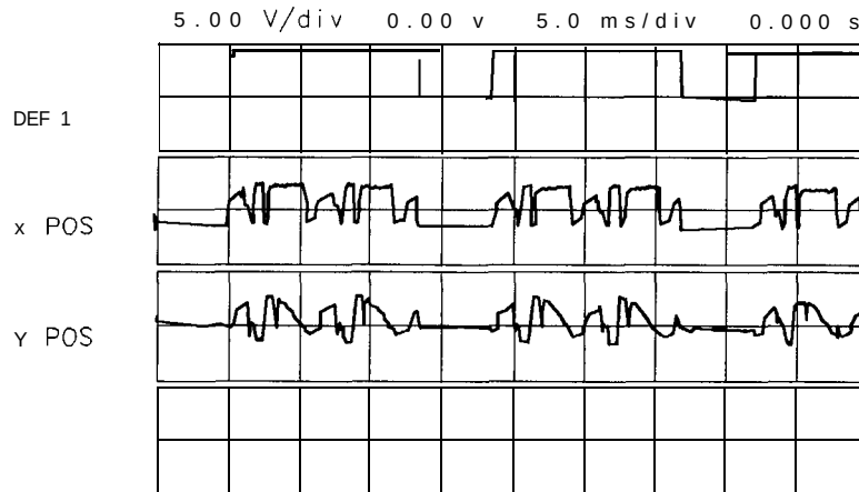
Figure 10-I 1. DEF1 Synchronization
