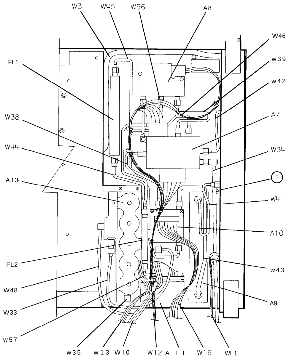
Figure 4-14. HP 6562E Assembly Locations
