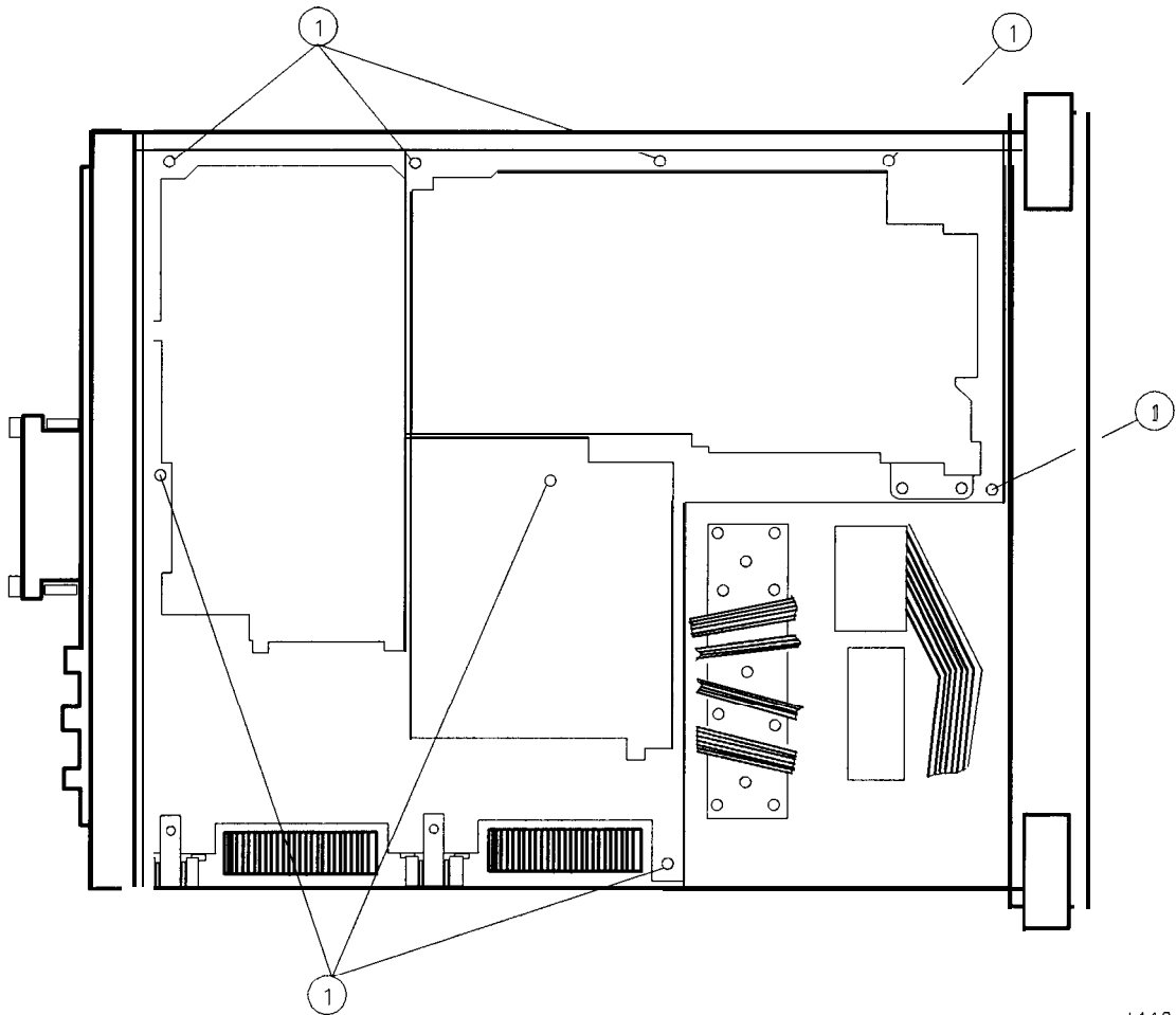
Figure 4-18. AI4 and AI5 Assembly Removal
