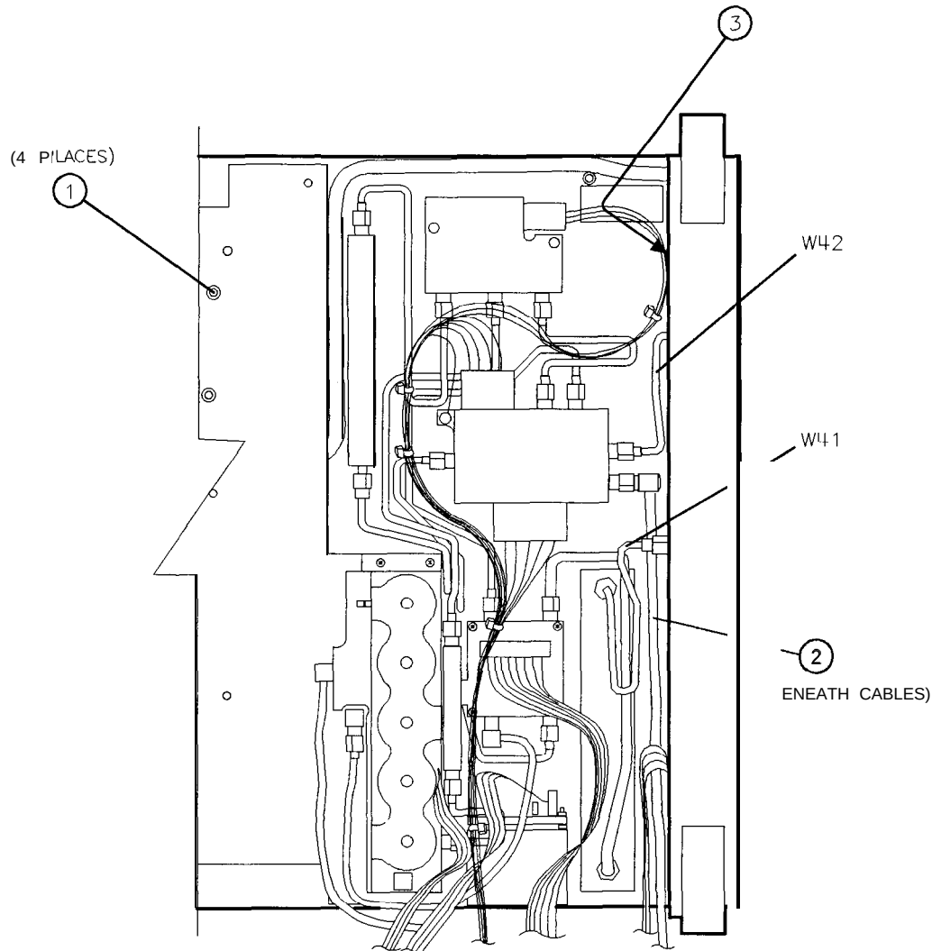
Figure 4-3. A9, A18, and Line-Switch Assembly Mounting Screws
