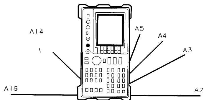
Figure 6-1. Hinged Assemblies
