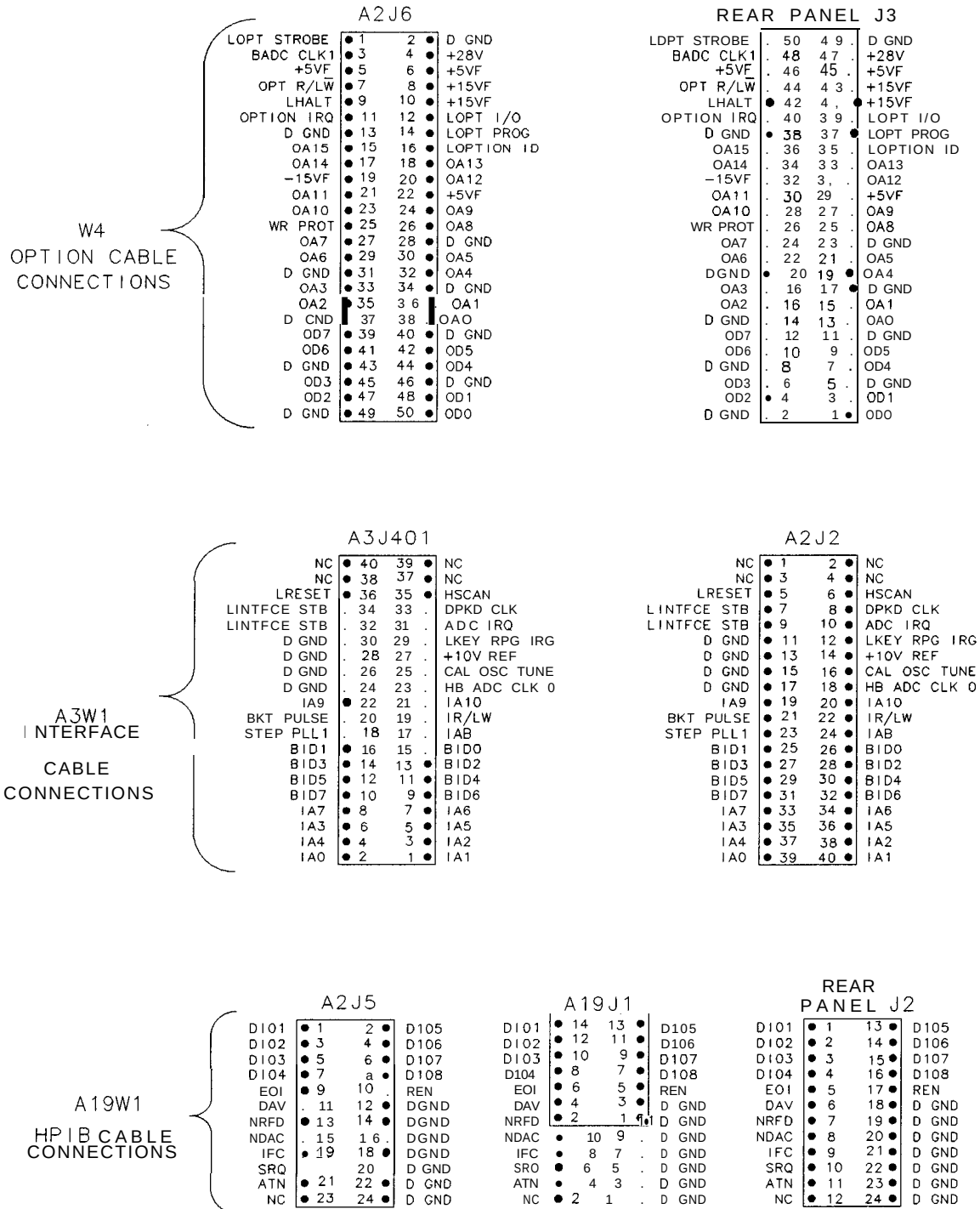
Figure 7-2. Ribbon Cable Connections (2 of 2)
