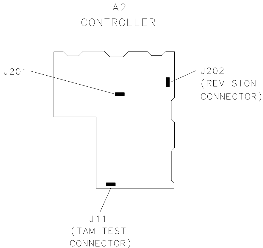
Figure 9-1 A2 Test Connectors
