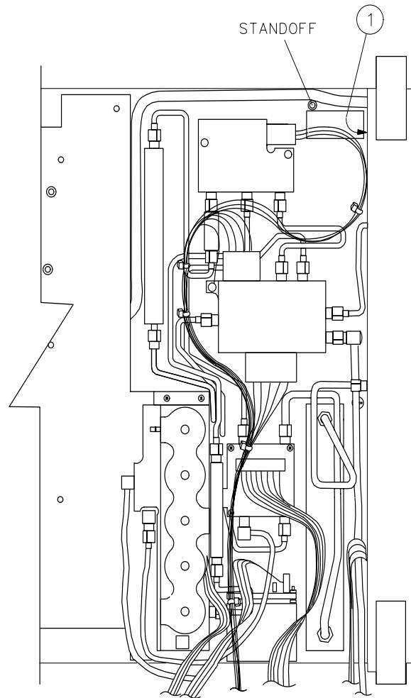
Figure 3-33 Line-Switch Mounting Screw and Cable Dress
