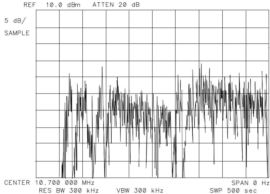
Figure 8-9 Noisy Signature
