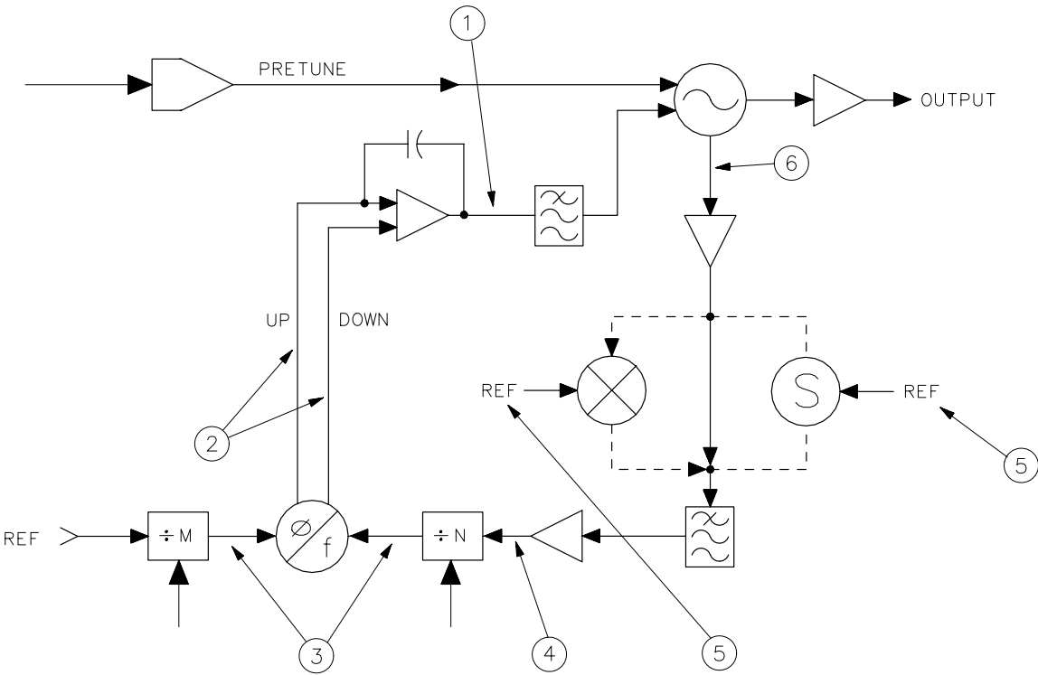
Figure 10-6 Unlocked PLL
