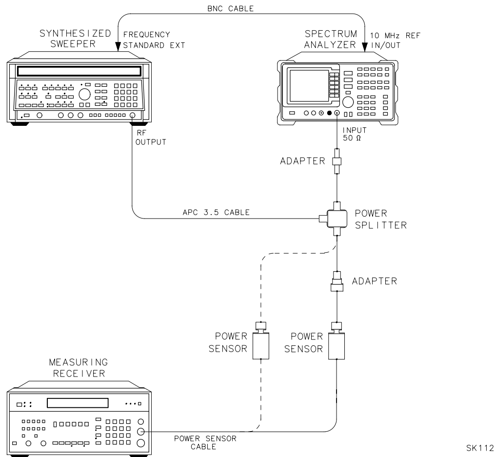
Figure 2-21 Frequency Response Adjustment Setup (8563E/EC)
