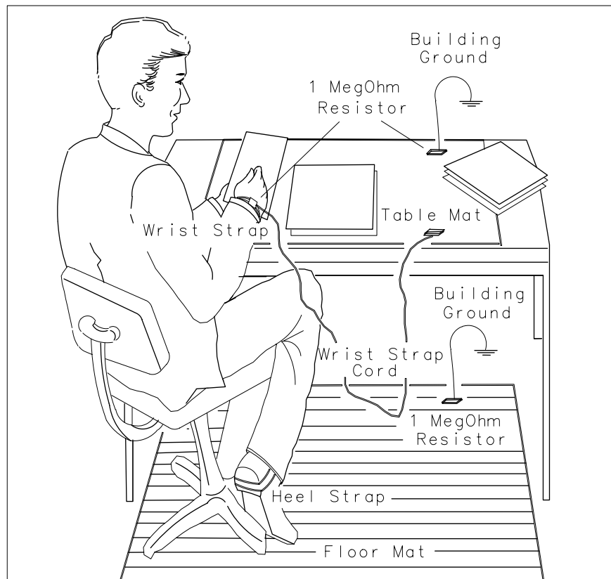
Example of a Static-Safe Workstation
