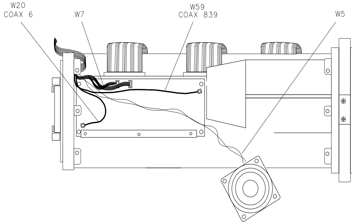
Figure 3-29 A16 Cable Routing
