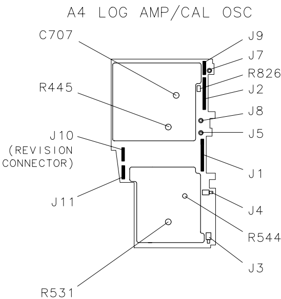
Figure 2a-4 DC Log Adjustment Locations
