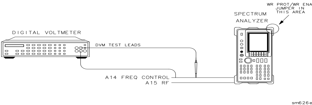
Figure 2-19 Dual Band Mixer Bias Adjustment Setup
