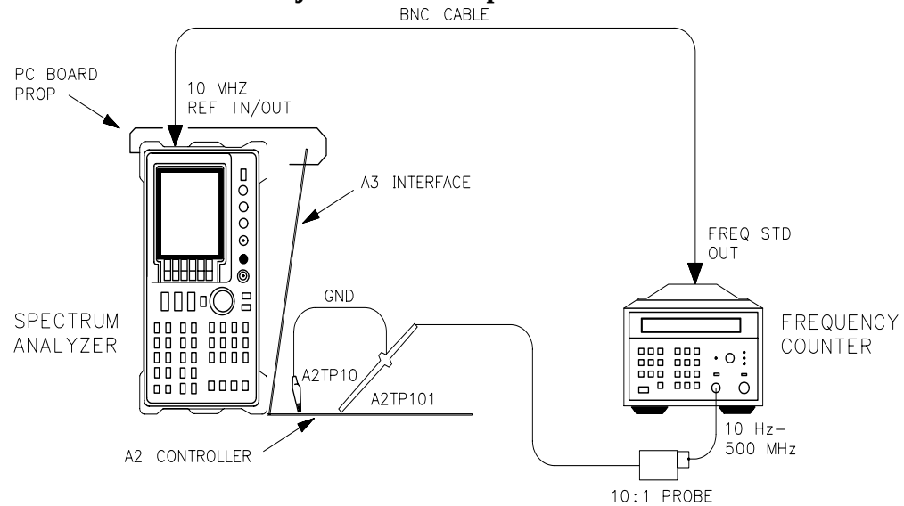
Figure 2-33 16 MHz PLL Adjustment Setup
