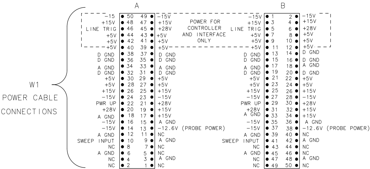
Figure 6-2 Ribbon Cable Connections (1 of 3)
