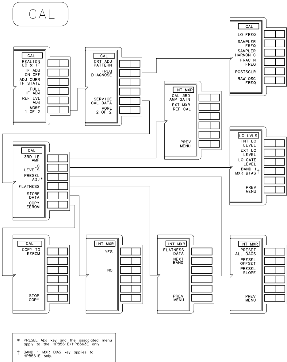
Figure 6-5 Service Cal Data Menu
