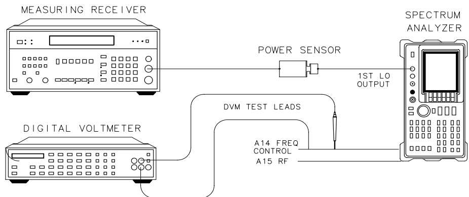
Figure 2-17 First LO Distribution Amplifier Adjustment Setup
