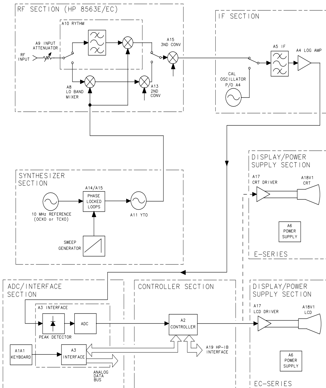
Figure 6-6 Functional Sections
