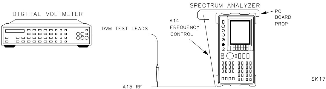
Figure 2-11 Sampler Adjustment Setup
