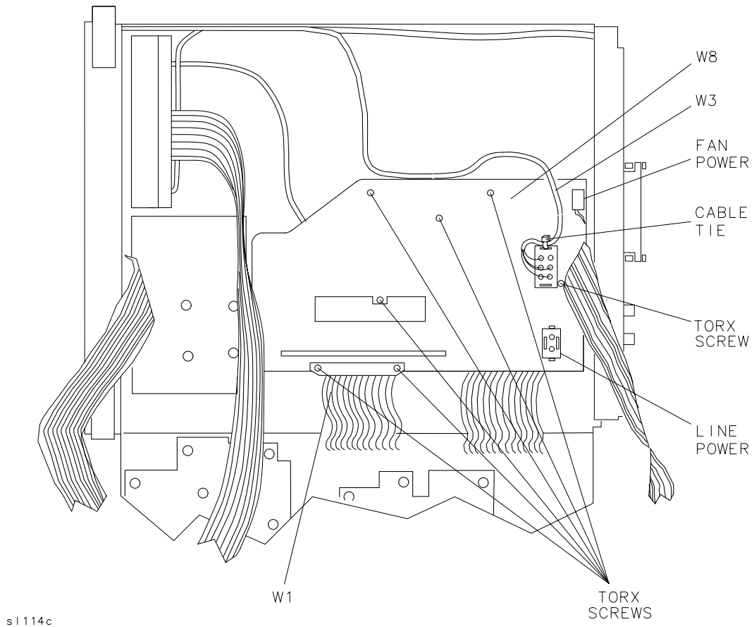
Figure 3-15 Power Supply Cover
