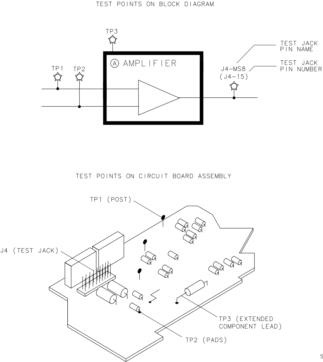
Figure 6-1 Assembly Test Points
