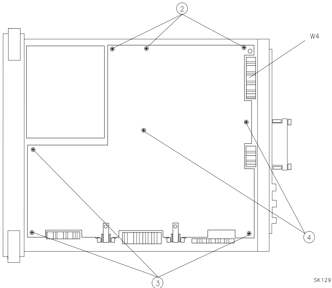
Figure 3-8 A2, A3, A4, and A5 Assembly Removal
