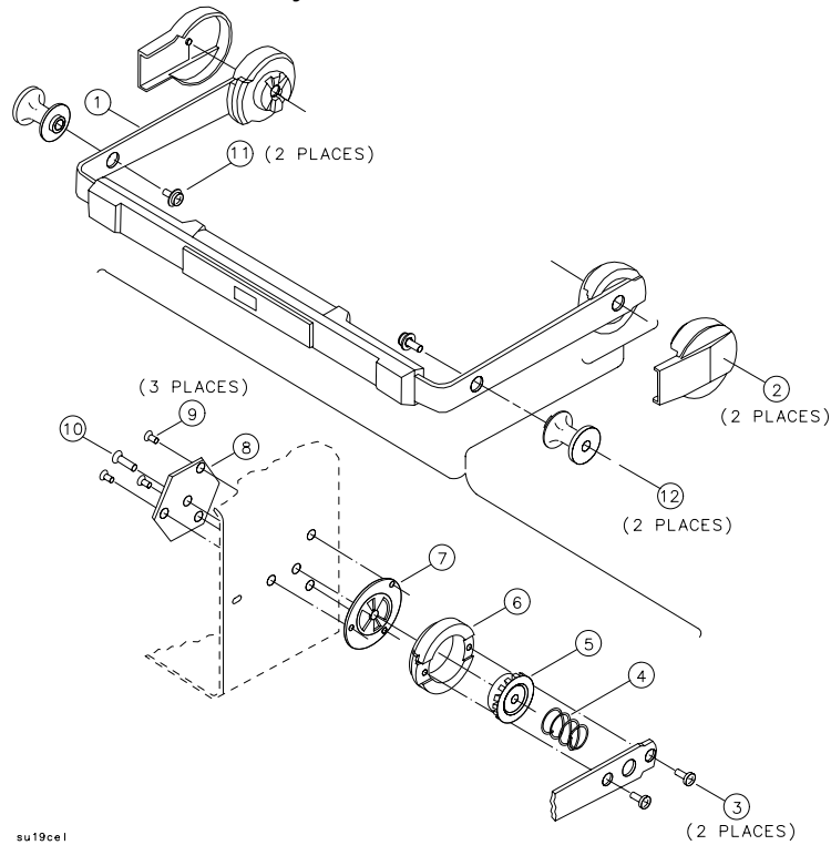
Handle Assembly Parts Identification
