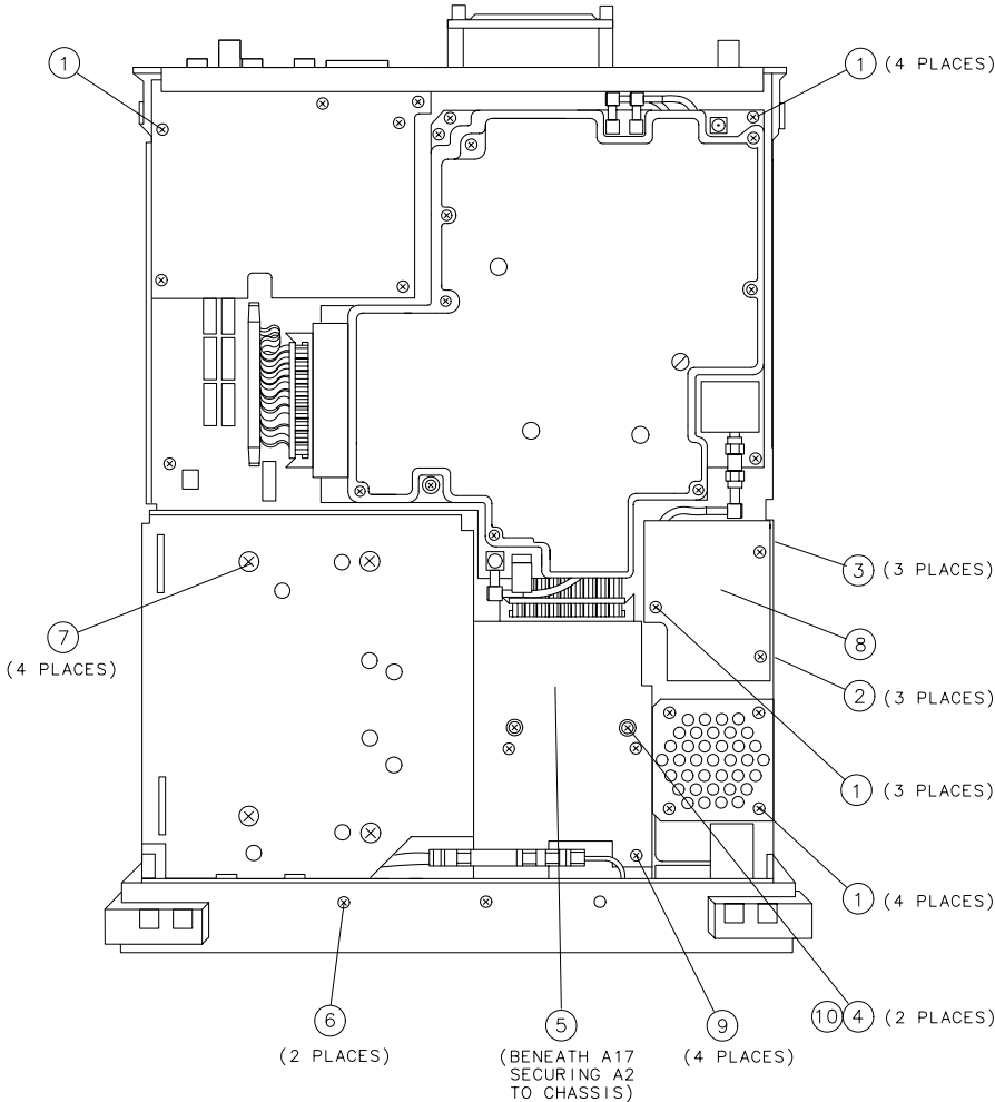
Figure 12-7 Chassis Bottom View Parts Identification
