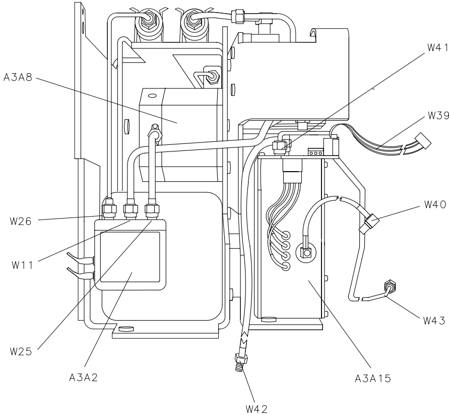
A3 Front-End Assembly, Rear View with A3A5 Removed 8593E (Options 009 and 010)
