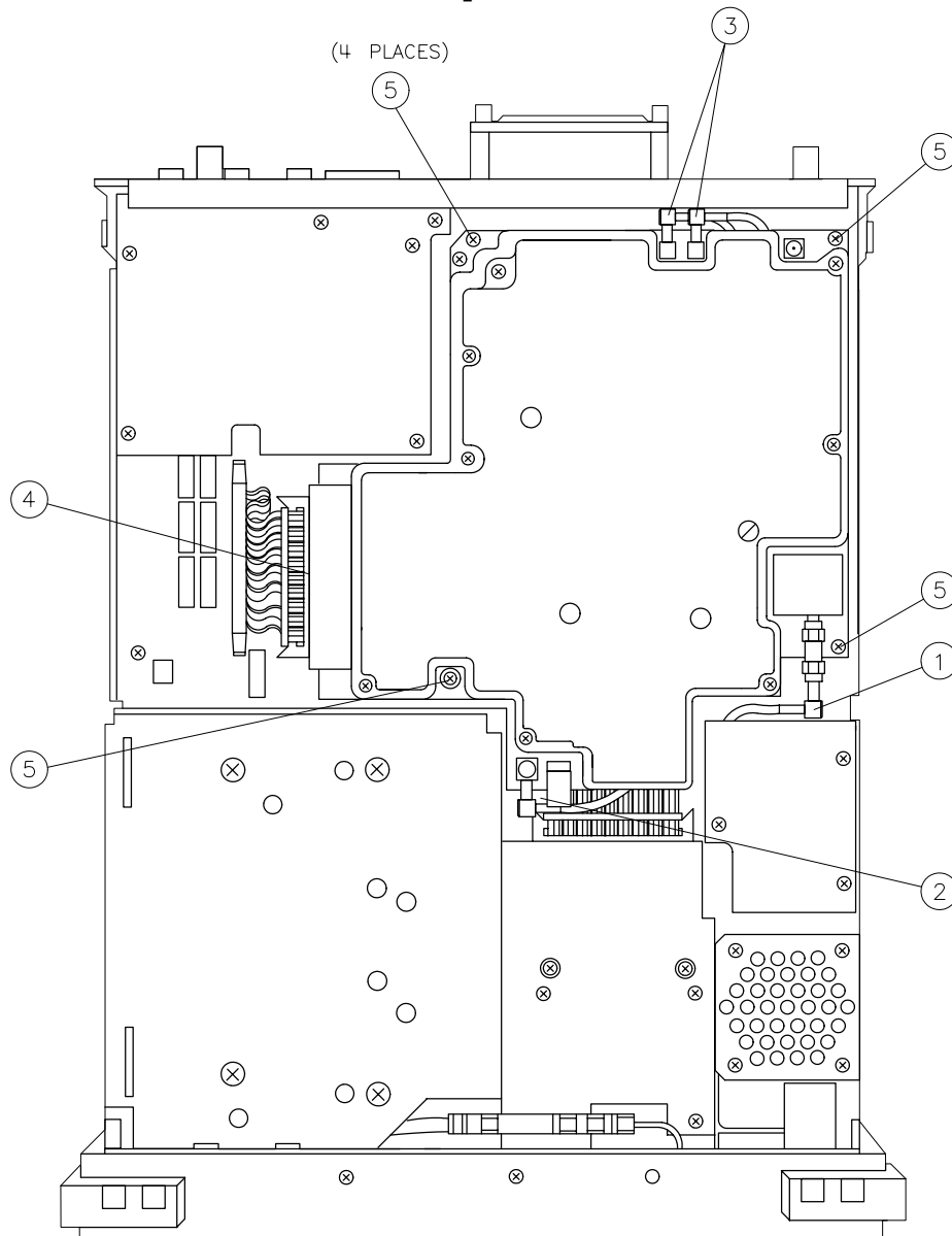
Figure 7-17 A25 Counter-Lock Replacement
