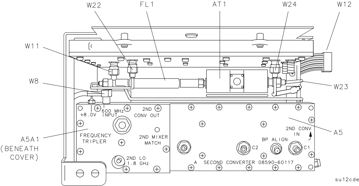
Figure 11-14 Front-End Assembly, Top View 8591C
