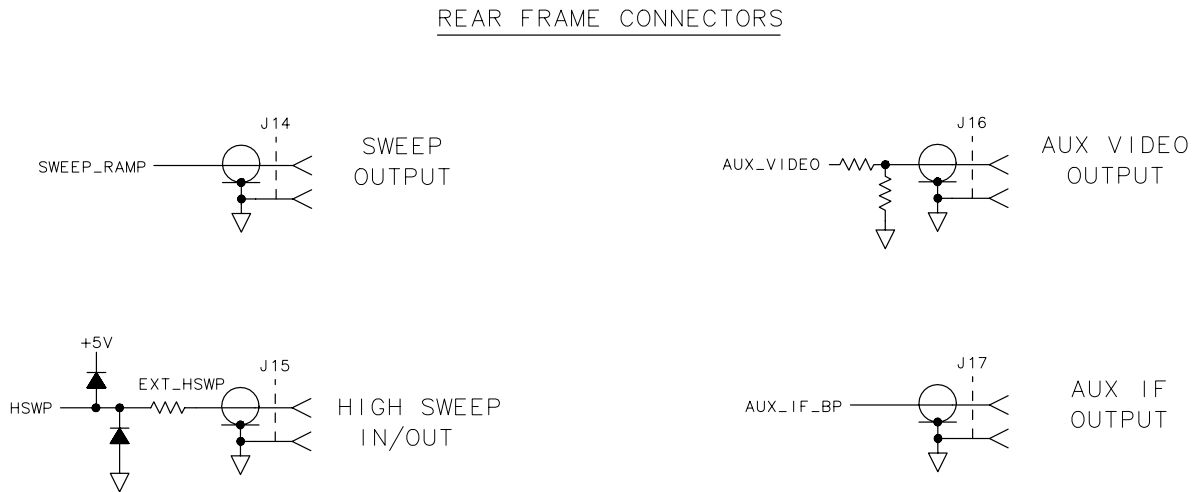
Figure 5-2 A15 Connectors with Additional Associated Circuitry (2 of 2)
