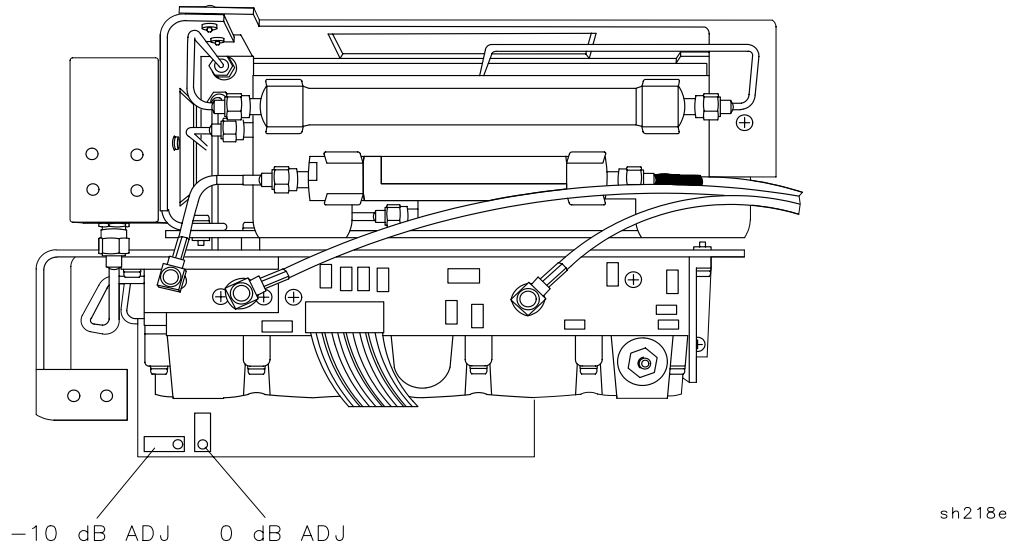
Figure 2-35 BITG Power Level Adjustment Locations
