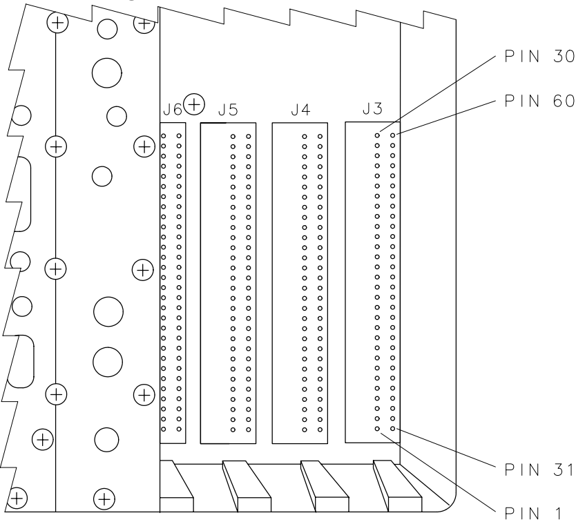
Figure 4-6 Card-Cage Connector-Pin Orientation
