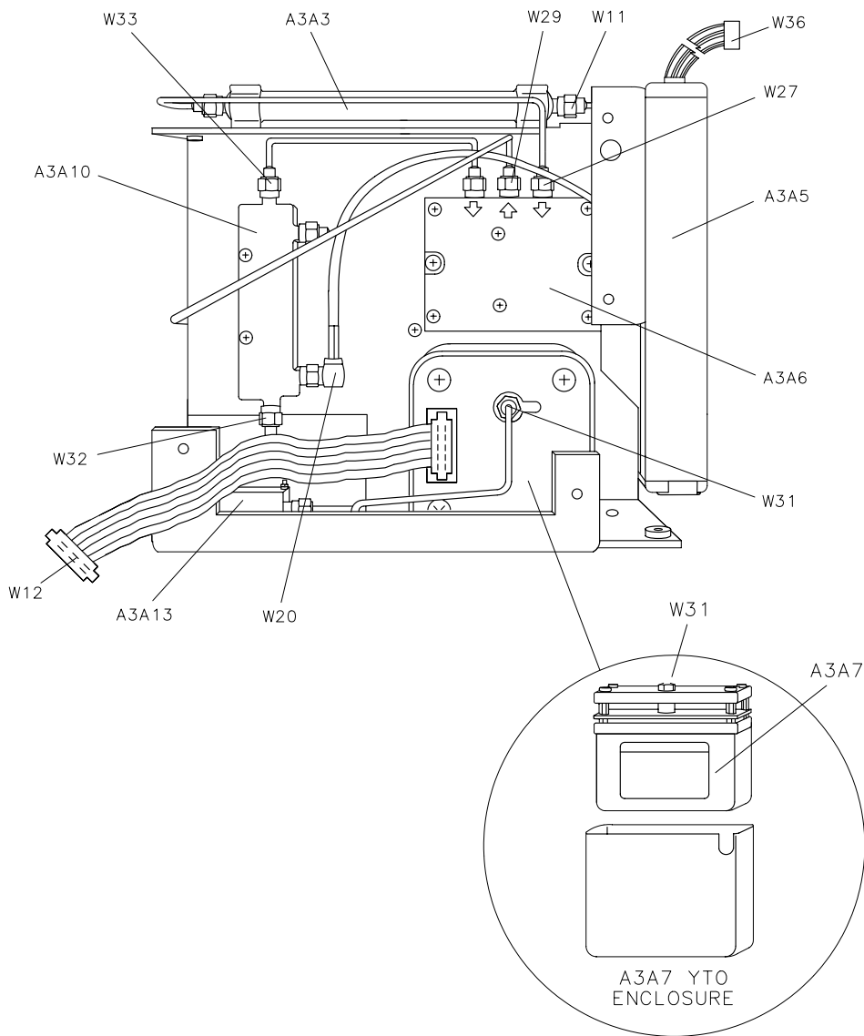
Figure 11-22 A3 Front-End Assembly, Right-Side View 8594E and 8594L
