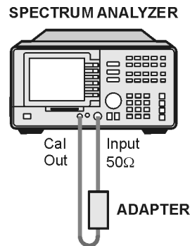
Figure 2-14 CAL AMPTD Adjustment Routine Setup
