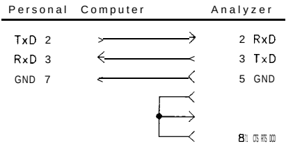
Figure C-4. 25-pin to O-pin 3-Wire Connection
