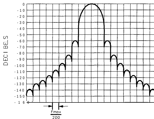
Figure 5-4. Hanning Filter Window
