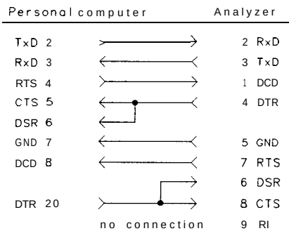
Figure C-2. HP 245426 25-pin to 9-pin Full Handshaking Connection
