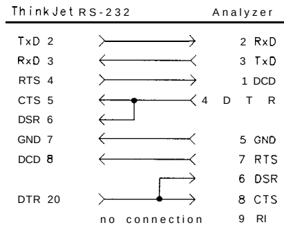
Figure C-6. 25-pin to 9-pin ThinkJet Printer Connection
