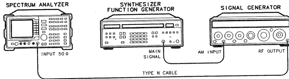
Figure 4-9. Sweep Time Accuracy Test Setup
