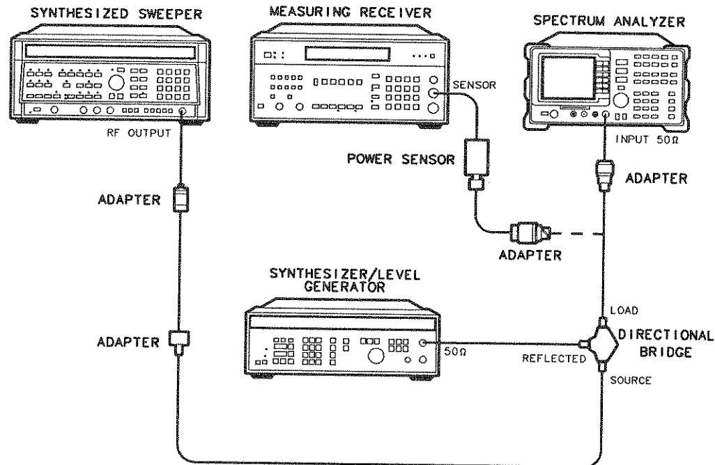
Figure 3-20. Gain Compression Test Setup
