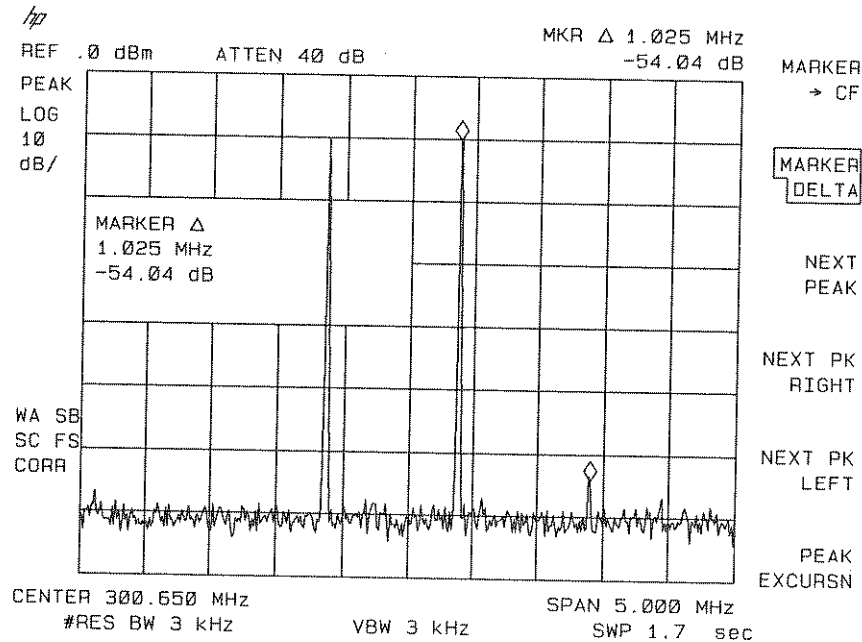
Figure 6-25. Measuring the Distortion Product
