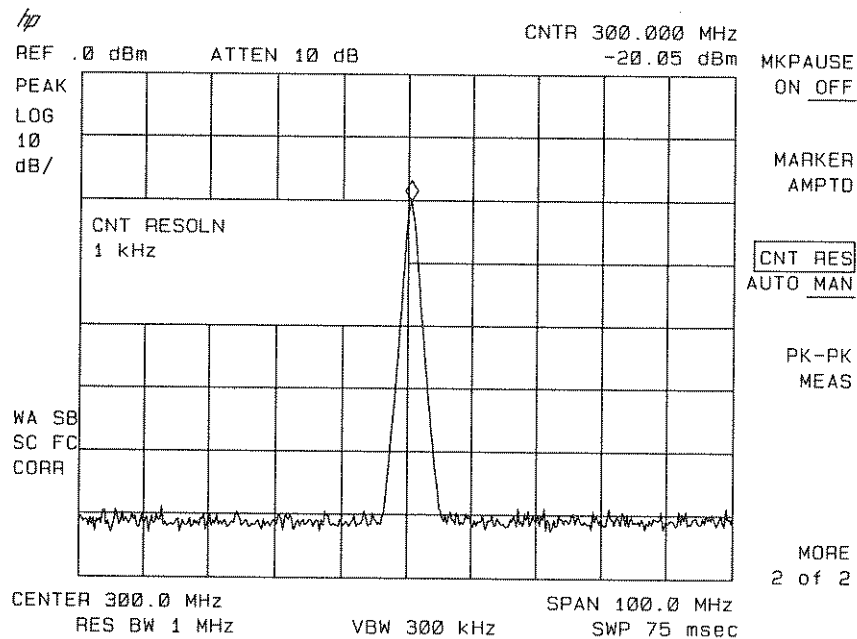
Figure 6-6. Using the Marker Counter
