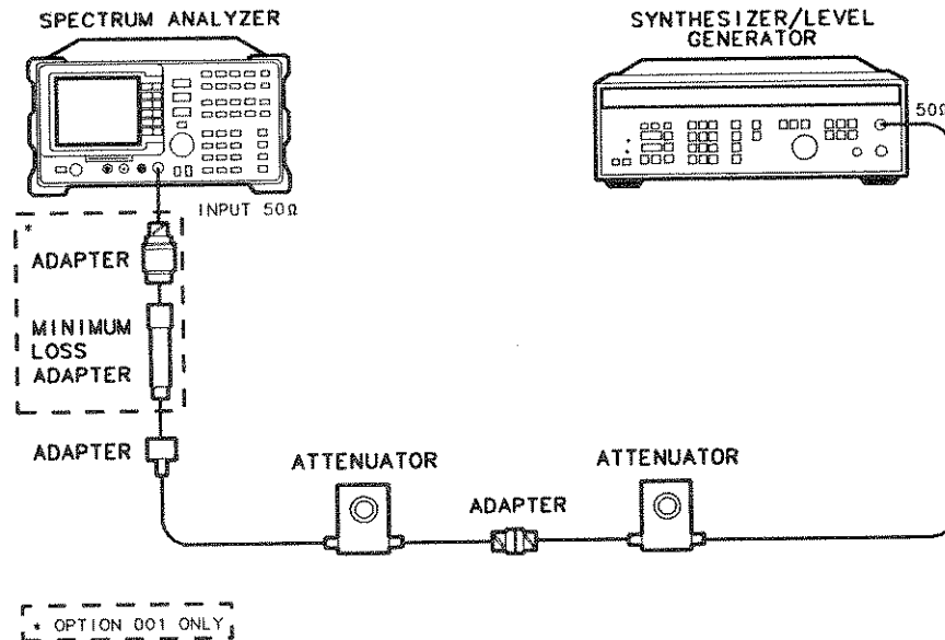
Figure 3-9. Input Attenuator Accuracy Test Setup
