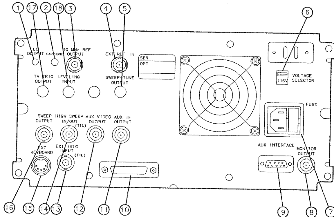
Figure 5-2. HP 8591A / HP 8593A Rear-Panel Overview
