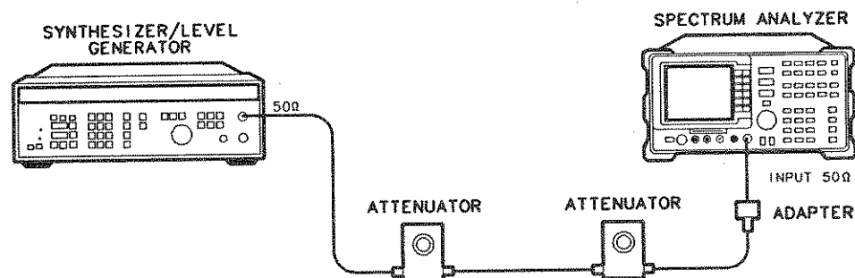
Figure 4-12. Reference Level Accuracy Test Setup
