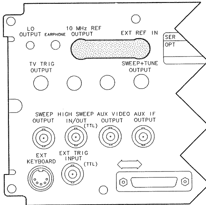
Figure 2-4. Reference Connector
