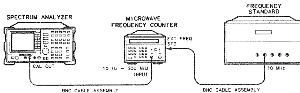
Figure 3-1. 10 MHz Reference Accuracy Test Setup (Standard Reference)
