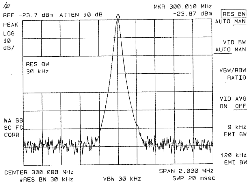
Figure 6-5. Signal Resolution with a 30 kHz Resolution Bandwidth
