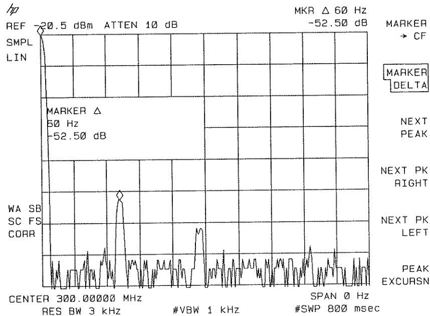
Figure 6-29. Using the FFT Function
