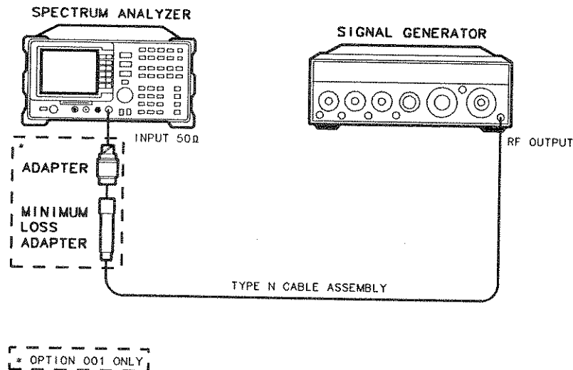
Figure 3-5. System Related Sidebands Test Setup
