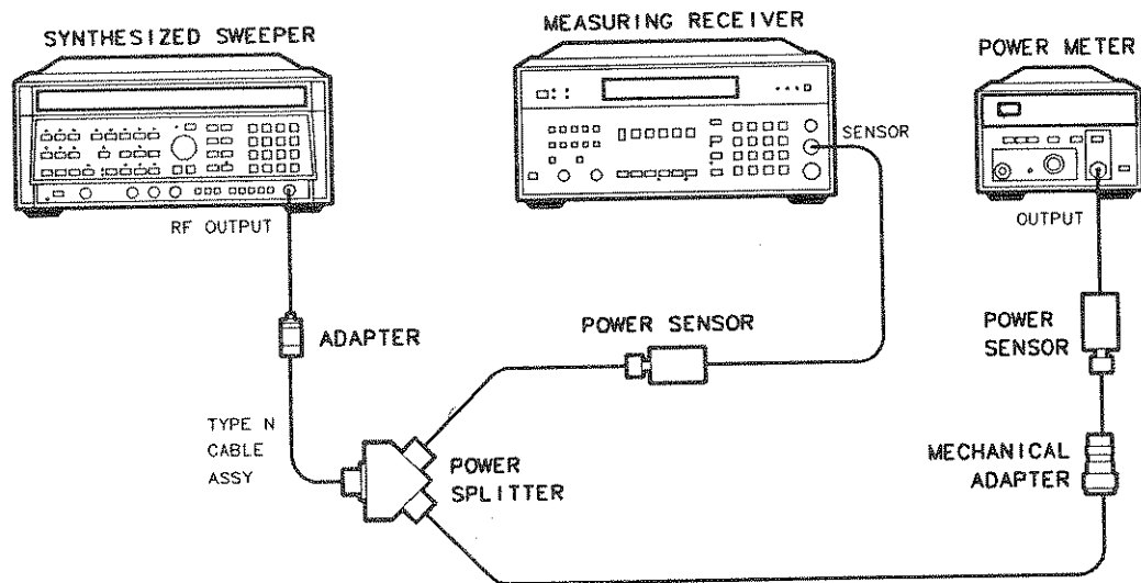
Figure 3-14. System Characterization Test Setup (Option 001)
