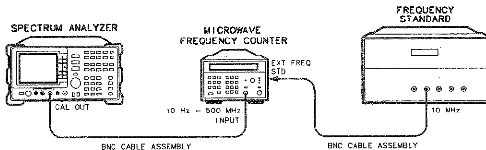
Figure 4-1. 10 MHz Reference Accuracy Test Setup (Standard Reference)
