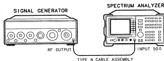
Figure 4-6. Residual FM Test Setup
