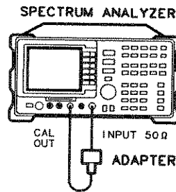
Figure 4-13. Resolution Bandwidth Switching Uncertainty Test Setup
