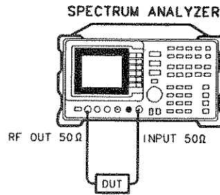
Figure 6-33. Transmission Measurement Test Setup
