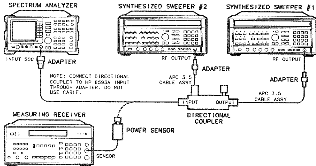
Figure 4-21. Third-Order Intermodulation Distortion Test Setup
