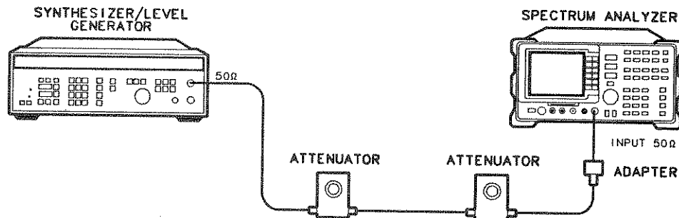
Figure 4-10. Scale Fidelity Test Setup
