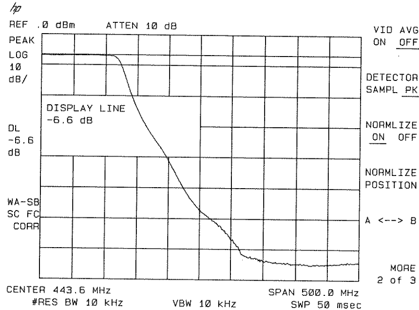
Figure 6-38. Normalized Trace
