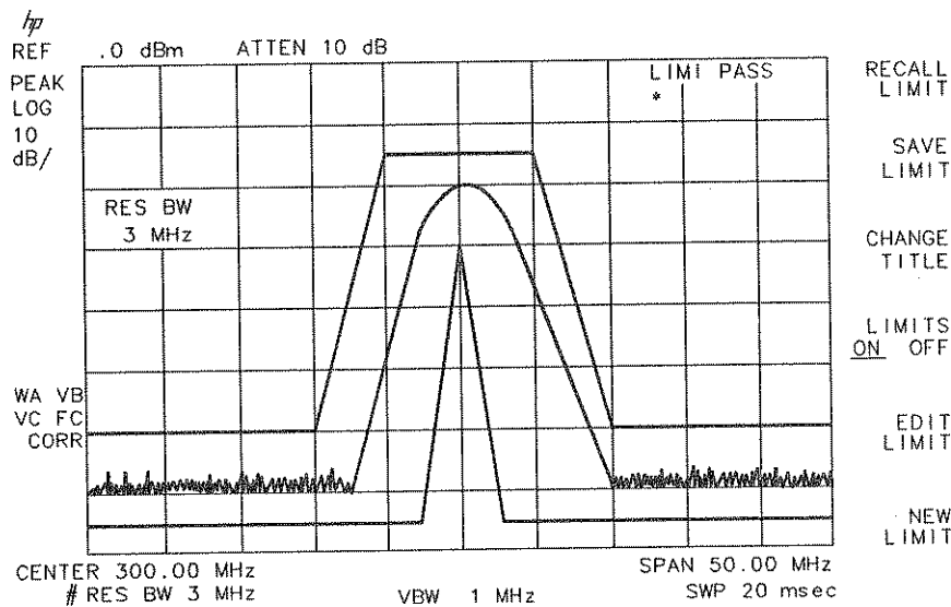
Figure 5-11. Upper and Lower Limit-Line Testing
