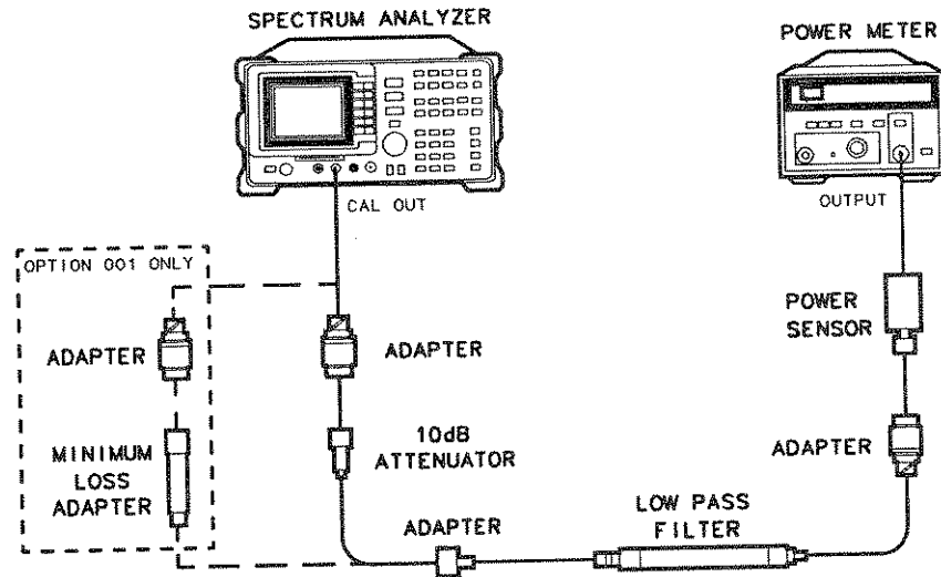
Figure 3-13. Calibrator Amplitude Accuracy Test Setup
