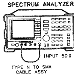
Figure 4-7. Frequency Span Accuracy Test Setup (Spans \geq 500 MHz)
