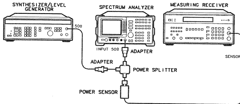
Figure 4-17. Frequency Response Test Setup (<50 MHz)
