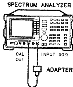
Figure 4-27. Fast Sweep Time Amplitude Test Setup
