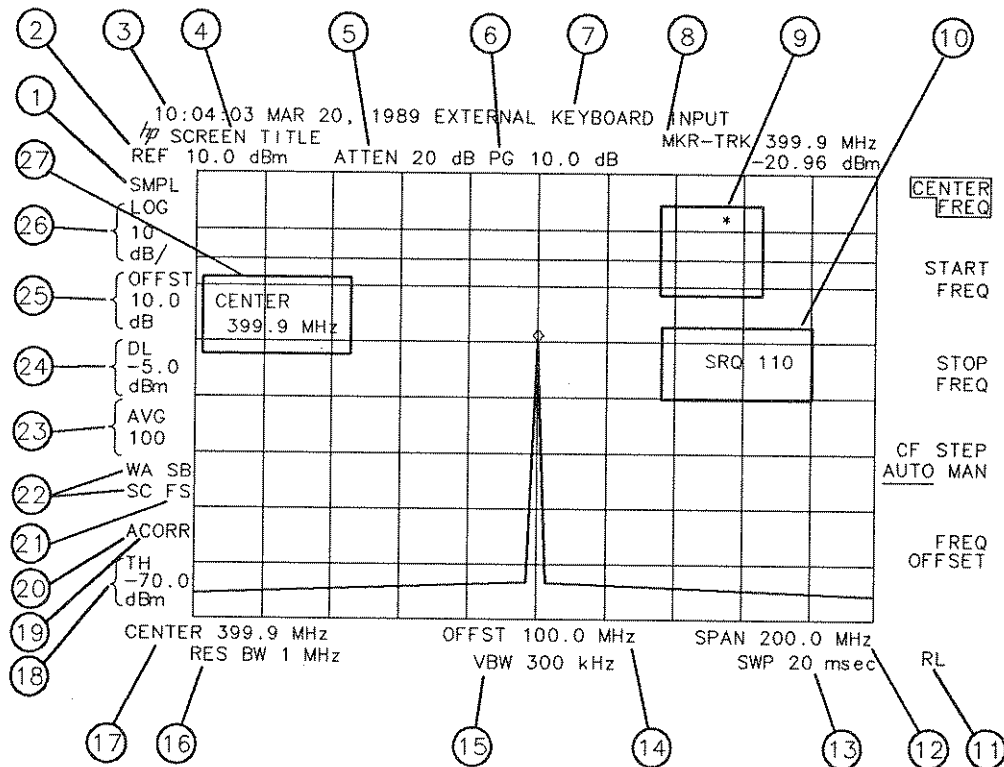
Figure 5-5. Screen Annotation
