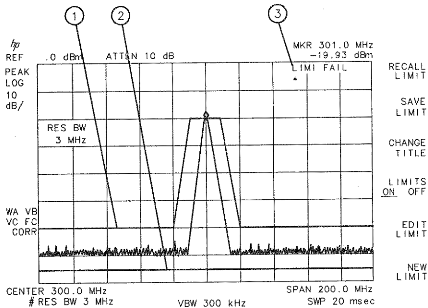
Figure 5-7. Typical Limit-Line Display
