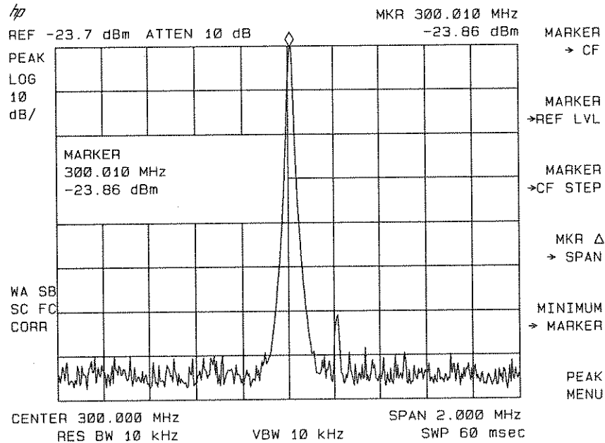
Figure 6-4. Signal Resolution with a 10 kHz Resolution Bandwidth
