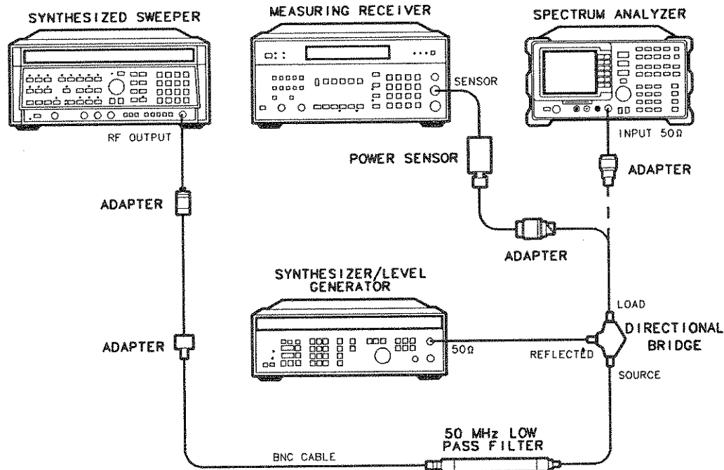
Figure 3-19. Third Order Intermodulation Distortion Test Setup
