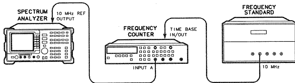
Figure 4-26. 10 MHz Reference Accuracy Test Setup, Option 004
