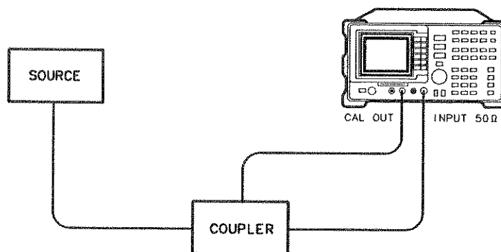
Figure 6-1. Set-Up for Obtaining Two Signals
