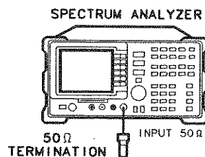
Figure 3-22. Residual Response Test Setup
