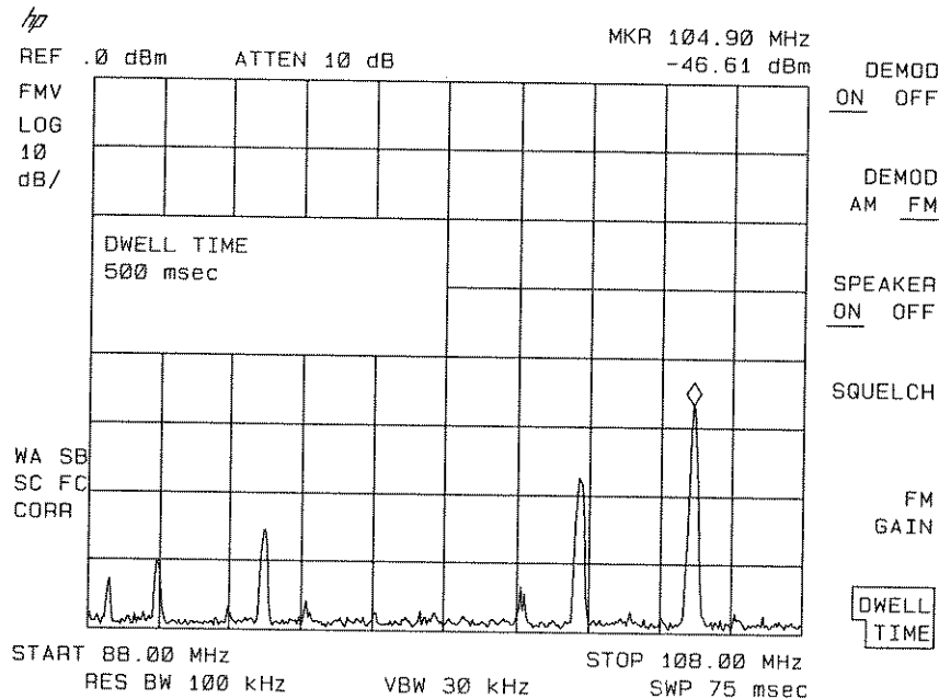
Figure 6-40. Demodulation of an FM Signal
