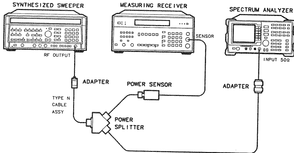
Figure 3-15. Frequency Response Test Setup, \geq 50 MHz
