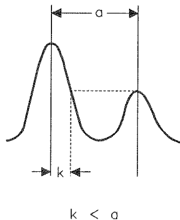
Figure 6-3. Resolution Bandwidth Requirements for Resolving Small Signals
