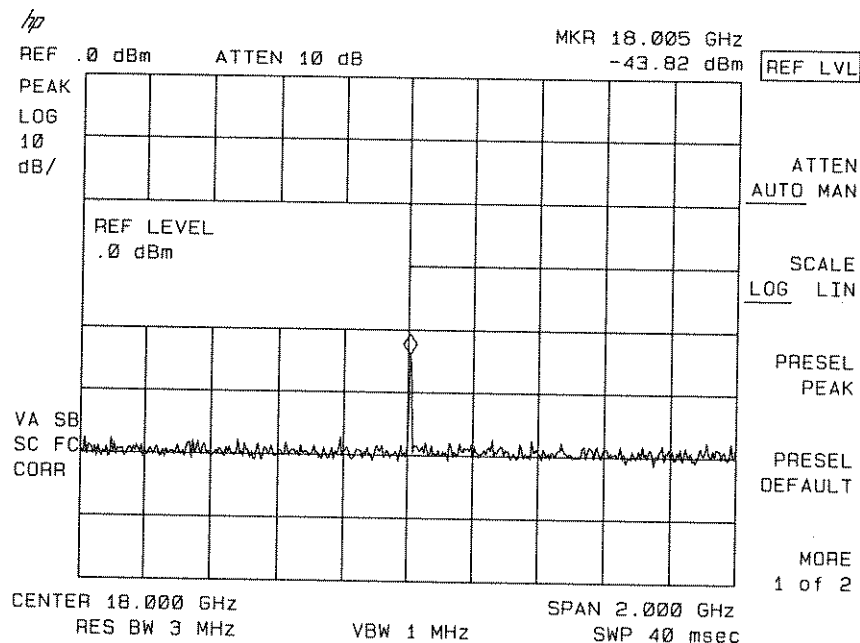
Figure 6-8. Peaking Signal Amplitude with Preselector Peak
