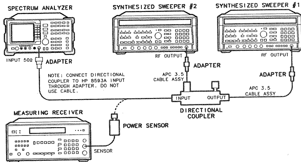
Figure 4-23. Gain Compression Test Setup
