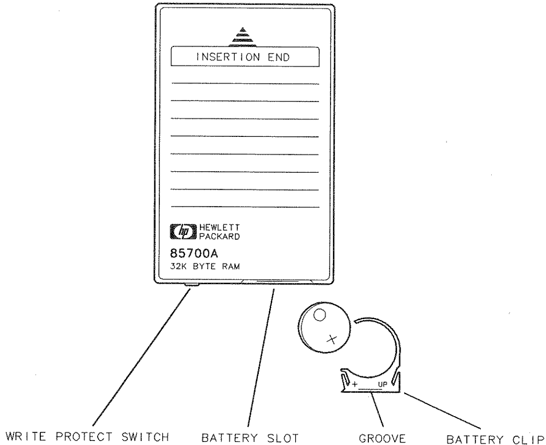
Figure 2-7. Memory Card Battery Replacement
