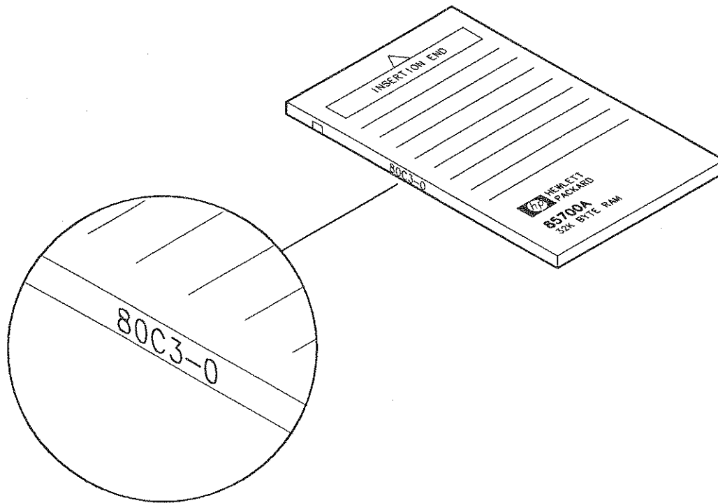
Figure 2-6. Memory Card Battery Date Code Location
