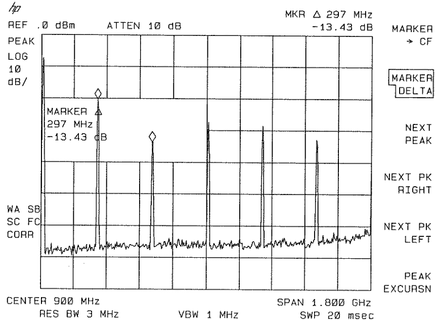
Figure 6-13. Using the Marker Delta Function
