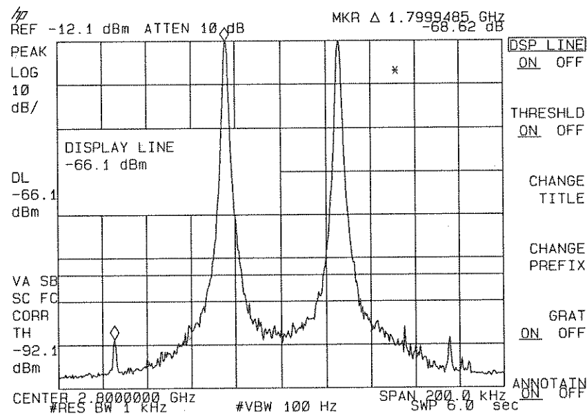
Figure 4-22. Third Order Intermodulation Distortion
