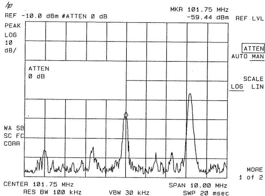
Figure 6-17. Using 0 dB Attenuation
