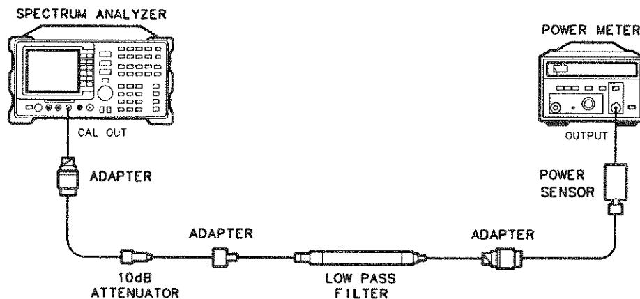
Figure 4-15. Calibrator Amplitude Accuracy Test Setup
