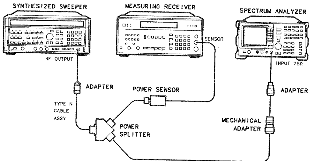
Figure 3-16. Frequency Response Test Setup, \geq 50 MHz, for Option 001
