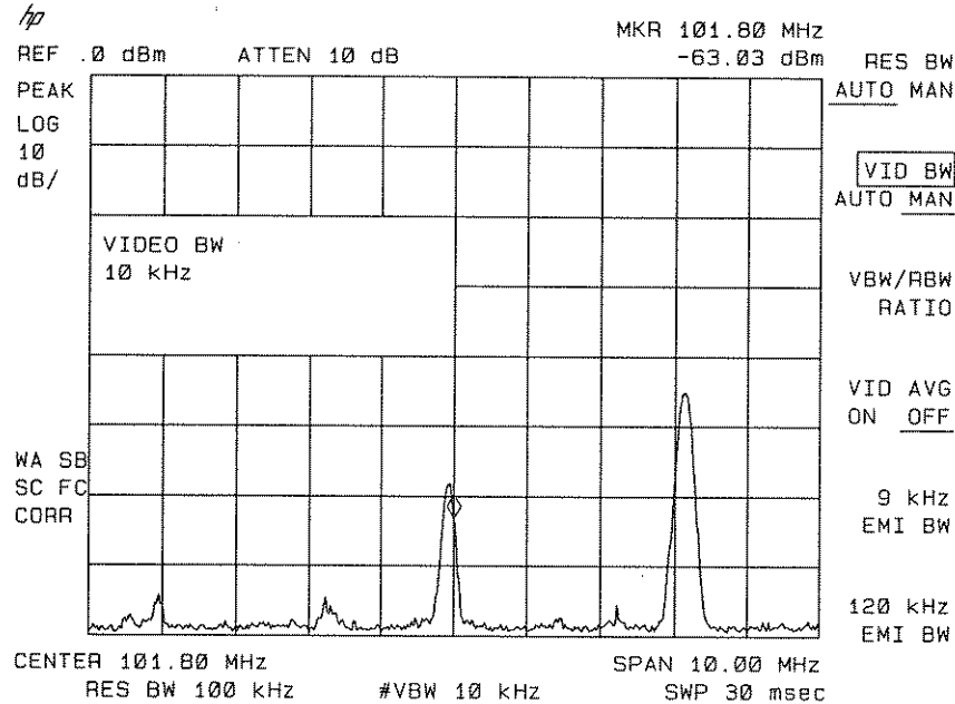
Figure 6-19. Decreasing Video Bandwidth
