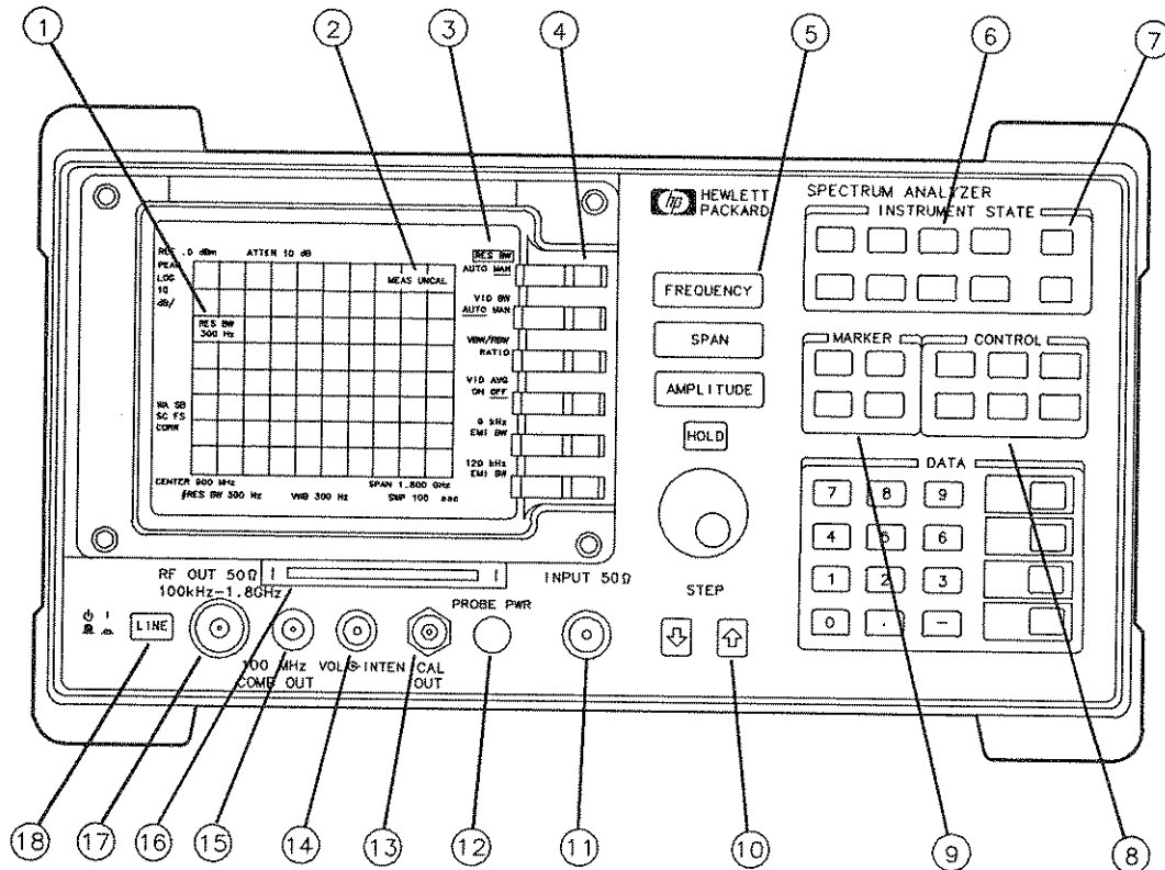
Figure 5-1. Front-Panel Feature Overview
