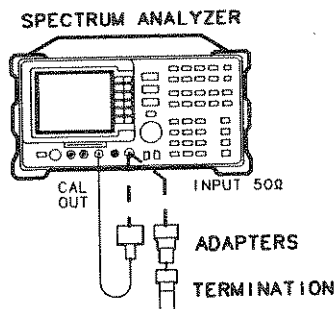
Figure 4-24. Reference Offset Test Setup
