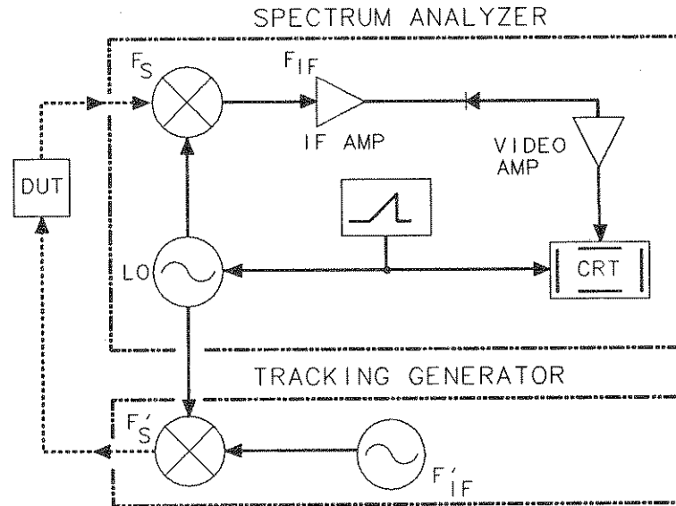
Figure 6-32. Block Diagram of a Spectrum-Analyzer/Tracking-Generator Measurement System
