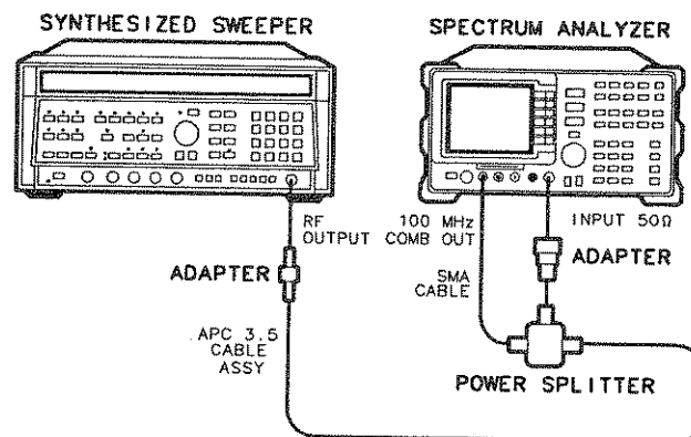
Figure 4-2. Comb Generator Frequency Accuracy Test Setup
