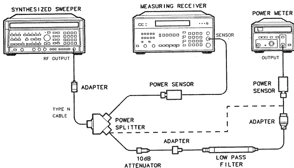
Figure 4-14. LPF Characterization
