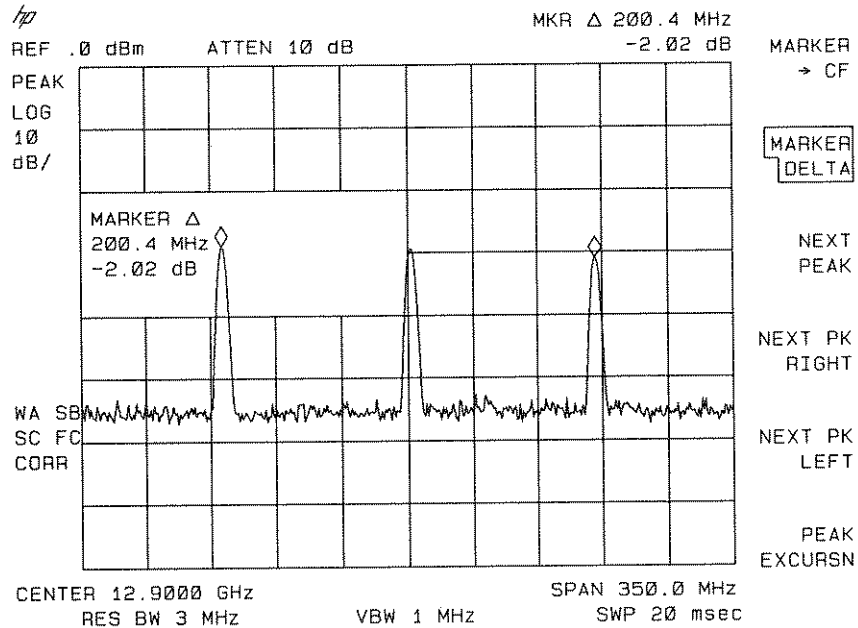
Figure 6-30. Using Harmonic Lock
