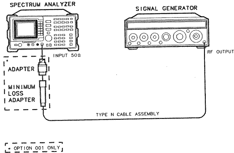
Figure 3-4. Residual FM Test Setup
