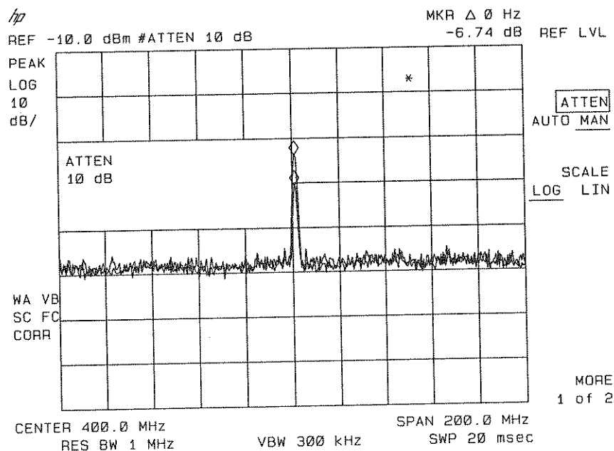
Figure 6-22. RF Attenuation of 10 dB
