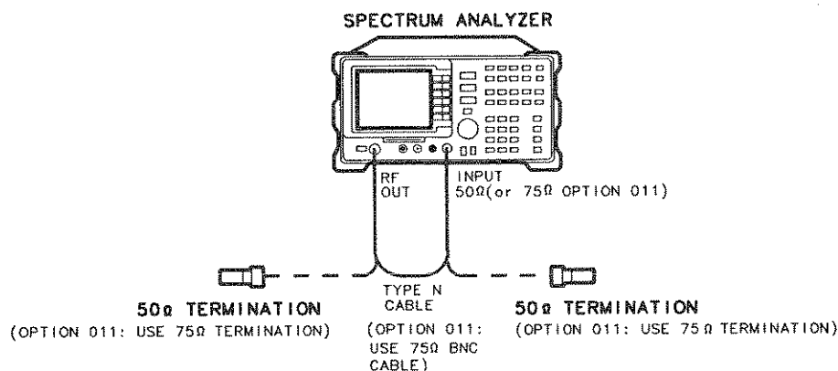
Figure 3-31. Tracking Generator Feedthrough Test Setup
