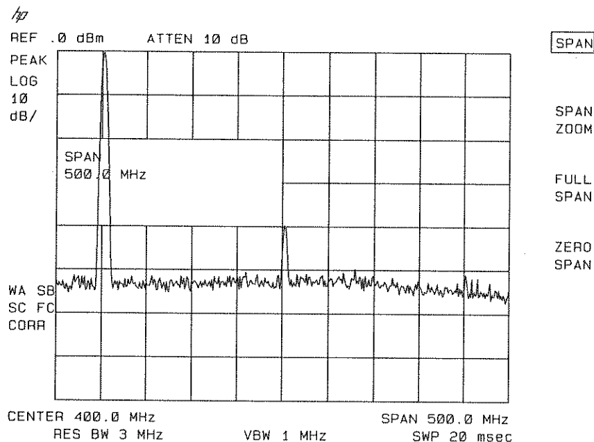
Figure 6-21. Harmonic Distortion
