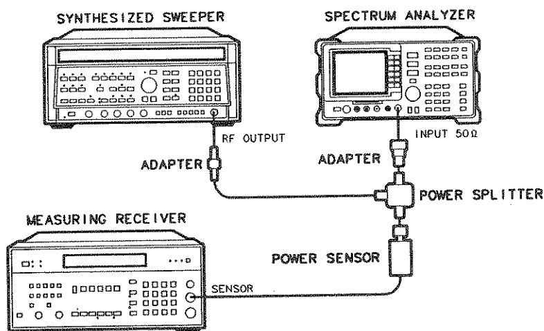
Figure 4-18. Other Input Related Spurious Test Setup
