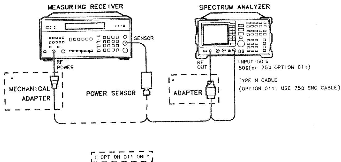
Figure 3-26. Absolute Amplitude, Vernier, and Power Sweep Accuracy Test Setup
