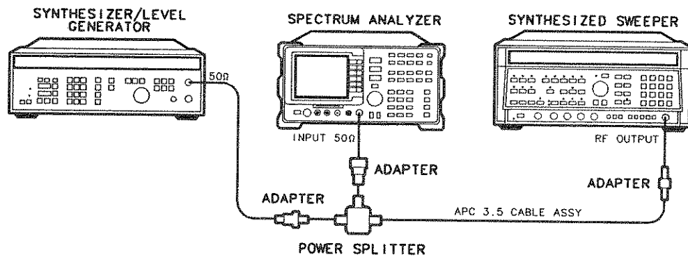
Figure 4-8. Frequency Span Accuracy Test Setup (Spans < 500 MHz)
