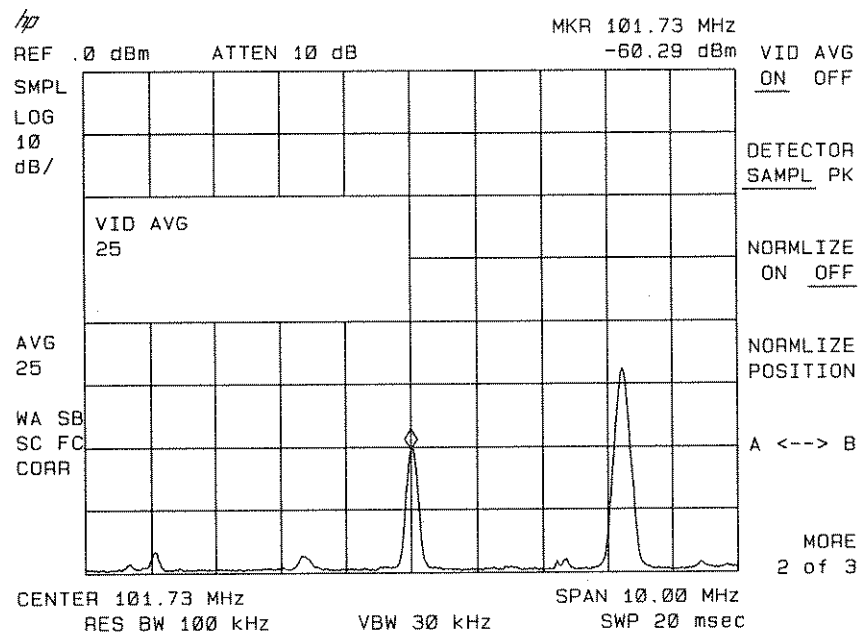
Figure 6-20. Using the Video Averaging Function
