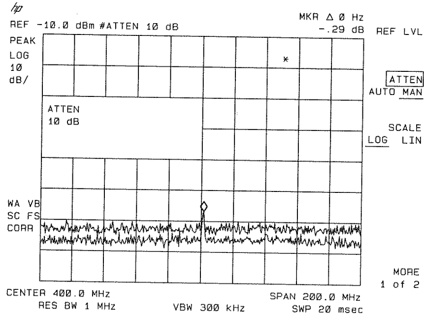
Figure 6-23. No Harmonic Distortion
