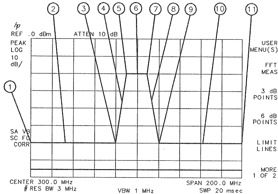
Figure 5-9. Limit-Line Segments
