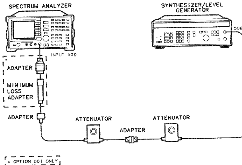
Figure 3-8. Scale Fidelity Test Setup
