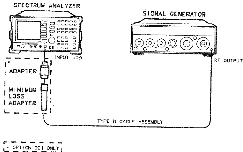
Figure 3-3. Noise Sidebands Test Setup
