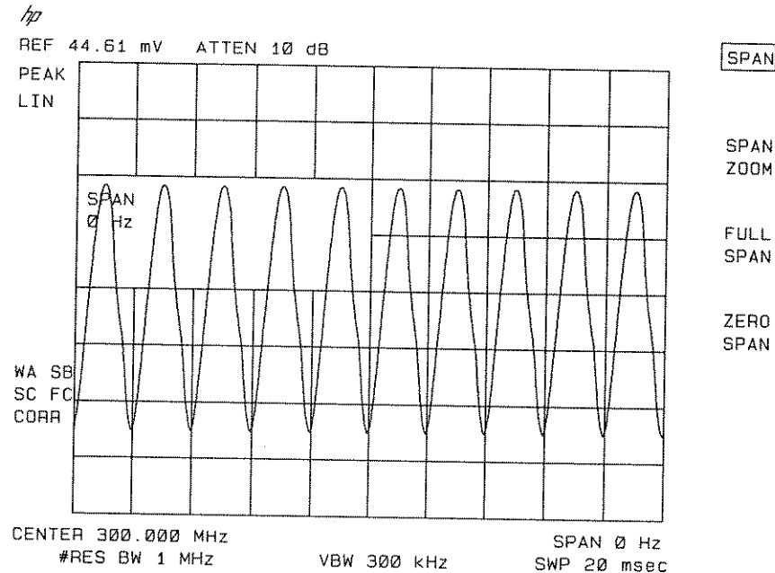
Figure 6-27. Measuring Modulation in Zero Span
