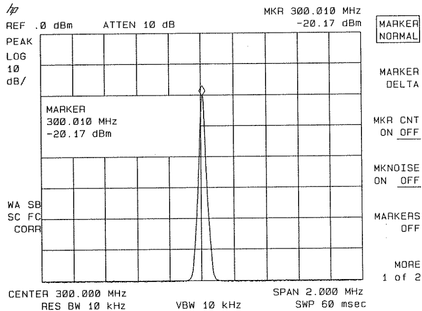
Figure 5-4. Reading the Amplitude and Frequency
