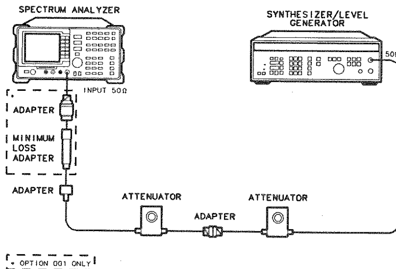
Figure 3-10. Reference Level Accuracy Test Setup
