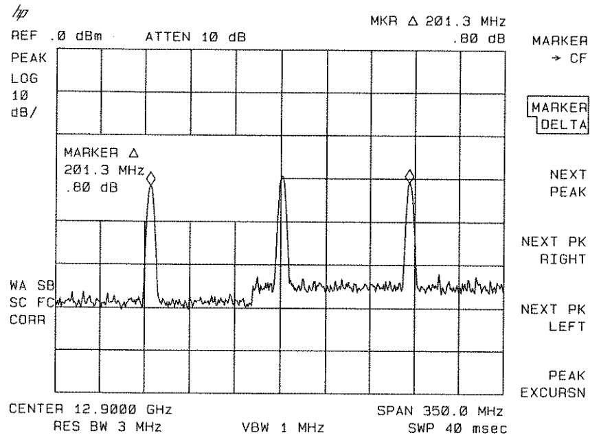
Figure 6-31. Harmonic Locking Off
