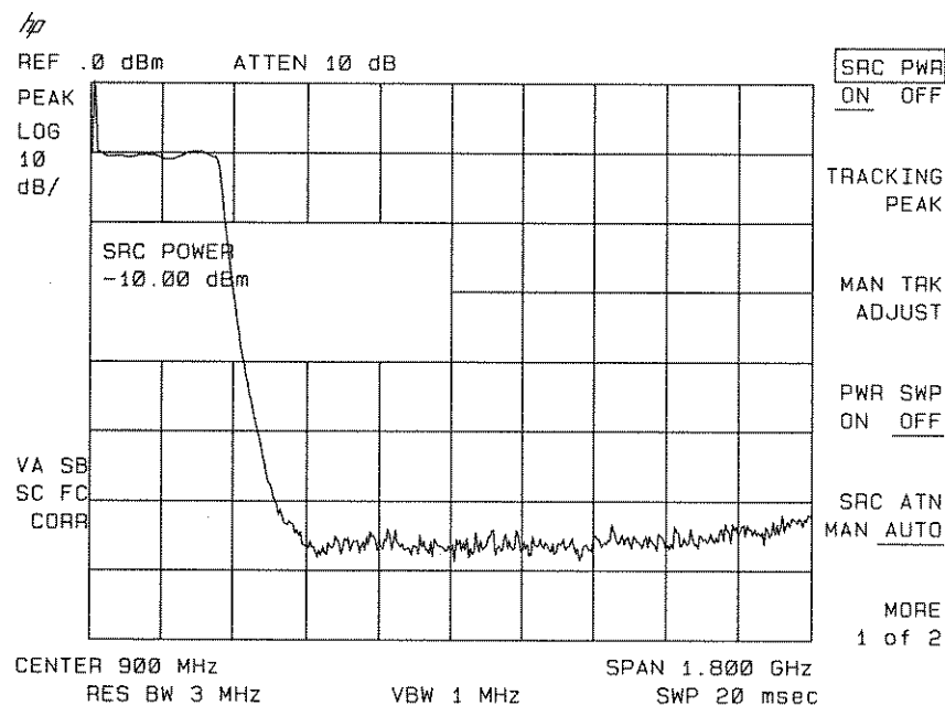
Figure 6-34. Tracking-Generator Output Power Activated
