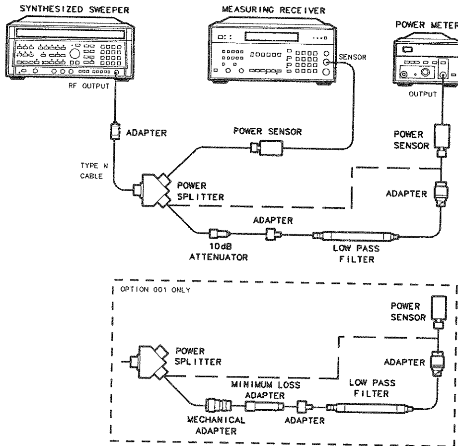
Figure 3-12. LPF Characterization
