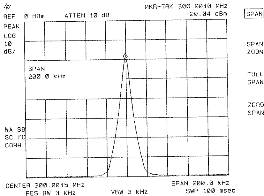
Figure 6-7. After Zooming In on the Signal
