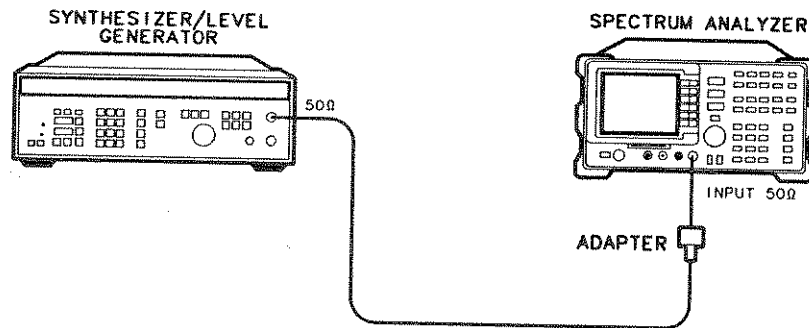
Figure 3-17. Frequency Response Test Setup (&lt;50 MHz)
