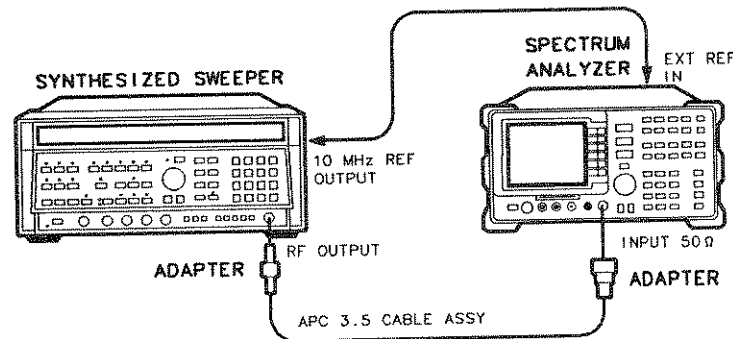
Figure 4-3. Frequency Readout Accuracy Test Setup
