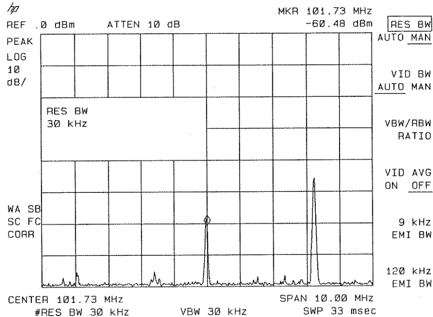
Figure 6-18. Decreasing Resolution Bandwidth
