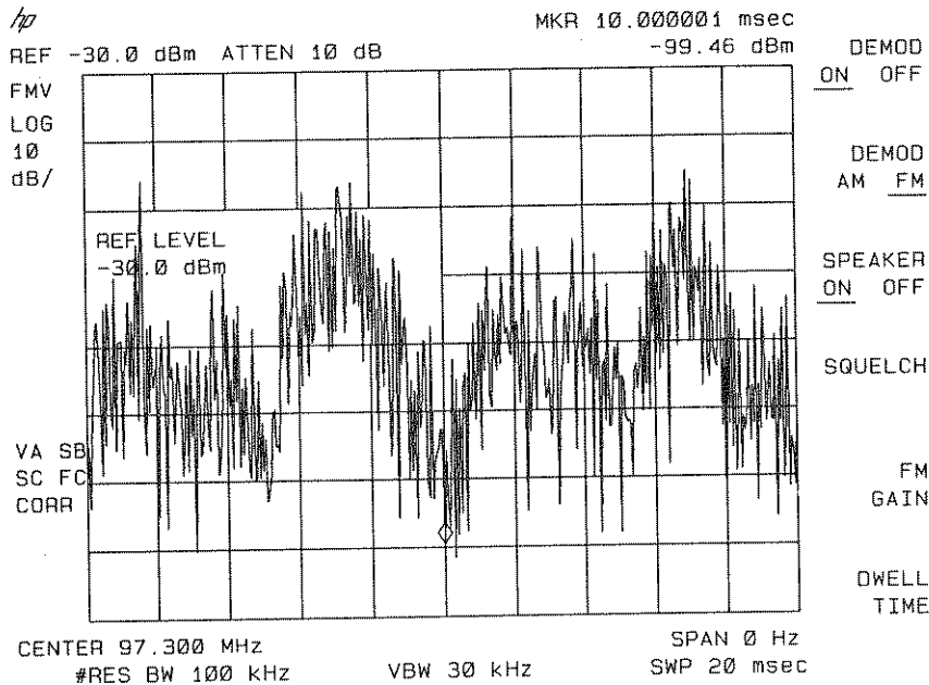
Figure 6-41. Continuous Demodulation of an FM Signal
