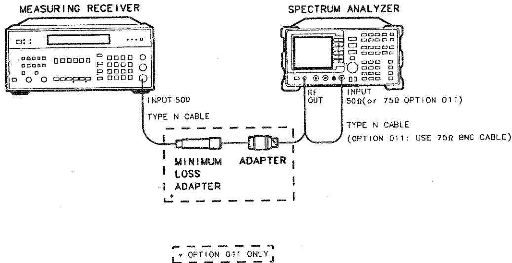
Figure 3-27. Output Attenuator Accuracy Test Setup
