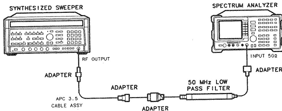
Figure 4-19. Second Harmonic Distortion Test Setup
