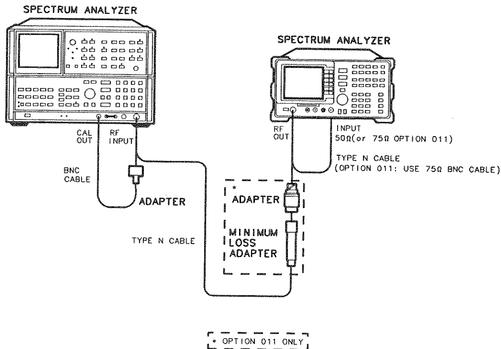
Figure 3-30. Non-Harmonic Spurious Outputs Test Setup
