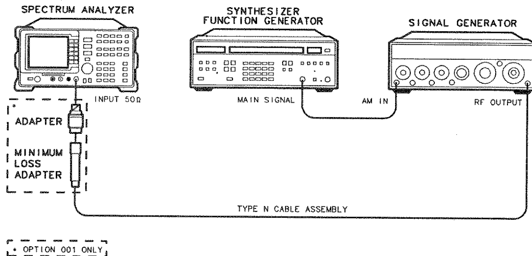
Figure 3-7. Sweep Time Accuracy Test Setup
