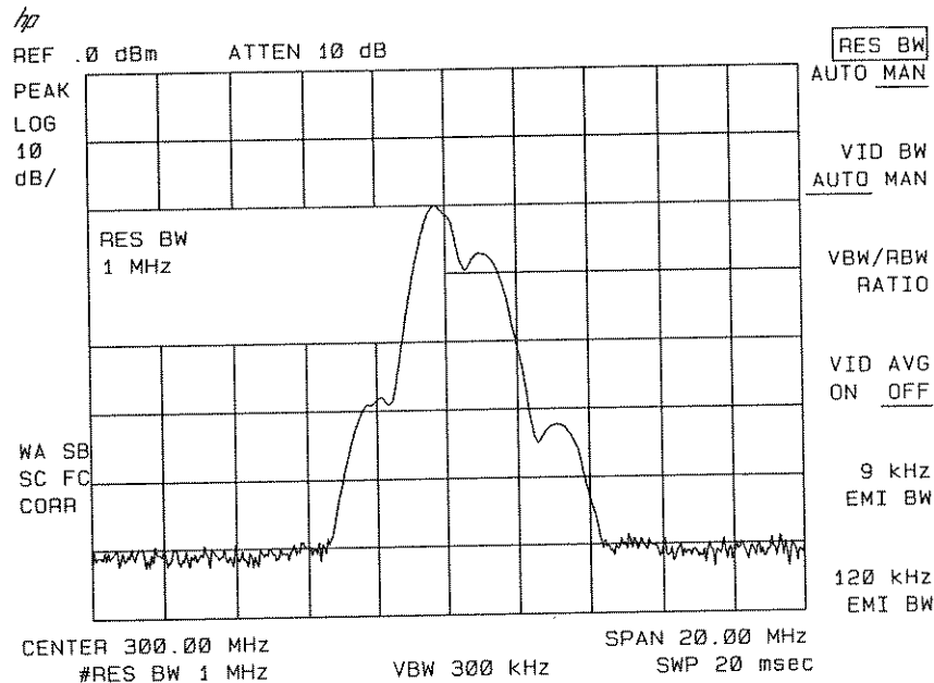
Figure 6-26. Viewing an AM Signal
