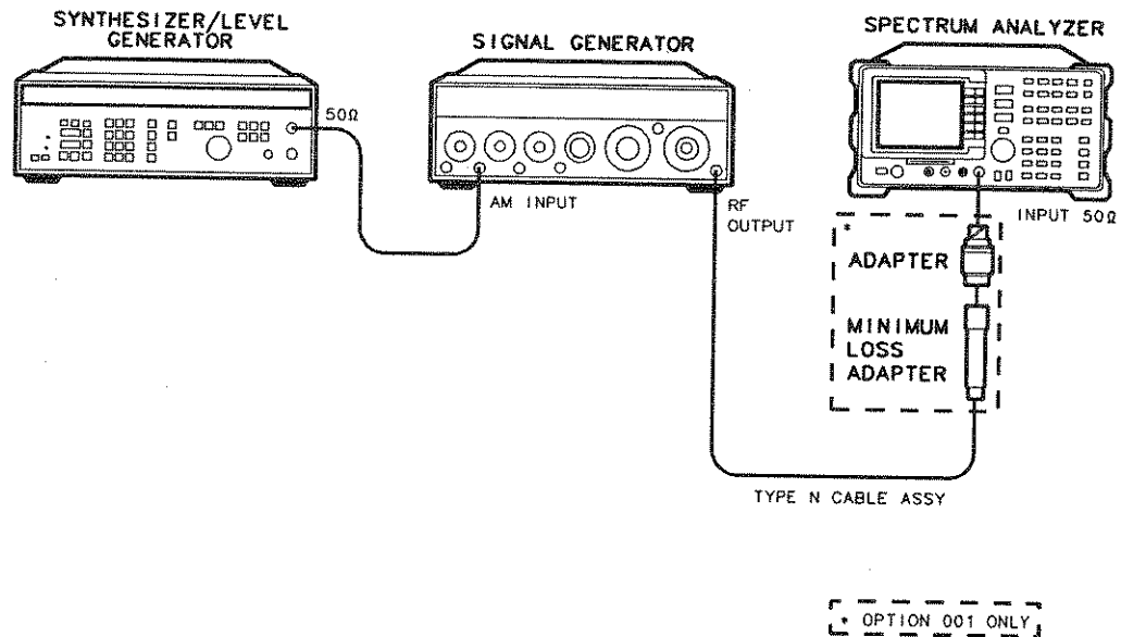
Figure 3-25. Fast Sweep Time Test Setup, Option 101
