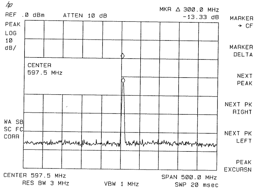
Figure 6-15. Frequency and Amplitude Difference Between Signals
