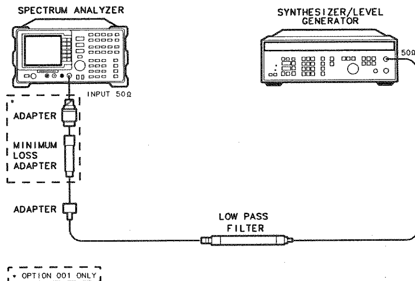
Figure 3-18. Second Harmonic Distortion Test Setup, 30 MHz
