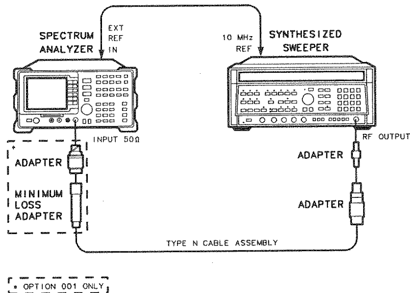
Figure 3-2. Frequency Readout Accuracy Test Setup
