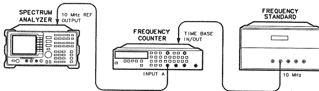
Figure 3-23. 10 MHz Reference Accuracy Test Setup, Option 004
