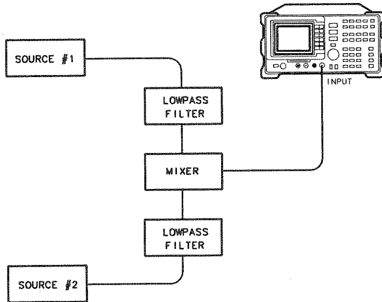
Figure 6-24. Third-Order Intermodulation Equipment Setup
