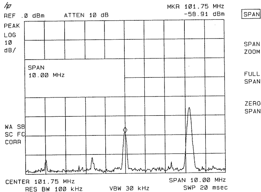
Figure 6-16. Low-Level Signal
