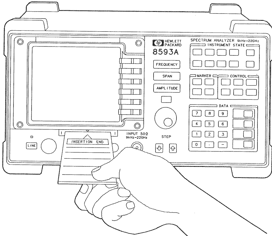
Figure 2-5. Inserting the Memory Card
