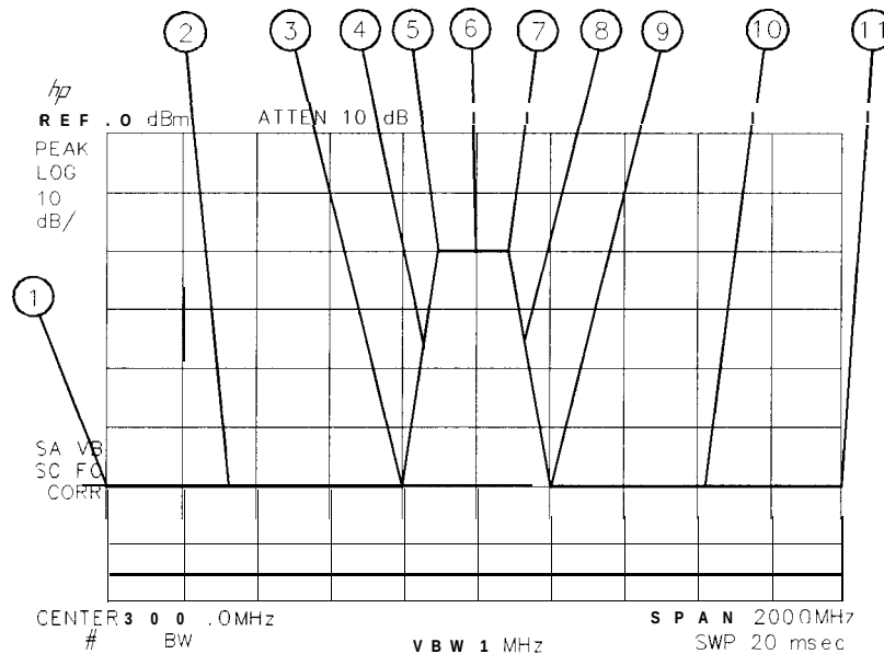
Figure 5-6. Limit-Line Segments
