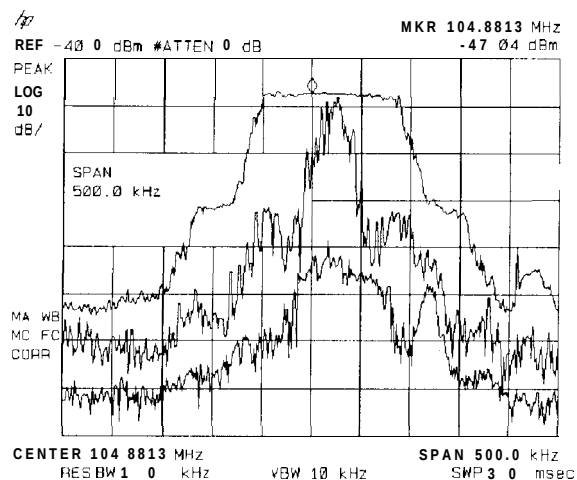
Figure 3-11. Viewing an Unstable Signal With Max Hold, Clear Write, and Min Hold
