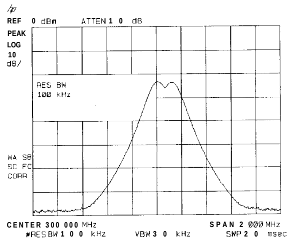
Figure 3-2. Resolving Signals of Equal Amplitude
