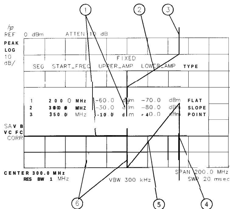
Figure 5-7. Segment Types
