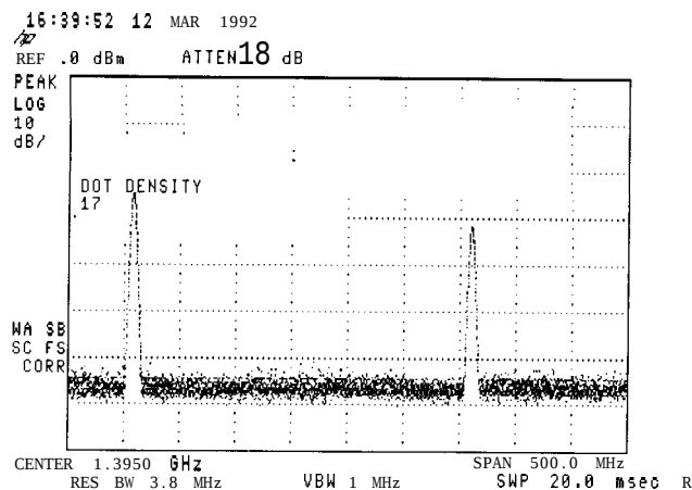
Figure 5-9. Analog + Display Mode
