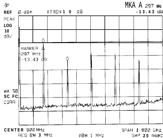
Figure 3-13. Using the Marker Delta Function
