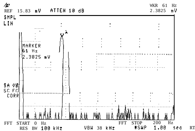
Figure 4-1. FFT Annotation
