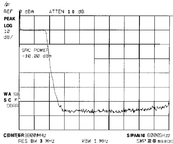
Figure 4-5. Tracking-Generator Output Power Activated
