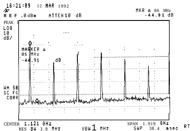
Figure 3-14. Using the Marker to Peak/Peak Function
