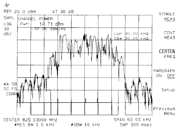
Figure 4-41. Channel Power
