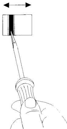
Figure 1-2. Setting the Line Voltage Selector Switch
