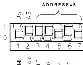
Figure 6-6. HP 7475A Plotter Switch Settings
