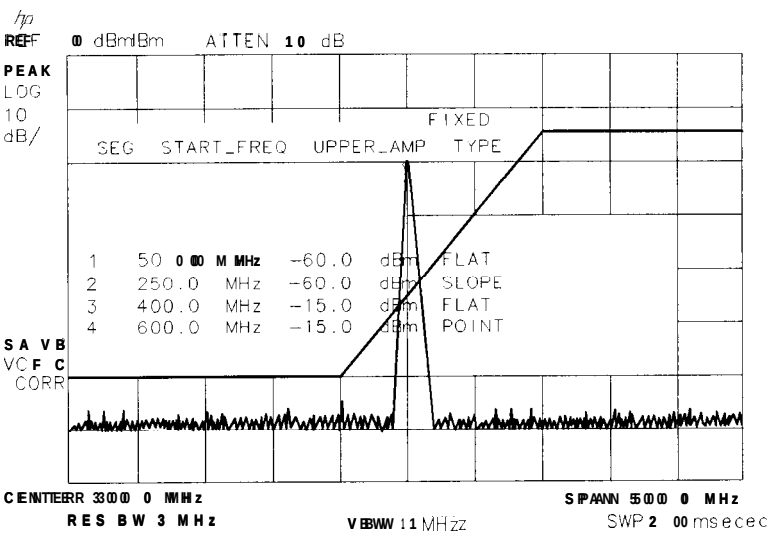
Figure 5-5. The Completed Limit-Line Table
