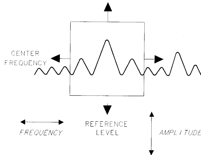
Figure 2-5. Relationship between Frequency and Amplitude
