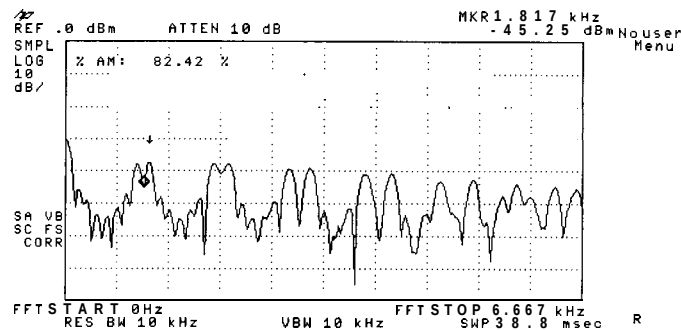
Figure 4-2. Percent Amplitude Modulation Measurement
