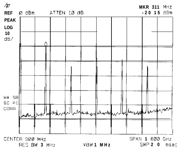
Figure 3-12. Placing a Marker on the CAL OUT Signal
