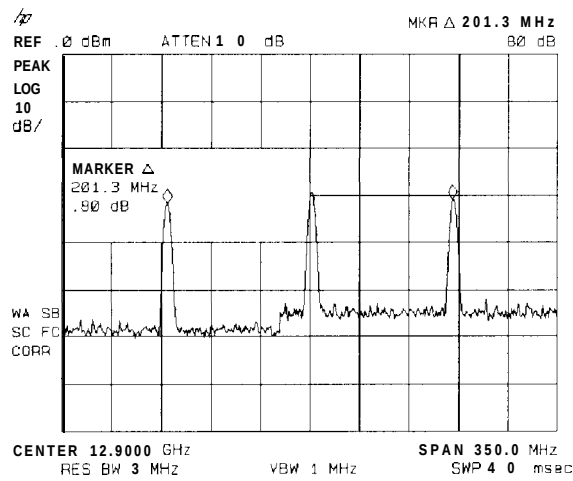
Figure 3-29. Harmonic Locking Off
