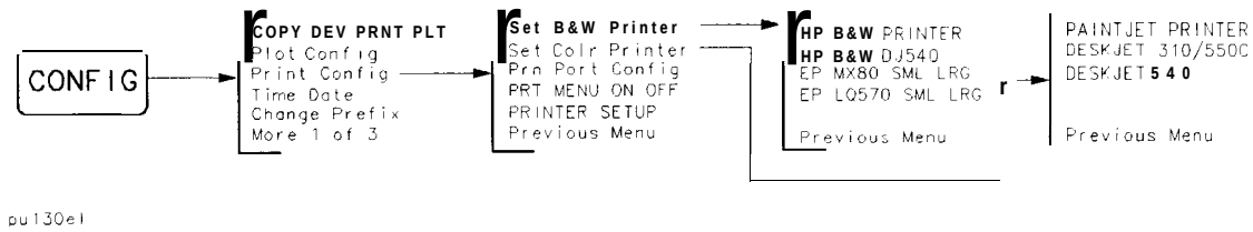
Figure 6-14. Printer Configuration Menu Map
