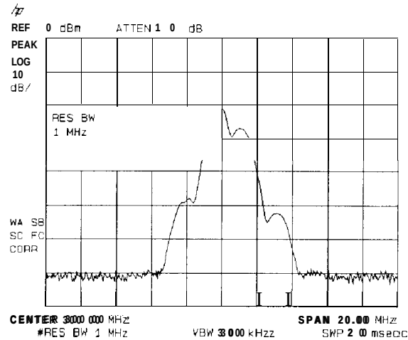
Figure 3-26. Viewing an AM Signal
