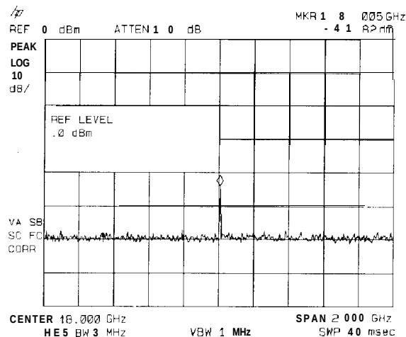
Figure 3-8. Peaking Signal Amplitude Using Preselector Peak
