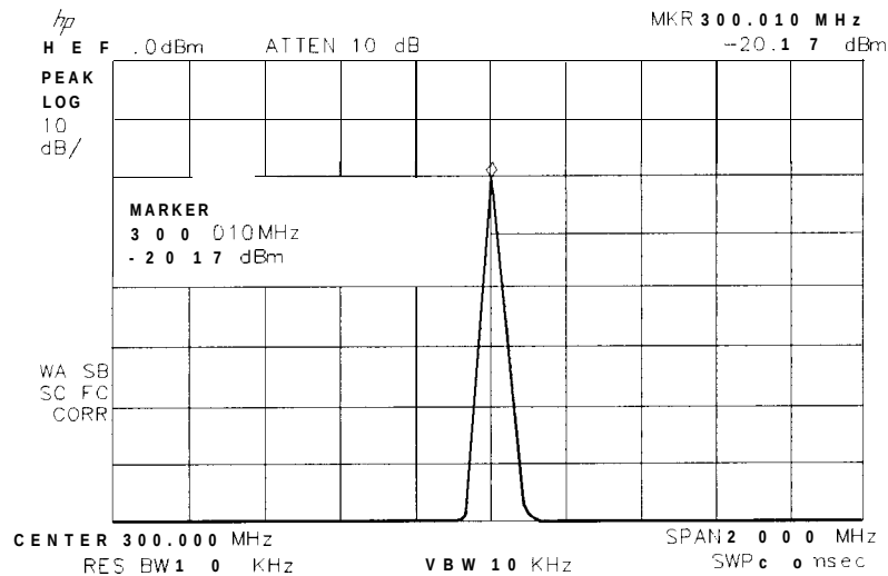
Figure 2-6. Reading the Amplitude and Frequency
