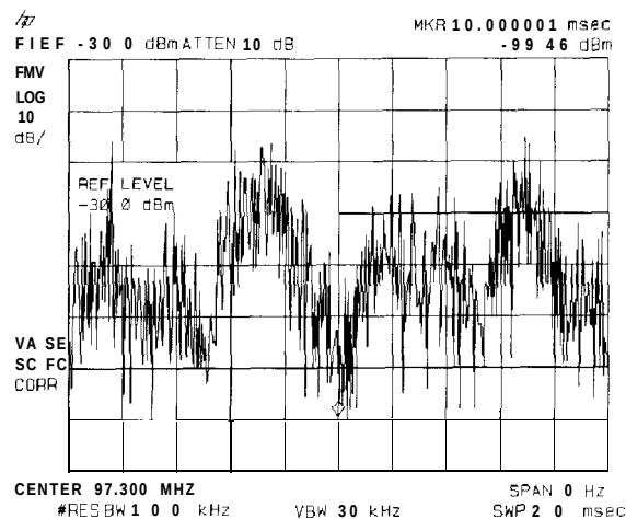
Figure 4-12. Continuous Demodulation of an FM Signal
