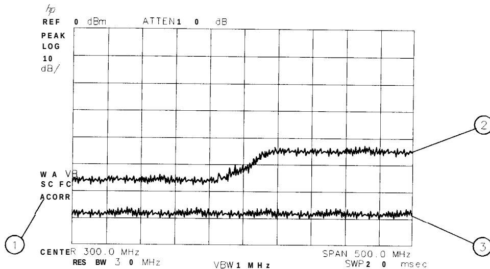
Figure 5-1 1. Amplitude-Correction Display
