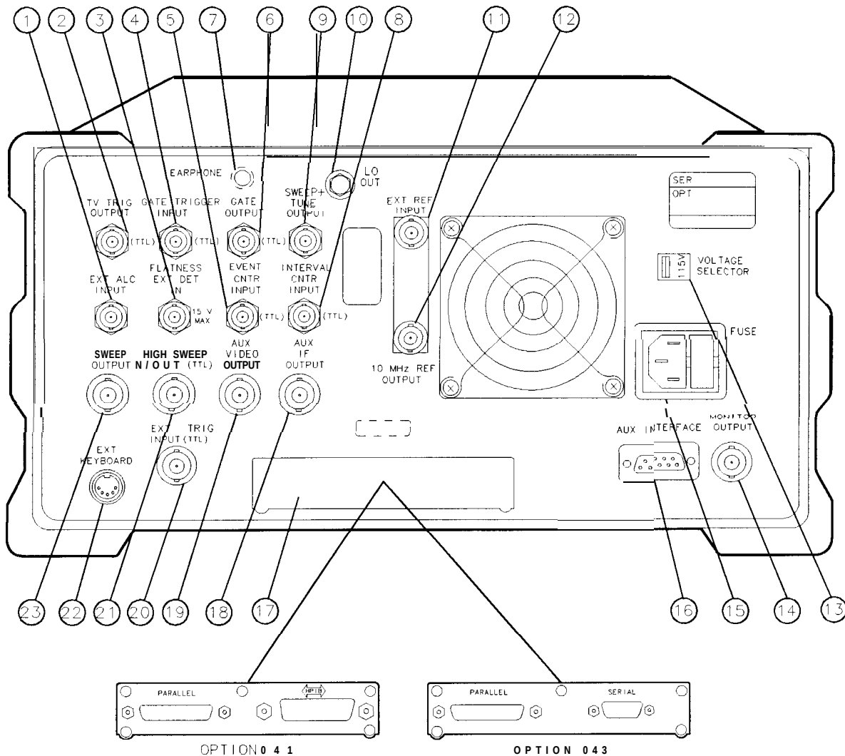
Figure 2-2. Rear-Panel Feature Overview
