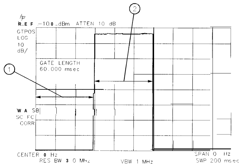
Figure 4-32. Gate On
