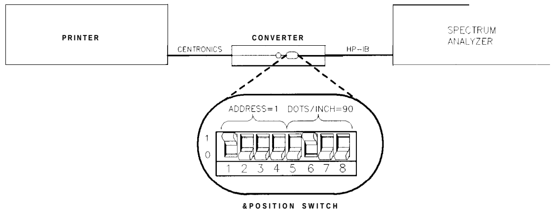
Figure 6-4. HP-IB to Centronics Converter Setup
