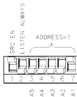
Figure 6-3. ThinkJet Printer Switch Settings
