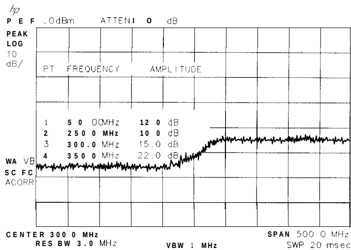
Figure 5-12. Completed Amplitude-Correction Table
