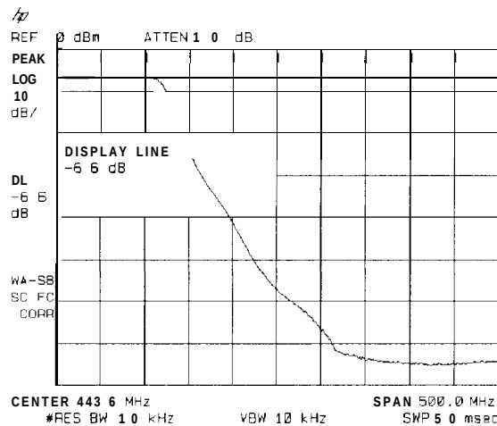
Figure 4-9. Normalized Trace
