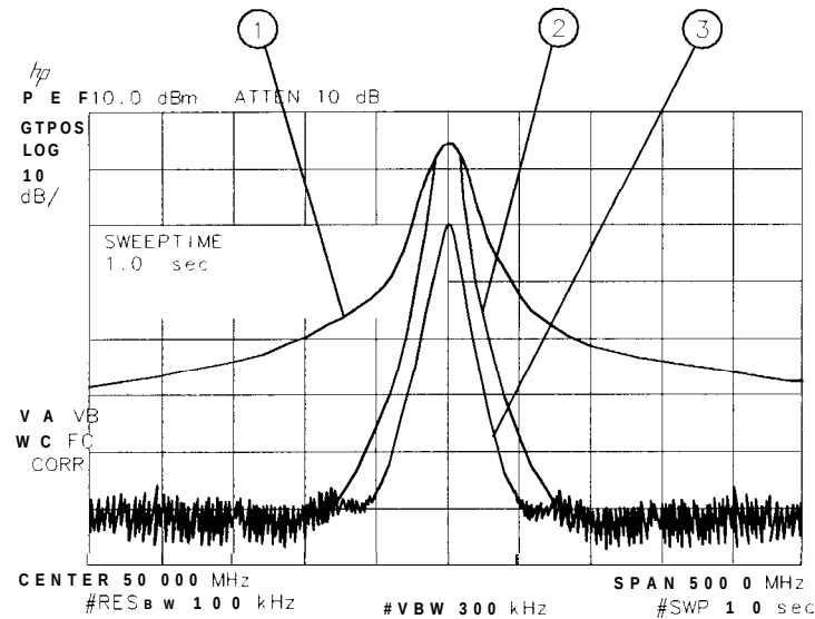
Figure 4-19. Viewing Time-Sharing of a Frequency with a Spectrum Analyzer
