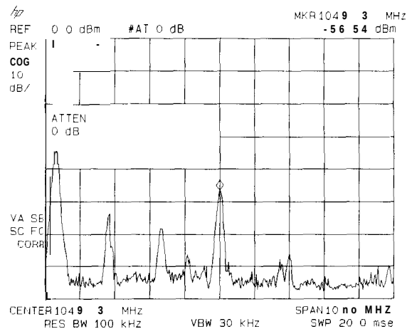
Figure 3-17. Using 0 dB Attenuation
