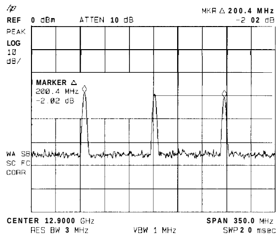
Figure 3-28. Using Harmonic Lock
