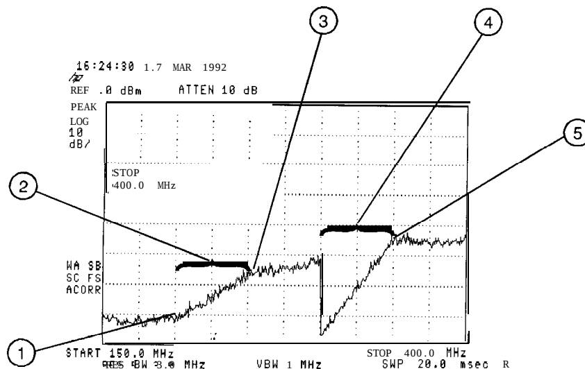
Figure 5-13. Amplitude-Correction Points
