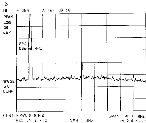
Figure 3-21. Harmonic Distortion
