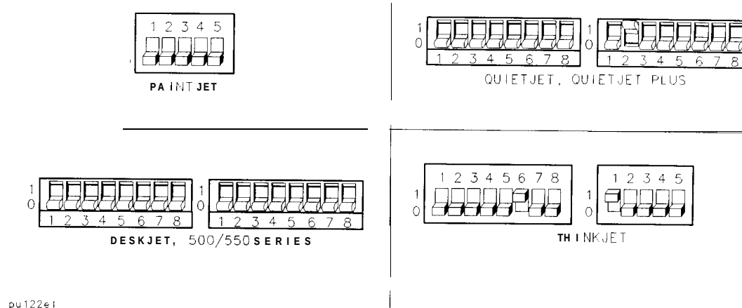
Figure 6-8. 9600 Baud Settings for Serial Printers
