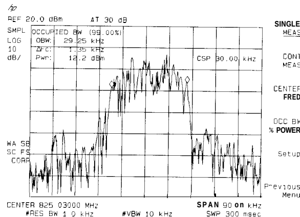
Figure 4-37. Occupied Bandwidth
