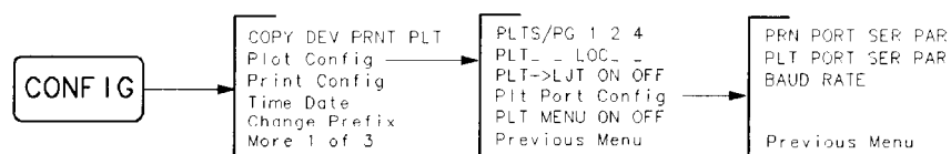
Figure 6-1 1. Baud Rate Menu Map
