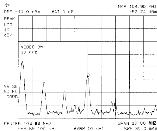
Figure 3-19. Decreasing Video Bandwidth
