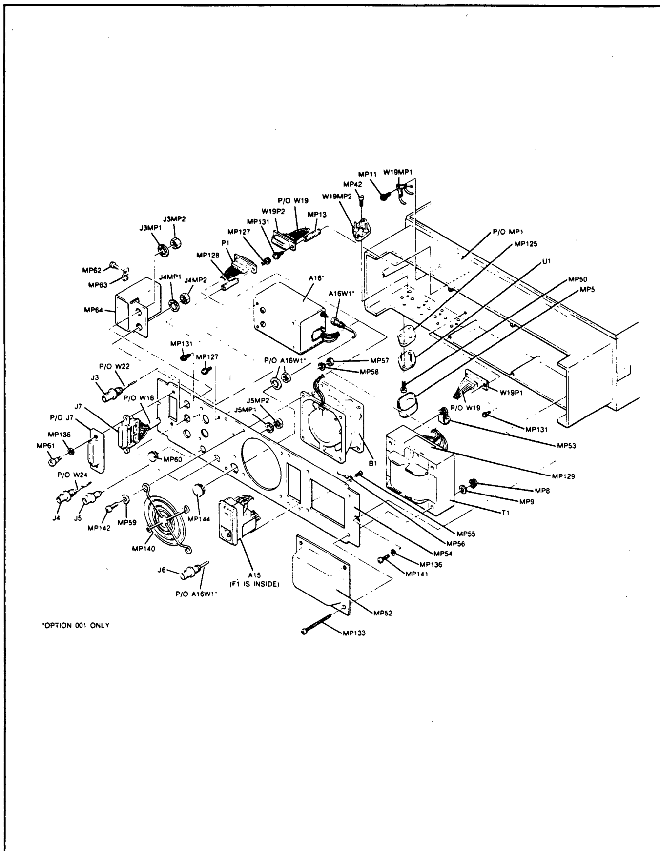
Figure 6-3. Exploded View of the Rear Panel
