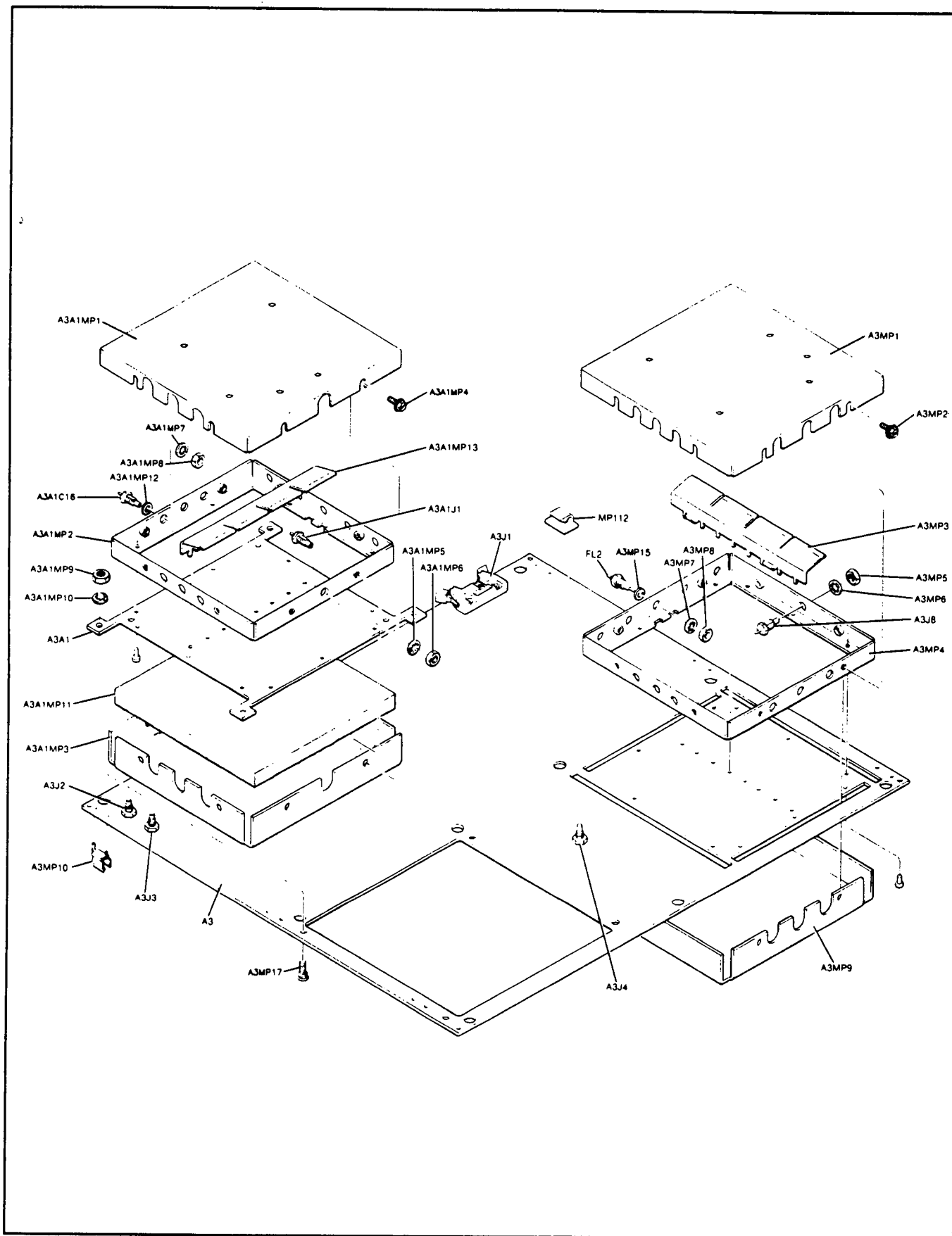
Figure 6-4. Exploded View of the A3A1 Assembly
