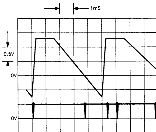
Figure 3. VCO Tune and Beatnote Detector.
