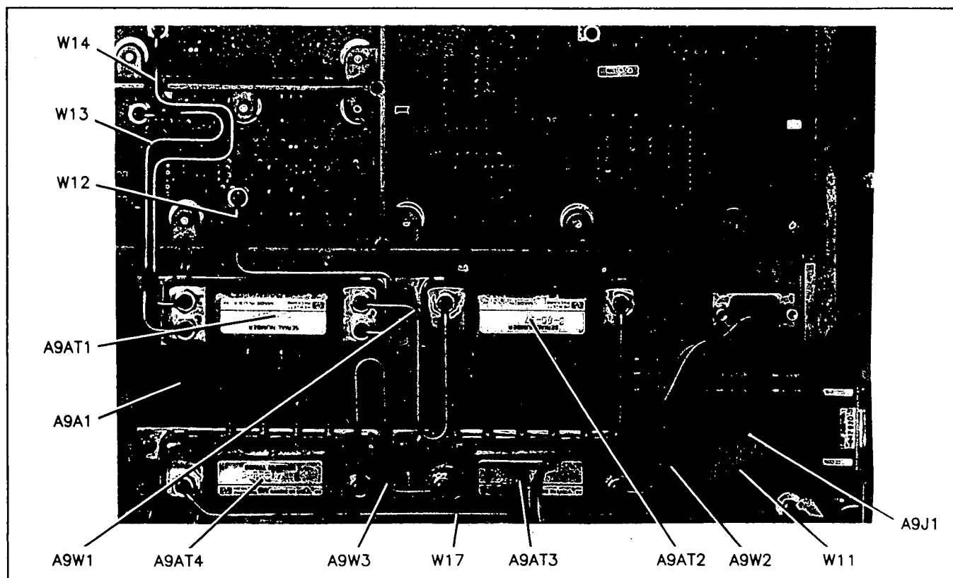
Figure 8-4. Attenuator Assembly A9.
