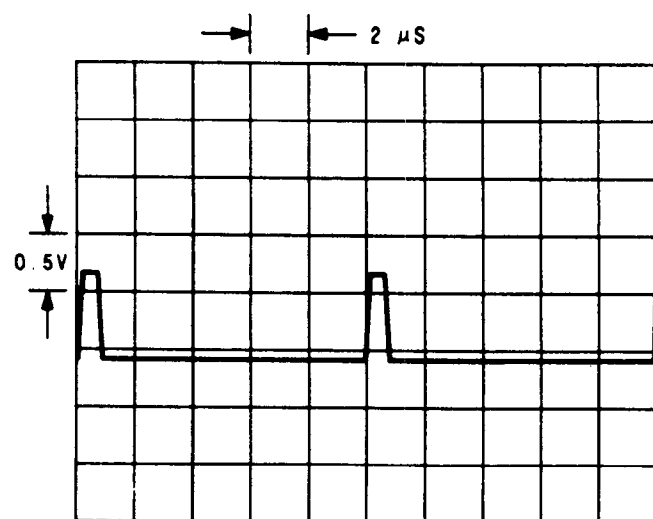
Figure 6. Oscilloscope Display of TP12 W3 to W3A position, Low Frequency Loop locked, Signal Generator's frequency 990 MHz.
