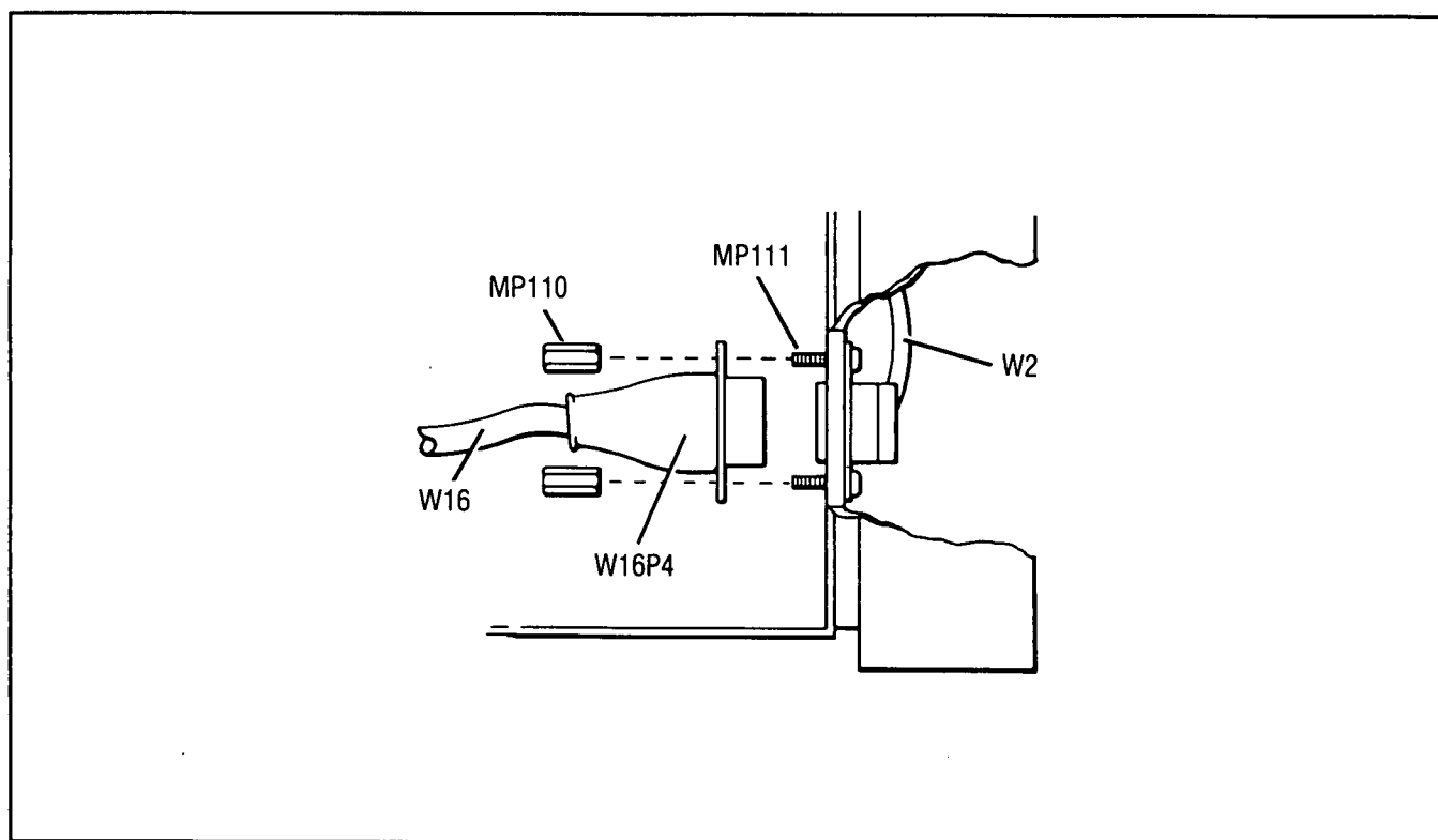
Figure 8–2. P/O A10/A11 Assembly Service Positioning.
