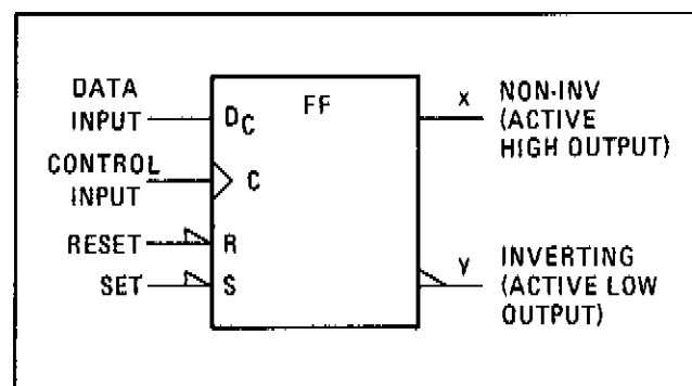
Figure 8-116. D-Type Flip-Flop (Edge-Triggered)
