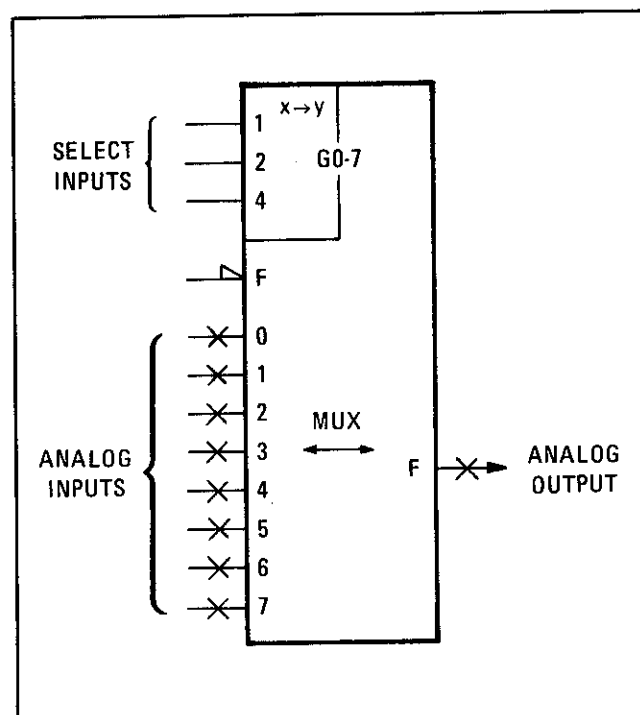
Figure 8-120. Analog Multiplexer
