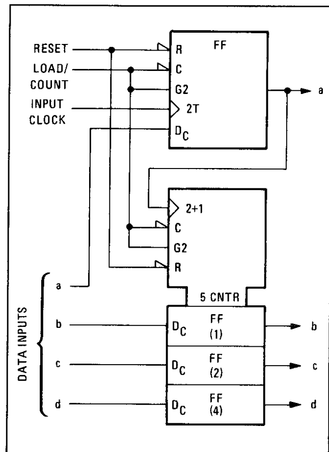
Figure 8-118. Presettable Counter
