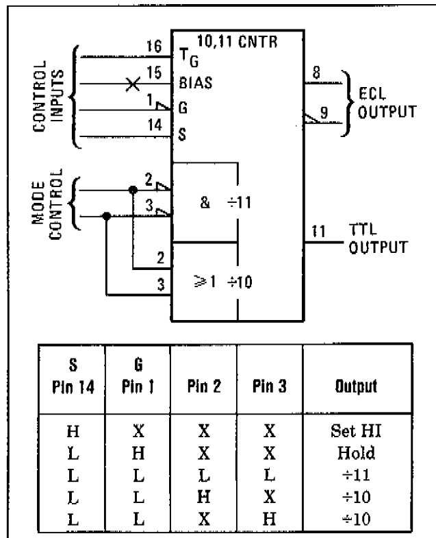
Figure 8-123. Divide-By-10/11 Prescaler
