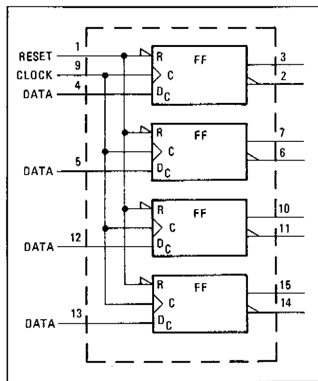
Figure 8-108. Quad D-Type Latch (Individual)
