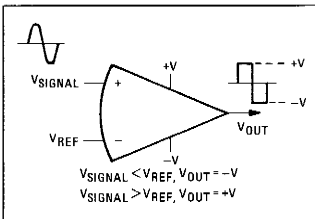
Figure 8-133. Non-Inverting Comparator
