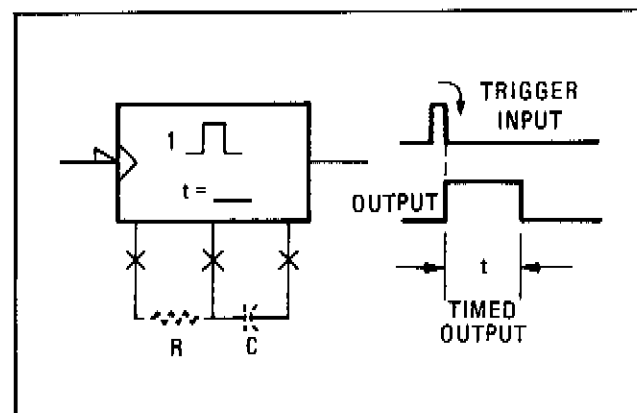
Figure 8-115. One-Shot Multivibrator
