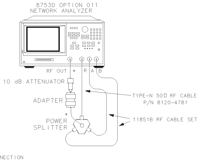
Figure 6-16. Receiver Trace Noise Test Setup
