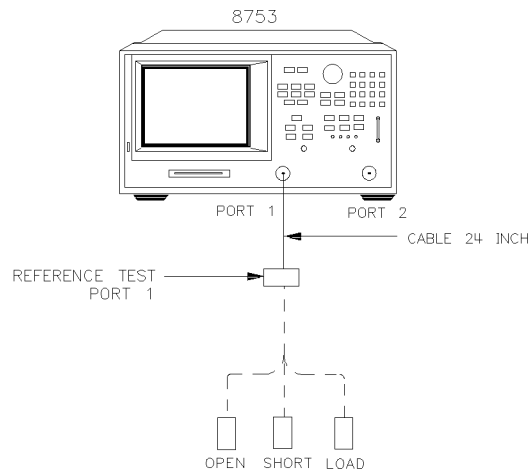
Figure 4-26. S11 1-Port Cal Test Setup
