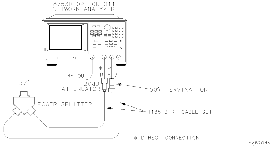
Figure 6-14. B into A Receiver Input Crosstalk Test Setup
