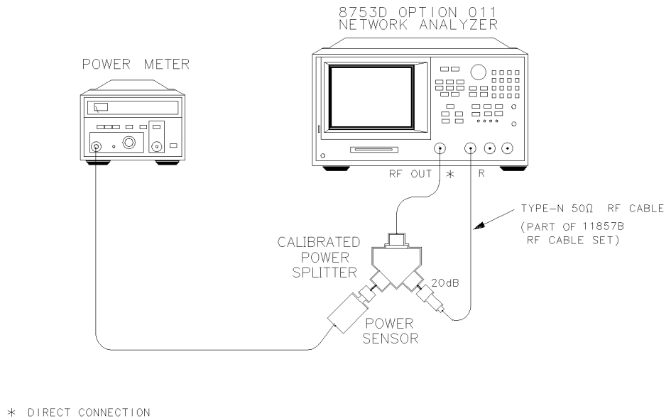
Figure 6-4. Power Range, Linearity, and Accuracy Test Setup
