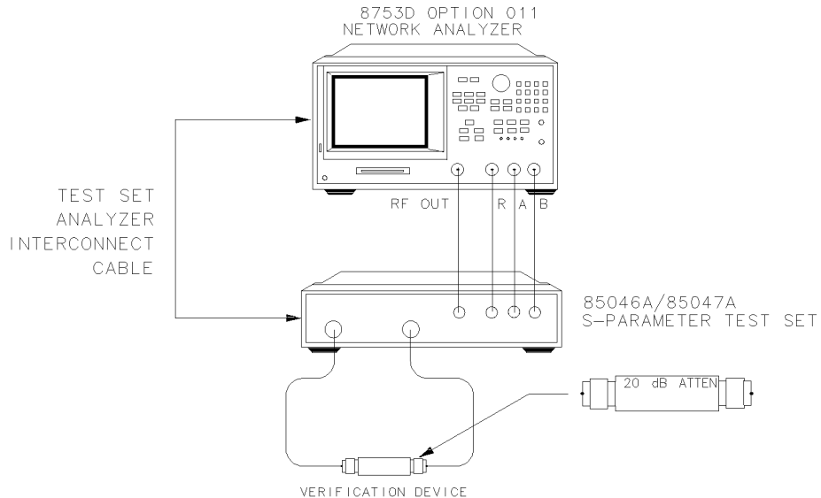
Figure 5-4. Connections for the 20 dB Verification Device
