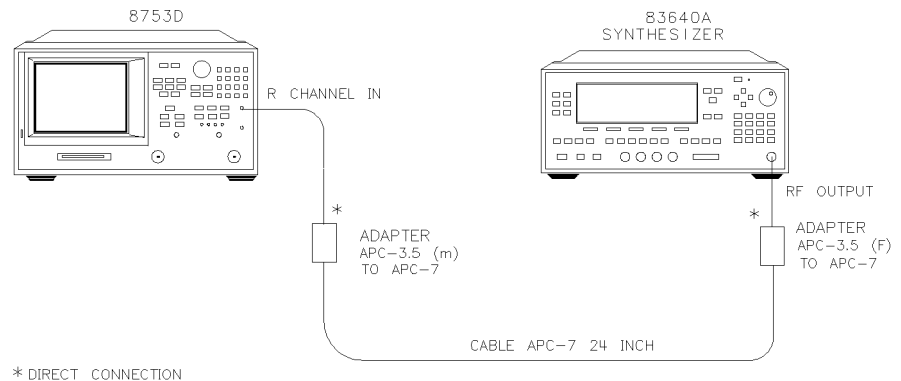
Figure 4-2. External Source Mode Frequency Range Test Setup
