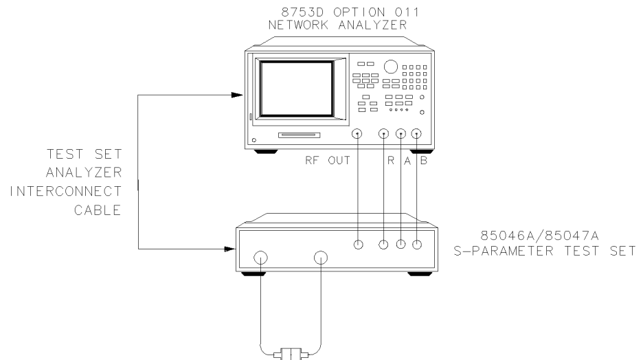
Figure 5-3. Transmission Calibration Setup
