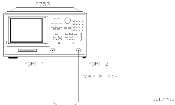
Figure 4-35. Test Port Phase Compression Test Setup
