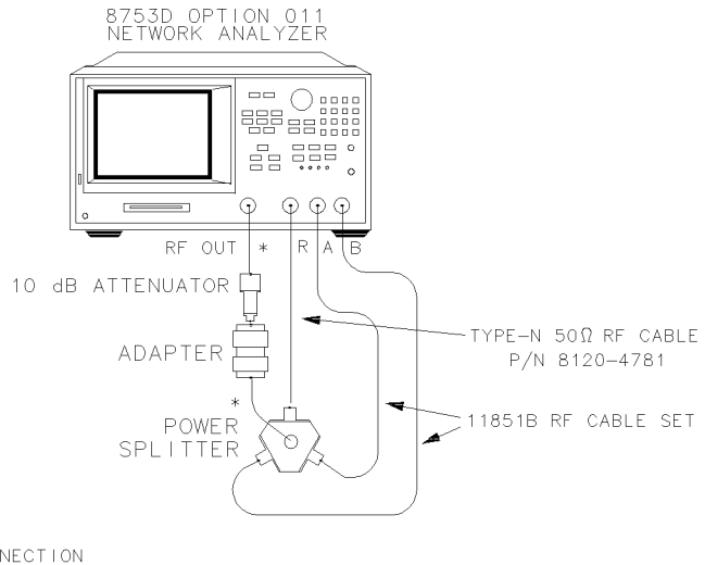
Figure 6-12. Phase Frequency Response Test Setup
