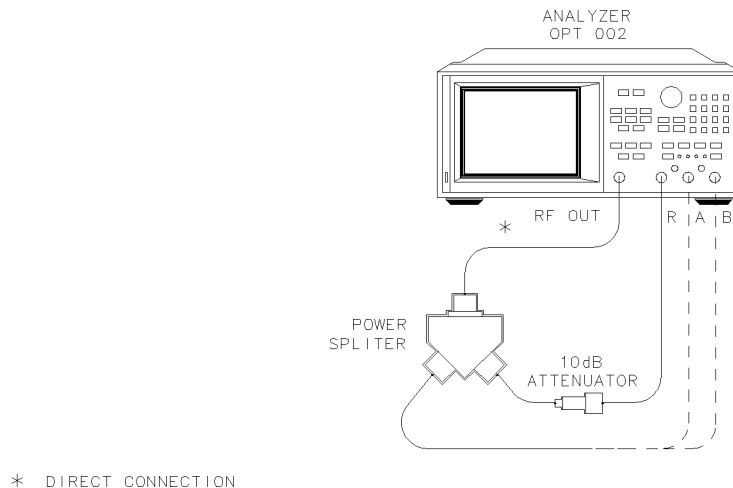
Figure 6-34. Receiver Harmonics Test Setup
