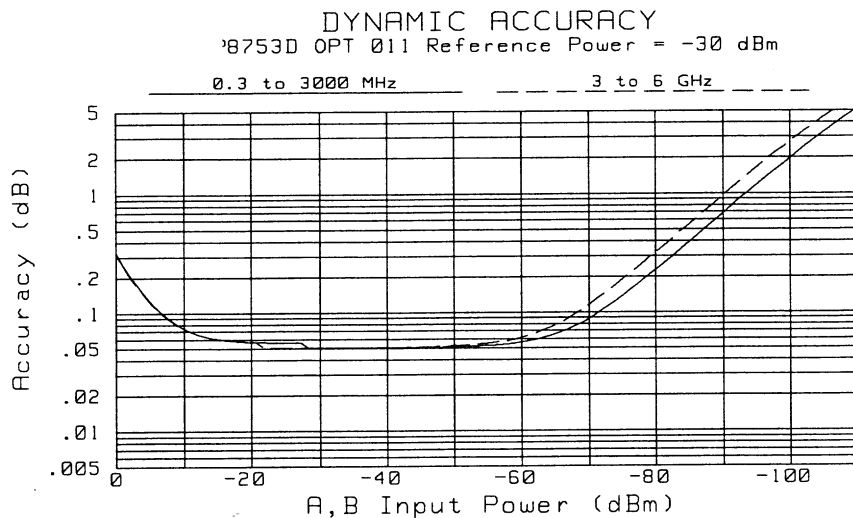
Figure 6-21. Receiver Magnitude Dynamic Accuracy
