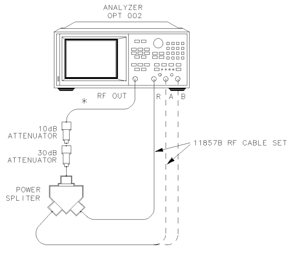
Figure 6-32. Source Harmonics Test Setup
