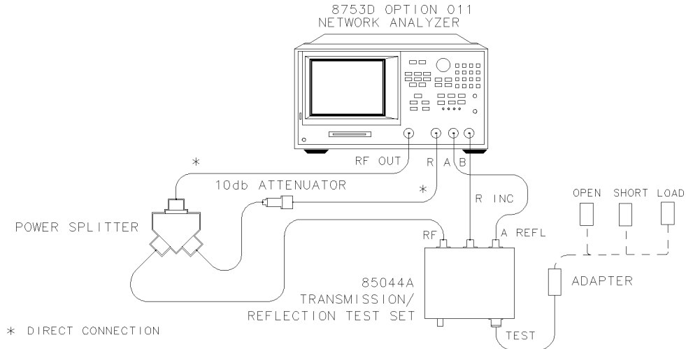
Figure 6-19. Receiver R Input Impedance Test Calibration Test Setup
