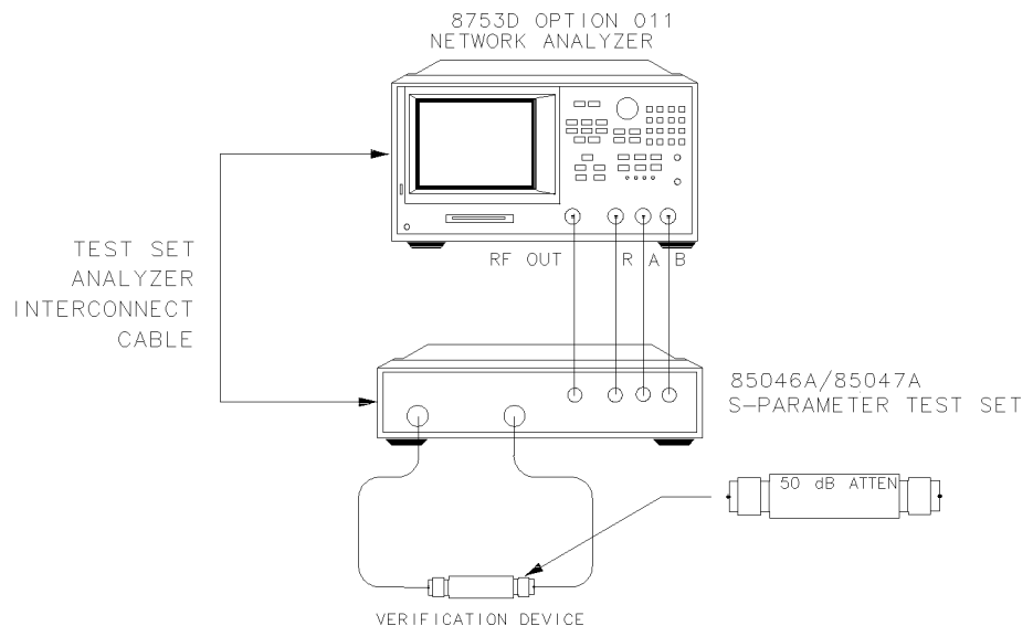
Figure 5-5. Connections for the 50 dB Verification Device
