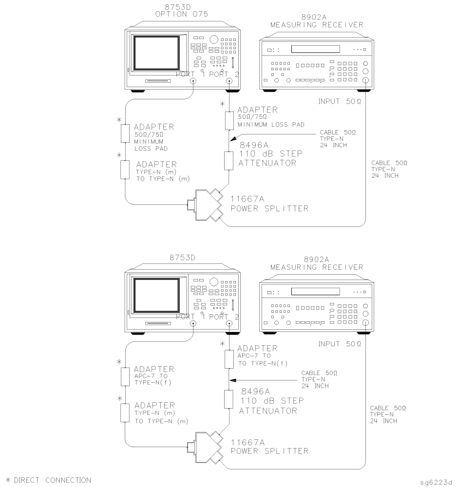
Figure 4-32. Test Port 1 Magnitude Dynamic Accuracy Test Setup
