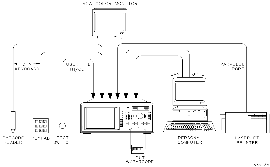
Figure 3-1 Example Test System Setup
