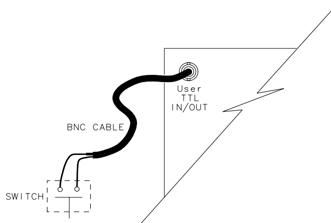
Figure 4-1 Connect a Switch to the USER TTL IN/OUT Connector
