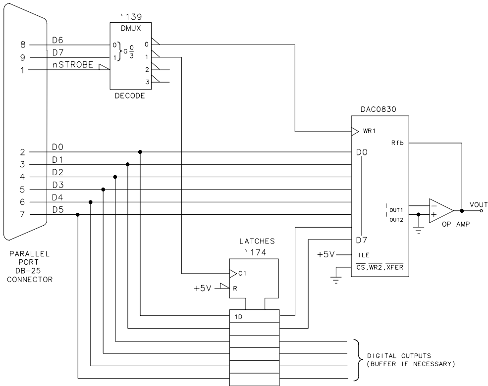
Figure 6-2 Digital Latch Circuit
