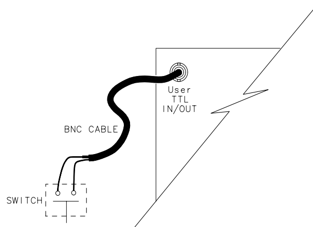
Figure 3-2 Connecting a Switch to the USER TTL IN/OUT Connector
