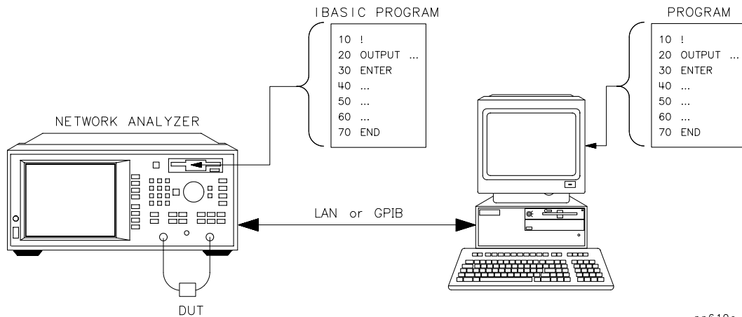
Figure 2-3 Network Analyzer Running IBASIC, Controlled by a Computer
