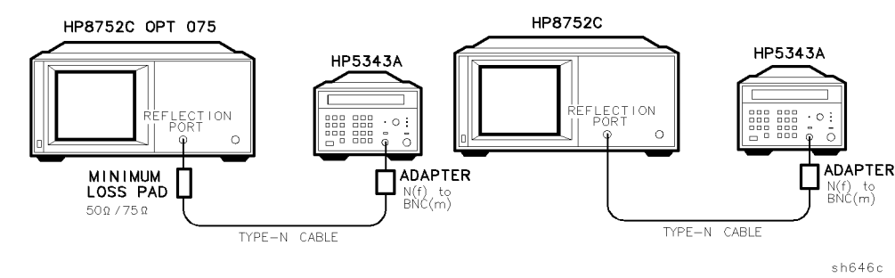
Figure 3-17. Reflection Test Port Output Frequency Accuracy Adjustment Setup
