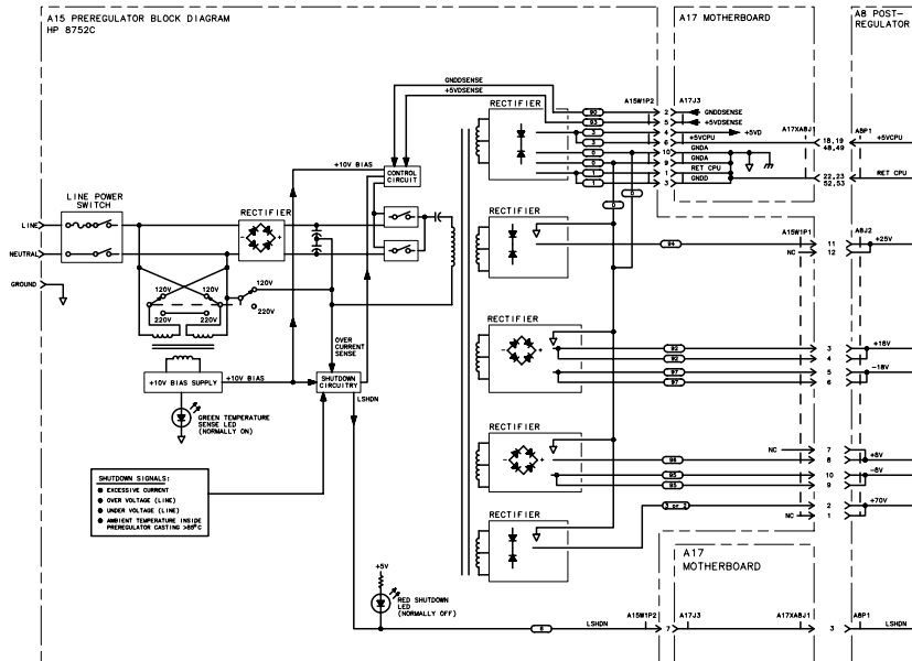
A15 PRE-REGULATOR
