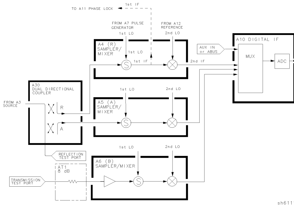
Figure 12-8. Receiver Functional Group (Option 006)
