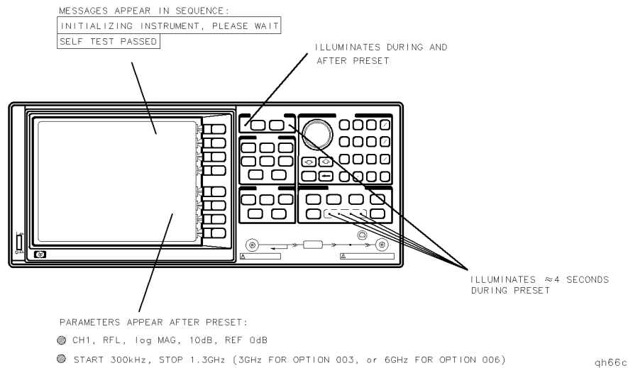
Figure 6-4. Preset Sequence
