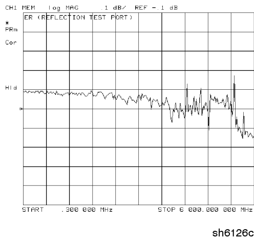
Figure 11-6. Typical E_R (Reflection Test Port)
