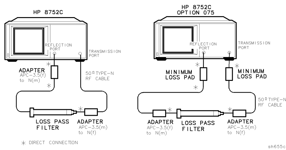
Figure 3-6. Cavity Oscillator Frequency Correction Constant Setup
