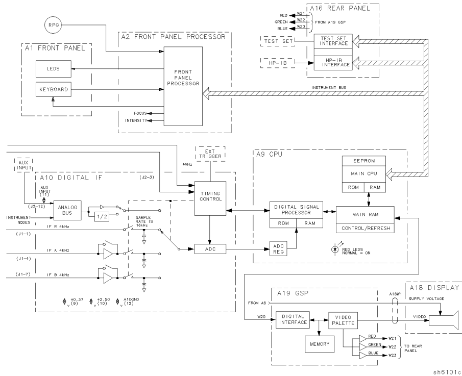
Figure 6-1. Digital Control Group Block Diagram
