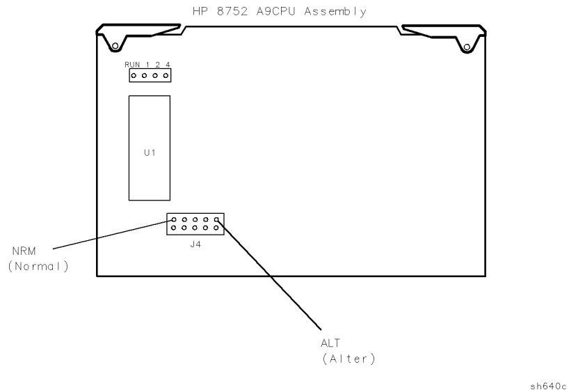
Figure 10-2. Jumper Positions on the A9 CPU
