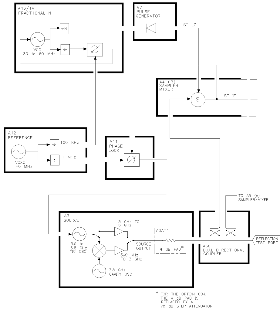
Figure 12-5. High Band Operation of the Source
