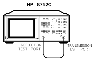
Figure 2-6. Transmission Test Port Input Noise Floor Level Test Setup 1
