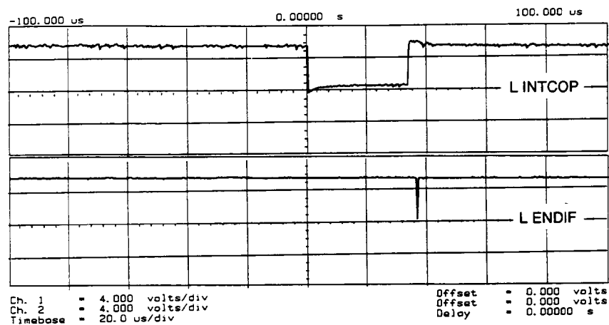
Figure 8-6. Digital Control Lines Observed Using L INTCOP as Trigger
