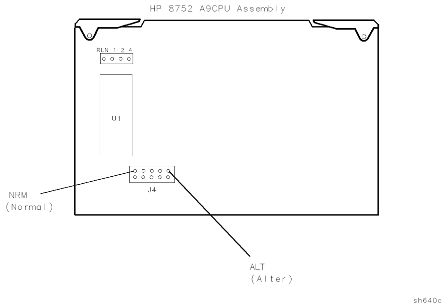
Figure 3-2. NRM (Normal) and ALT (Alter) Positions of A9 CC Jumper
