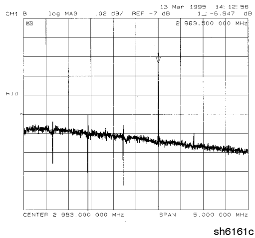
Figure 3-10. Typical Display of Five Spurs without Filter
