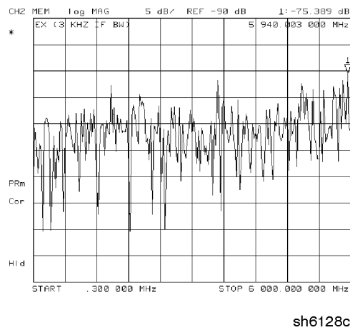
Figure 11-8. Typical E_X with 3 kHz Bandwidth
