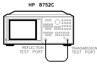
Figure 2-10. Transmission Test Port Input Noise Floor Level Test Setup 1
