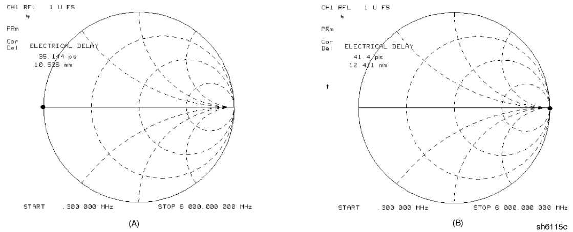
Figure 9-2. Typical Smith Chart Traces of Good Short (a) and Open (b)
