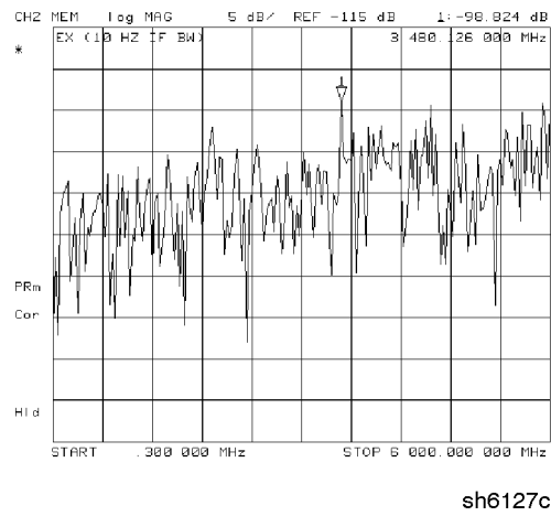
Figure 11-7. Typical E_X with 10 Hz Bandwidth
