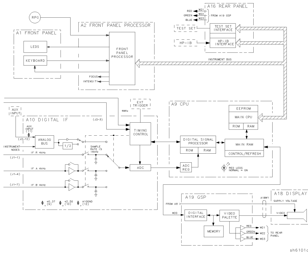
Figure 12-3. Digital Control Group, Block Diagram
