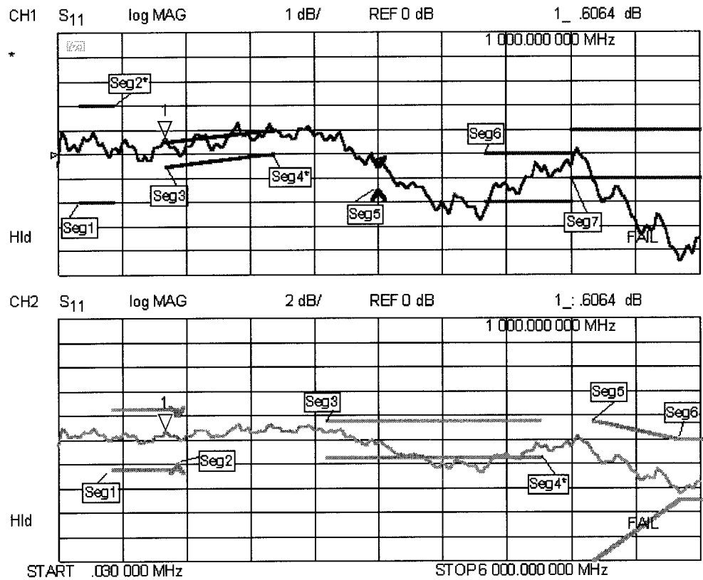
Figure 1-4 Limit Segments Versus Limit Lines
