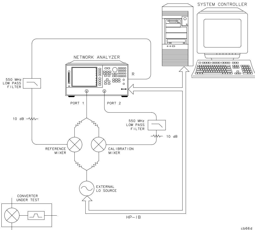
Figure 1-3 Connections: Comparison of Two Mixers — Group Delay, Amplitude or Phase
