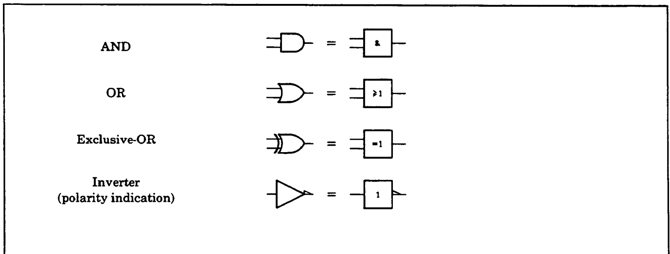
Figure 8-37. Gate Symbols
