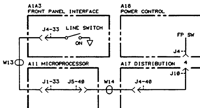
Figure 8-15. FPSW Signal Path
