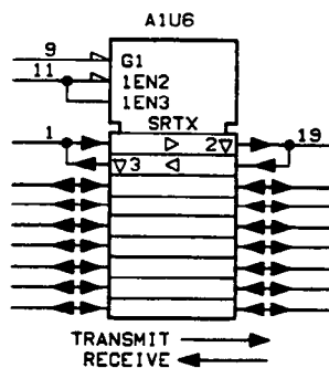
Figure 8-39. 3-State Bidirectional Transceiver
