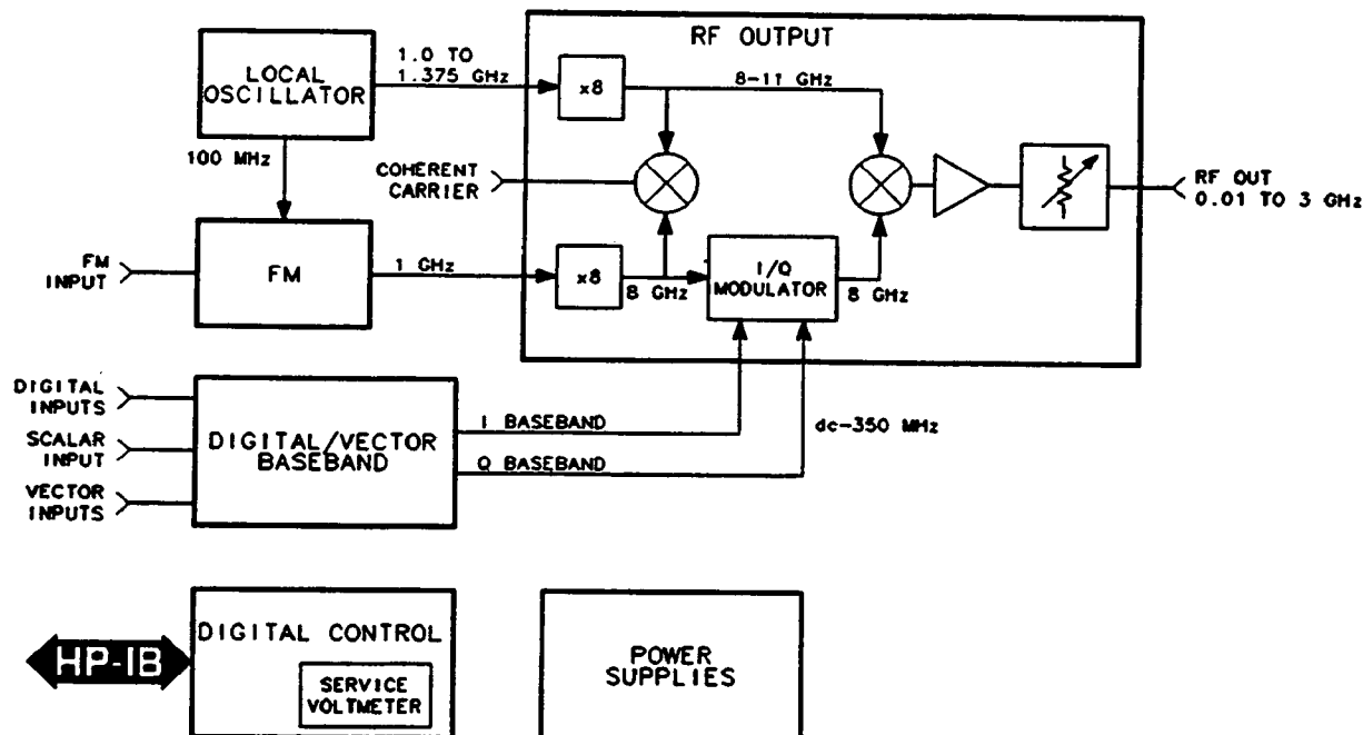
Figure 8-1. Simplified Block Diagram
