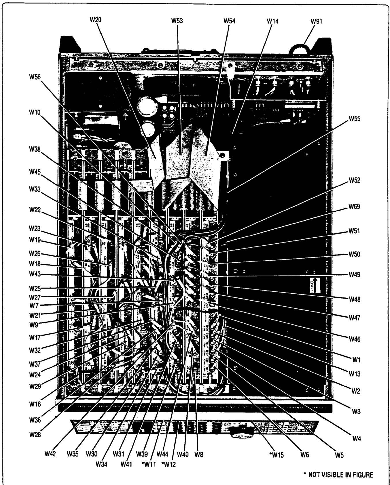
Figure 6-9. Frame Cabling
