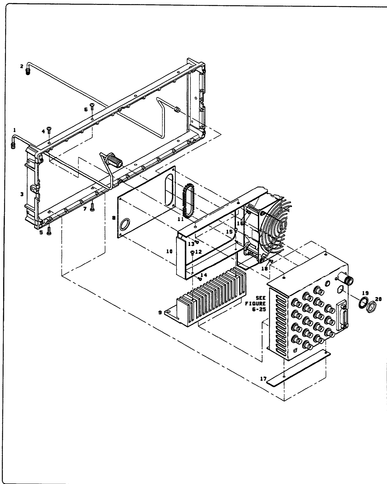
Figure 6-24. Partial Rear Panel (Option 001)
