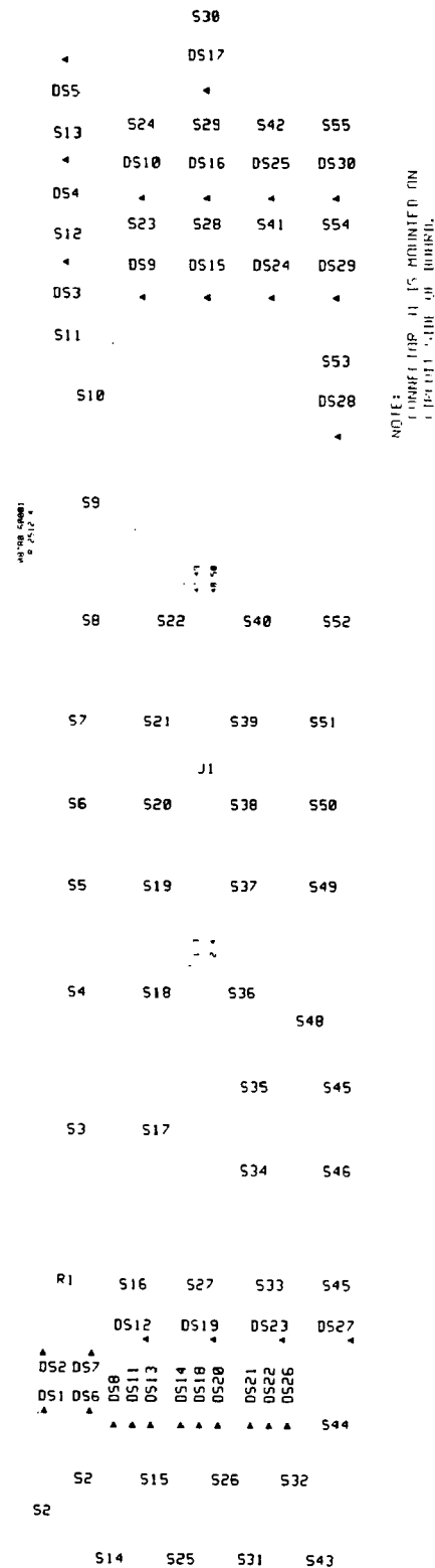
Figure 8-17. A1A2 Keyboard Assembly Component Locations
