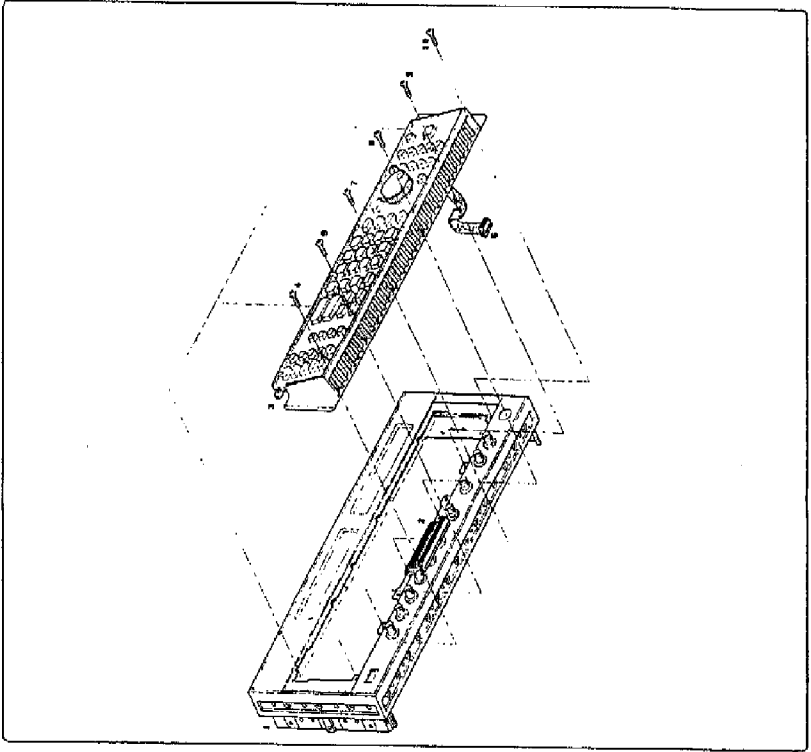
Figure 8-13. Frame Removal
