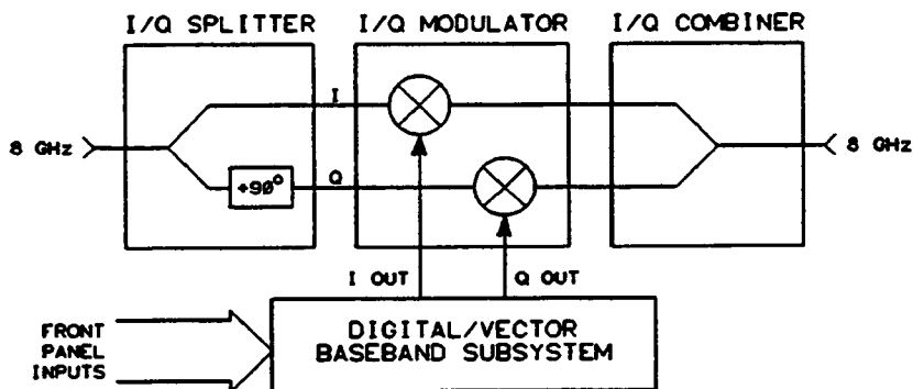
Figure 8-9. Vector Modulation
