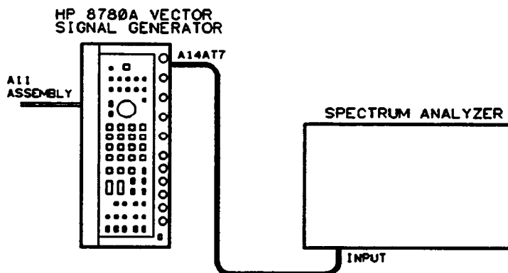
Figure 5-3. LO Multiplier SRD Adjustment Setup
