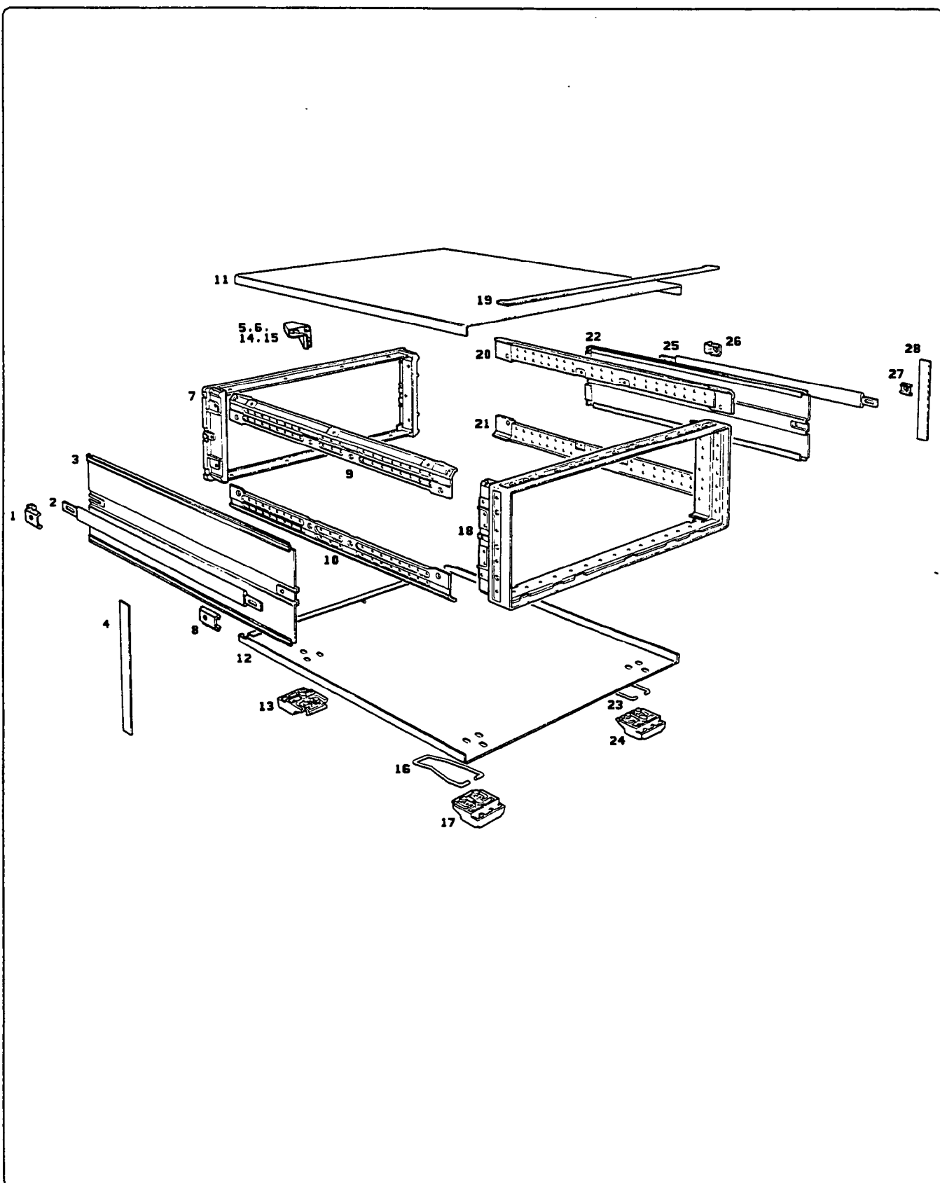
Figure 6-2. Cabinet Parts
