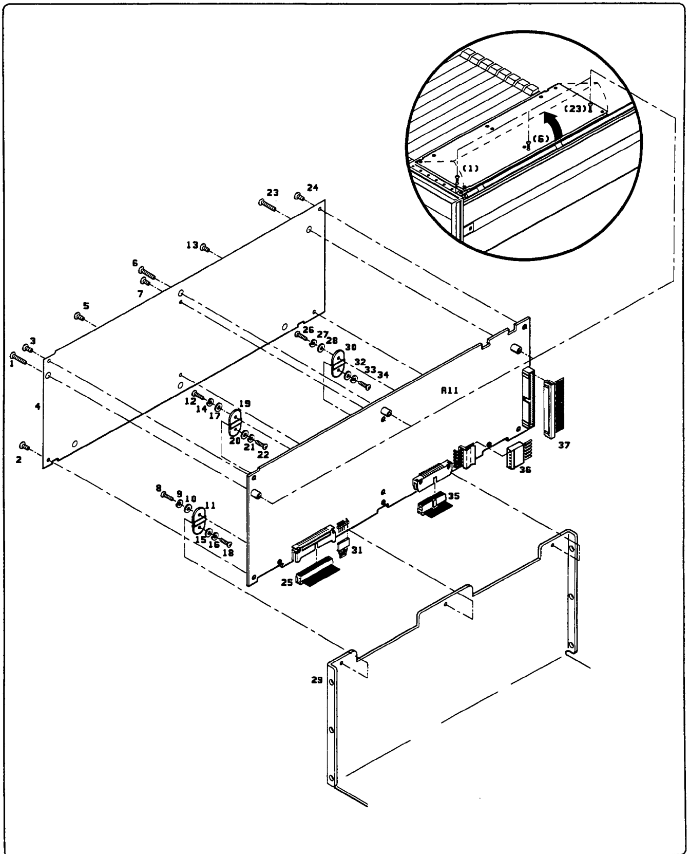
Figure 6-12. Microprocessor Assembly (Plate, Hinging, Cabling)
