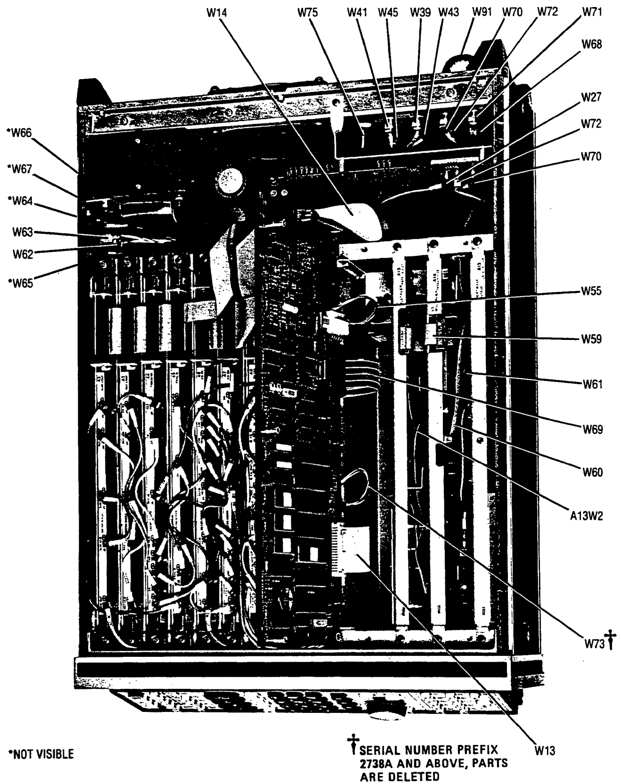
Figure 6-10. Deck and Rear Panel Cabling
