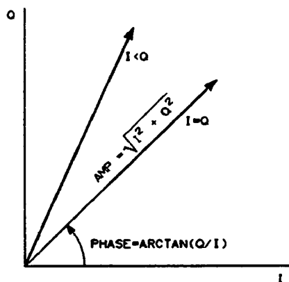
Figure 8-8. Vector Components
