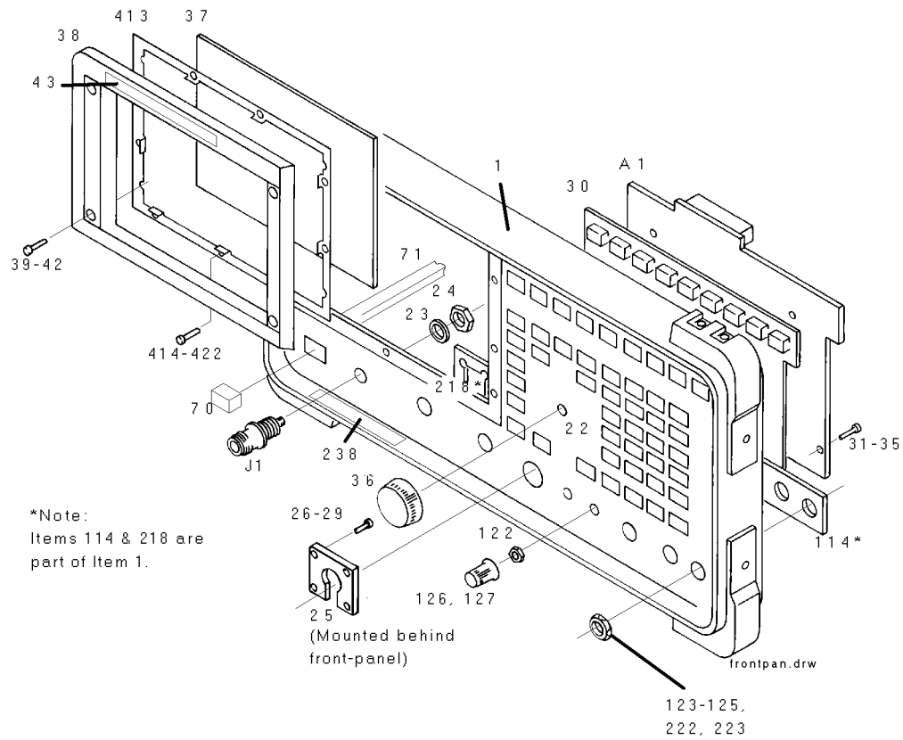
Front Panel
