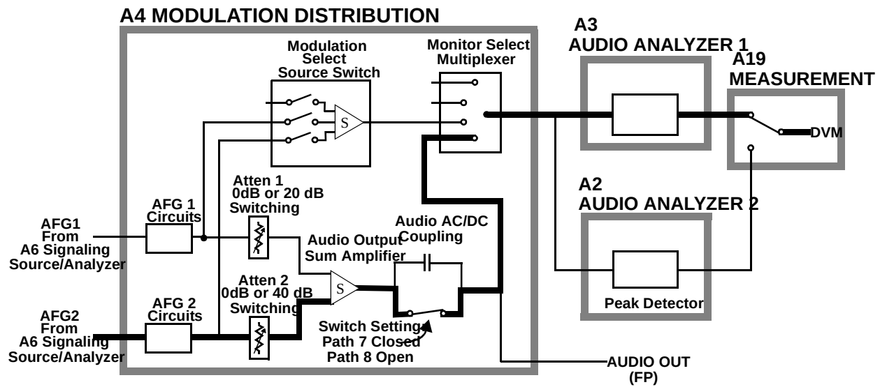
Figure 62 Preliminary Audio Path 7 and 8
