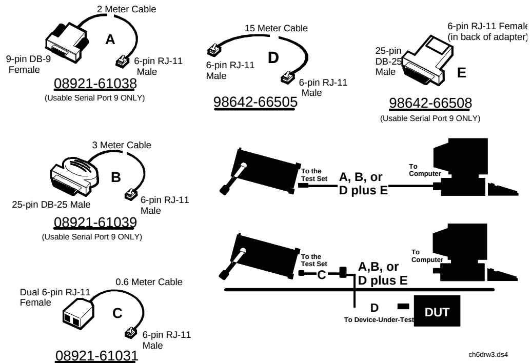
Figure 25 Available Agilent RS-232 Serial Cables and Adapters
