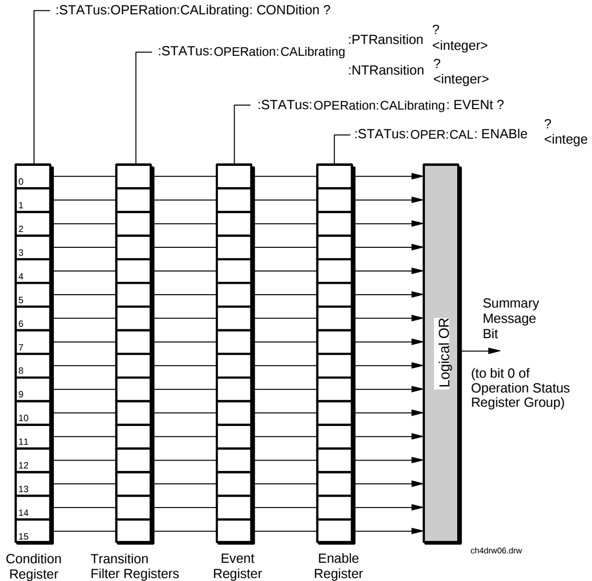
Figure 11 Calibrating Status Register Group
