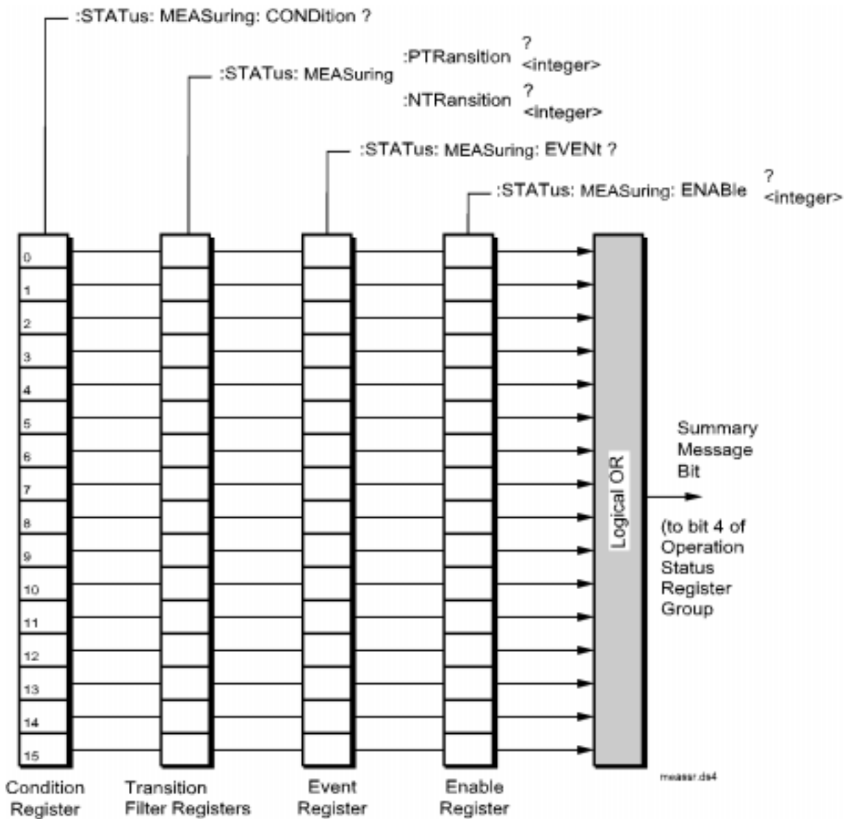
Figure 22 Measuring Status Register Group
