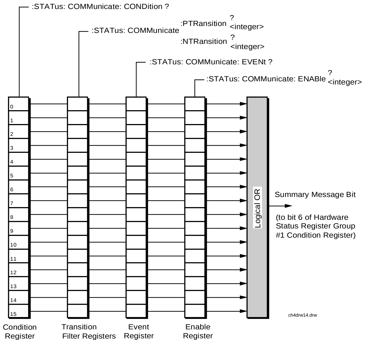
Figure 18 Communication Status Register Group
