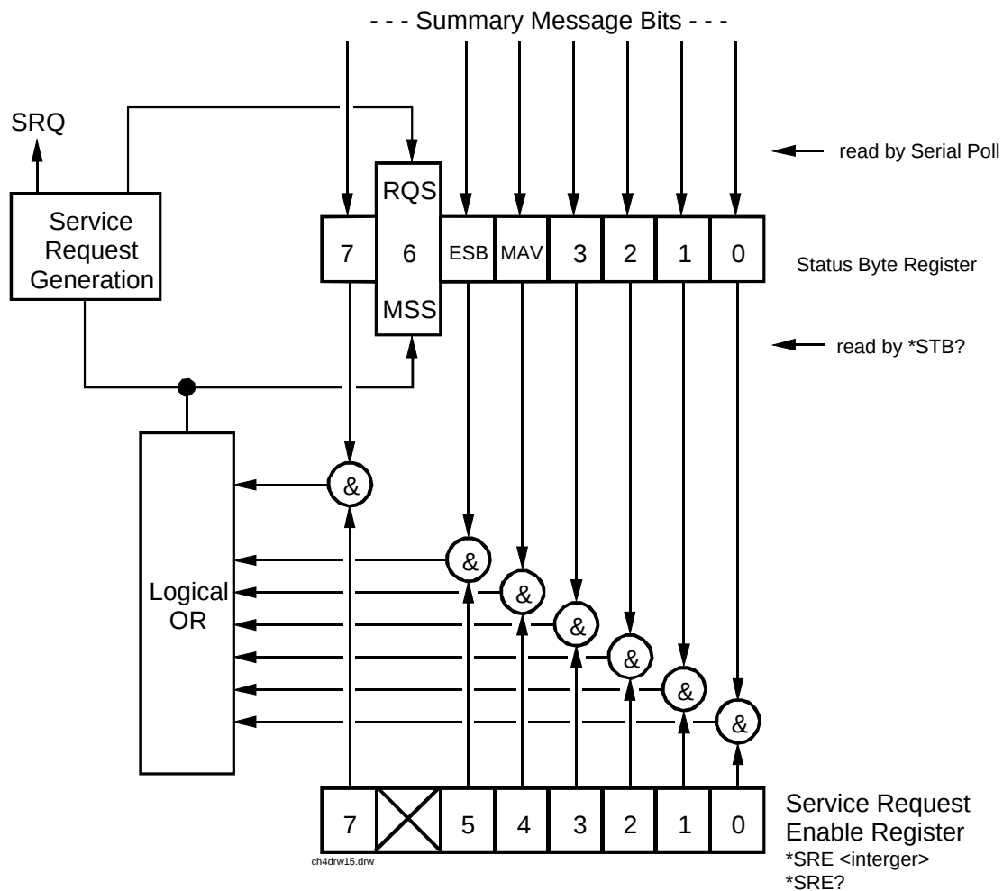
Figure 29 Status Byte/Service Request Enable Register
