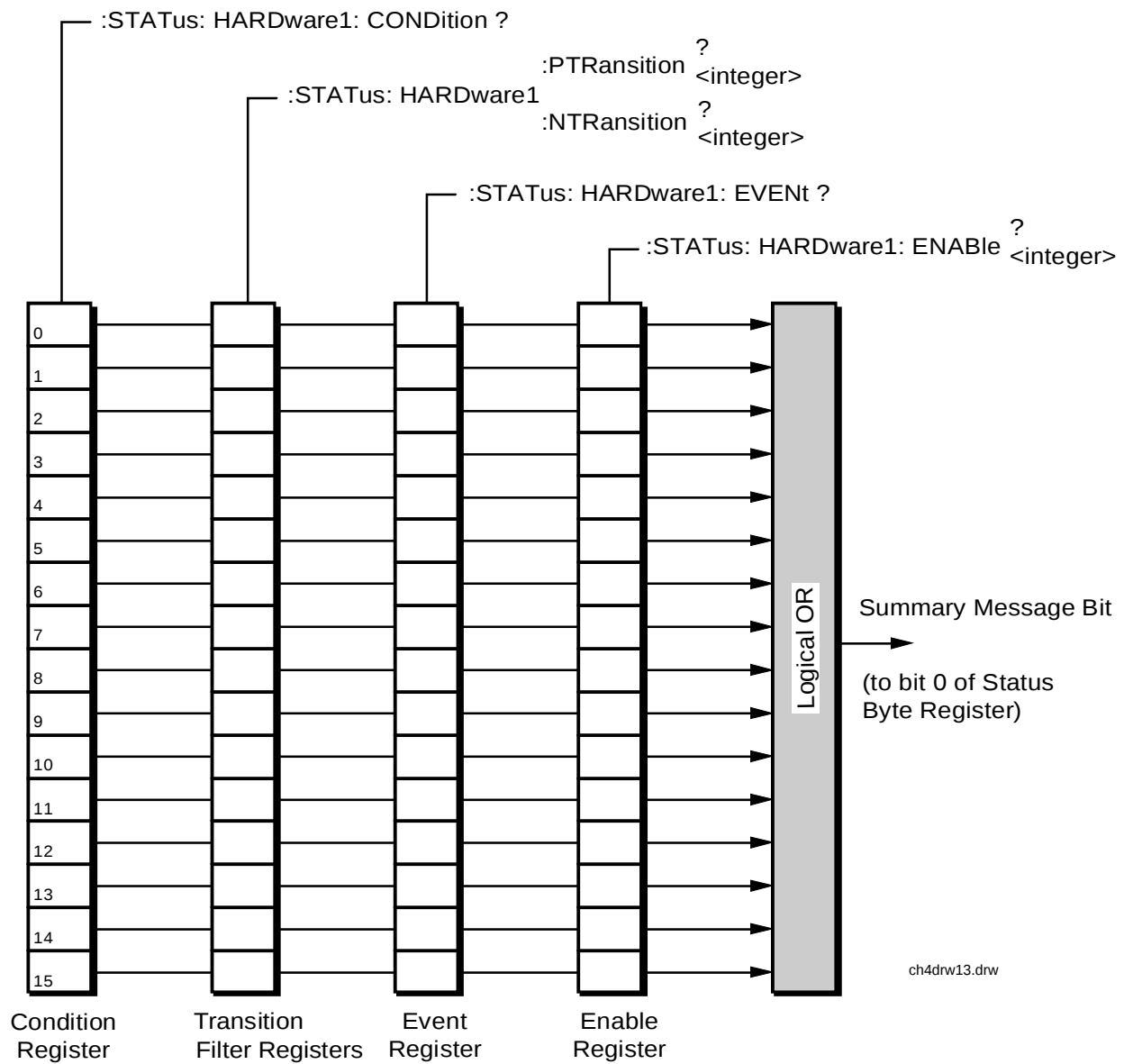
Figure 20 Hardware 1 Status Register Group
