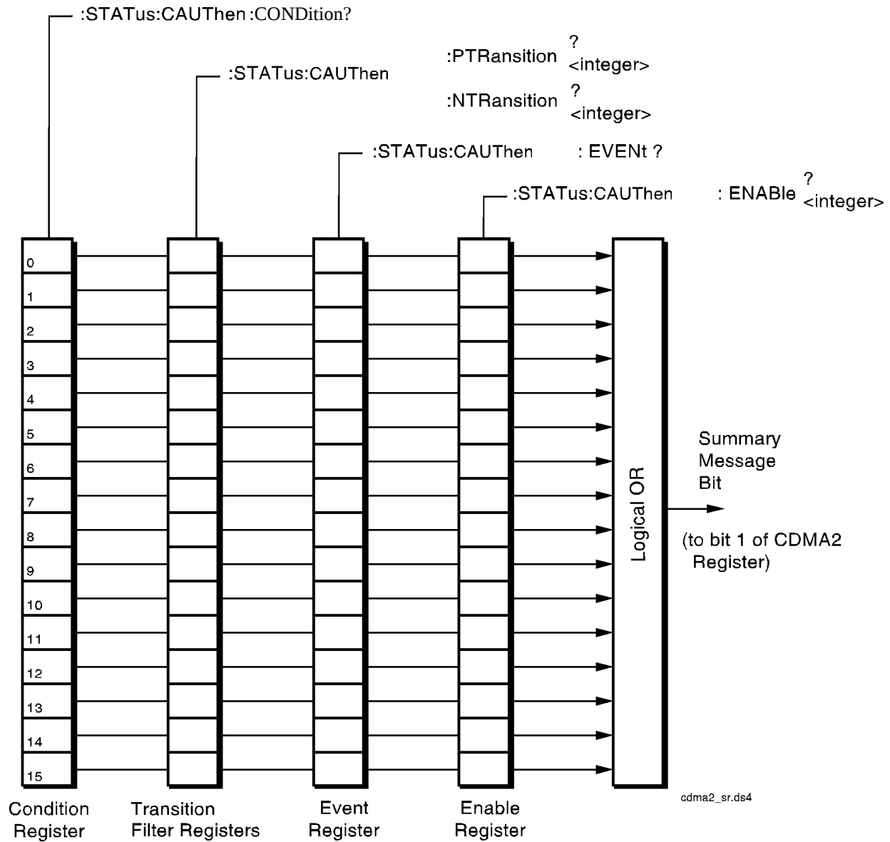
Figure 14 CDMA Authentication Status Register Group
