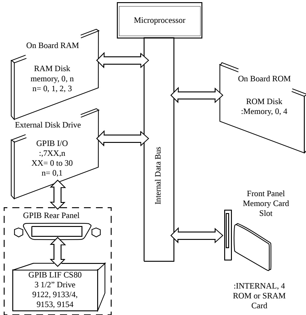
Figure 30 Internal and External Mass Storage Devices
