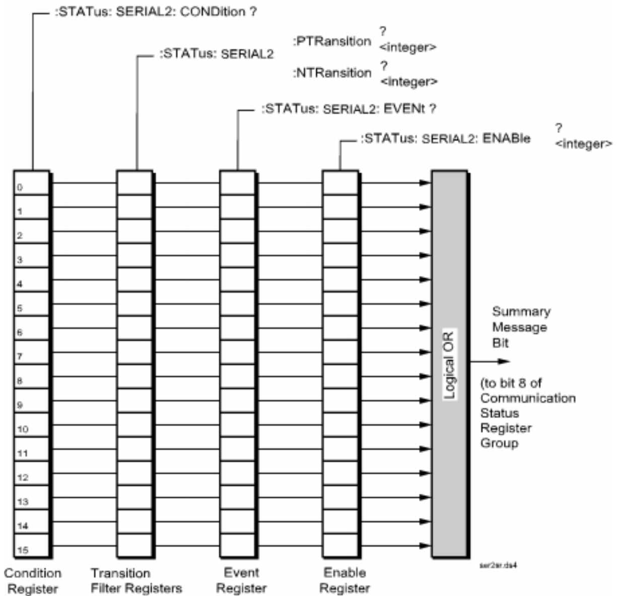
Figure 27 Serial 2 Status Register Group
