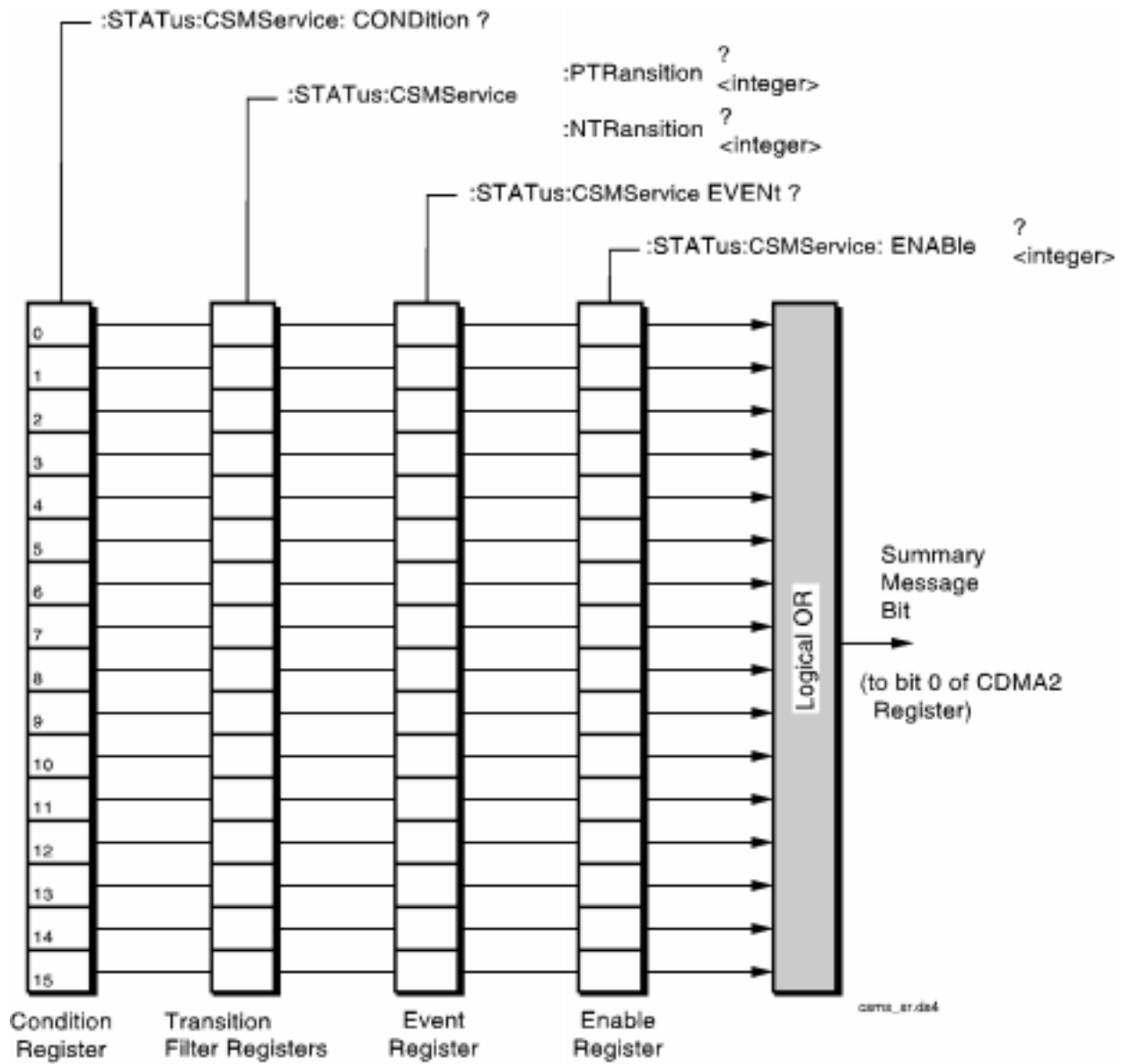
Figure 15 CDMA SMS Status Register Group
