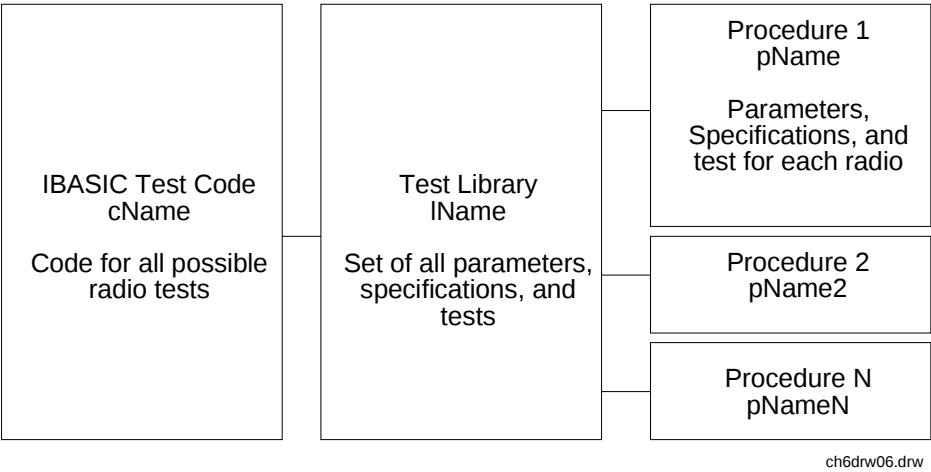
Figure 40 TESTS Subsystem File Relationship
