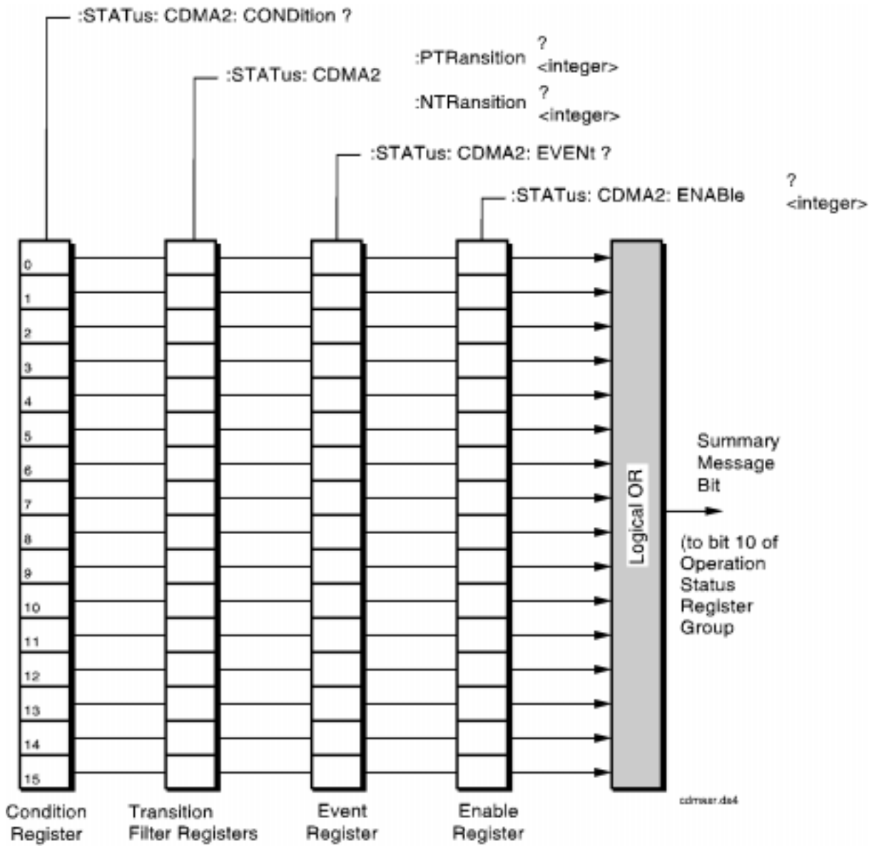
Figure 17 CDMA_2 Status Register Group
