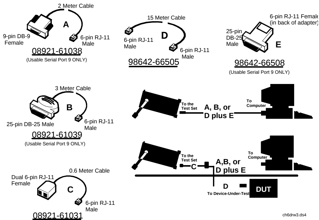
Figure 36 Available HP RS-232 Serial Cables and Adapters
