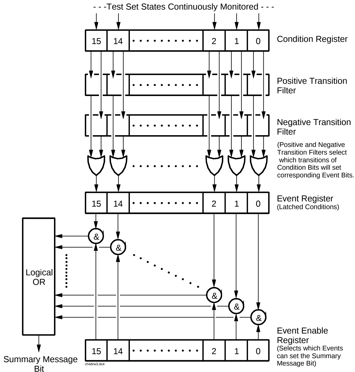
Figure 8 Status Data Structure - Register Group Model
