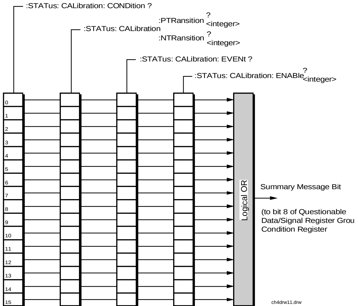
Figure 12 Calibration Status Register Group
