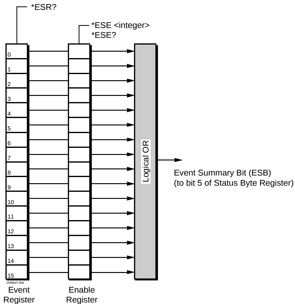
Figure 28 Standard Event Status Register Group
