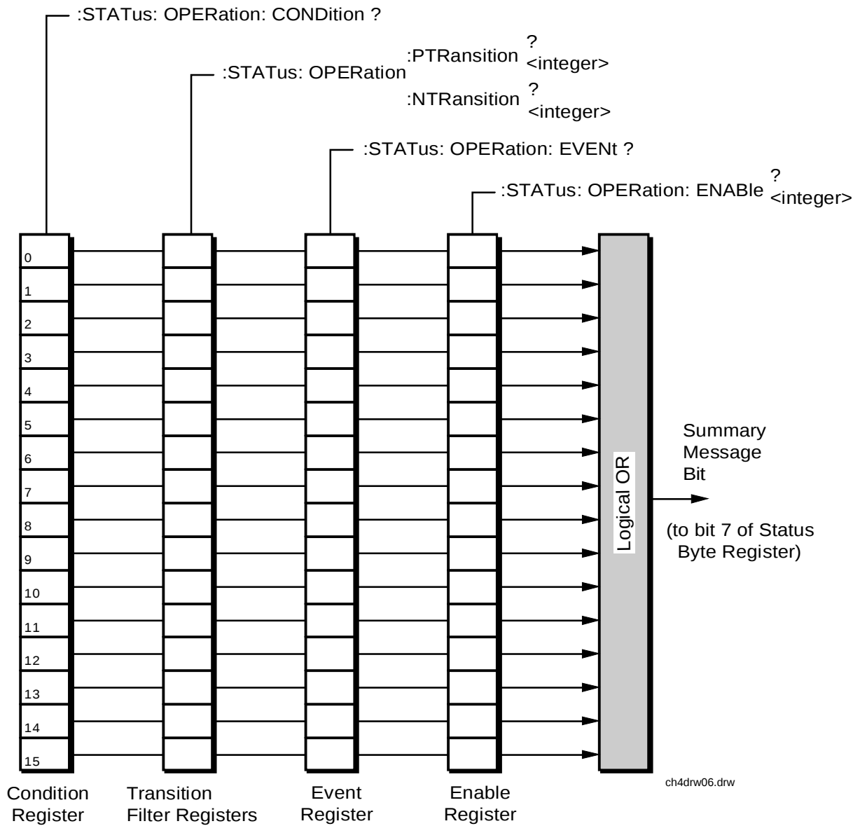
Figure 23 Operation Status Register Group
