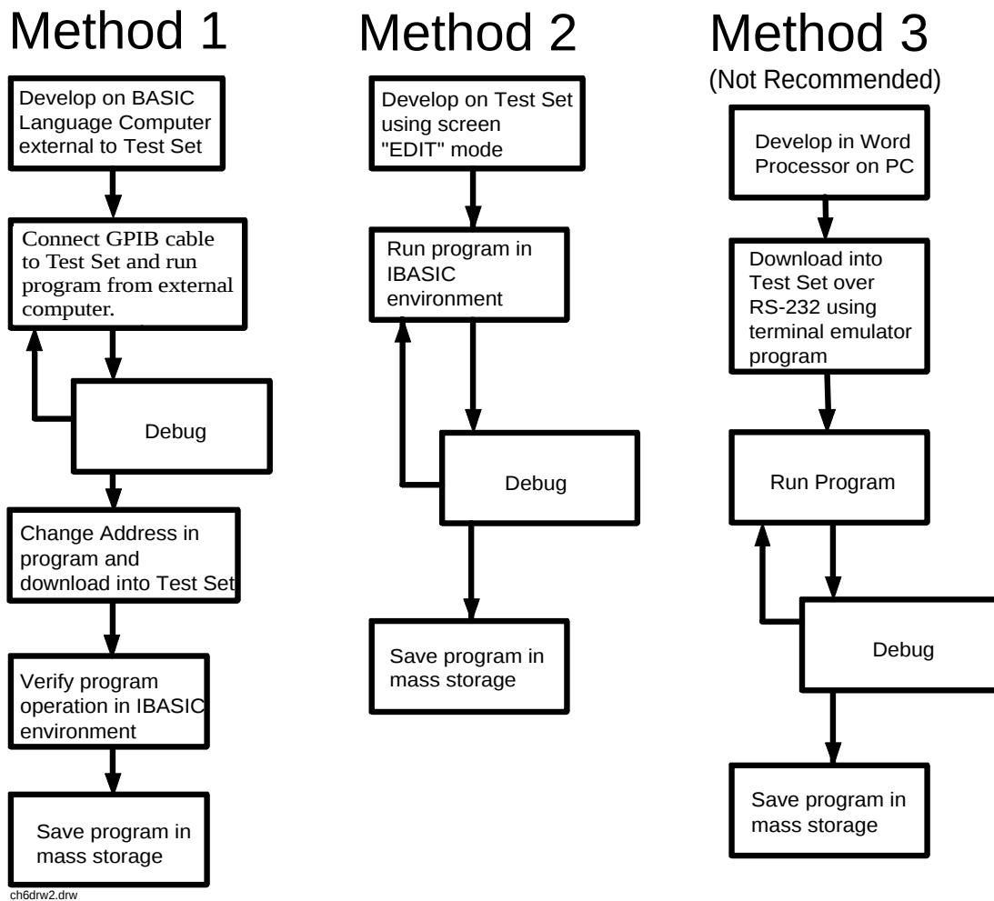
Figure 35 Program Development Methods
