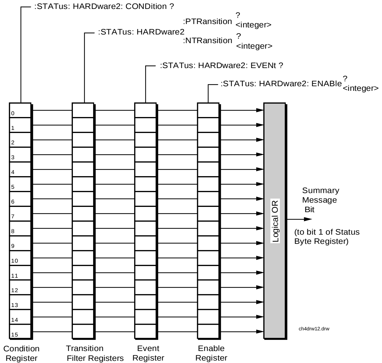
Figure 21 Hardware 2 Status Register Group
