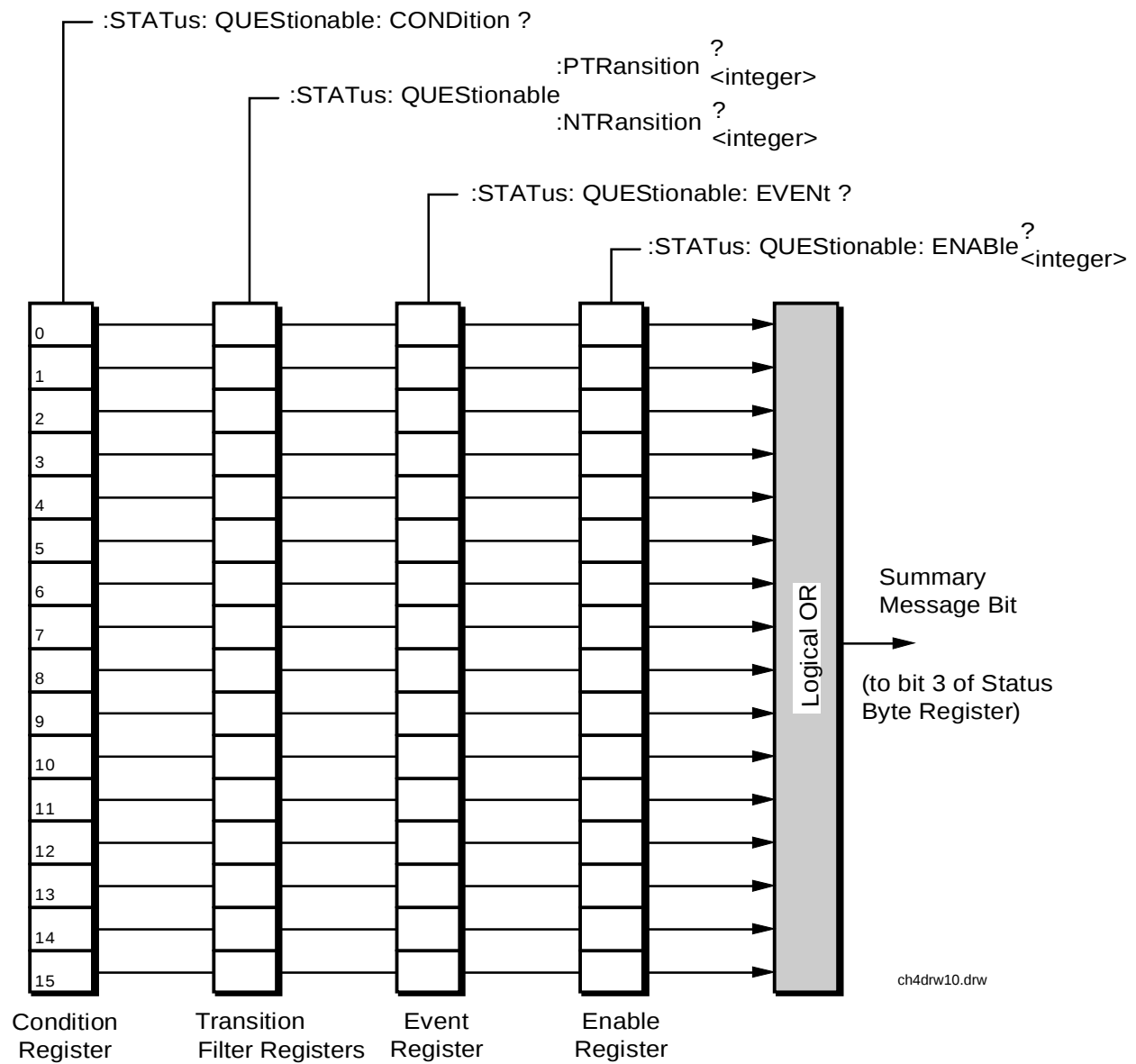
Figure 25 Questionable Data/Signal Register Group
