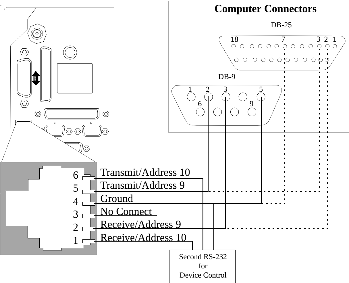
Figure 37 Connecting the Test Set Serial Port to a PC or Terminal
