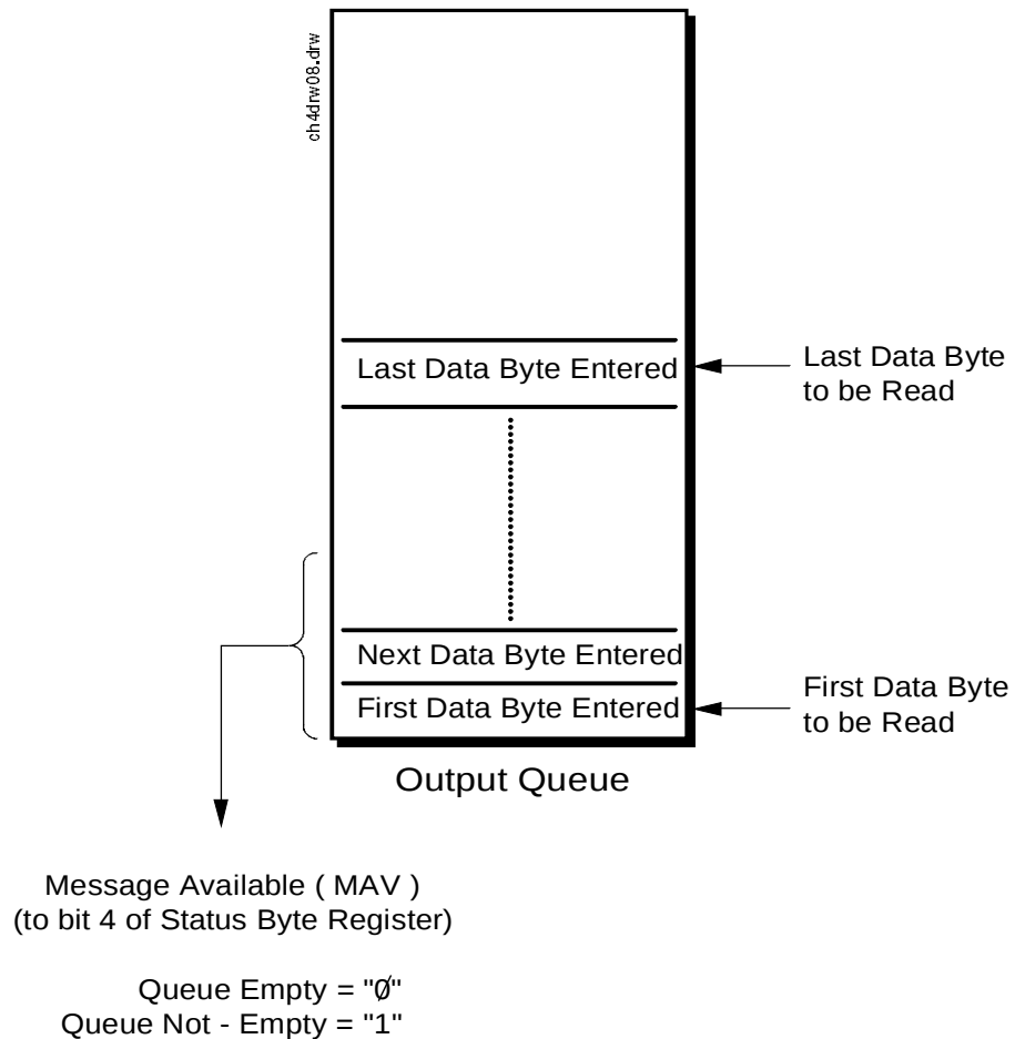
Figure 24 Output Queue Group
