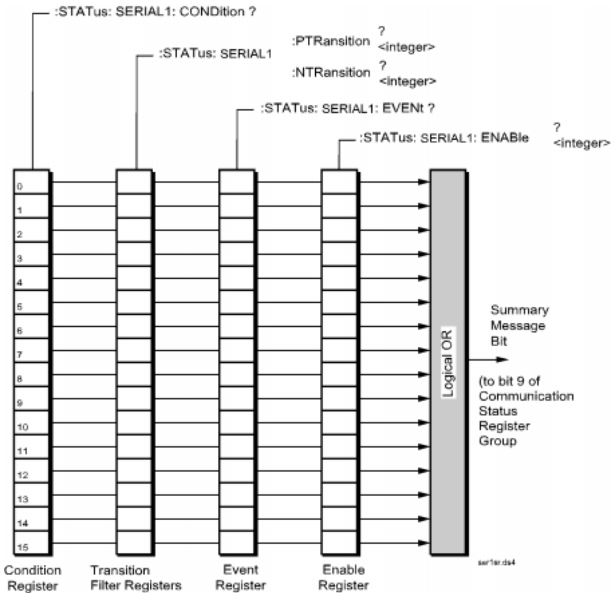
Figure 26 Serial 1 Status Register Group
