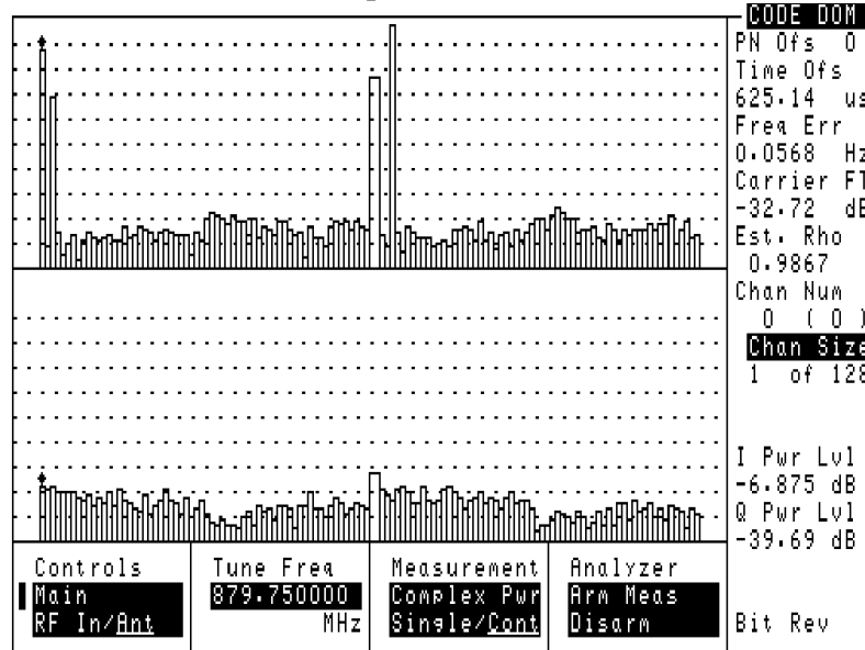
Figure 3-14 Code Domain Complex Power
