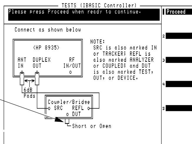
Figure 4-6 Swept Return Loss Measurement Connections
