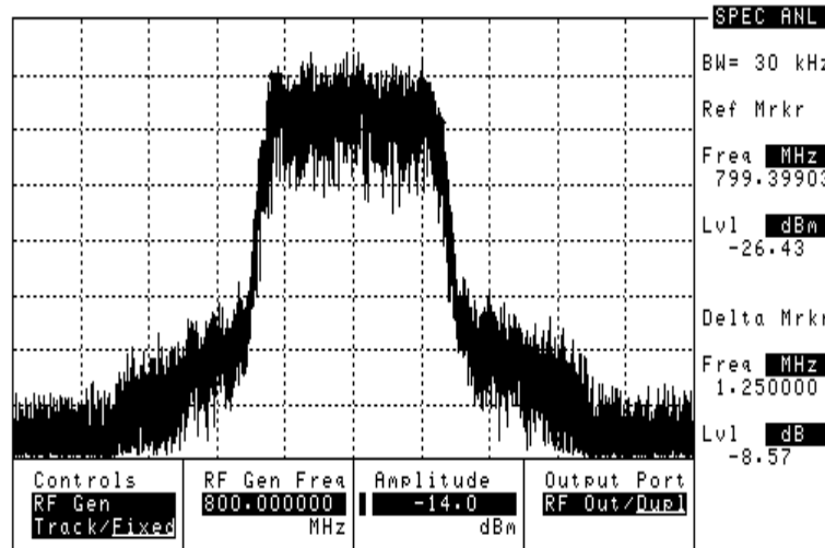
Figure 3-21 Standard CDMA Signal
