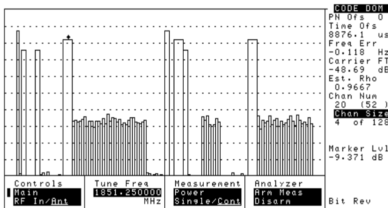
Figure 3-8 The Code Domain Analyzer Display (IS-2000)
