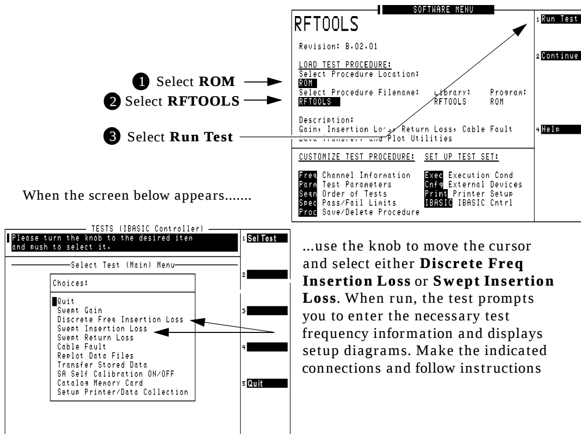
Figure 4-1 Loading and Running the Insertion Loss Test
