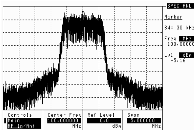
Figure 3-22 CDMA Signal with “Shoulders” Distortion
