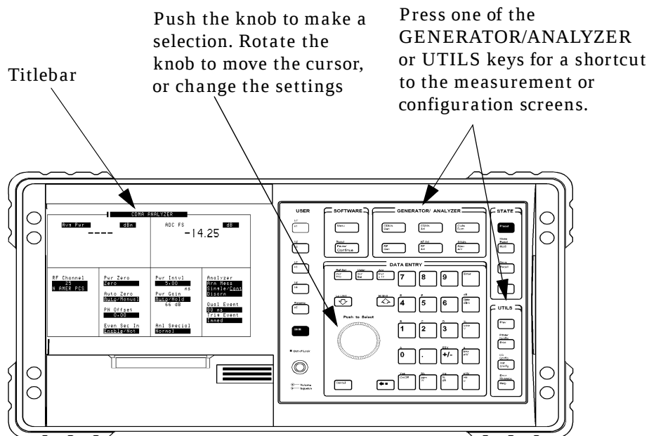
Figure 2-2 Using the cursor-control Knob or Screen Keys
