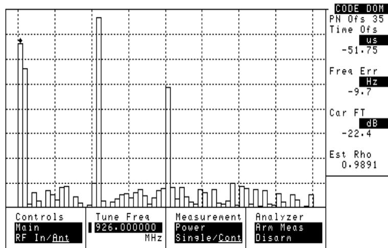
Figure 3-7 The Code Domain Analyzer Display (IS-95).
