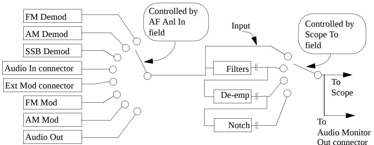
Figure 4-2 Inputs and Filters for the Oscilloscope
