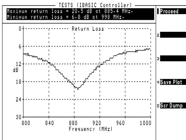
Figure 4-7 Swept Return Loss Measurement Results
