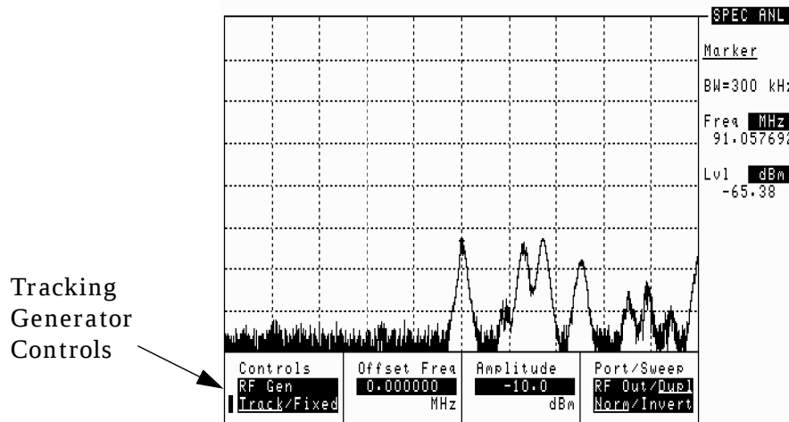
Figure 4-9 Spectrum Analyzer with Tracking Generator Controls Displayed
