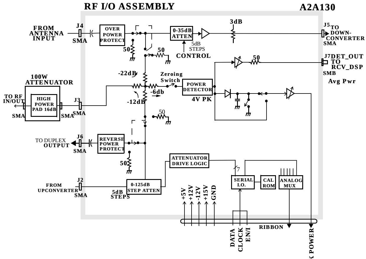
Figure 3-2 Block Diagram for RF, DUPLEX, and ANT Ports
