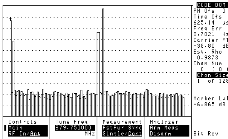
Figure 3-15 Fast Power Synchronize
