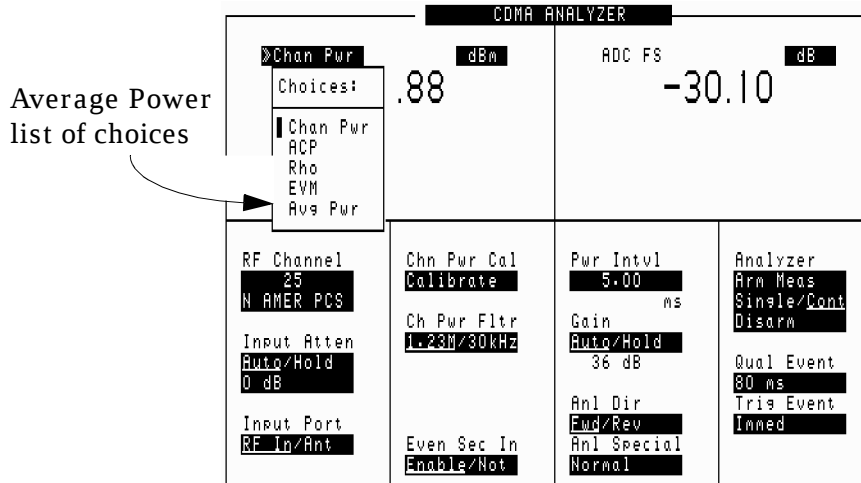
Figure 3-3 Average Power Measurement List of Choices
