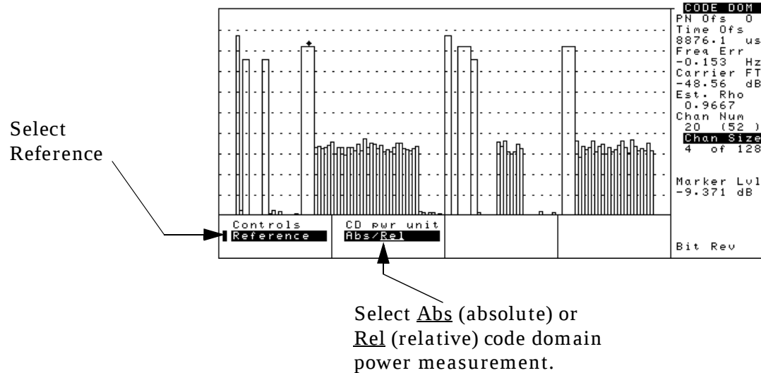
Figure 3-12 Selecting Absolute or Relative Code Domain Power – IS-2000
