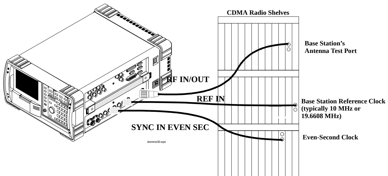
Figure 3-1 Connections for Testing a CDMA Base Station
