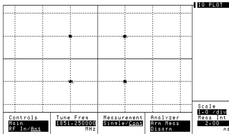
Figure 3-17 IQ PLOT screen
