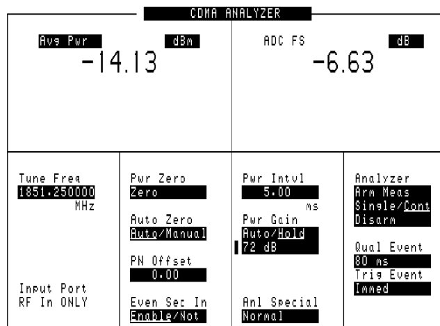
Figure 3-4 Average Power Measurement Results
