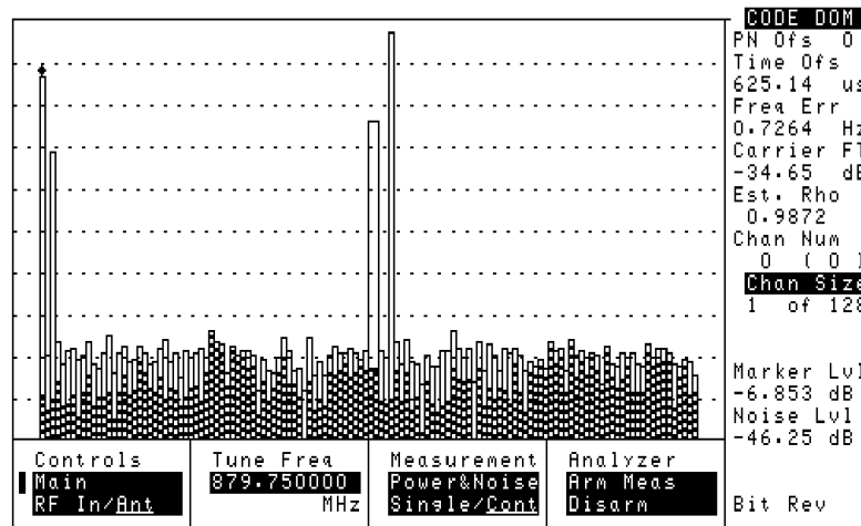
Figure 3-13 Code Domain Power & Noise
