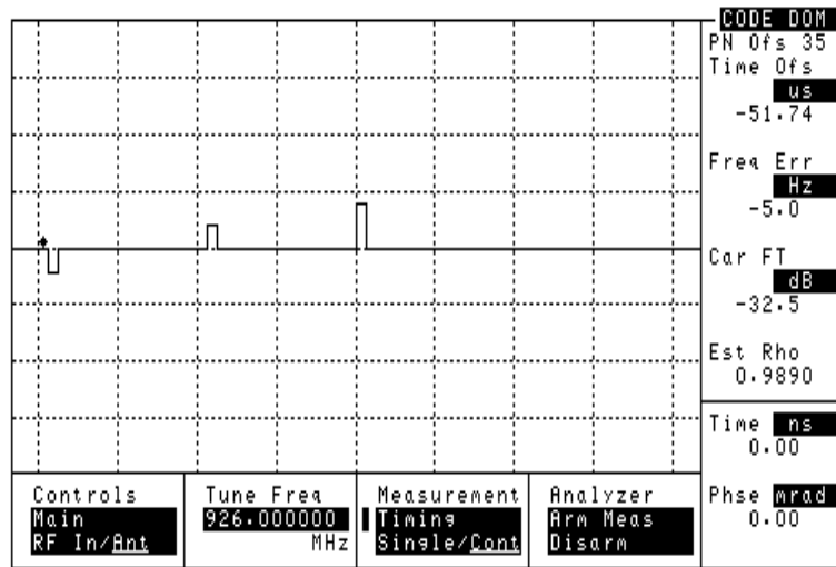
Figure 3-10 Code Domain Timing
