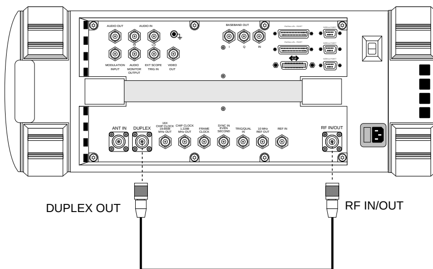
Figure 2-1 CDMA Loopback Test Connections
