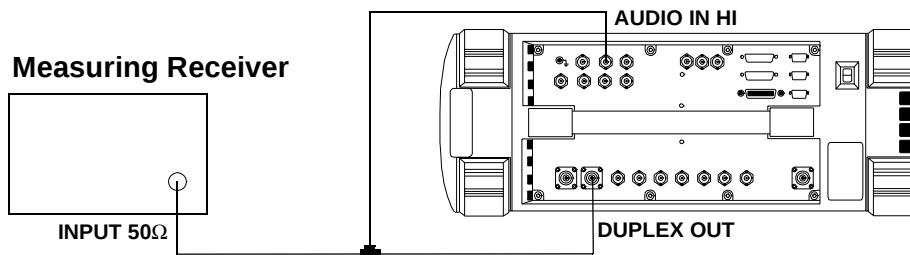
Figure 8-22 Setup
