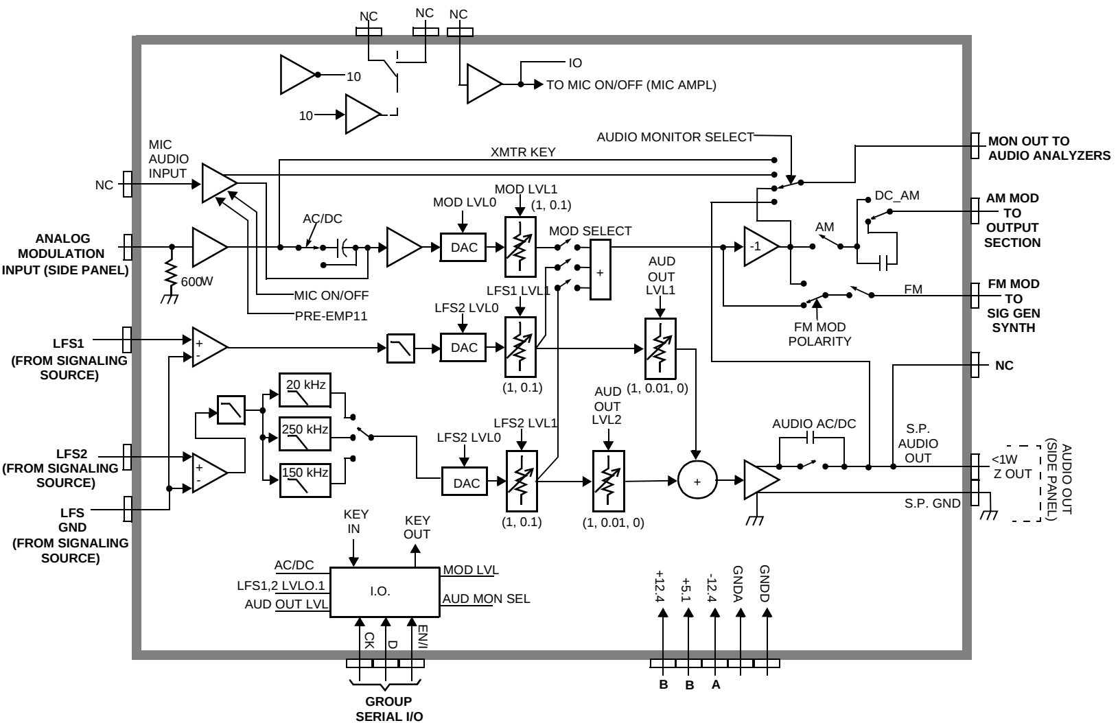
Modulation Distribution Assembly, A2A44
