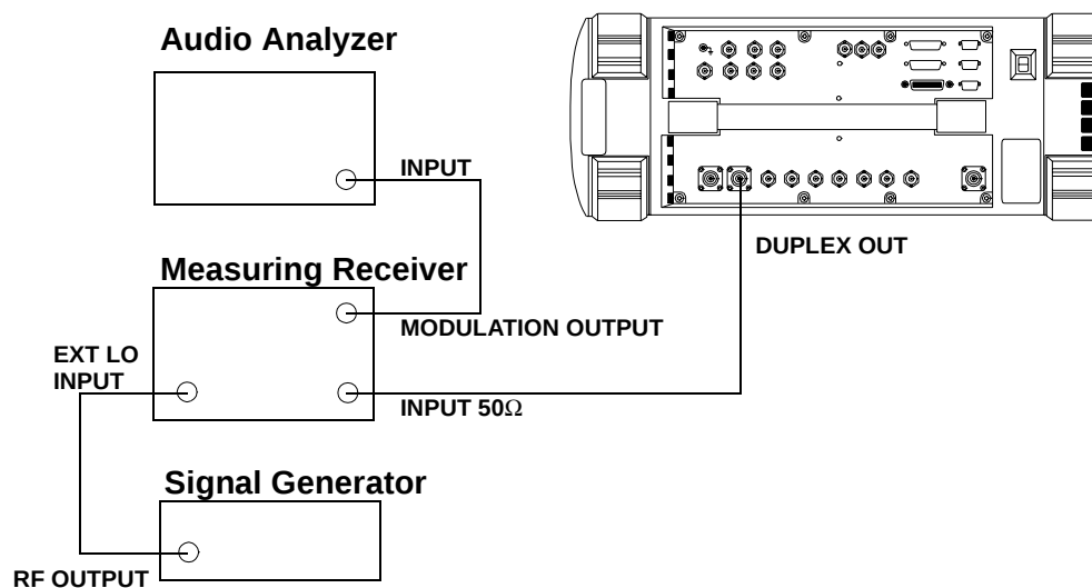
Figure 8-7 Setup for Measurements to 1 GHz
