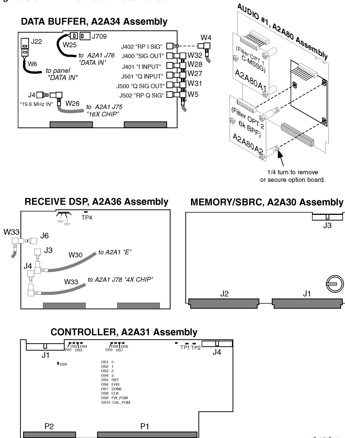
Figure 5-9 PC Board Assemblies
