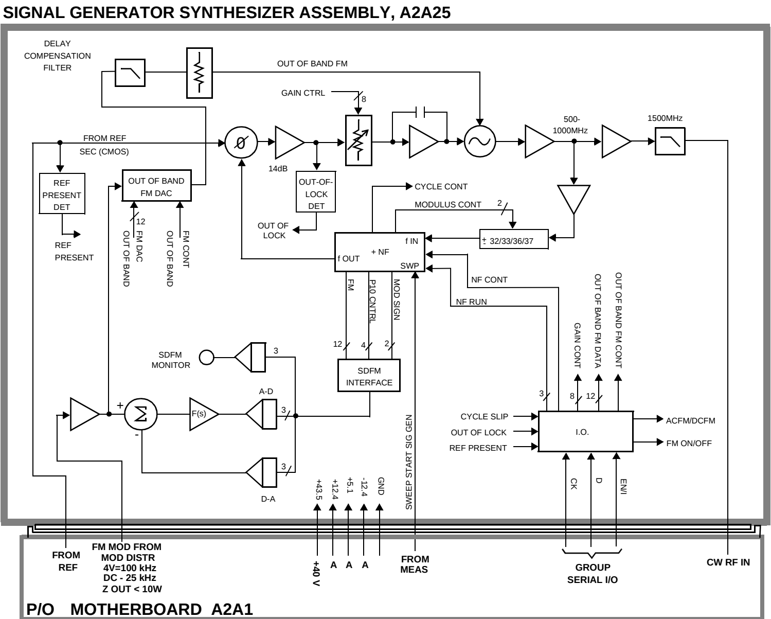
Signal Generator Synthesizer Assembly, A2A25
