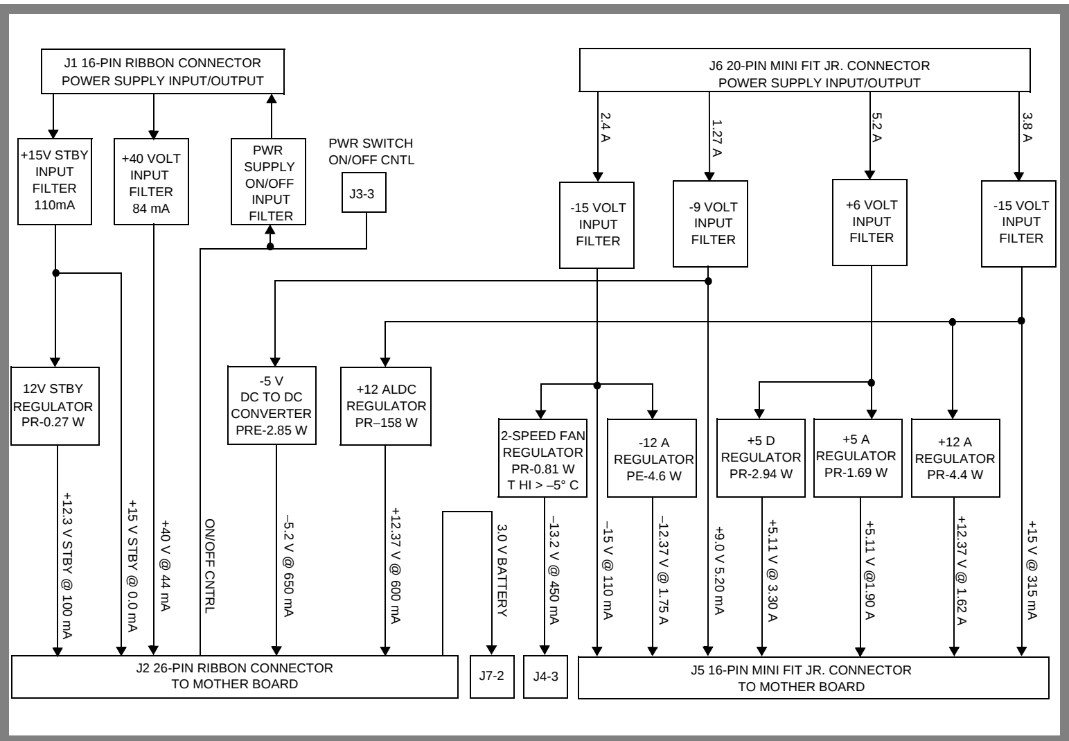
Power Supply Regulator Assembly, A3A1
