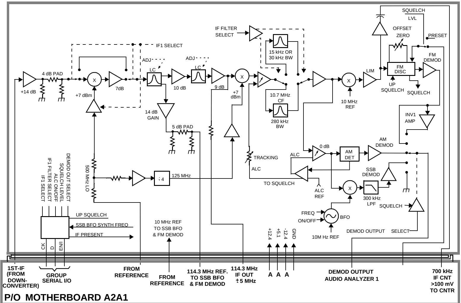
Receiver Assembly, A2A21
