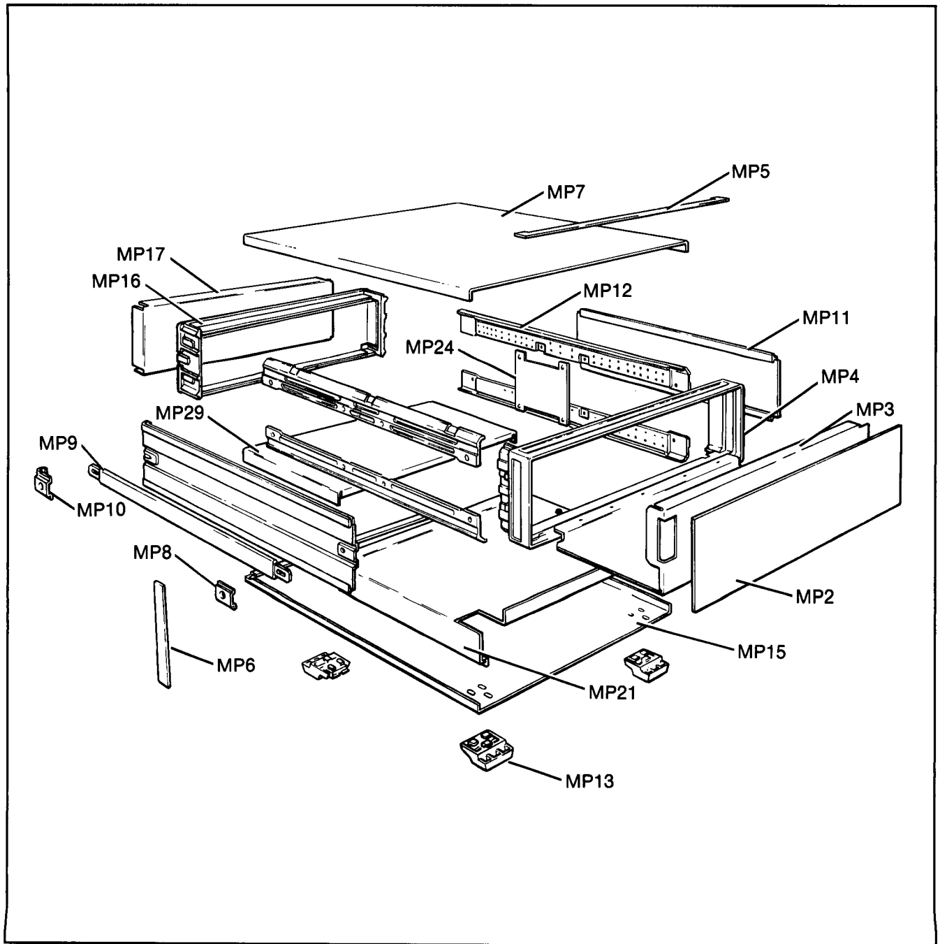
Figure 6. Cabinet Parts
