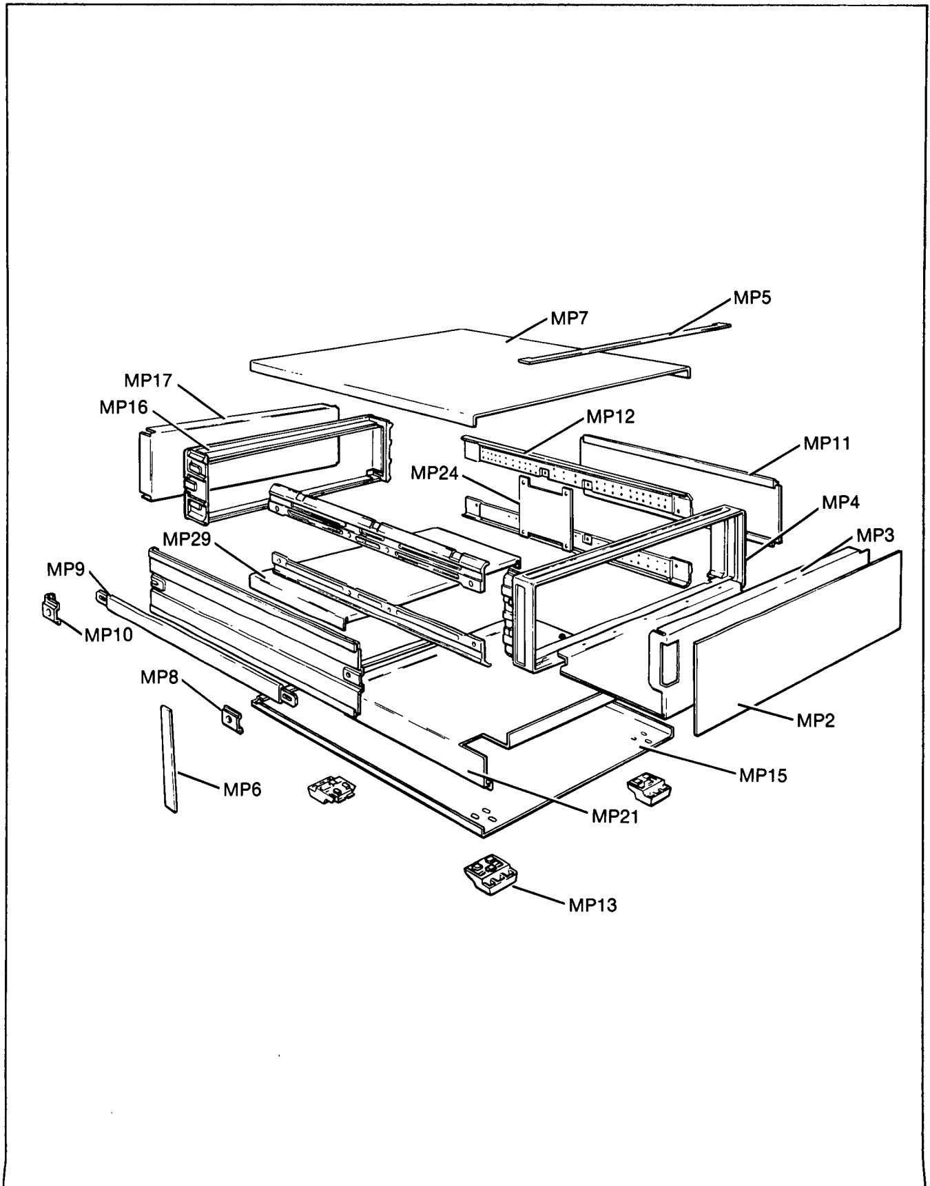
Figure 6. Cabinet Parts
