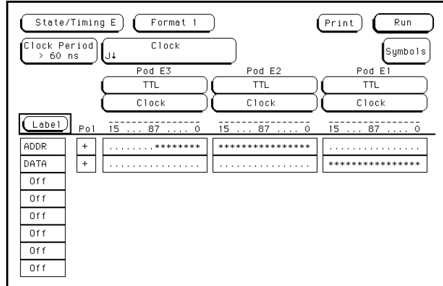
Figure 12-2. State Format Specification Menu
