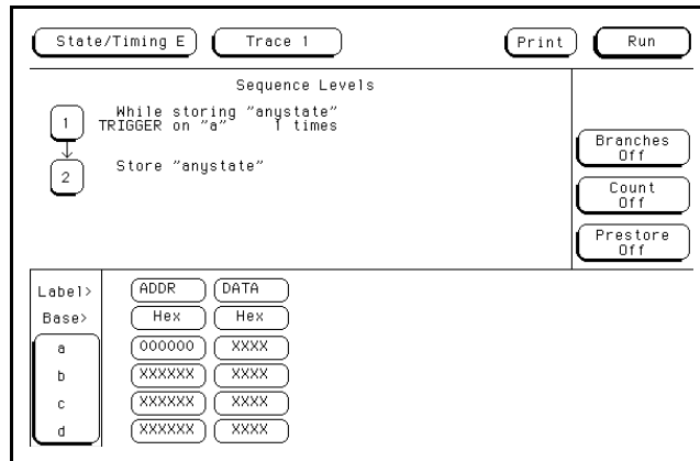
Figure 8-18. State Trace Specification
