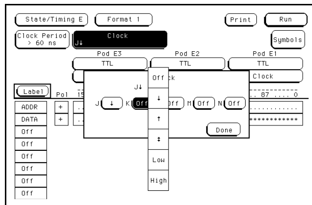
Figure 3 - 2. State Clock Pop-up with K Pop-up
