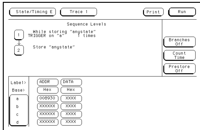
Figure 12-3. State Trace Specification Menu
