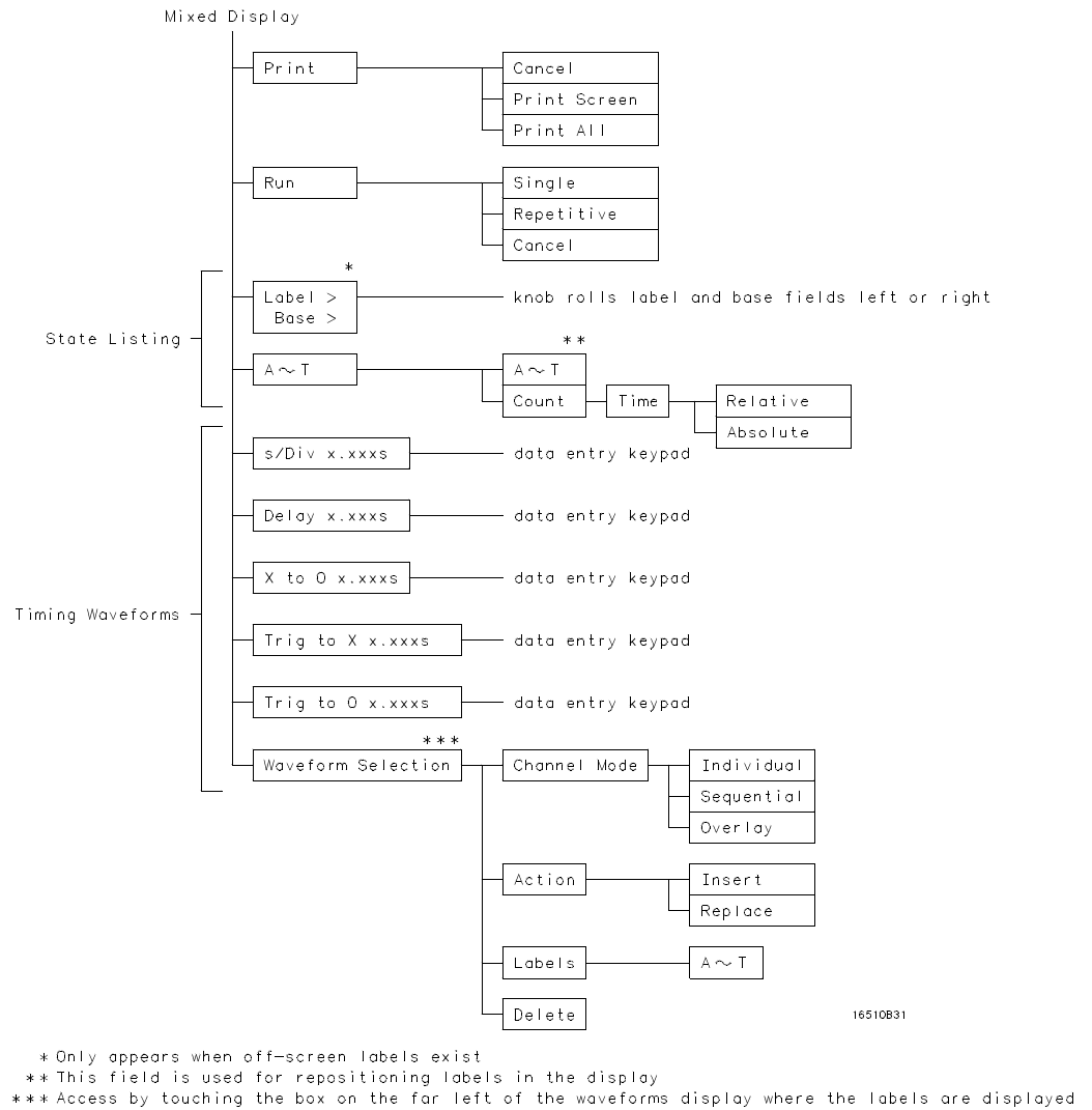
Figure 4-11. Mixed Display Menu Map
