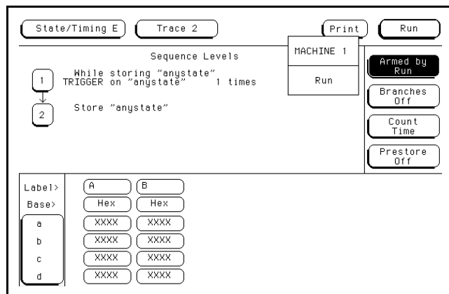
Figure 5-65. Armed By Pop-up Menu
