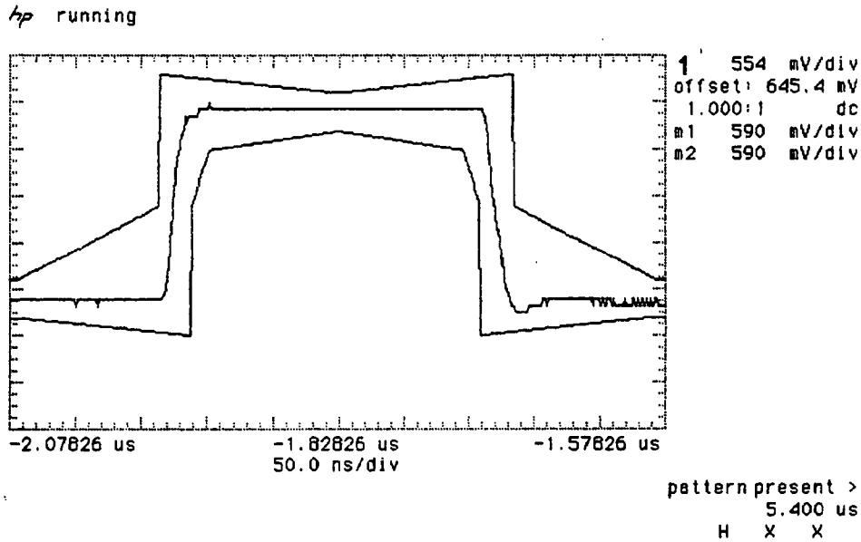
Figure 3-31. 2 Mb/s Isolated Positive Pulse
