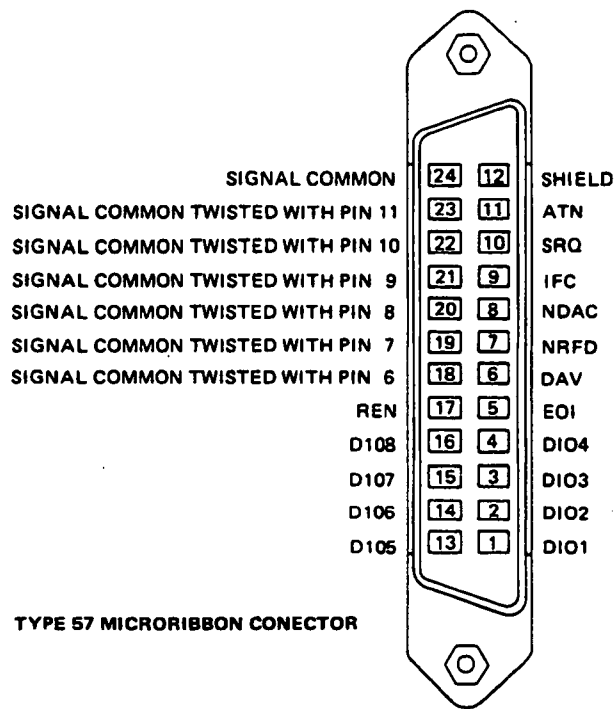
Figure 2-2. HP-IB Connections and Logic Levels
