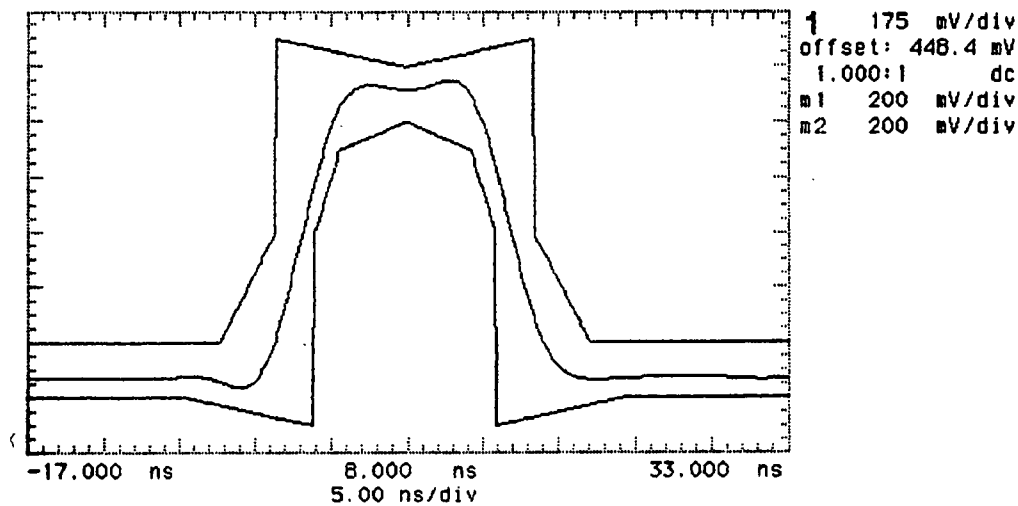
Figure 3-10. 34 Mb/s Isolated Positive Pulse
