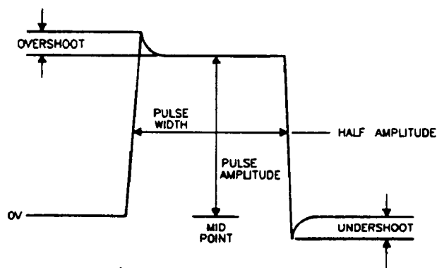
Figure 3-2. 704 kb/s Pulse Criteria
