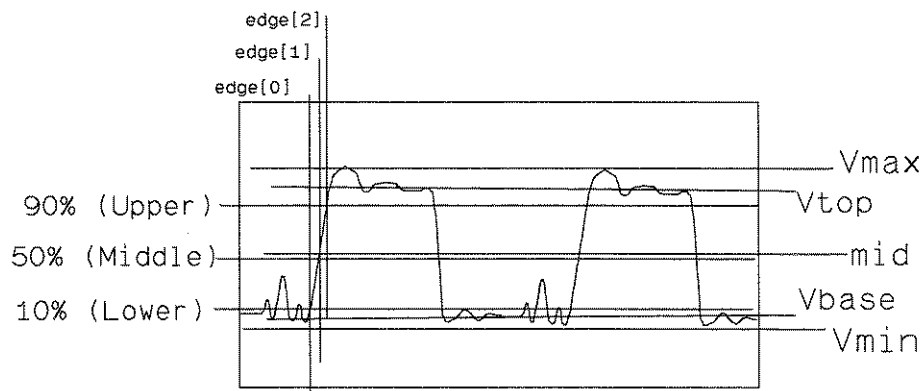
Waveform definitions used to make voltage measurements
