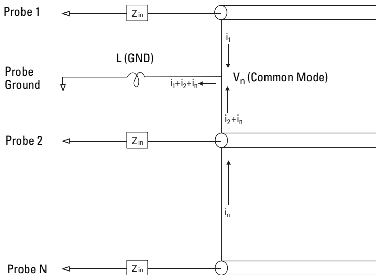
Common Mode Input Voltage Model
