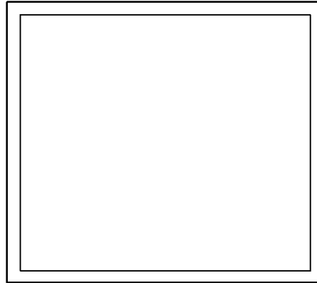
Figure 1-24. Draw Box
