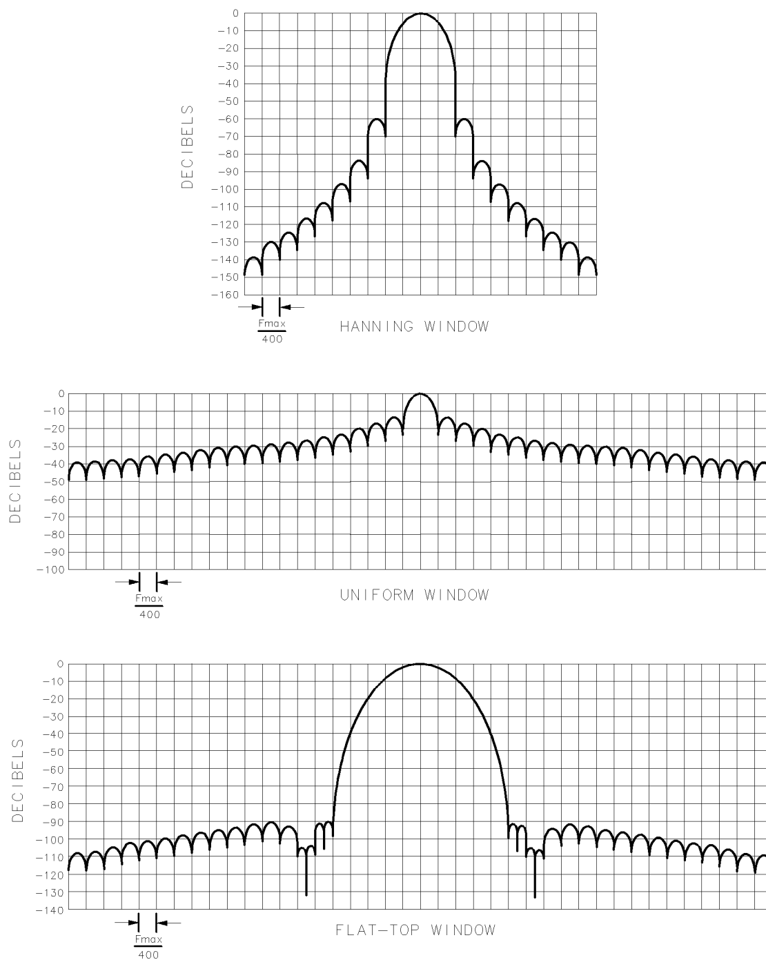
Figure 2-4. Fourier Transforms of Hanning, Flat Top, and Uniform Trace Windows
