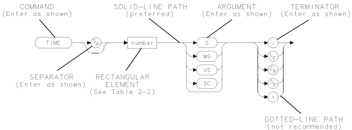
Figure 2-1. Syntax-Diagram Elements
