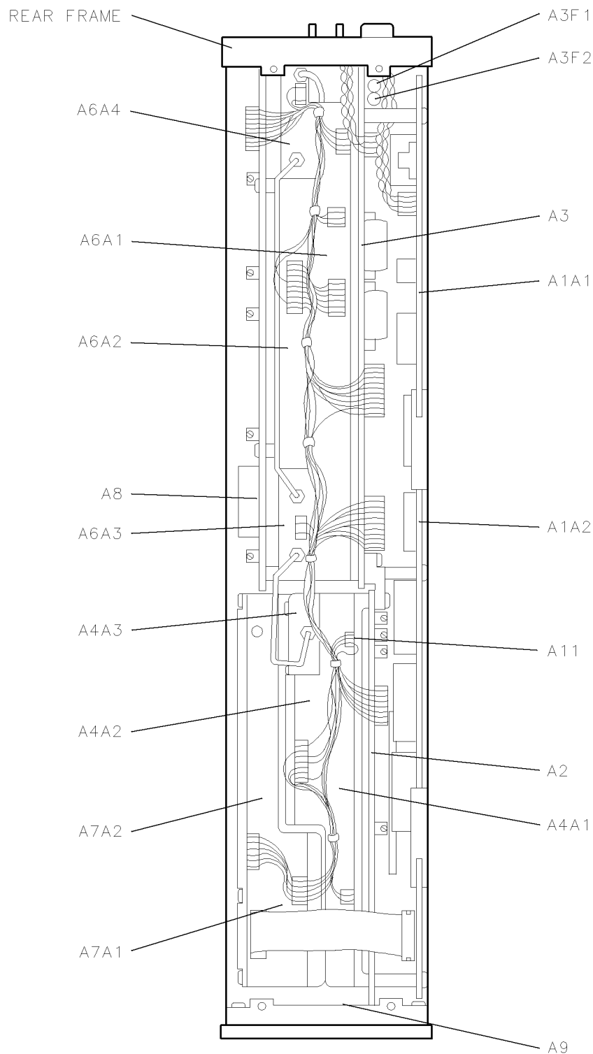
Figure 10-7. Overall Parts Identification Drawing, Top View (Assembly Locations)
