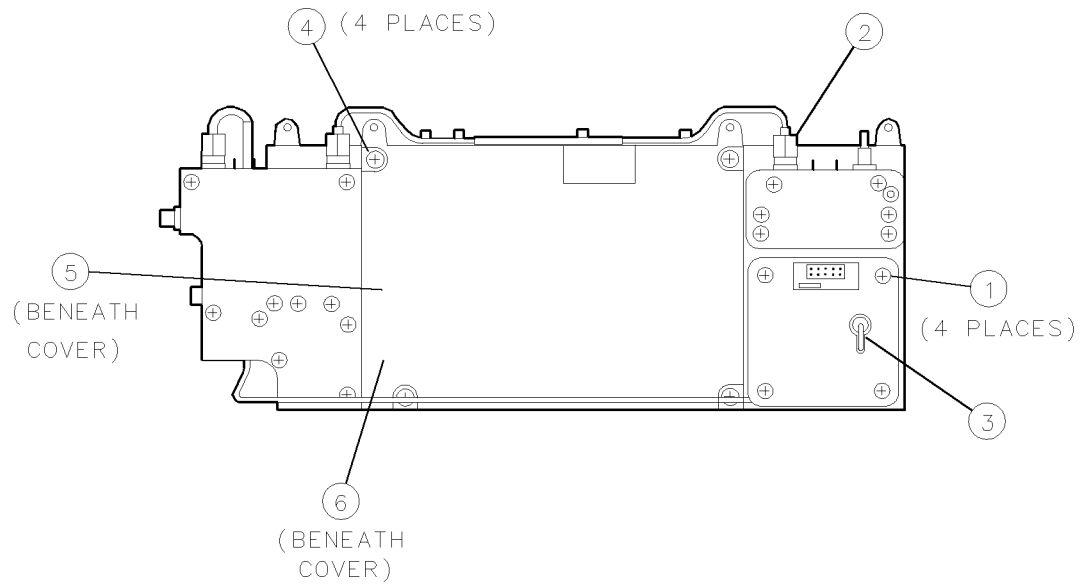
Figure 9-9. A6A2 YTO Lock Removal/Replacement
