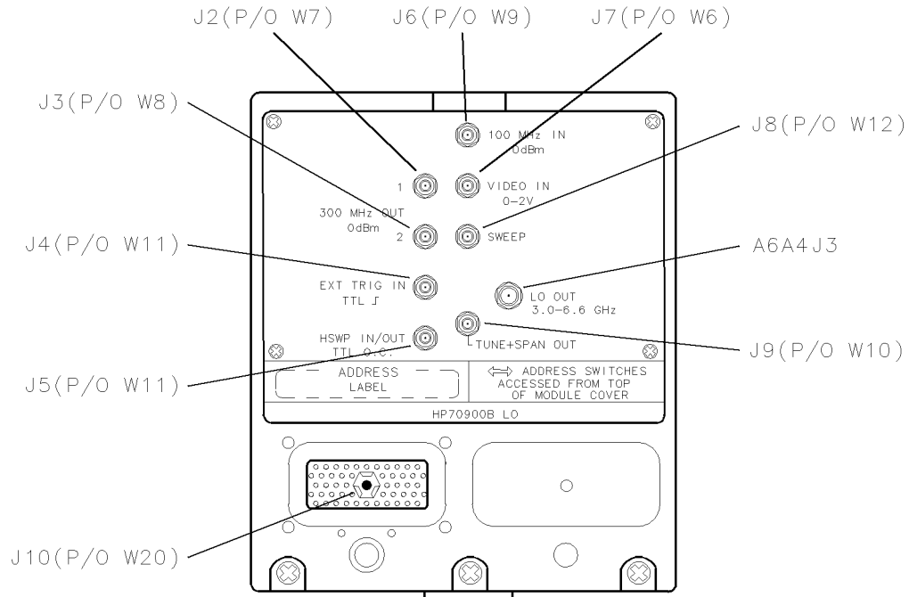
Figure 10-5. Overall Parts Identification Drawing, Rear Panel Connectors
