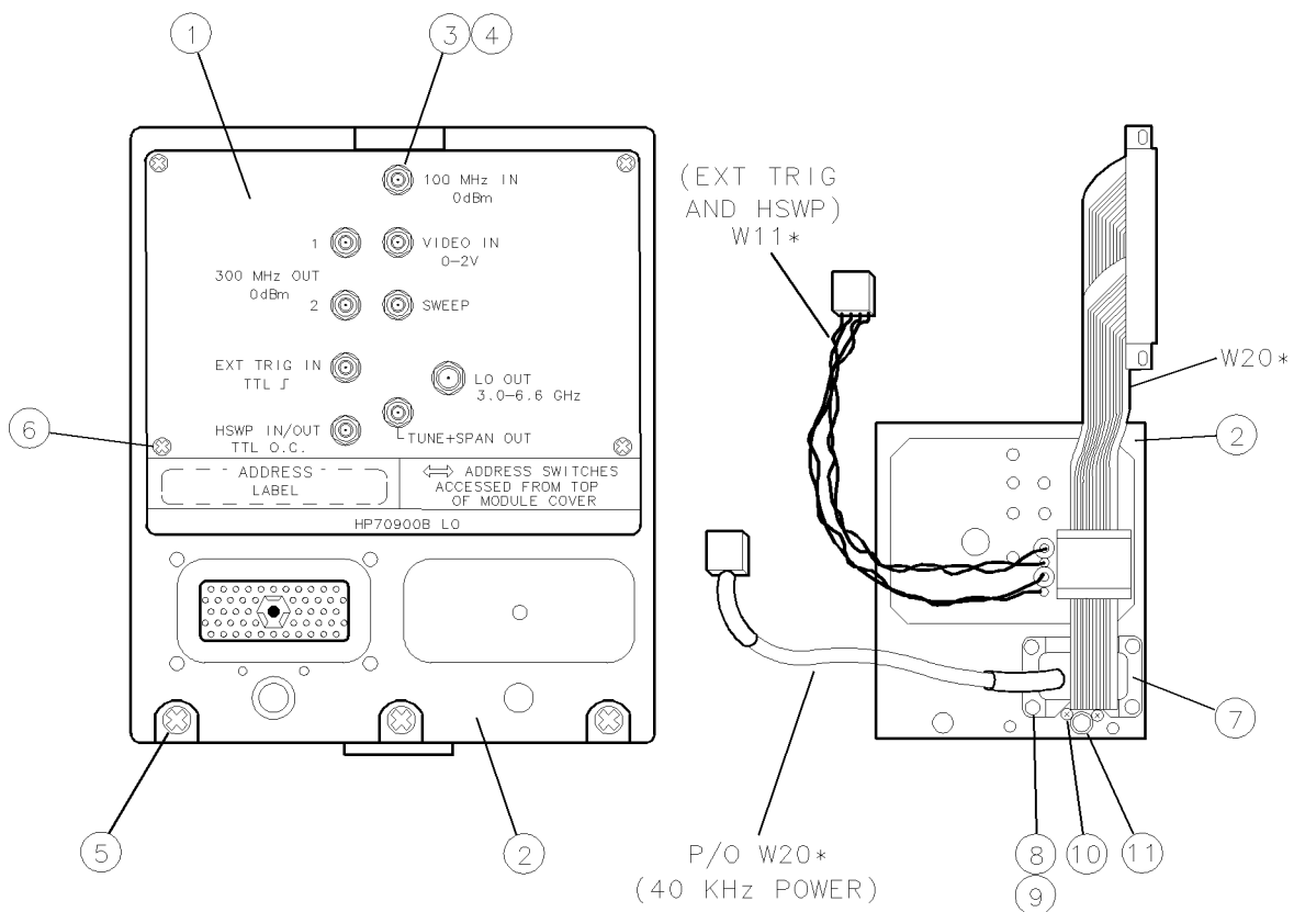
Figure 10-4. Overall Parts Identification Drawing, Rear View (Rear-Frame)
