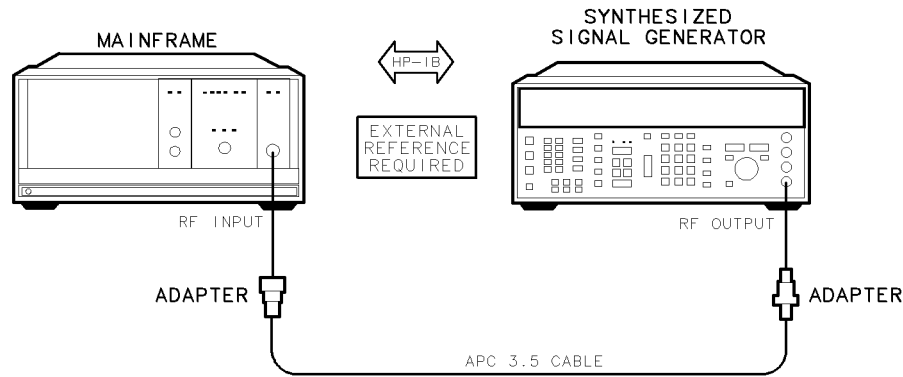
Figure 7-17. LO Frequency Error versus Sweep Time Test Setup
