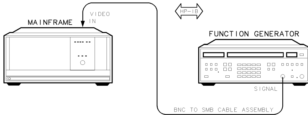
Figure 7-11. Video Detector Tracking Test Setup
