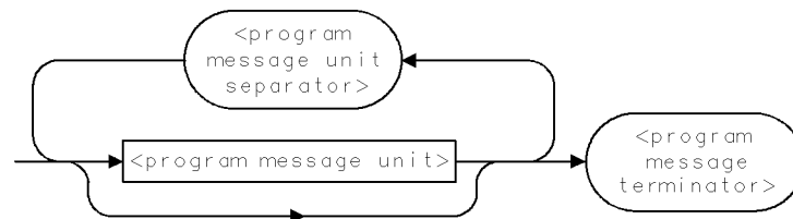
Figure 2-1. Terminated <program message> Functional Element Syntax
