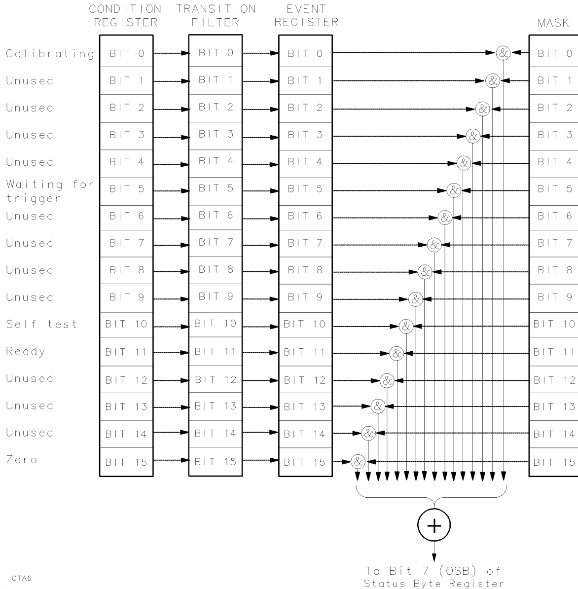
Figure 1-2. Status Data Structure (2 of 2)
