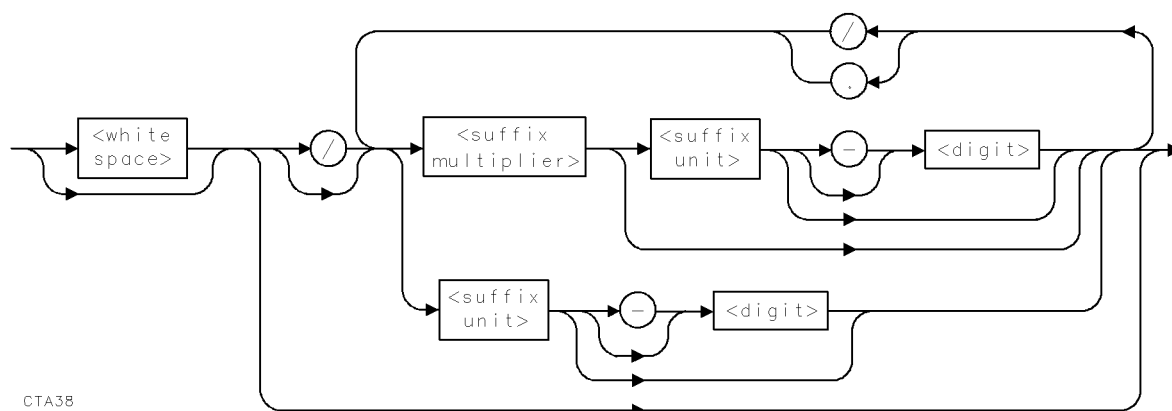
Figure 2-11. &lt;suffix program data&gt;
