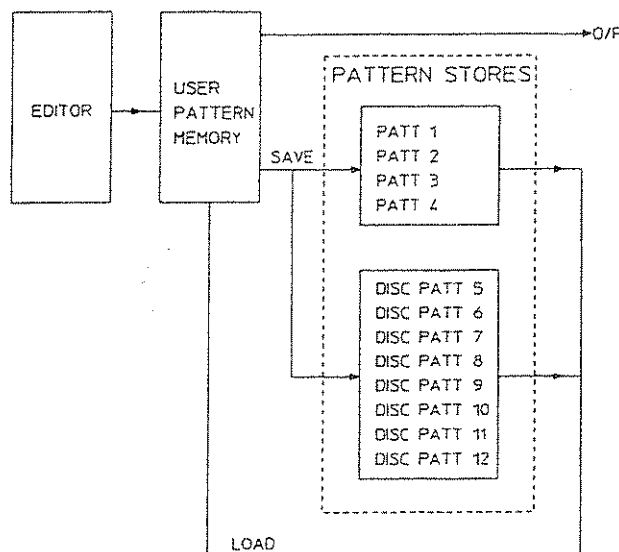
Figure 6-1. The Editor
