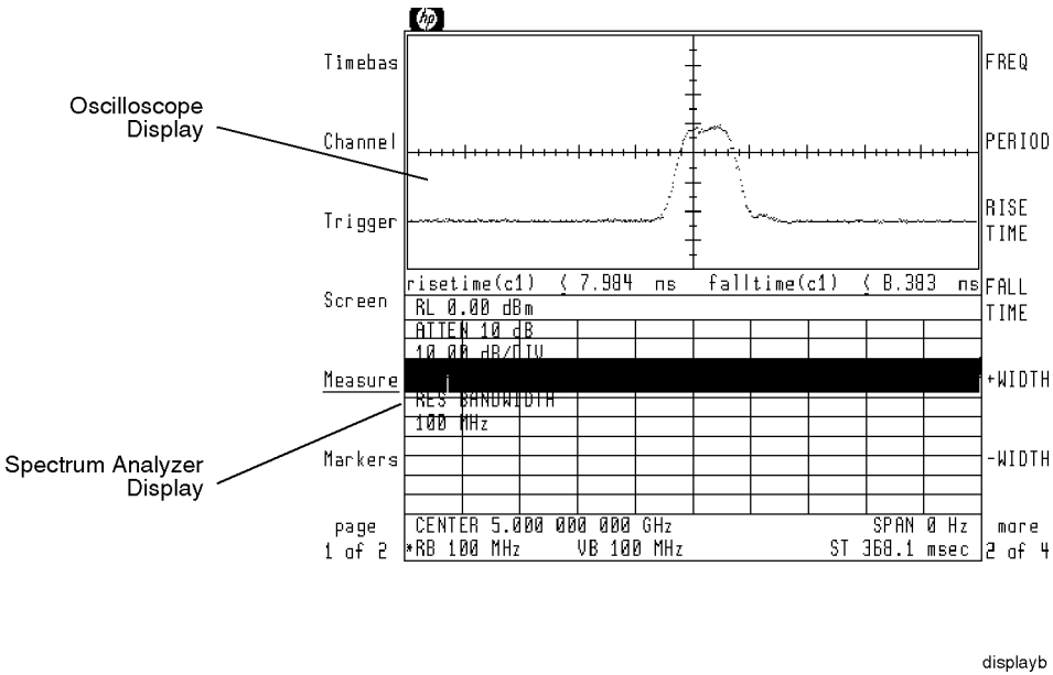
HP 70703A Oscilloscope Display of VIDEO Output
