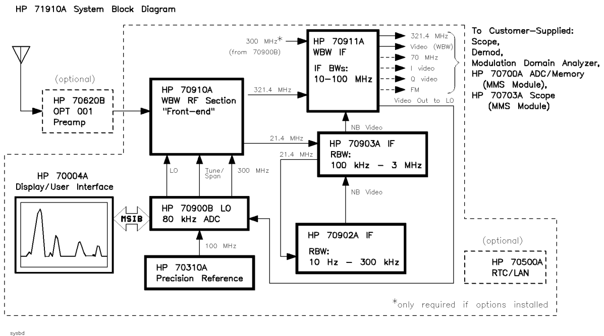
HP 71910A System Block Diagram
