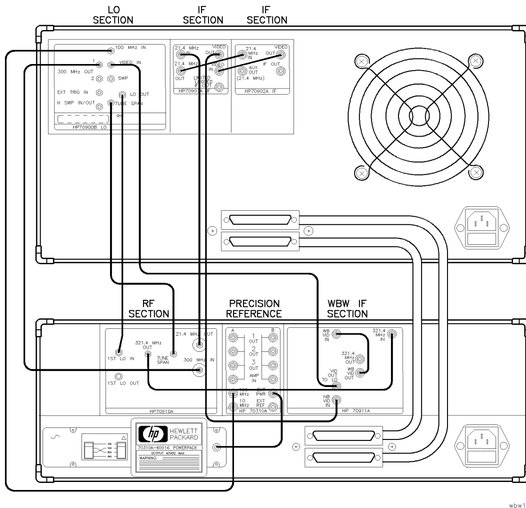
Rear-Panel Connections for the Standard HP 71910A
