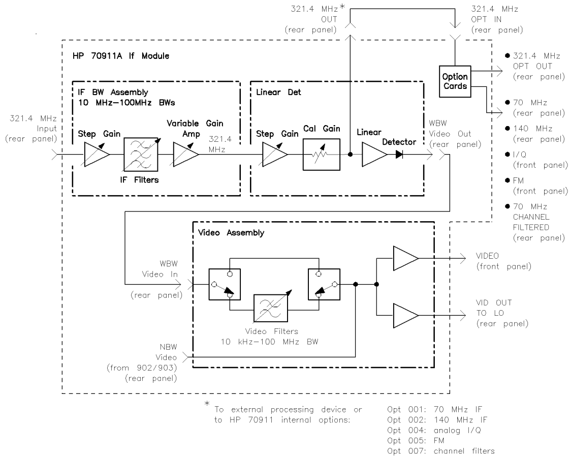
HP 70911A IF Module Block Diagram
