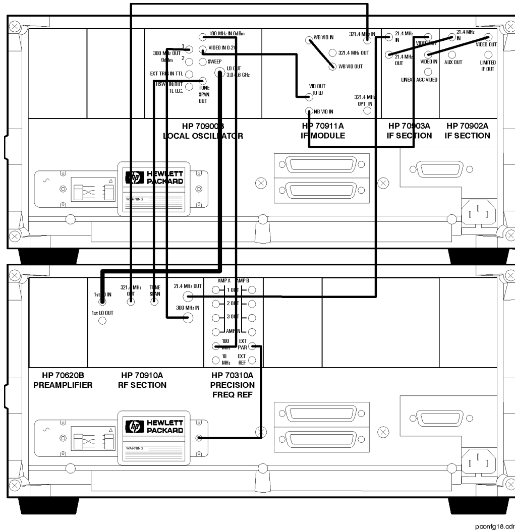
Rear-Panel Connections for the Standard HP 71910P with Two Mainframes and an HP 70620B Preamplifier Added
