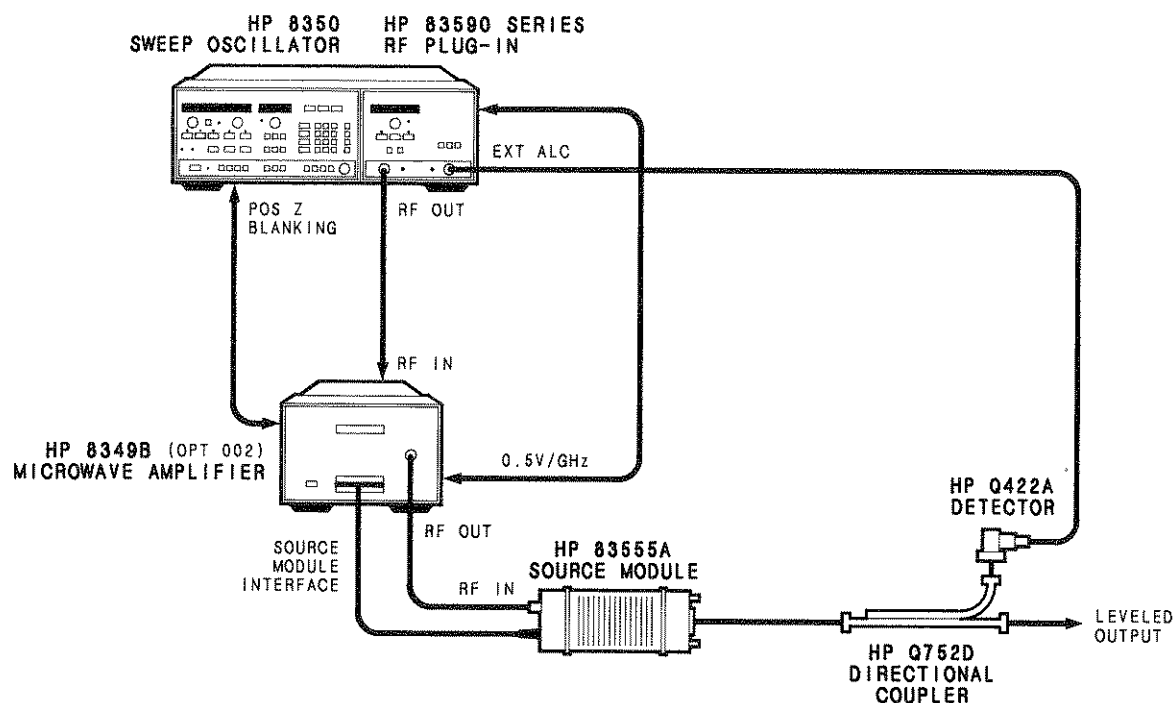
Figure 2-3. External Crystal Detector Leveling at the HP 83555A Output
