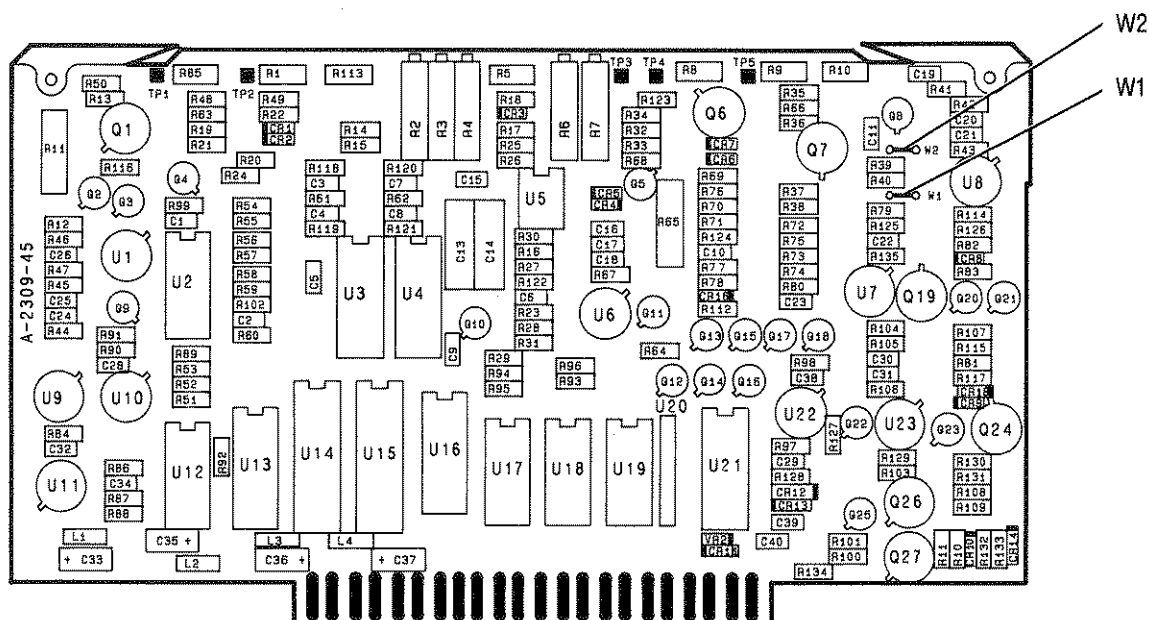
Figure 2. A28 SYTM Driver Assembly Component Locations
