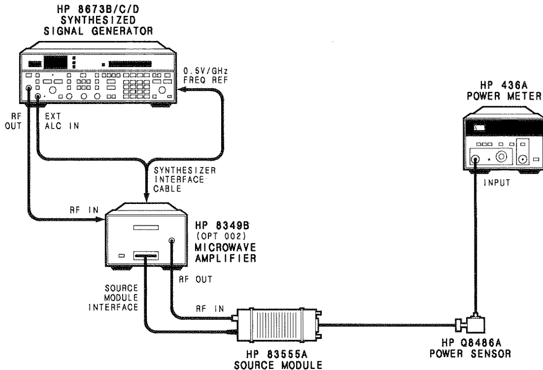
Figure 2-4. System Configuration
