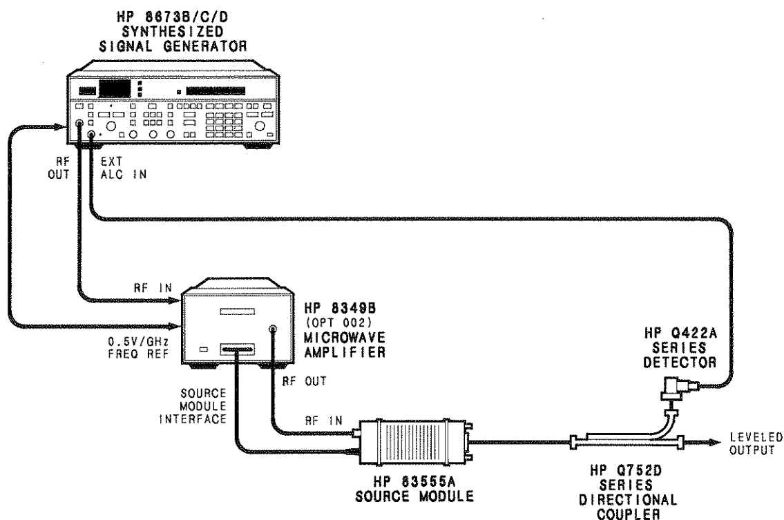
Figure 2-2. External Crystal Detector at the HP 83555A Source Module Output.
