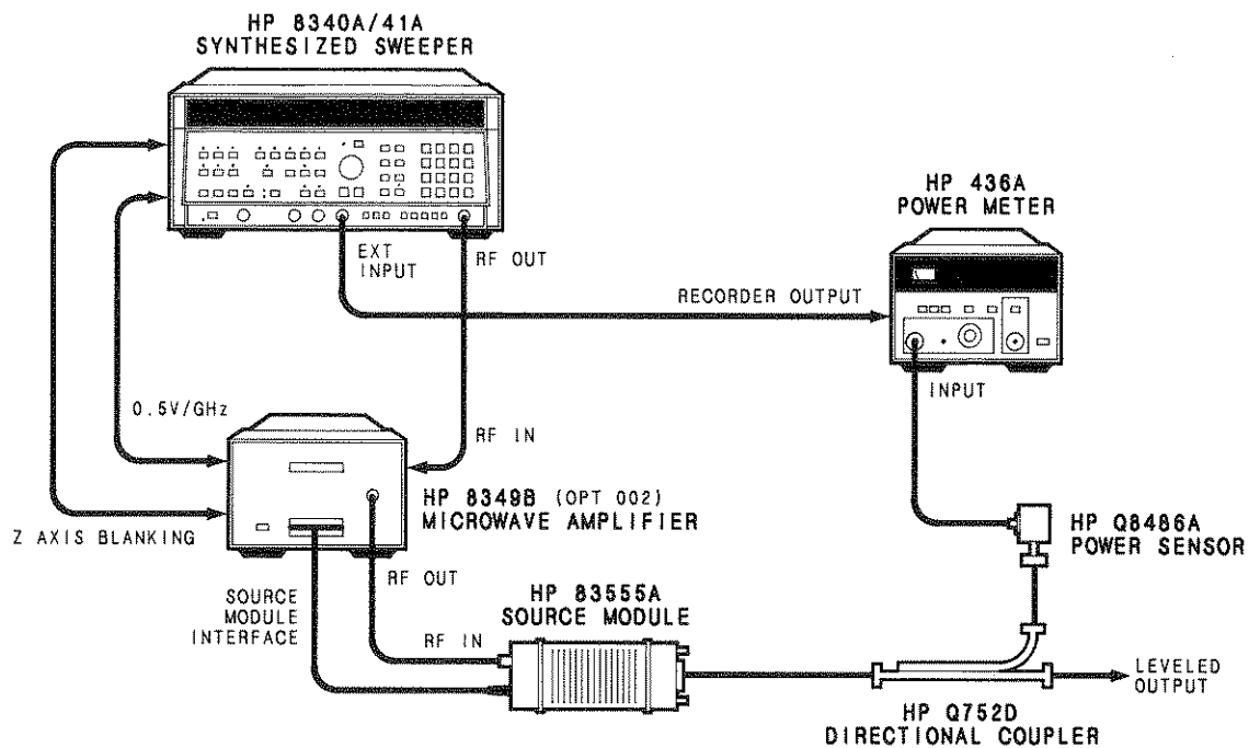
Figure 2-3. External Power Meter Leveling at the HP 83555A Source Module Output
