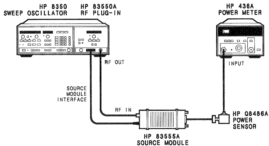
Figure 2-5. System Configuration
