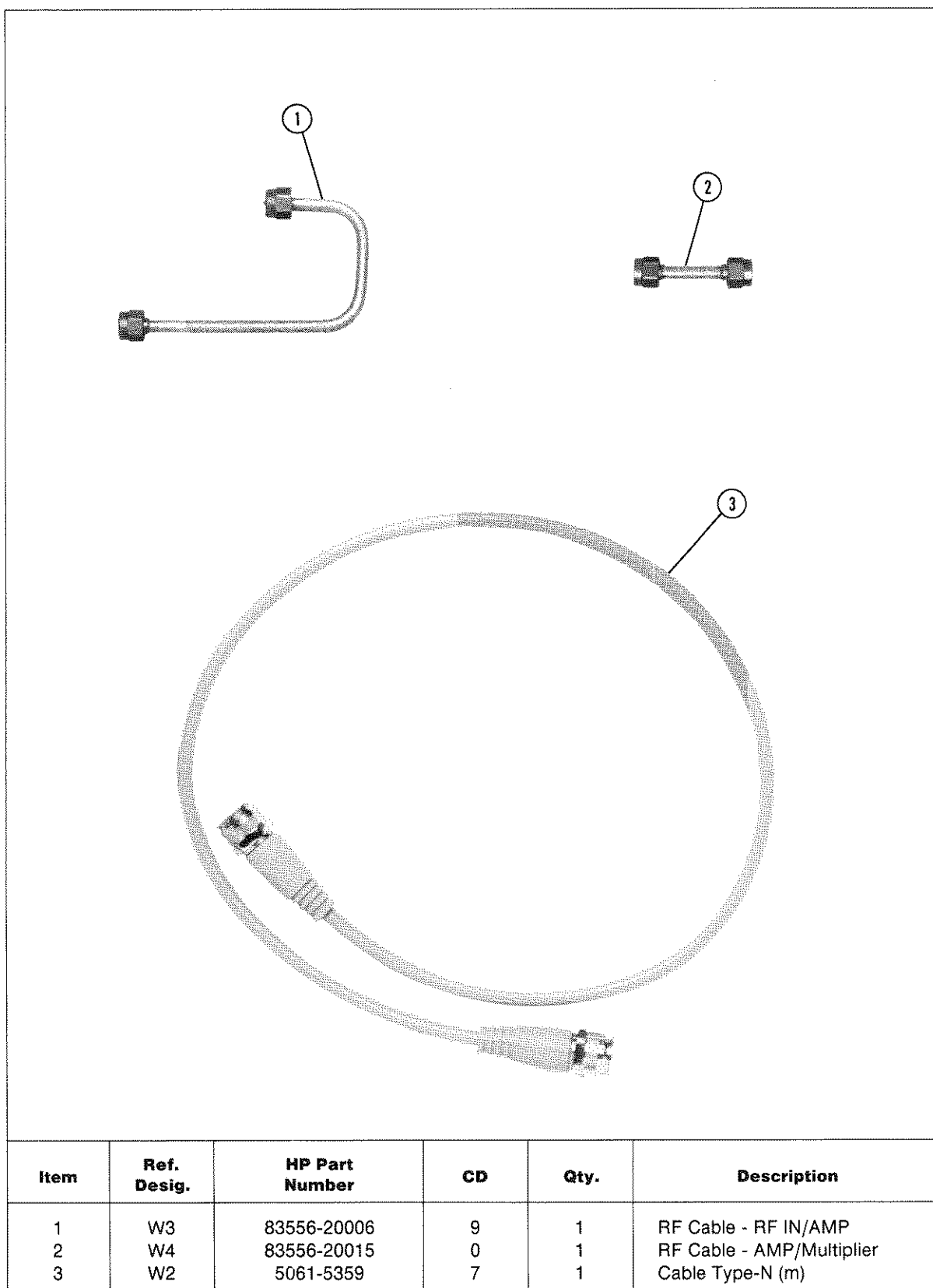
Figure 3-13. RF Cables Identification
