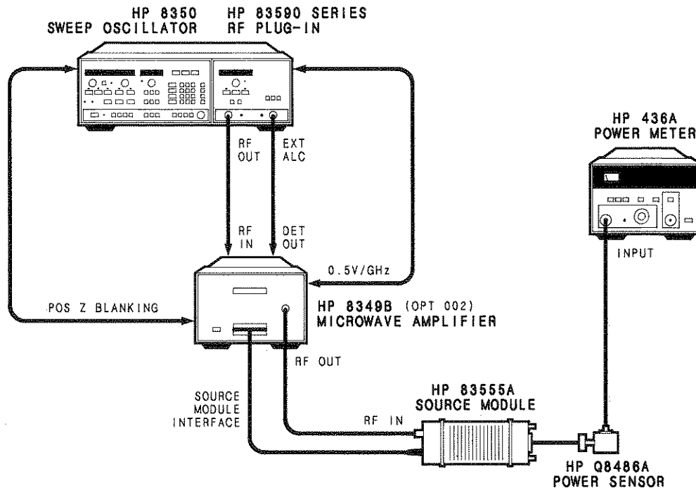
Figure 2-5. System Configuration
