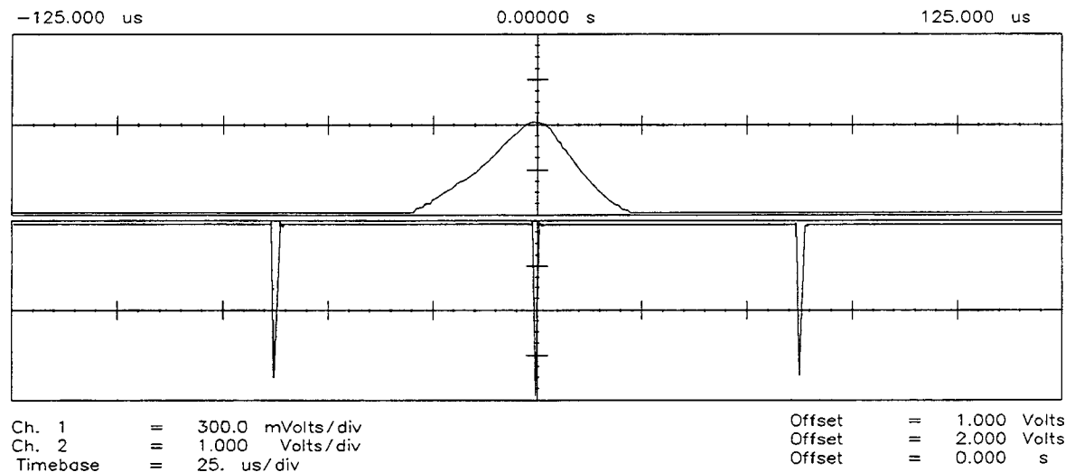
Figure 1-4. Video Signal on the Oscilloscope
