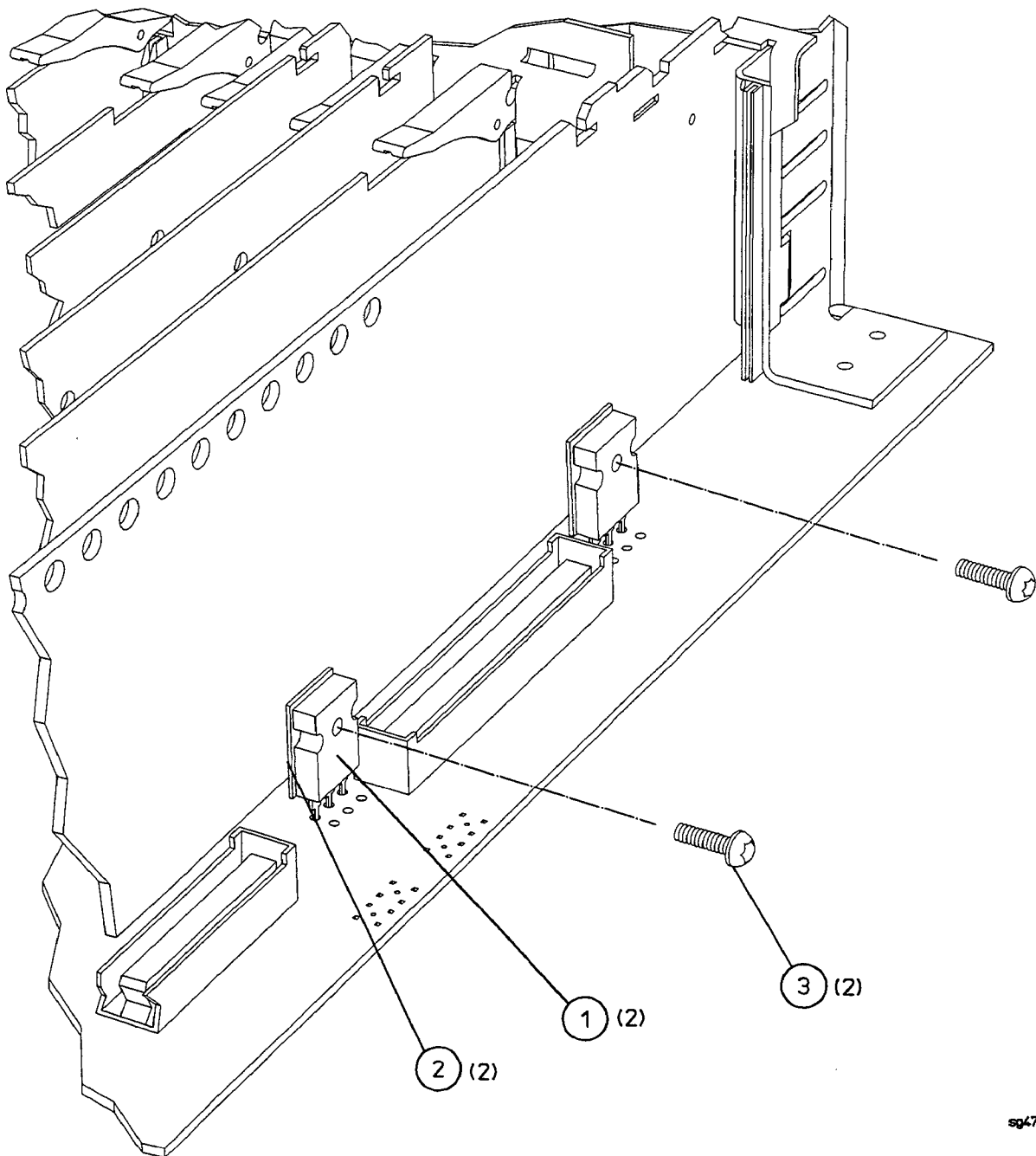
Figure 6-6. FET Assembly
