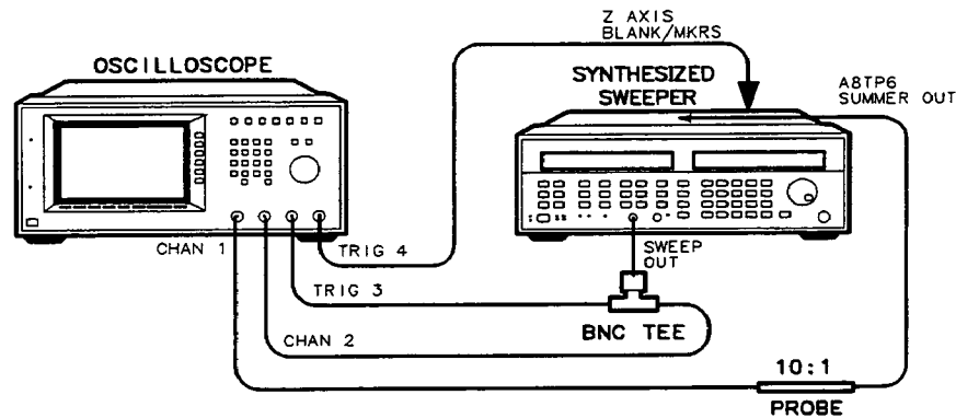
Figure 2-19. Start of Sweep DYO Adjustment Setup
