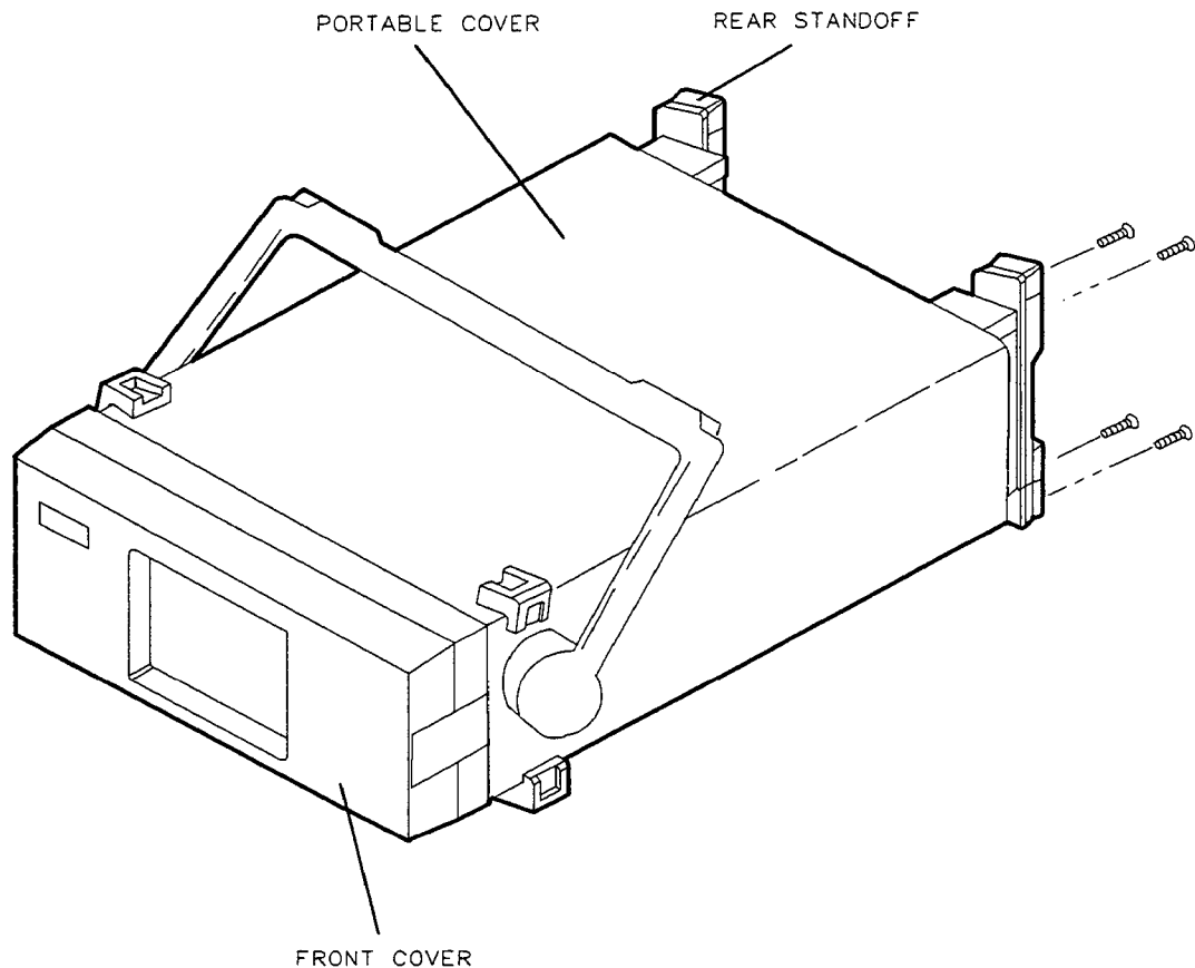
Figure 4-3. Portable Cover
