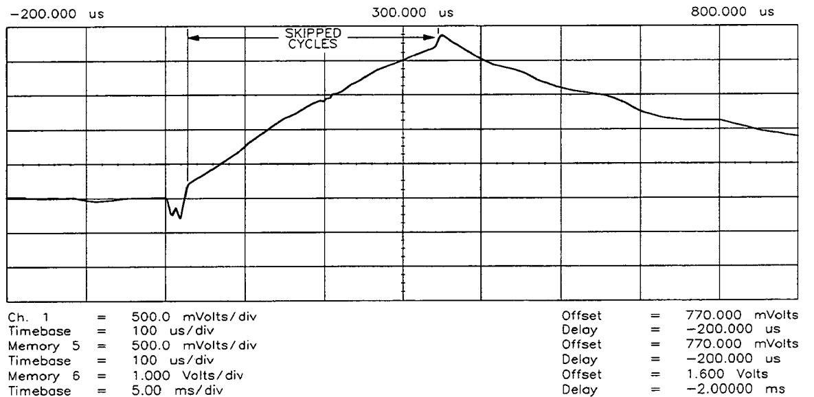
Figure 2-20. Skipped Cycles before Adjustment
