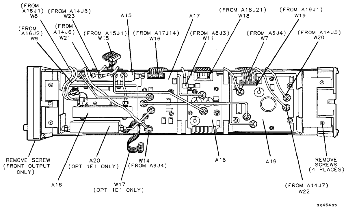
Figure 4-16. Screw and Cable Locations for RF Deck
