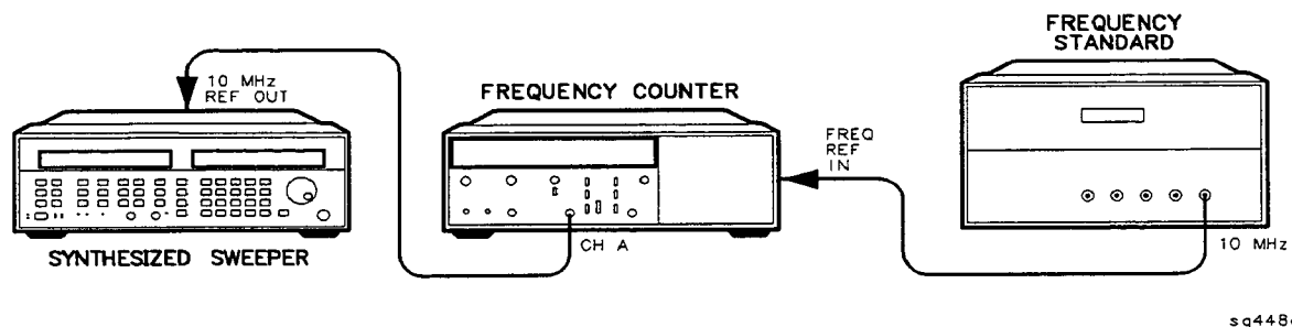
Figure 2-1. 10 MHz Standard Adjustment Setup
