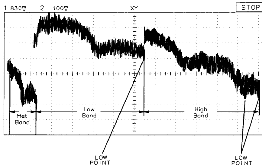
Figure 2-24. Low Power Points during Slow Sweep
