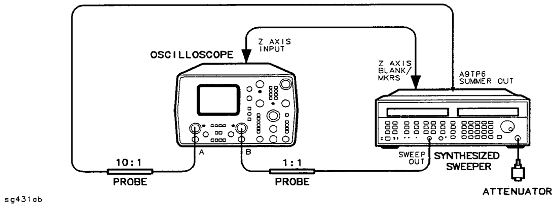
Figure 2-13. SAF Sense Adjustment Setup
