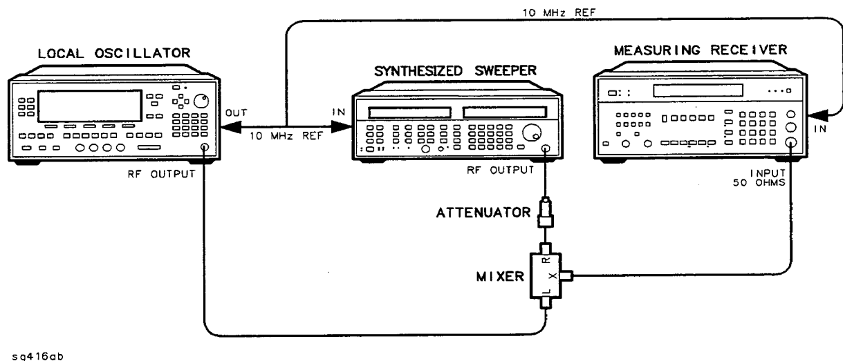
Figure 1-11. Residual FM Test Setup
