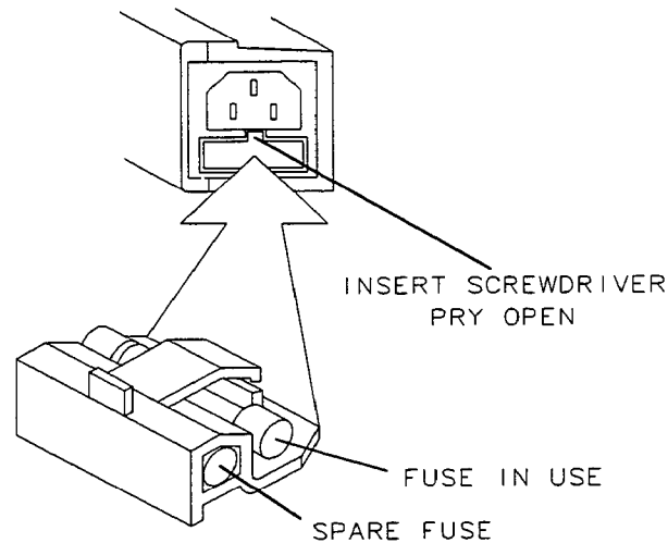
Figure 4-2. Fuse Removal
