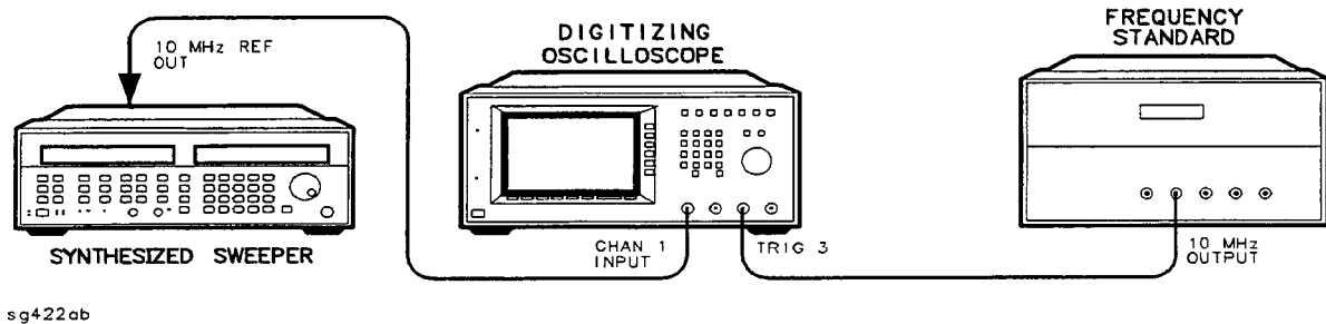
Figure 1-1. Internal Timebase: Aging Rate Test Setup
