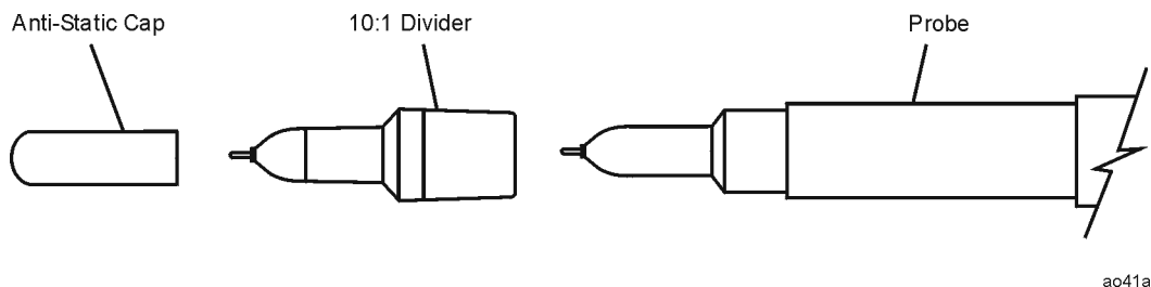
Figure 1 Probe with 10:1 Divider and Anti-Static Protection Cap
