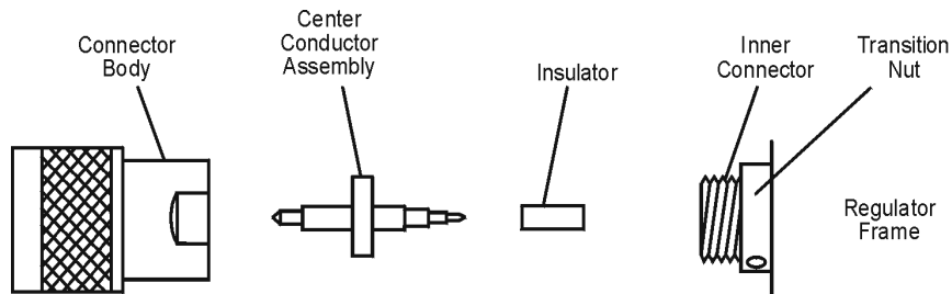
Figure 7-9 Output Connector Parts
