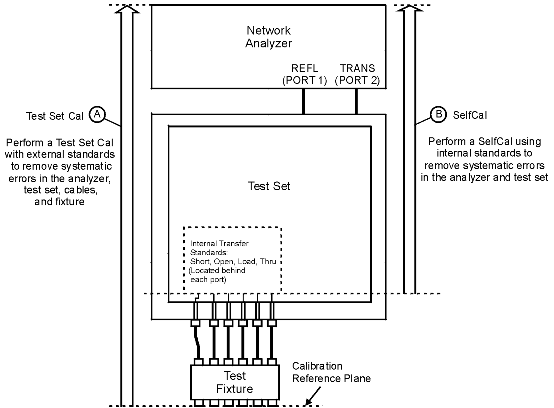
Figure 3-4 Drift Removal: Test Set Cal and SelfCal
