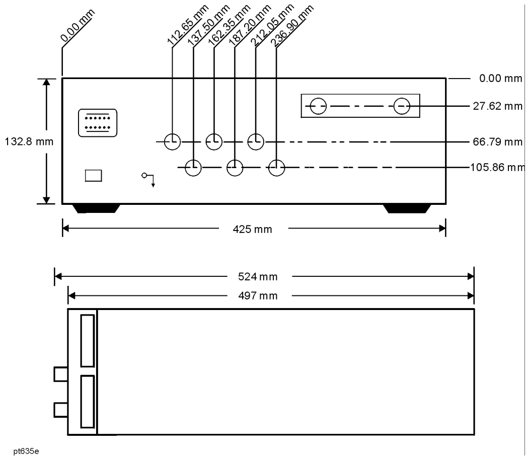
Physical Dimensions of the 87075C Option 006 Multiport Test Set 1
