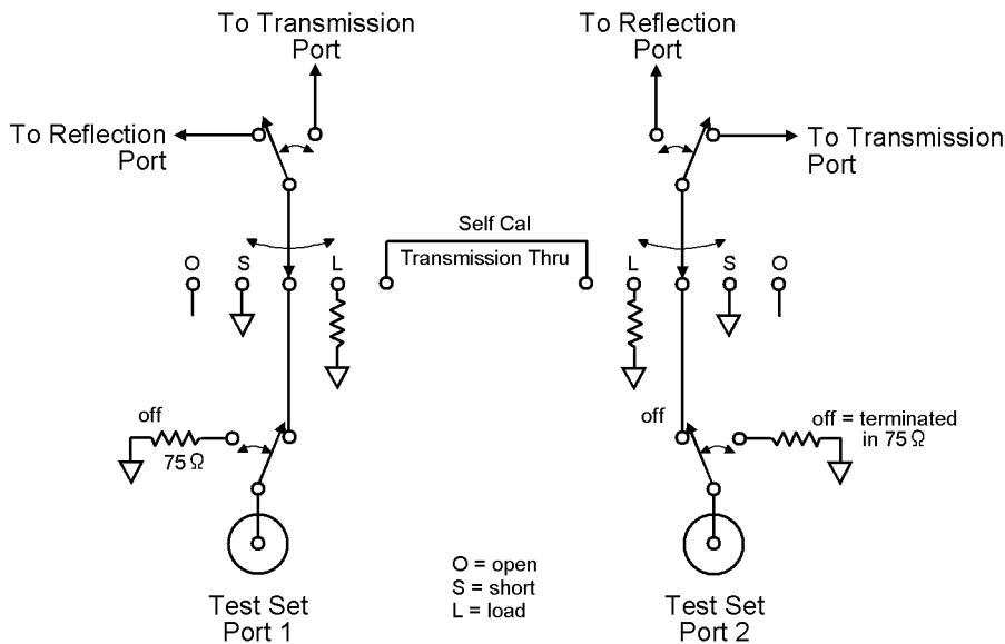
Figure 3-3 Internal Transfer Standards
