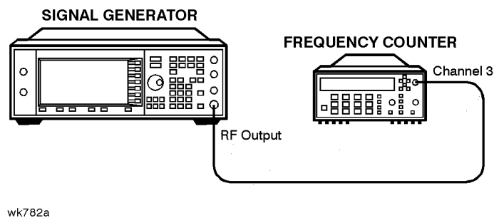
Figure 5-12 FM In-Band DAC Offset Calibration
