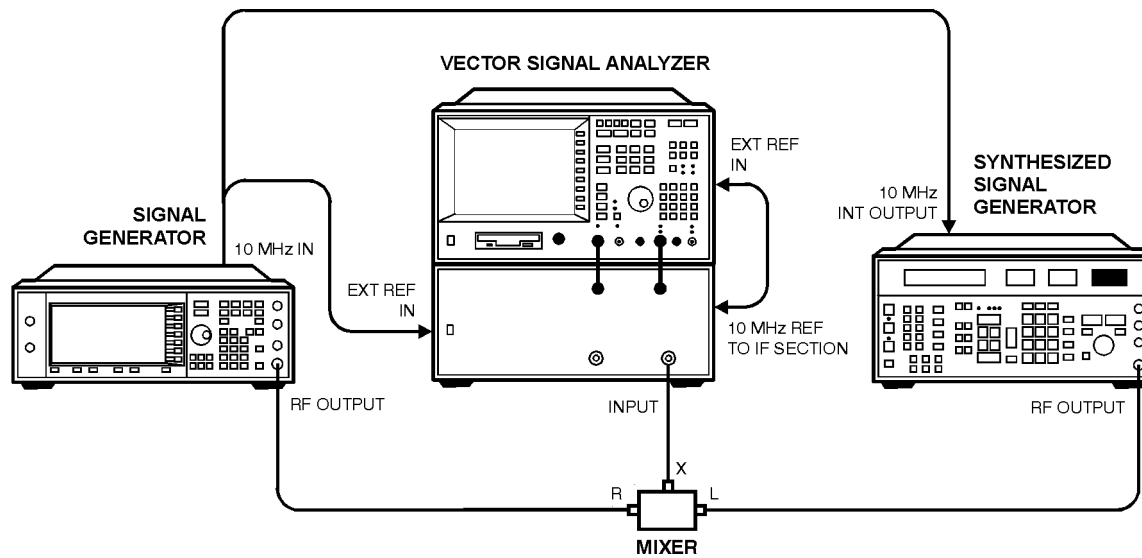
Figure 4-27 Custom I/Q RF Modulation Quality > 2000 MHz Test Setup
