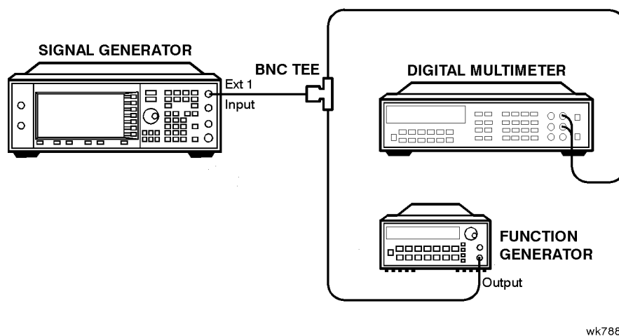
Figure 5-22 External Input Peak Detector Calibration Setup
