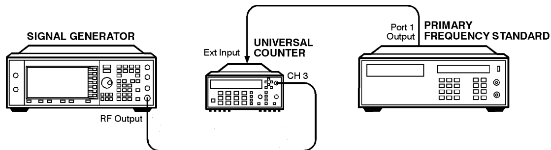
Figure 5-9 Timebase DAC Calibration Setup
