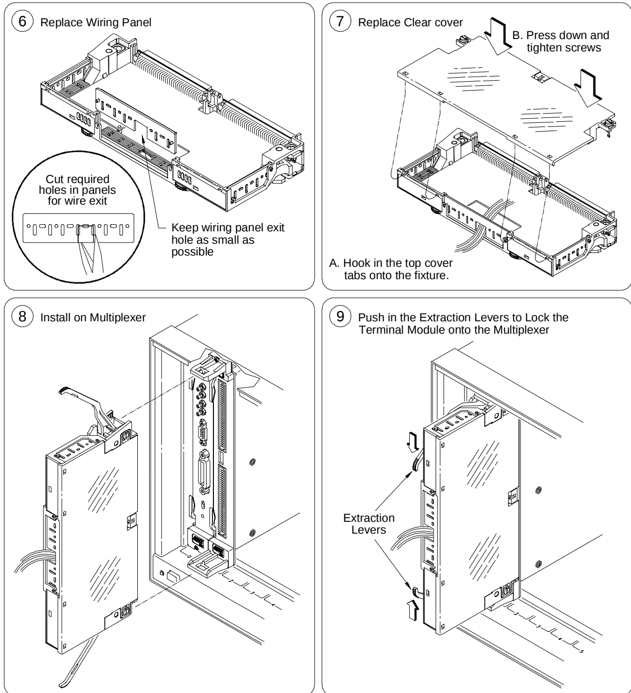
Figure 1-12. Steps to Wire Terminal Modules (continued)
