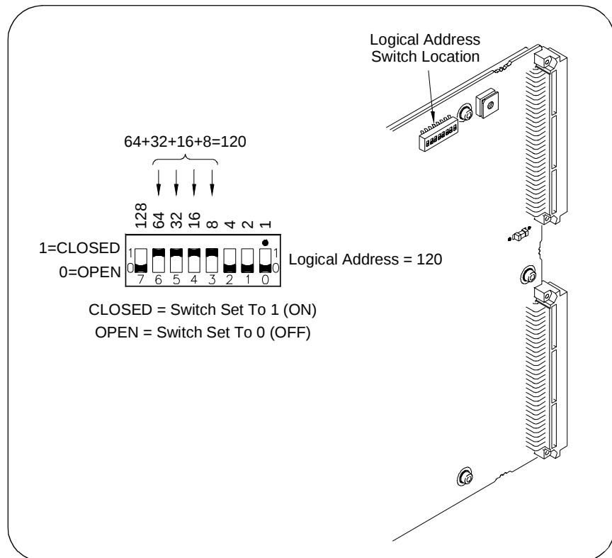
Figure 1-4. Setting the Logical Address Switch
