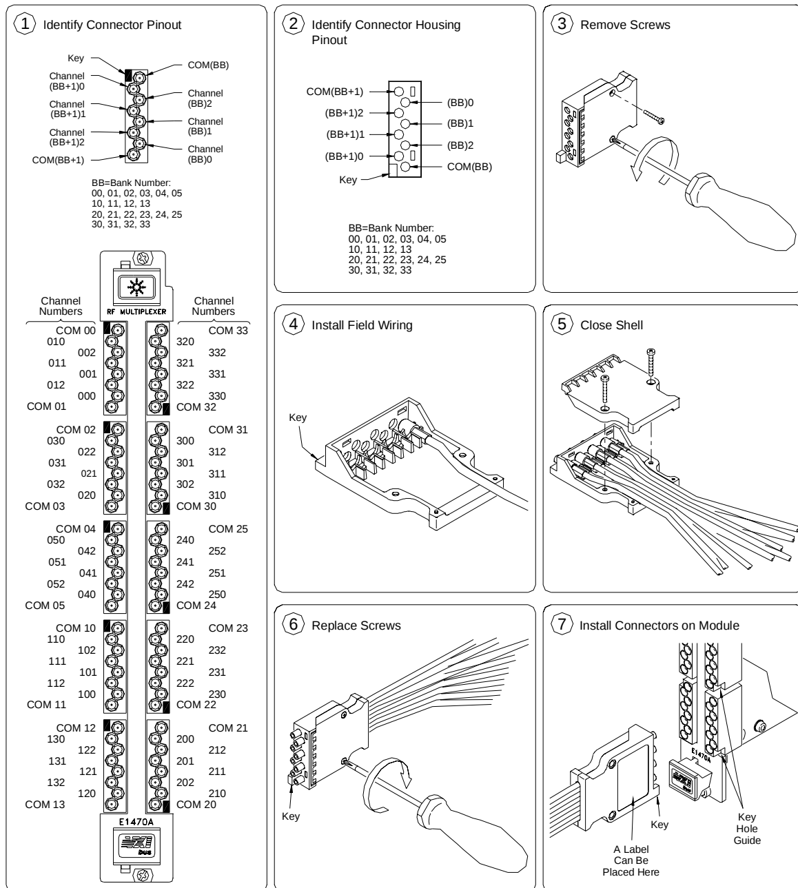
Figure 1-6. Installing User Wiring
