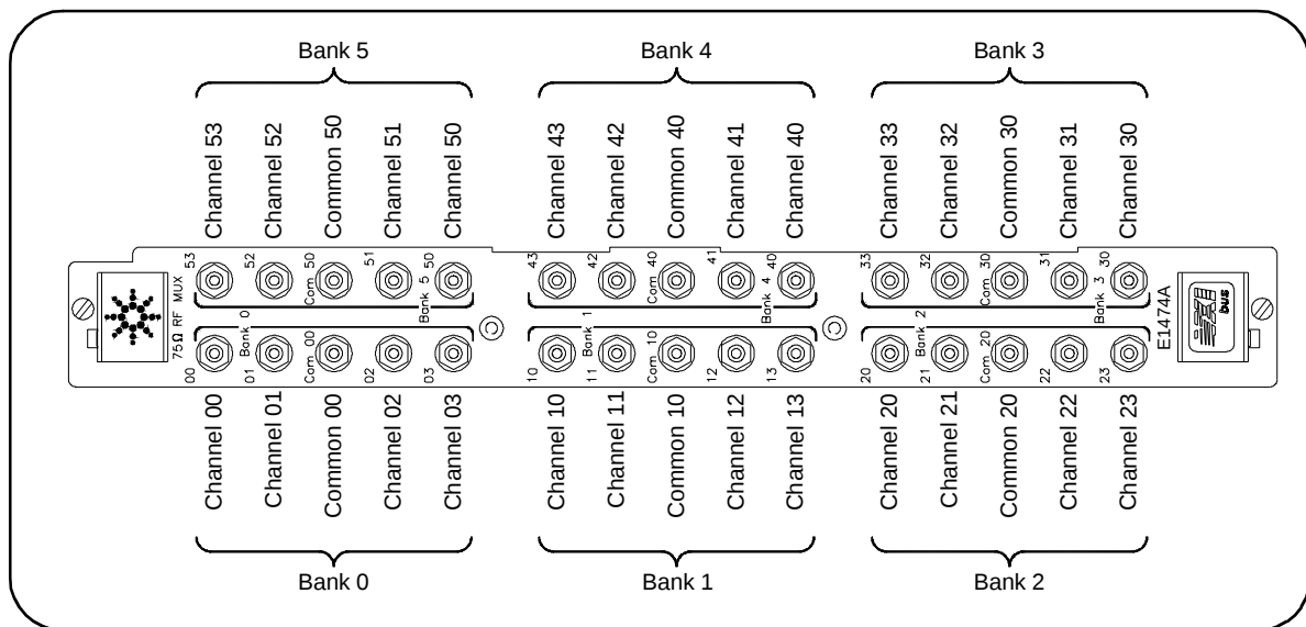
Figure 2-6. 75 Ohm SMB Connector Locations
