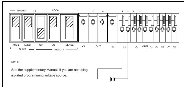
Figure 6. Remote Voltage Programming, Constant Voltage
