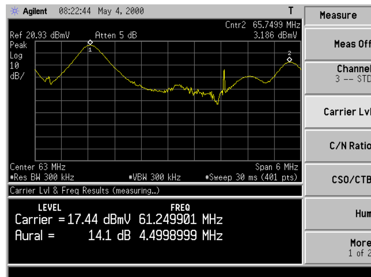
Measuring the Visual Level and Aural Carrier Difference (NTSC-M)
