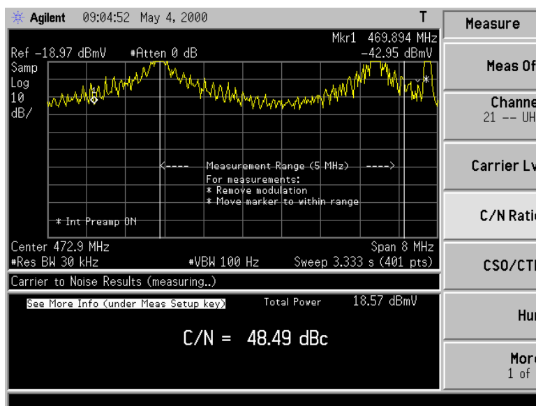
Figure 2-6 Carrier-to-Noise (PAL-B/G)
