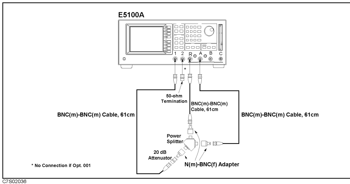
Figure 3-26. Magnitude Ratio Frequency Response Test Setup-2
