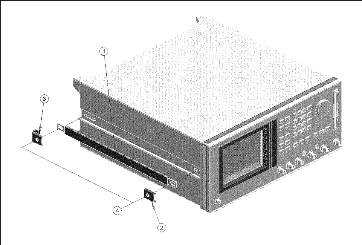
Figure 13-62. Strap Handle
