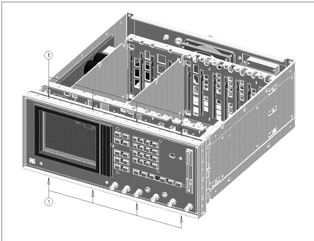
Figure 13-58. Front Screws
