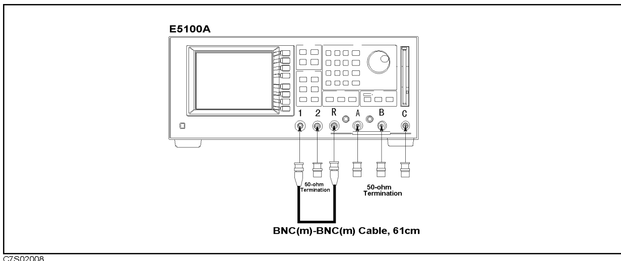
Figure 2-10. R into A, B, C Input Crosstalk Test Setup
