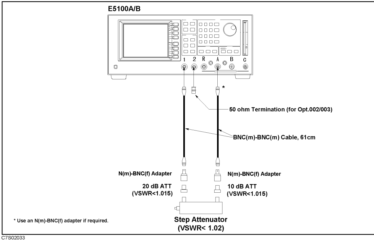
Figure 3-24. Dynamic Accuracy Test Setup 3 for Opt.118
