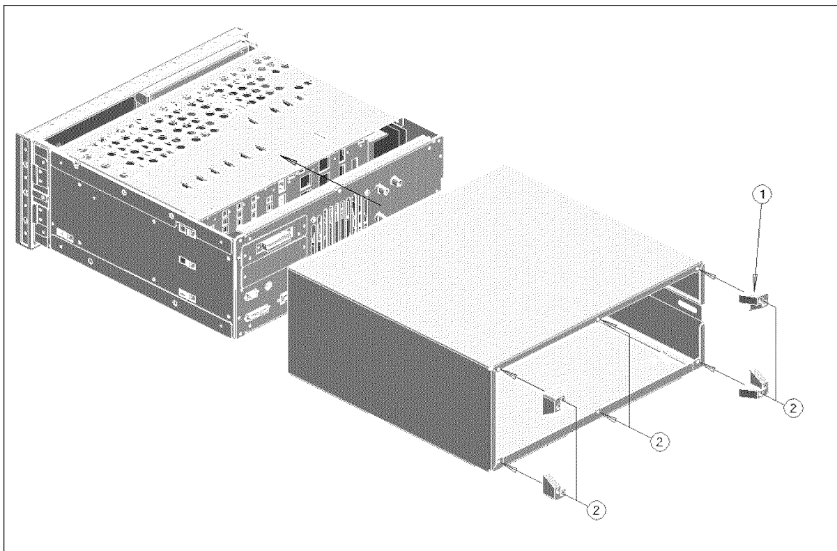
Figure 13-61. Rear Foot
