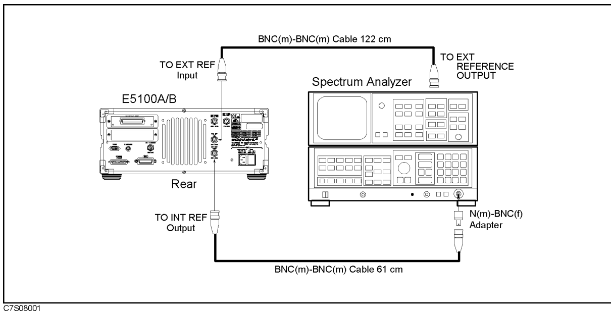
Figure 9-1. INT REF Test Setup
