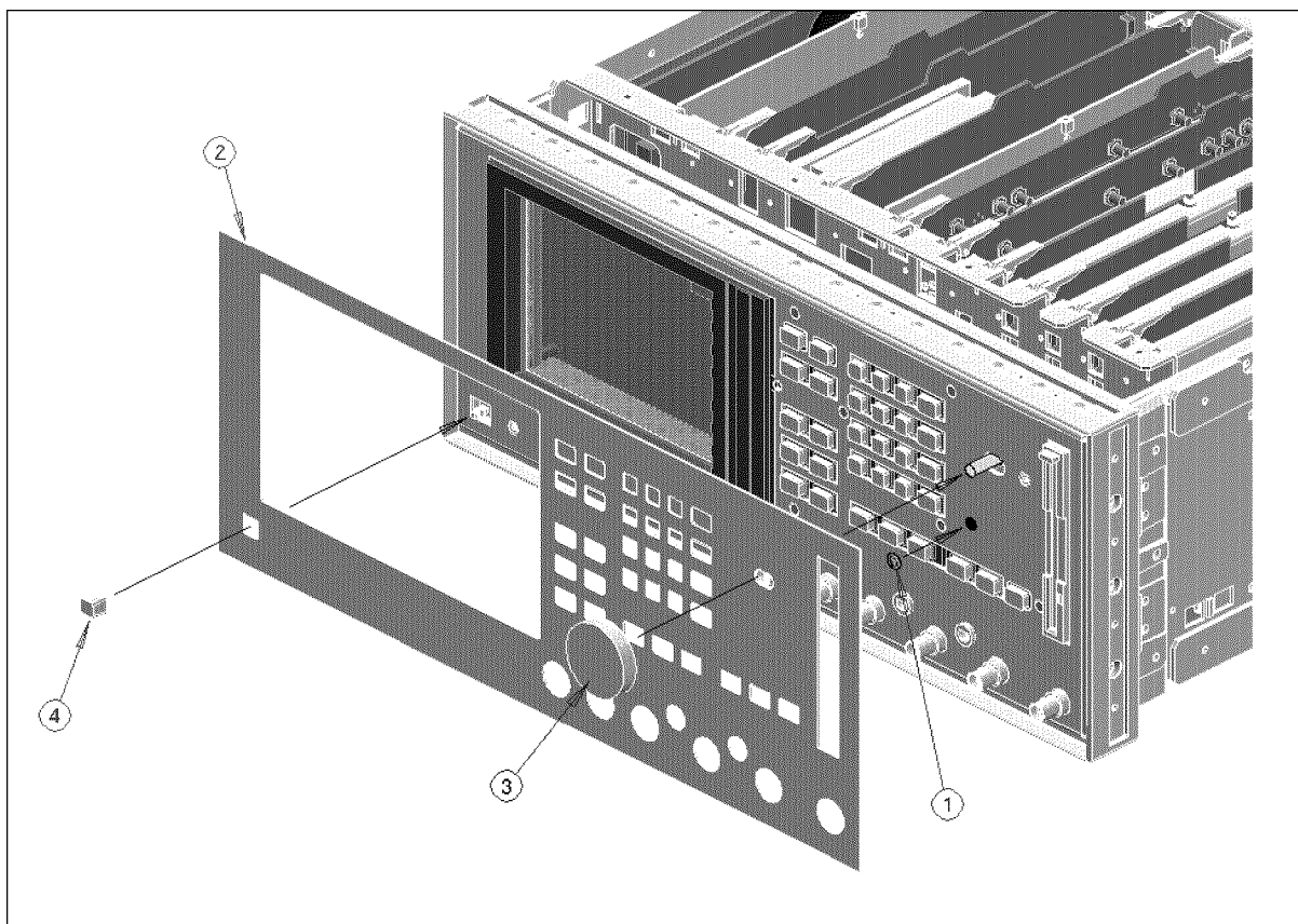
Figure 13-41. Front Panel Assembly
