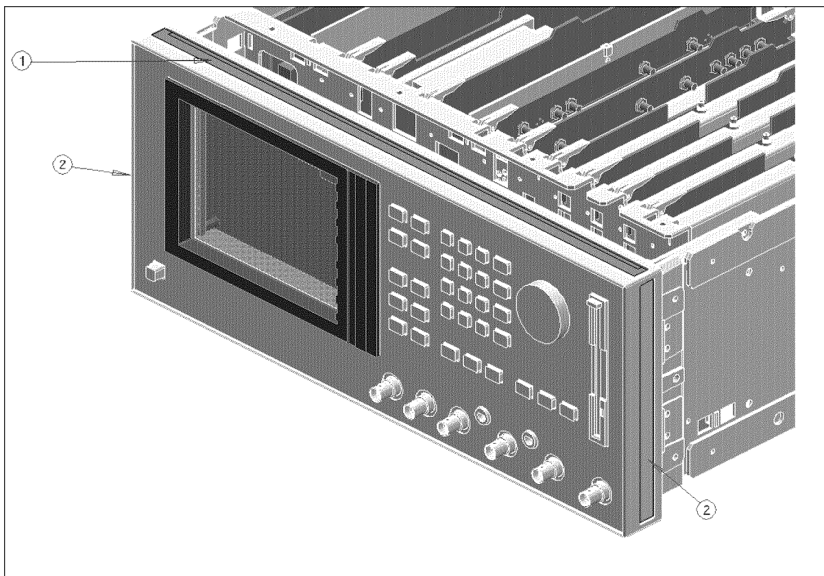
Figure 13-59. Front Trim
