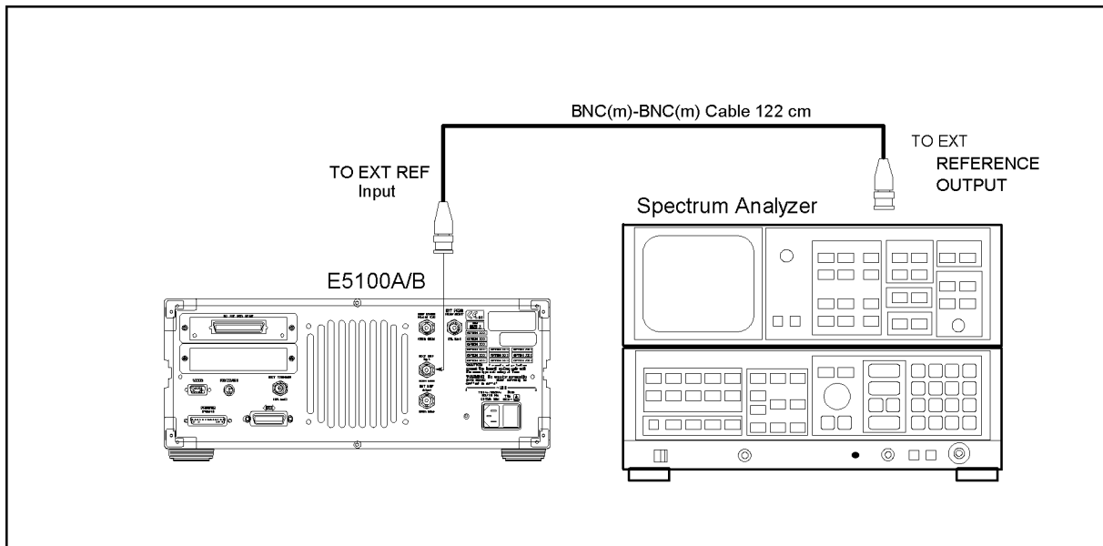
Figure 9-3. EXT REF Test Setup
