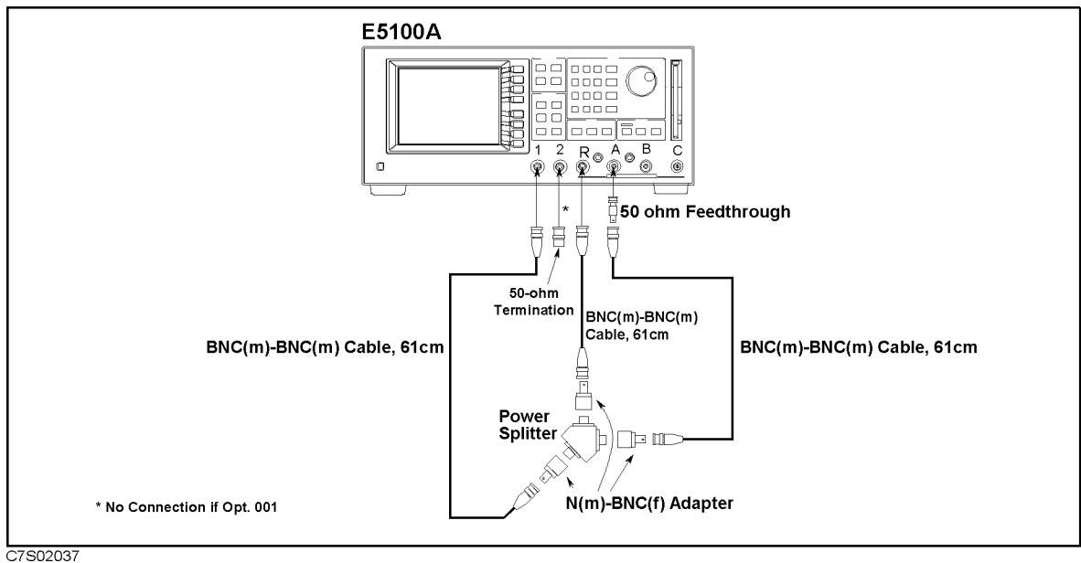
Figure 2-31. Magnitude Ratio Frequency Response Test Setup-3
