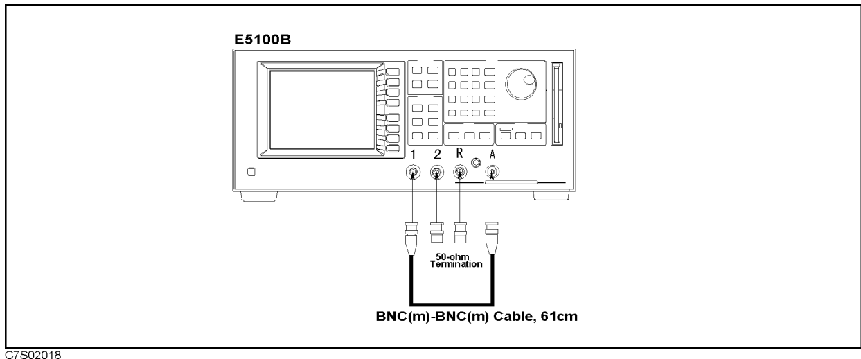
Figure 2-15. A into R Input Crosstalk Test Setup
