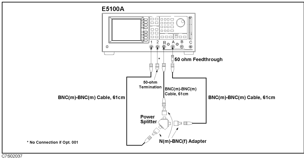
Figure 3-27. Magnitude Ratio Frequency Response Test Setup-3
