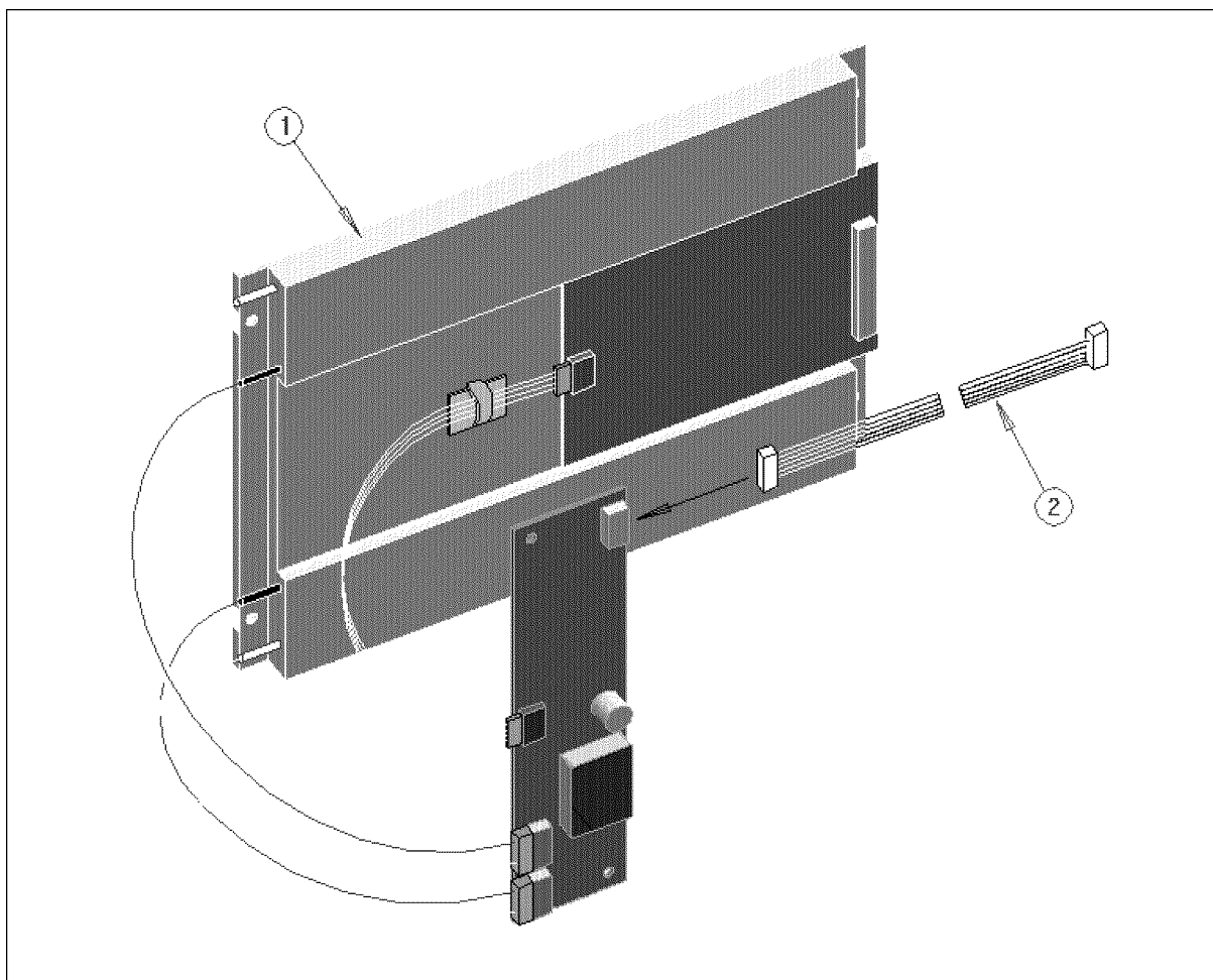
Figure 13-30. Color LCD Assembly 3/6
