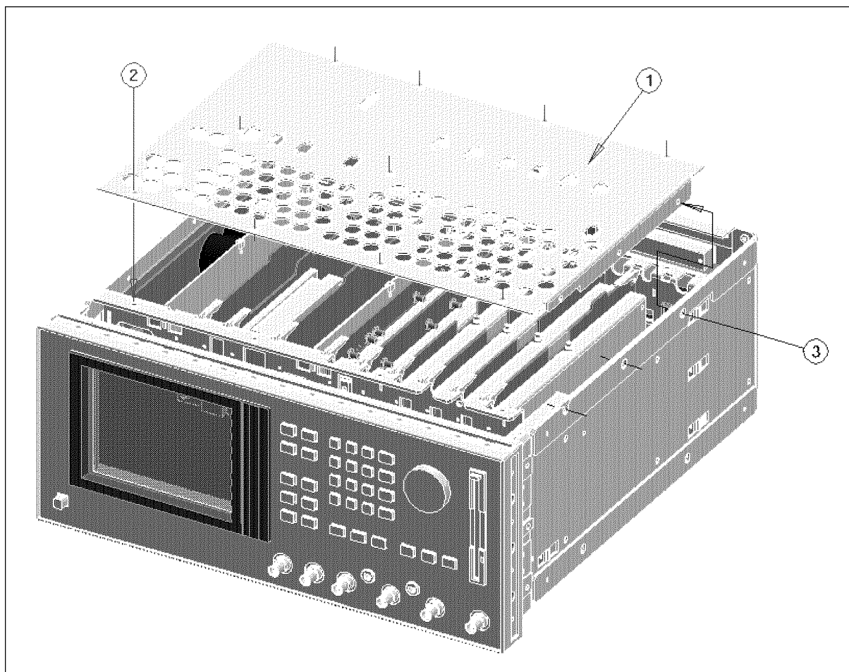
Figure 13-60. Shield Plate
