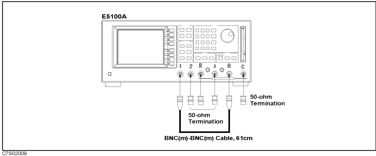
Figure 2-12. B into R, A, C Input Crosstalk Test Setup
