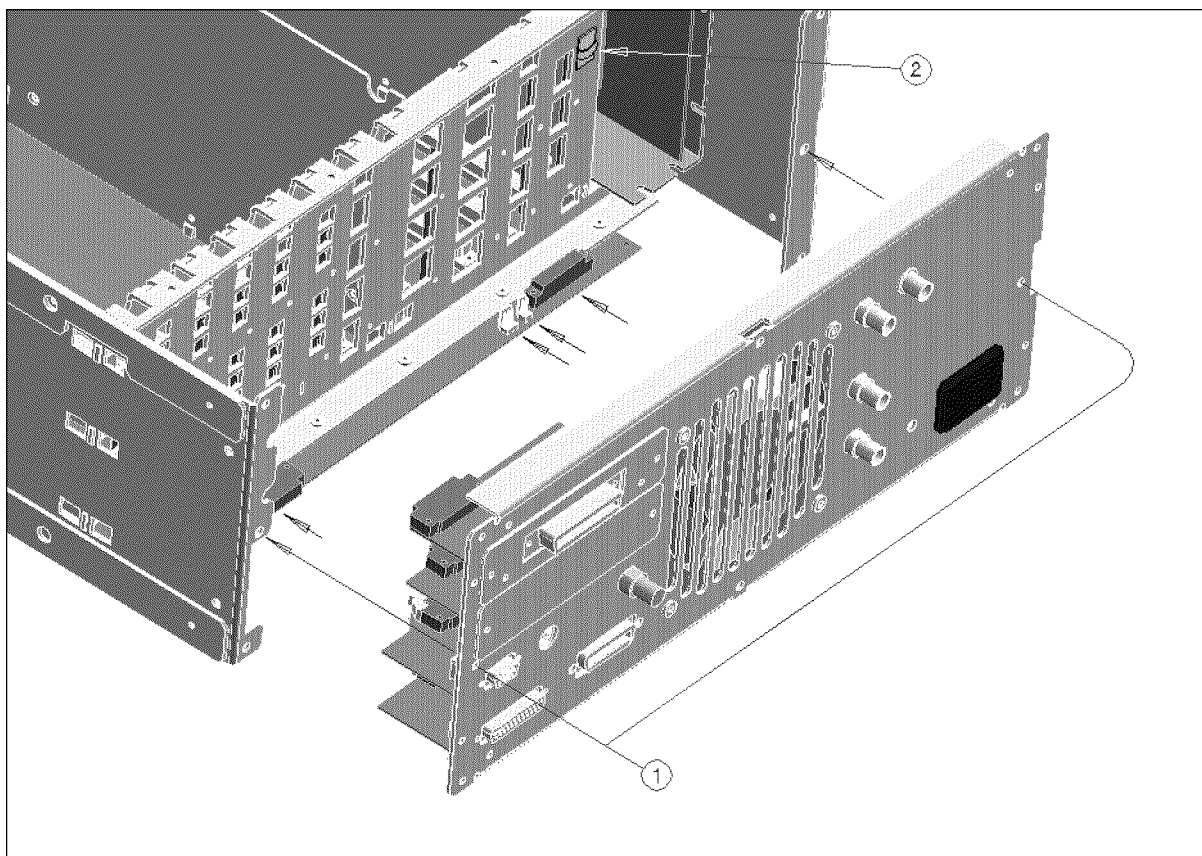
Figure 13-55. Rear Assembly
