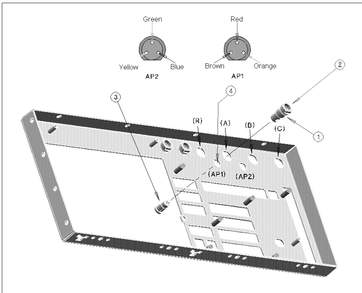
Figure 13-21. Input Port and Probe Power Connector Assemblies
