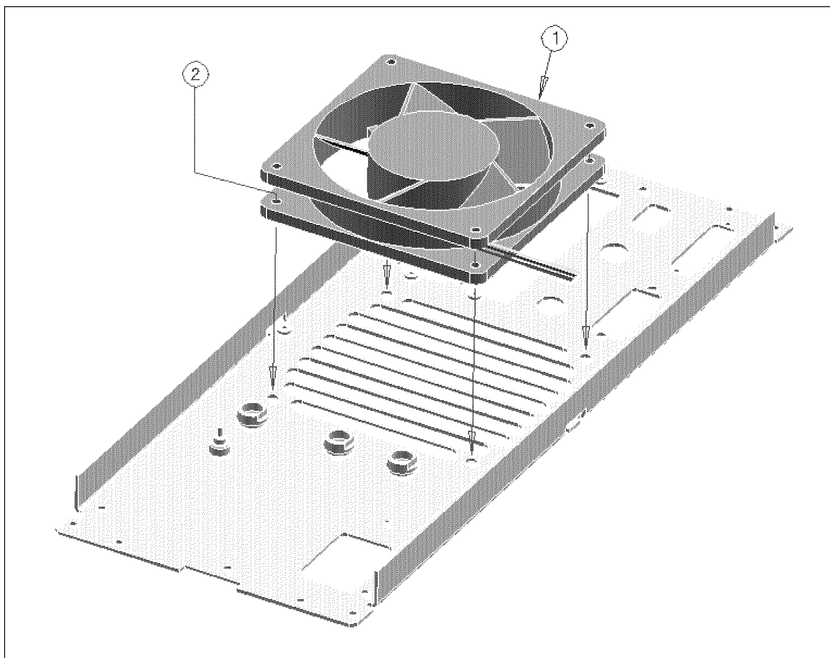
Figure 13-47. Fan Assembly
