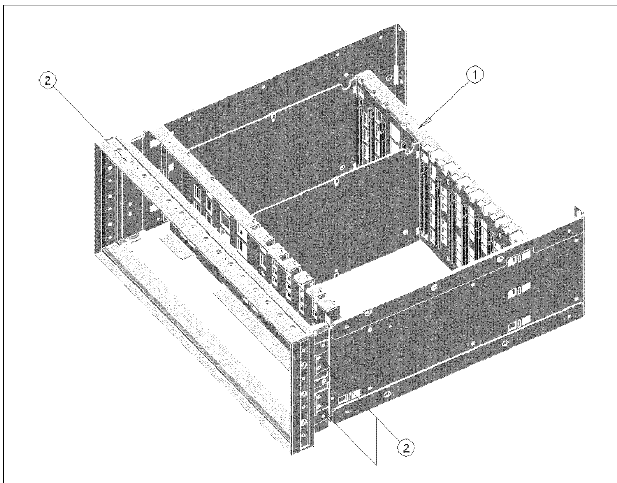
Figure 13-57. Chassis Parts
