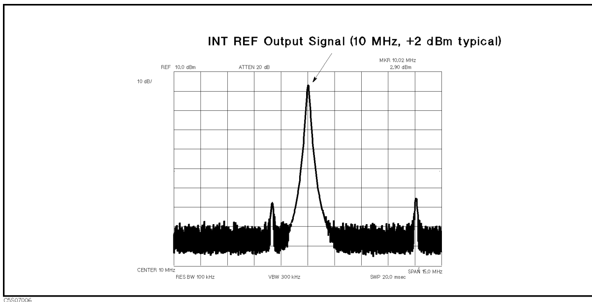
Figure 9-2. Typical INT REF Signal
