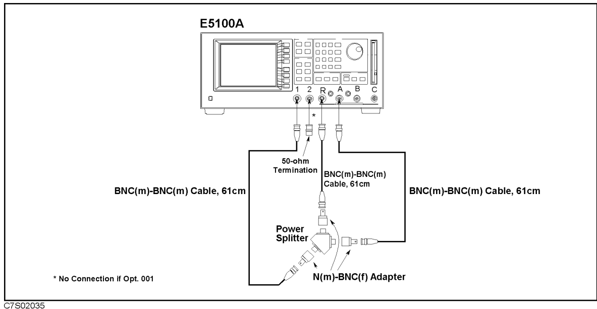
Figure 3-25. Magnitude Ratio Frequency Response Test Setup-1
