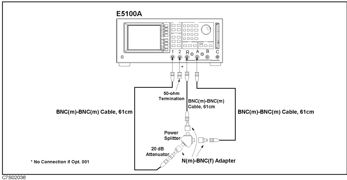
Figure 2-30. Magnitude Ratio Frequency Response Test Setup-2
