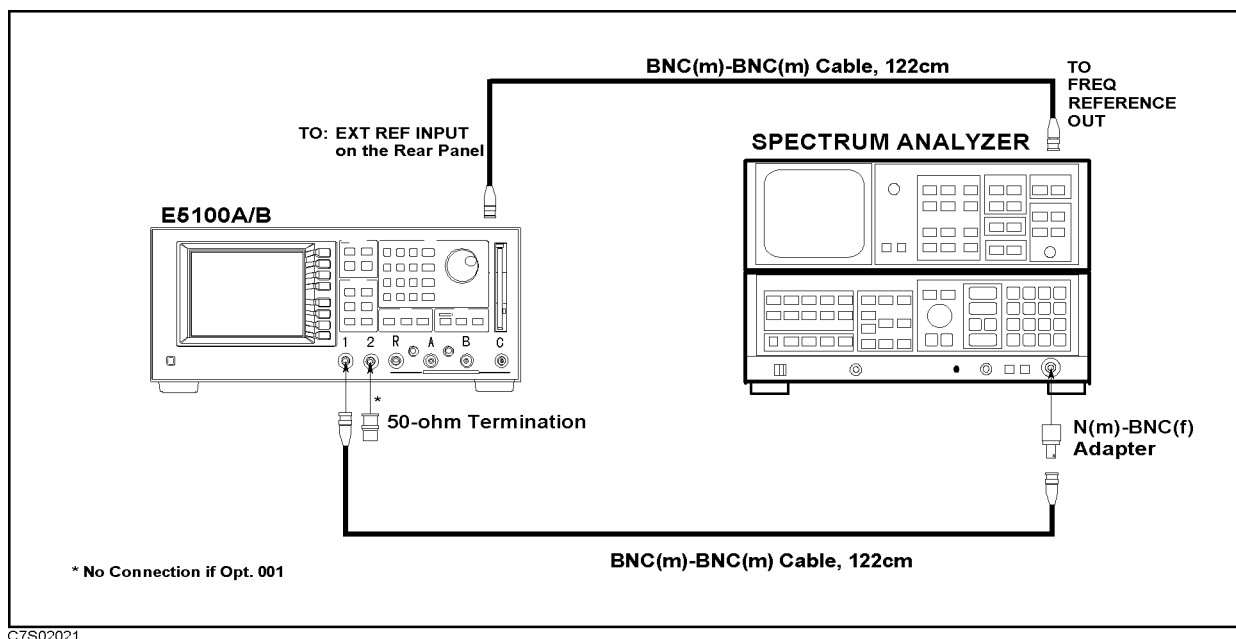
Figure 2-3. Non-Harmonic Spurious Test Setup
