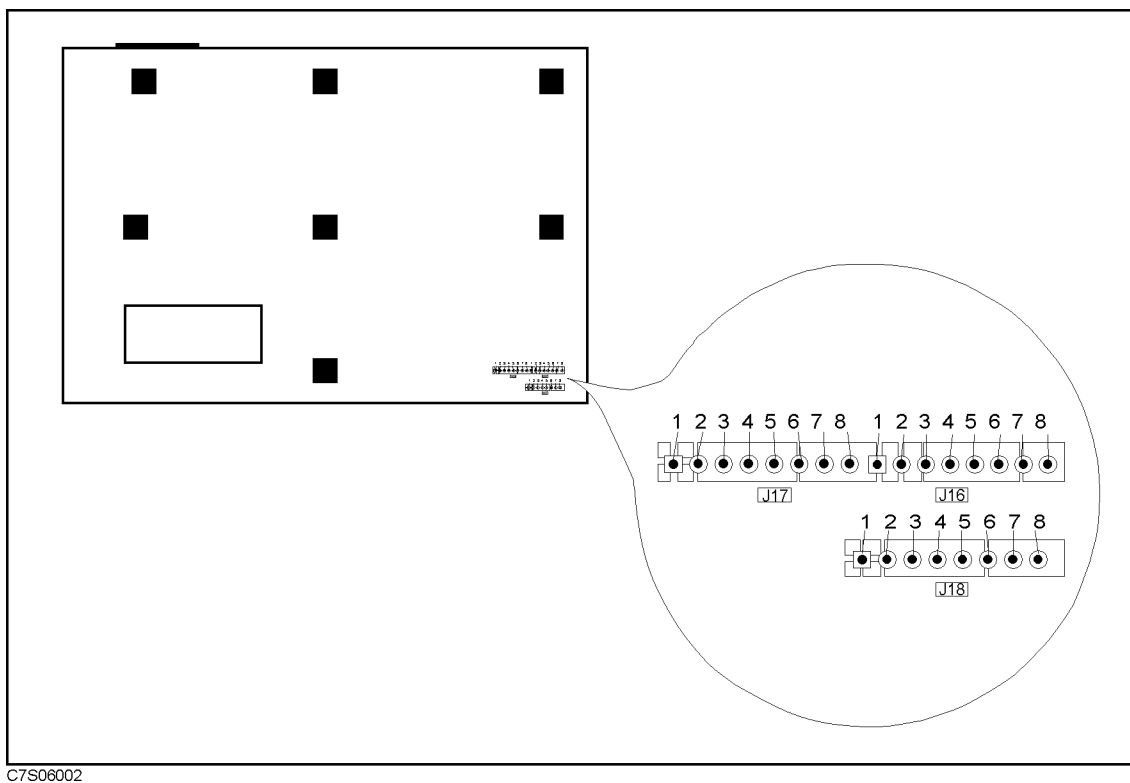
Figure 7-2. Power Supply Output Pins on A20 Mother Board
