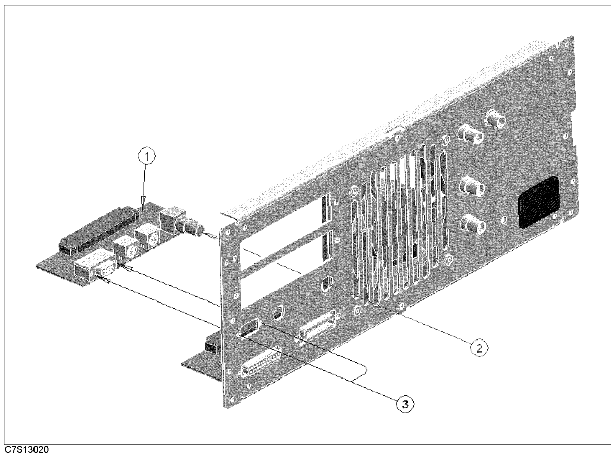
Figure 13-50. External Display/KeyBoard I/F
