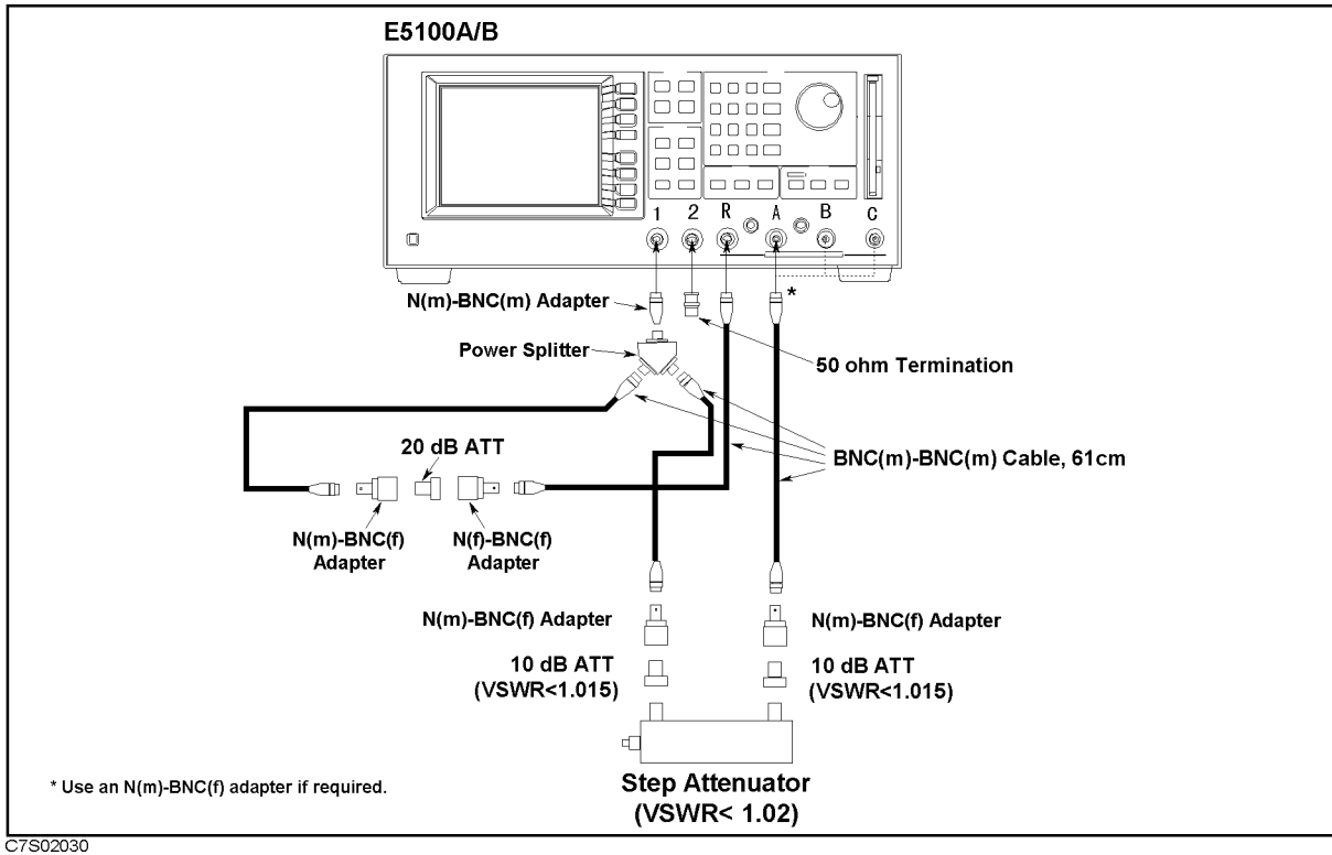
Figure 2-25. Dynamic Accuracy Test Setup 3 for Opt.200/300/400 with Opt.003 without Opt.010
