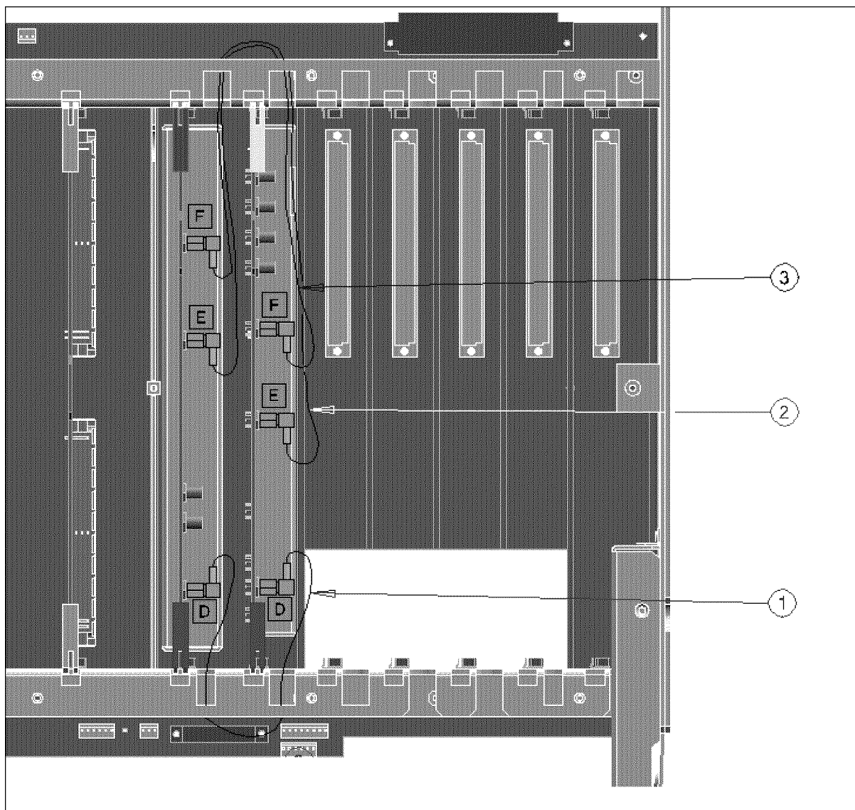
Figure 13-13. RF Cables (A27 to A24)
