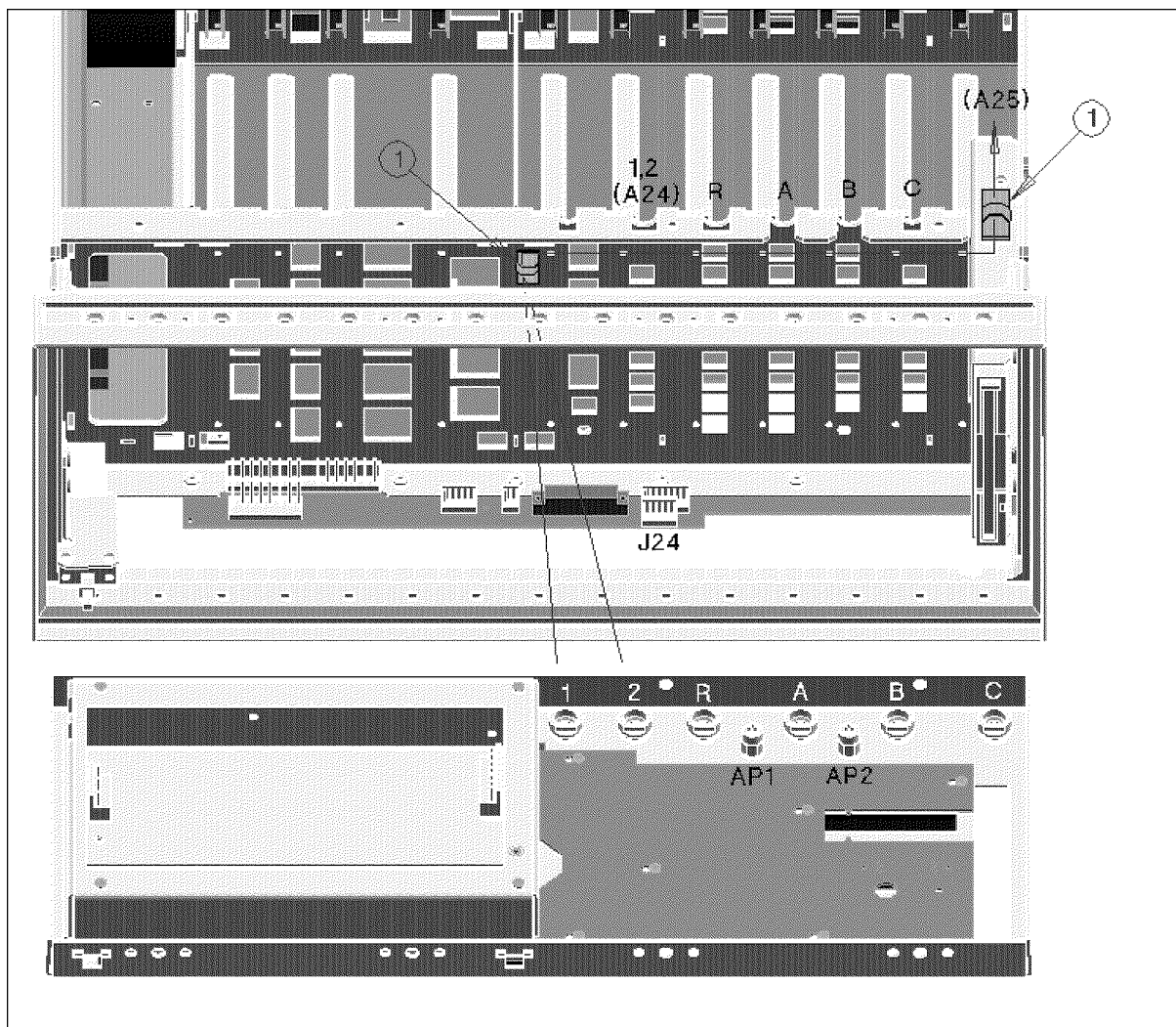
Figure 13-20. RF OUT Cable Clamps (Opt.010 or 600)
