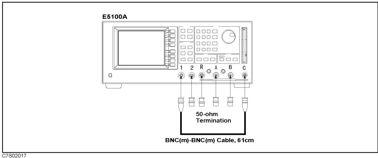
Figure 2-13. C into R, A, B Input Crosstalk Test Setup
