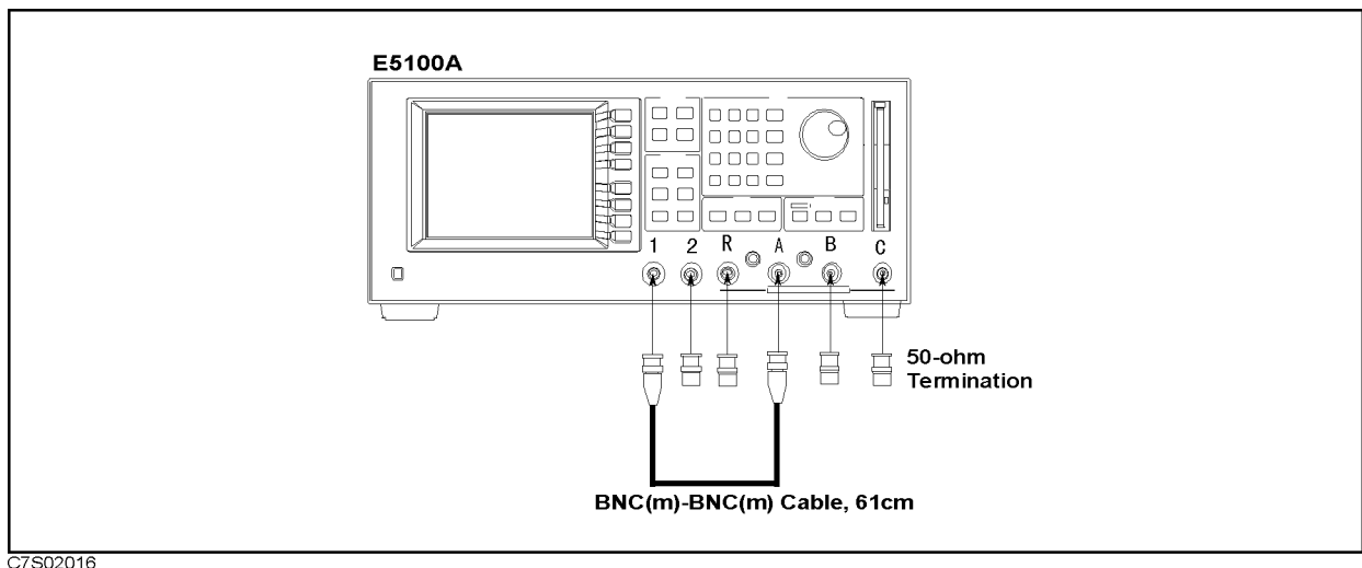
Figure 3-10. A into R, B Input Crosstalk Test Setup
