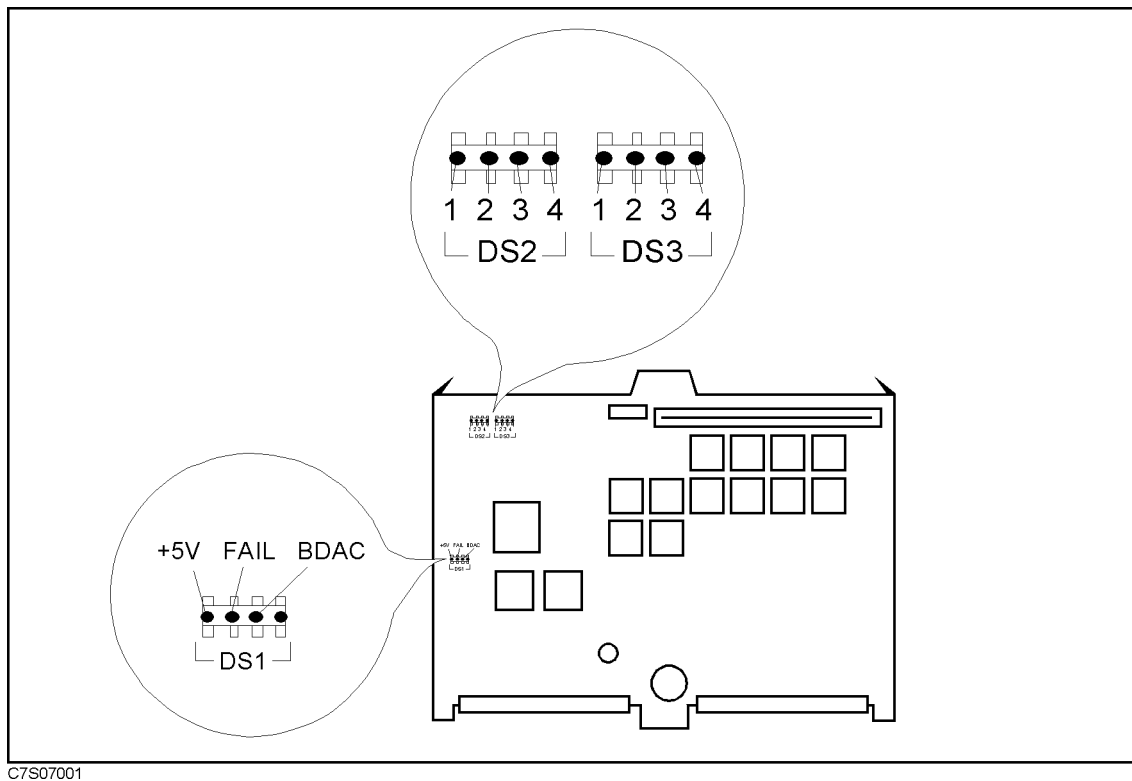
Figure 8-2. A1 CPU LED Location
