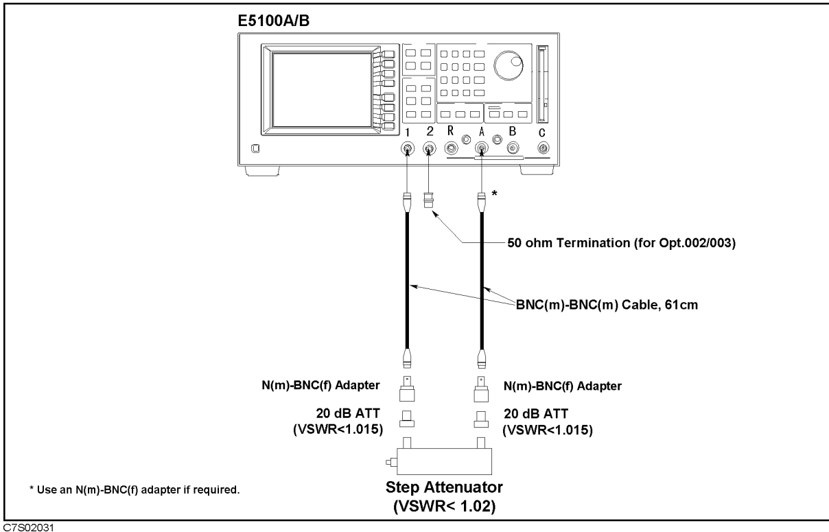
Figure 3-22. Dynamic Accuracy Test Setup 1 for Opt.118
