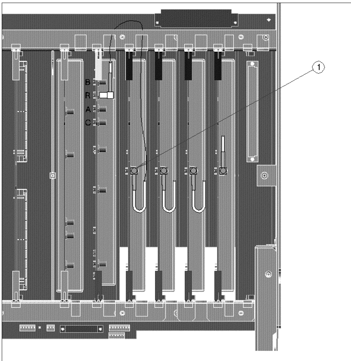
Figure 13-16. RF Cables (A24 to A26)
