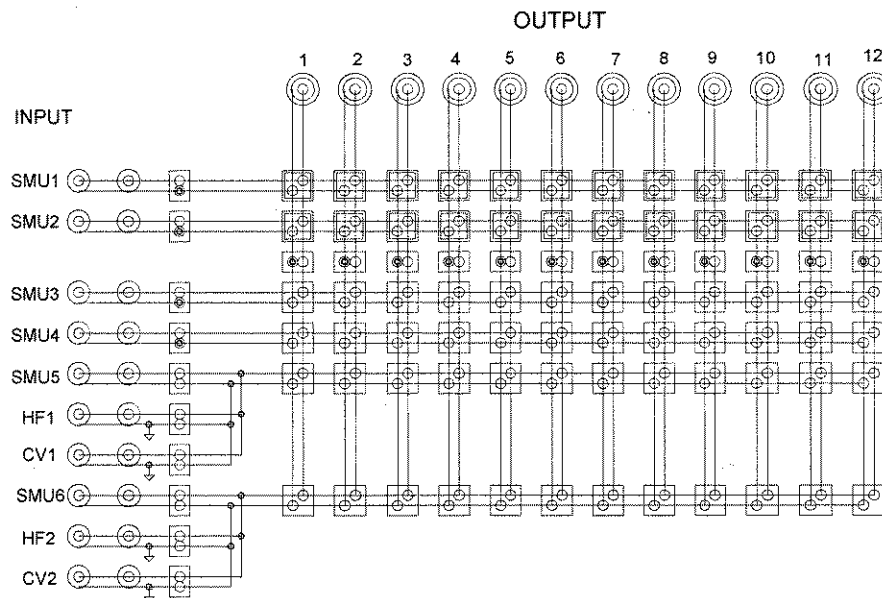
Agilent E5252A Block Diagram
