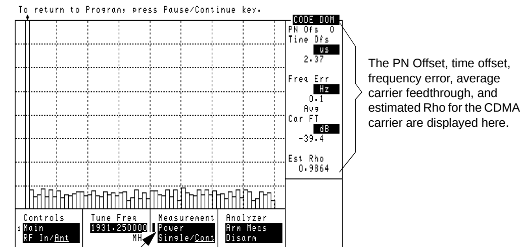
Figure 4-8 Making Code Domain Analyzer Measurements
