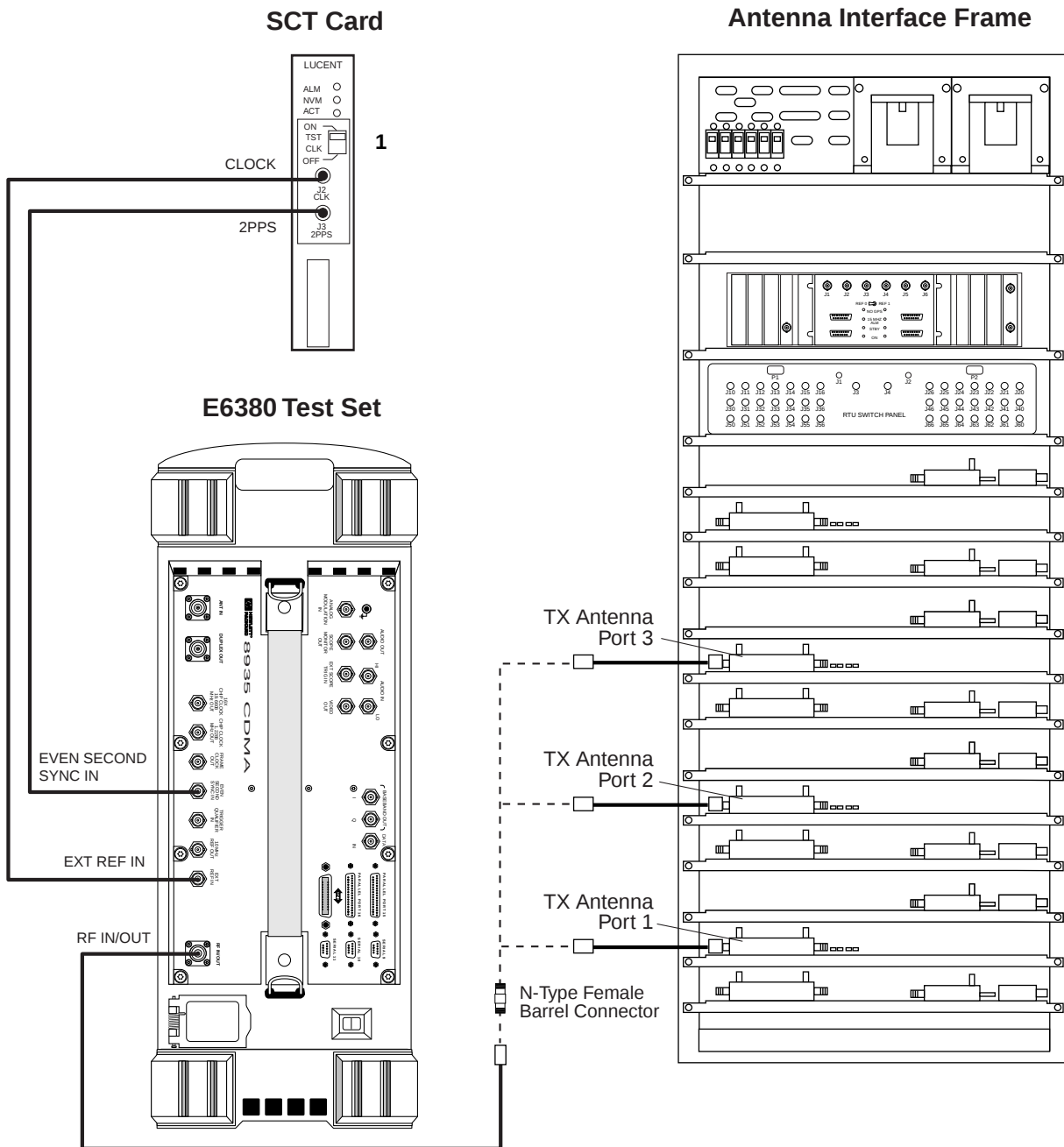
Figure 3-4 Series II Base Station TX Antenna Port (Out of Service) Connections
