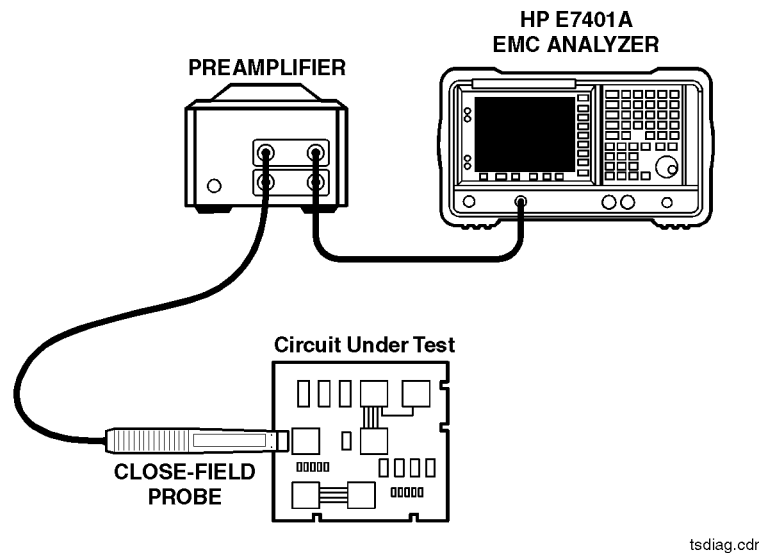
EMC Diagnostic Measurement Setup
