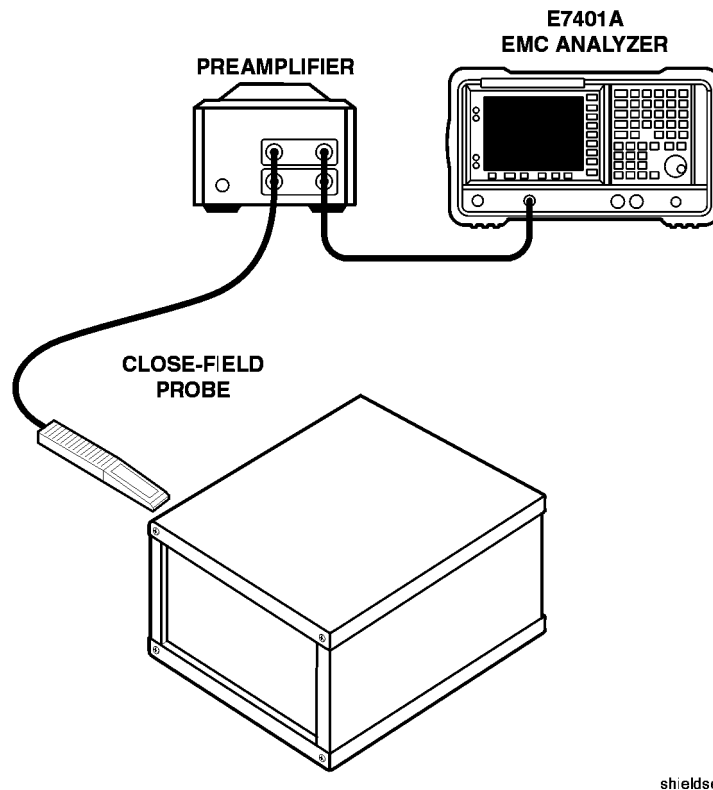
Probing a Shield Seam
