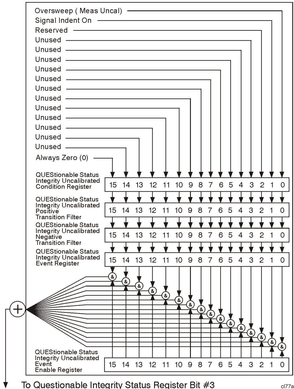
Questionable Status Integrity Uncalibrated Register Diagram
