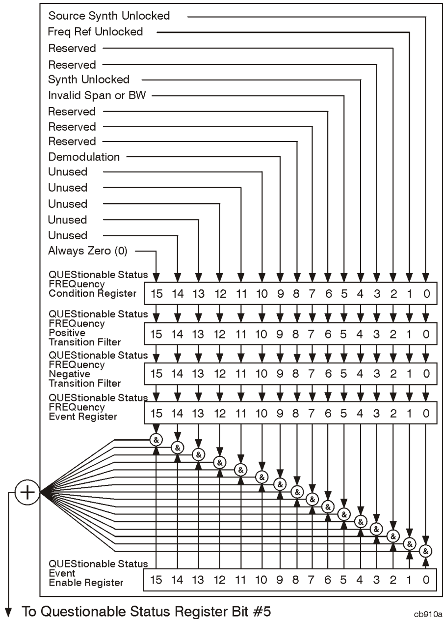
Questionable Status Frequency Register Diagram
