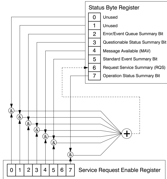
Status Byte Register Diagram
