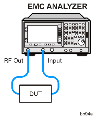
Figure 2-5 Transmission Measurement Test Setup
