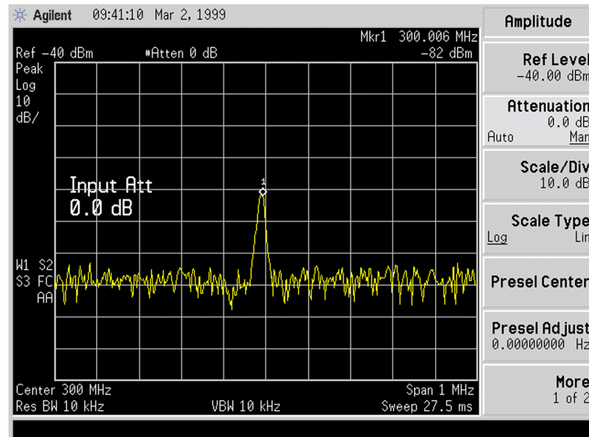
Figure 1-28 Using 0 dB Attenuation
