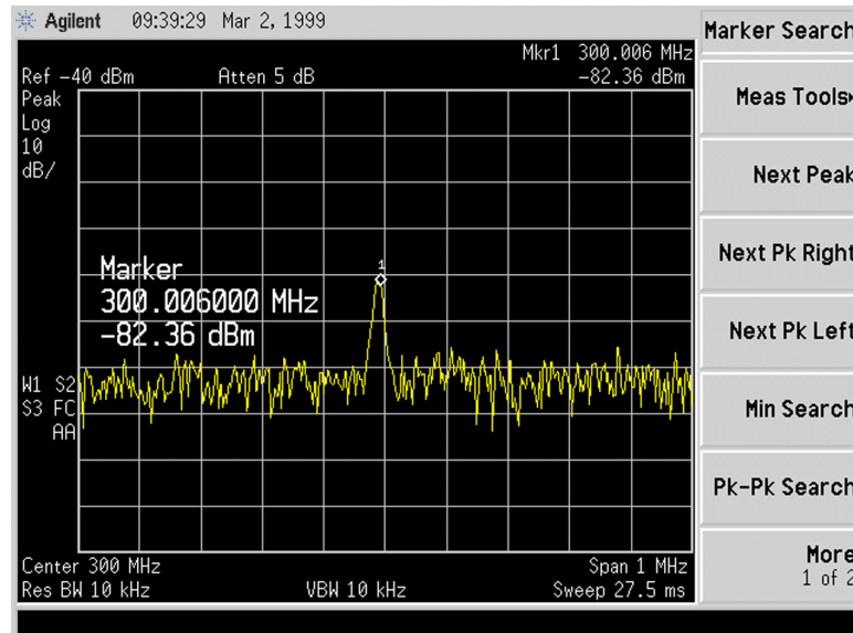
Figure 1-26 Low-Level Signal
