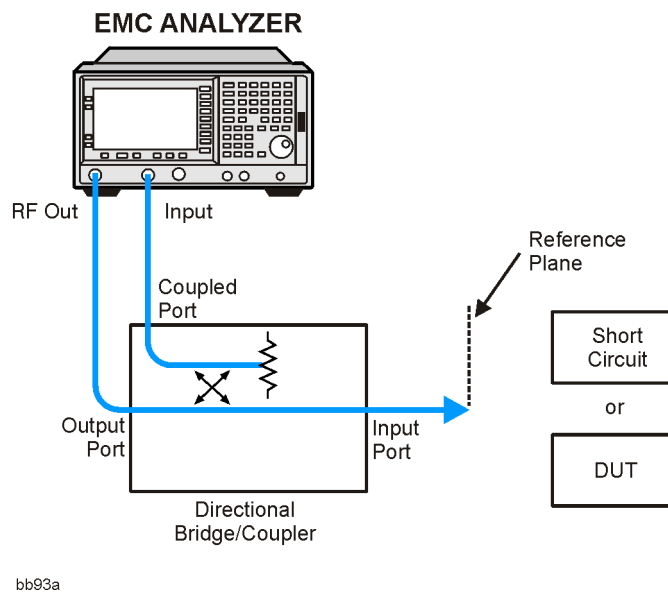
Figure 2-13 Reflection Measurement Short Calibration Test Setup
