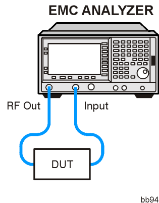
Figure 2-8 Transmission Measurement Test Setup
