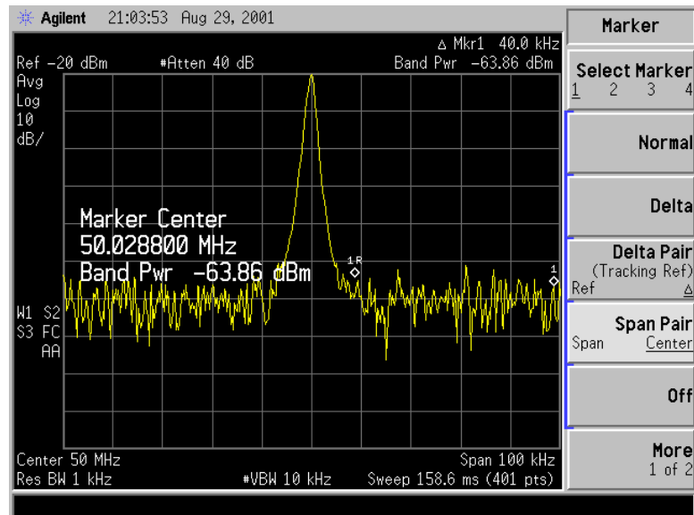
Figure 1-49 Measuring the Power in the Span
