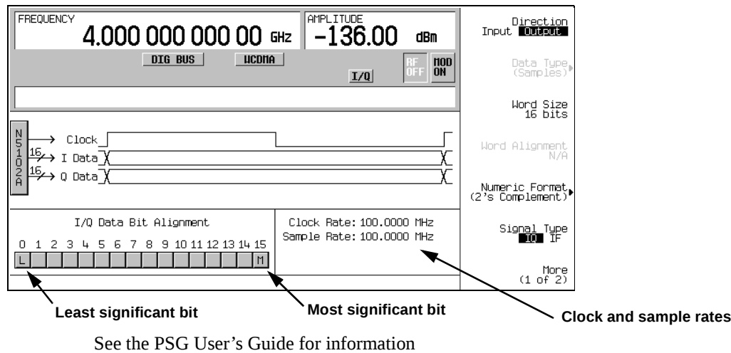
Figure 11-1 Data Setup Menu for a Parallel Port Configuration
