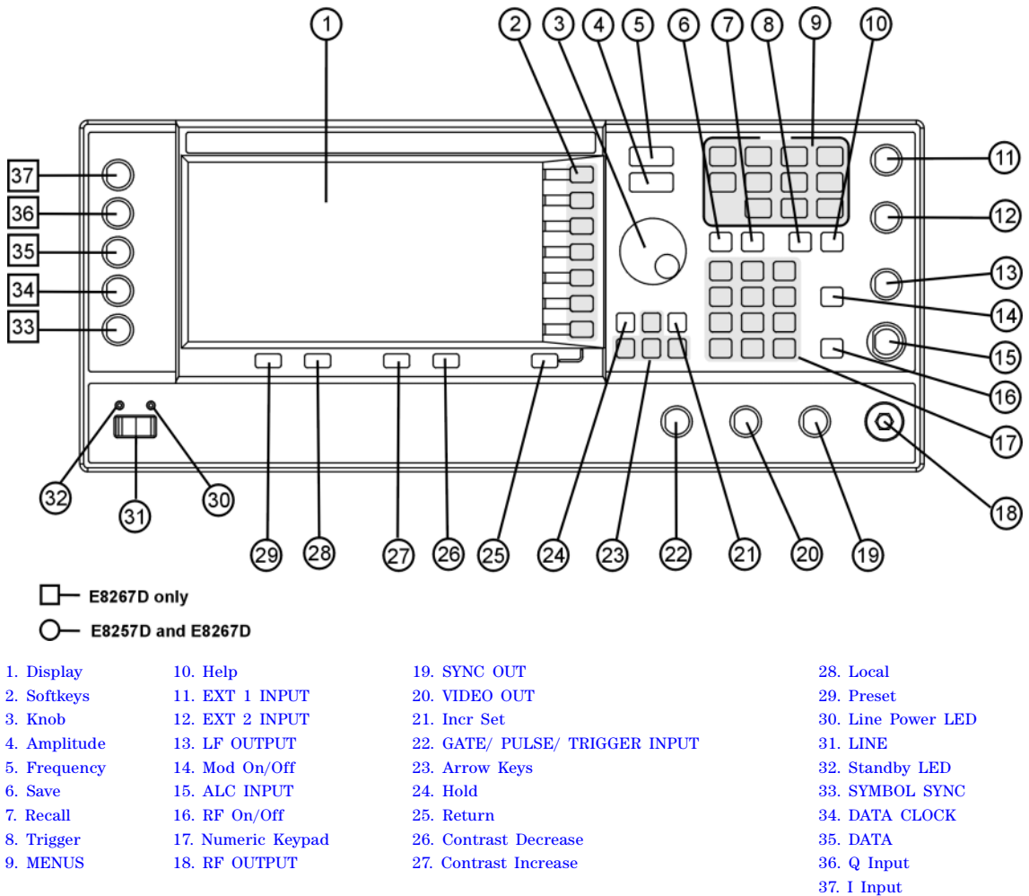
Figure 1-1 Standard E8267D Front Panel Diagram
