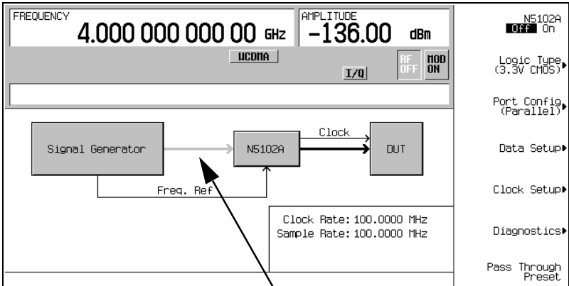
Figure 11-9 First-Level Softkey Menu
