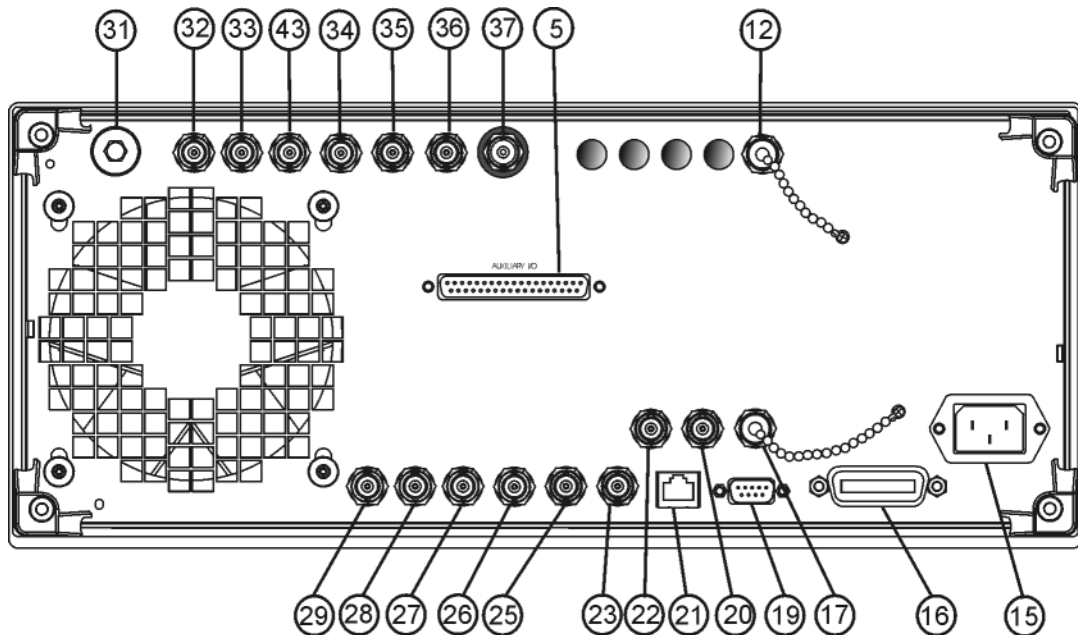
Figure 1-6 E8257D Option 1EM Rear Panel
