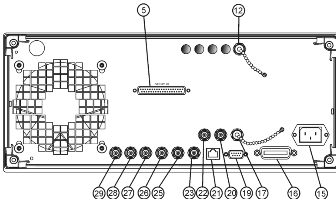
Figure 1-5 Standard E8257D Rear Panel
