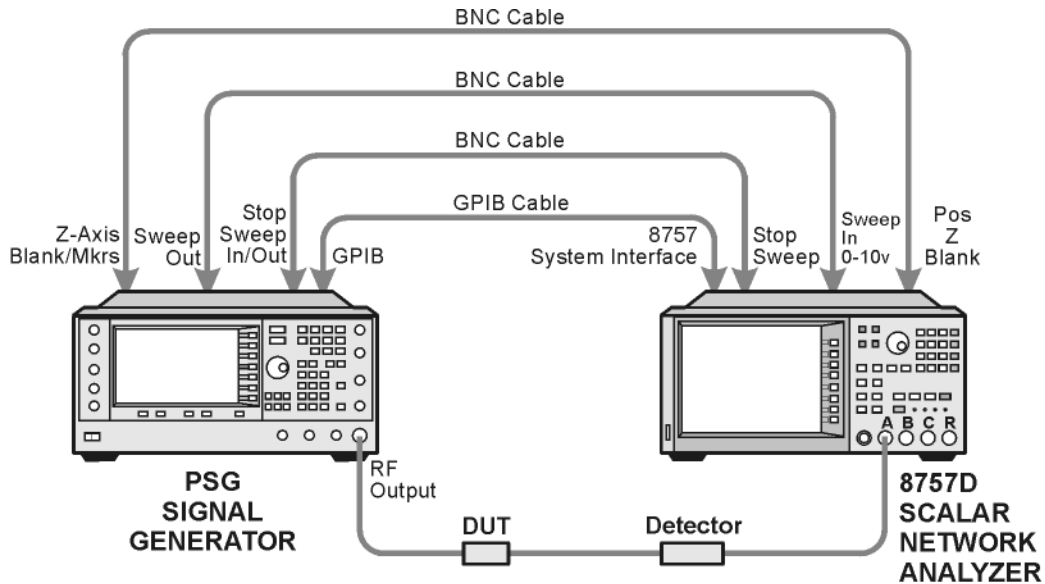
Figure 2-2 Equipment Setup
