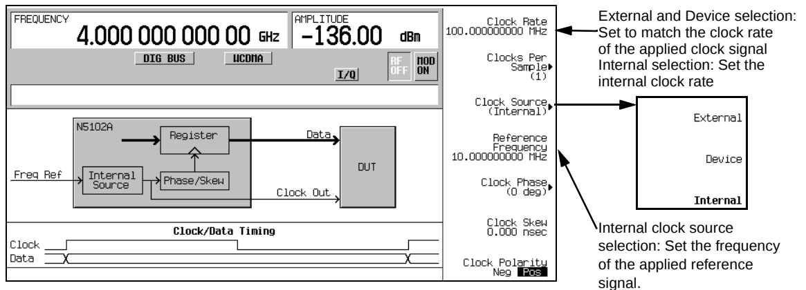
Figure 11-2 Clock Source Selection
