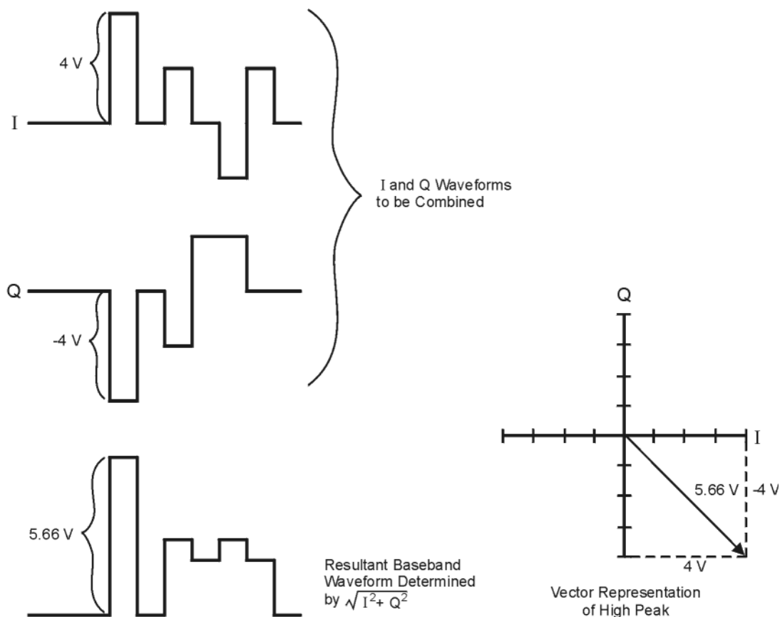
Figure 3-11 Combining the I and Q Waveforms
