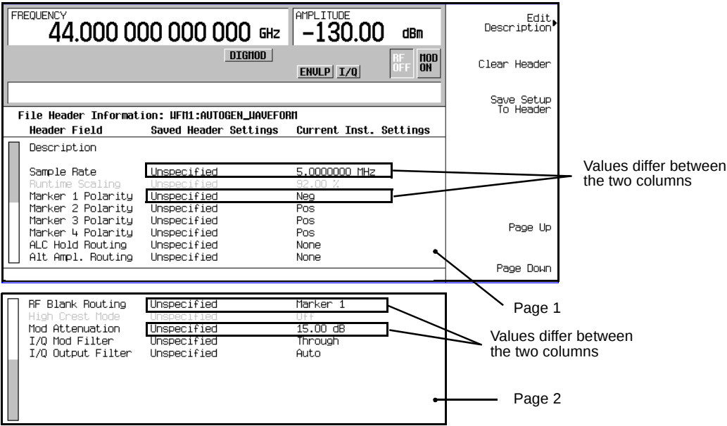
Figure 3-5 Saved File Header Changes
