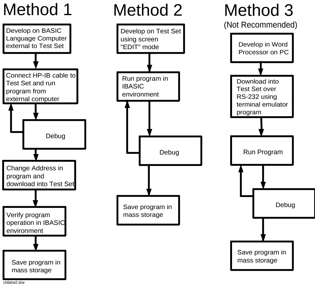
Figure 40 Three Possible Development Methods
