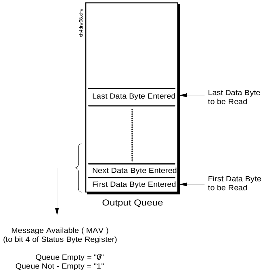
Output Queue Group
