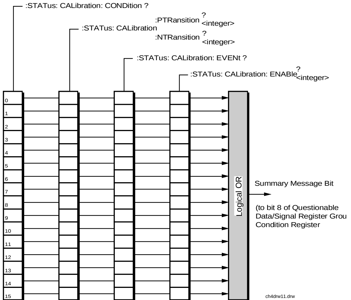
Figure 12 Calibration Status Register Group
