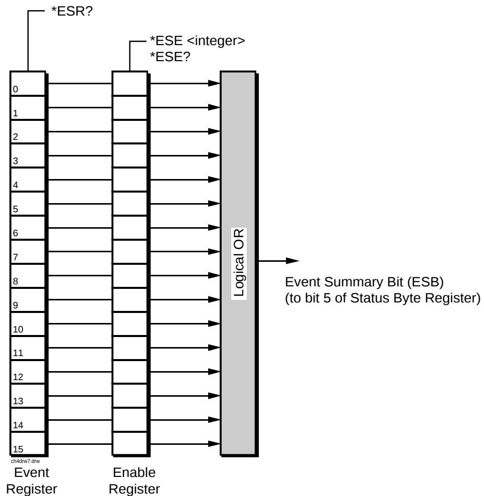
Standard Event Status Register Group
