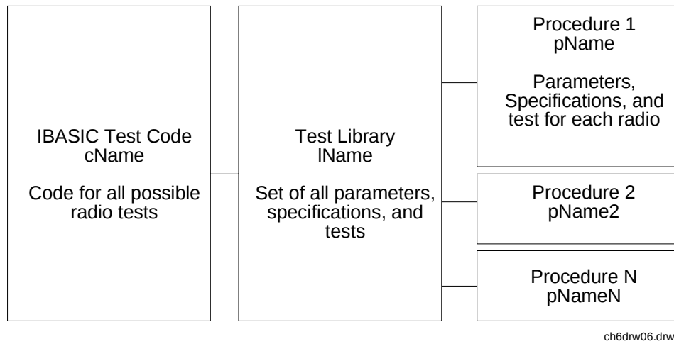
Figure 42 TESTS Subsystem File Relationship
