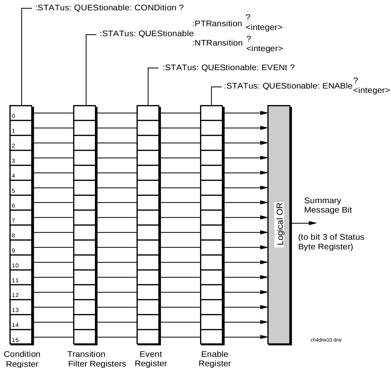
Figure 28 Questionable Data/Signal Register Group
