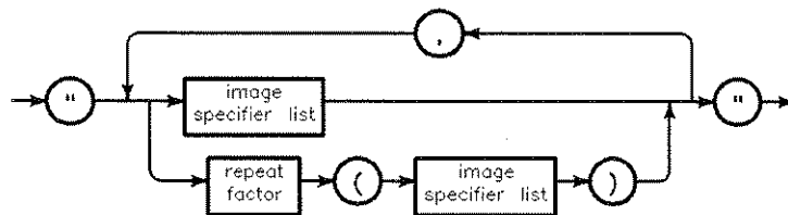
literal form of image specifier
