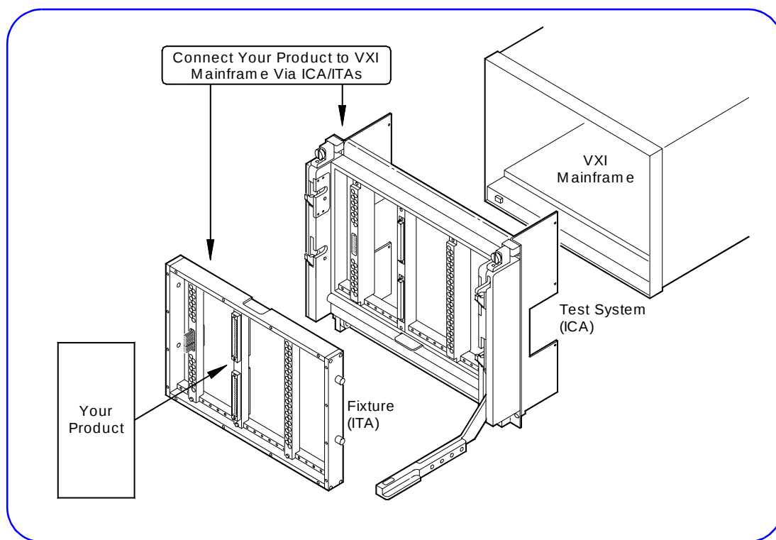
Figure 36. Typical Mass Interconnect Connections
